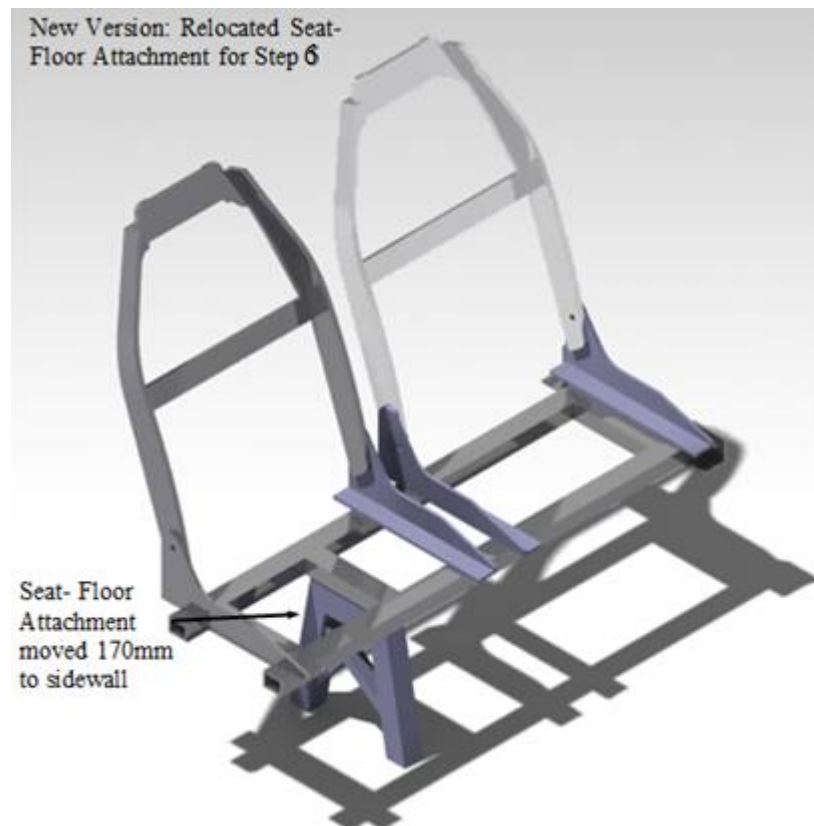
Figure 5.45. Seat Design
