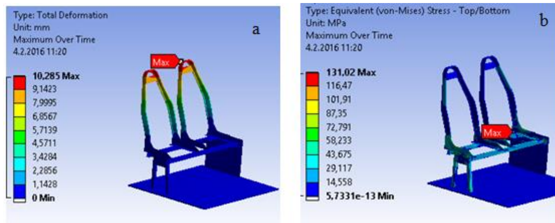
Figure 5.20. APTA &amp; ECE Regulation 80 Deceleration Analysis Results a) Total Deformation b) Maximum Equivalent Stress
