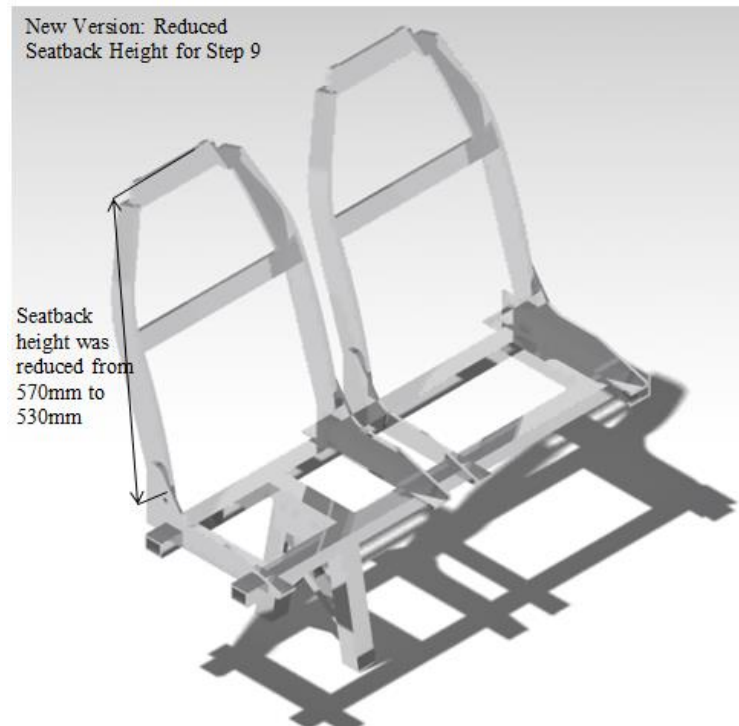
Figure 5.51. Seat Design
