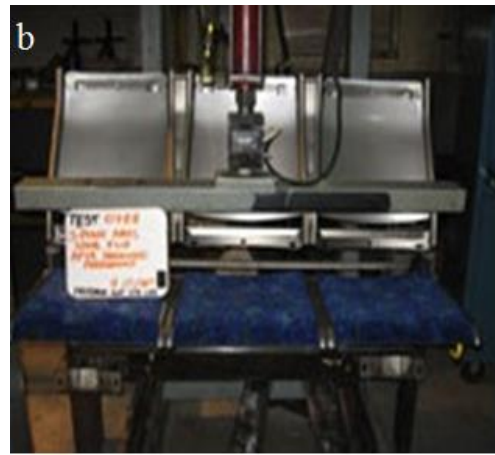
Figure 4.8. Actual APTA Seat Tests Photos a) APTA Horizontal Seatback Load Application b) APTA Vertical Force Application (Anonymous, 2016f)
