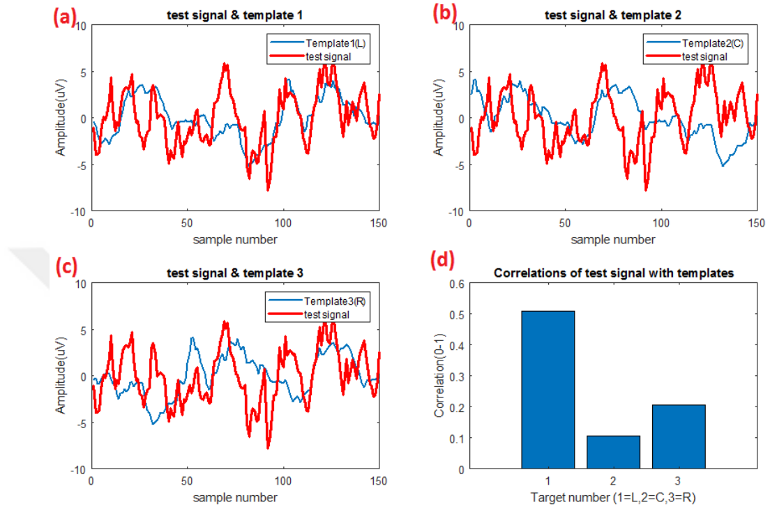
Figure 4.9: (a) The target template1 (blue) and the test signal (red)(b) The target template2 (blue) and the test signal (red)(c) The target template3 (blue) and the test signal (red) (d) The correlations of the test signal with the target templates
