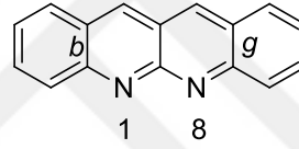
dibenzo[ b,g ][1,8]naftiridin
