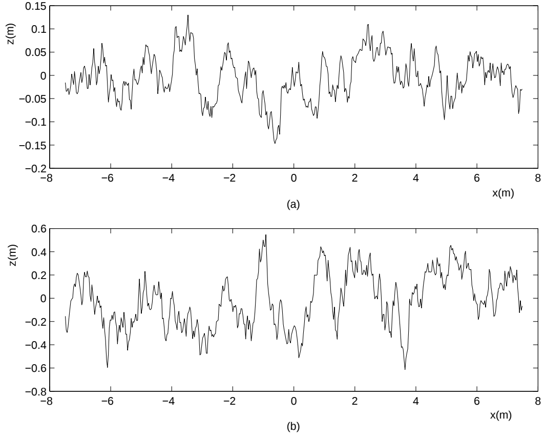
Figure 2.7: (a) Exponentially correlated moderately rough surface with \sigma = \lambda/6 , L_c = \lambda , so that the rms slope is = 13^\circ at 1 GHz (b) Exponentially correlated very rough surface with \sigma = 0.707\lambda , L_c = \lambda , so that the rms slope is = 45^\circ at 1 GHz
