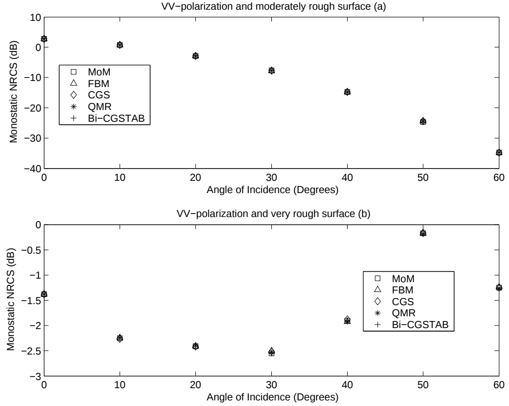
Figure 5.10: Comparison of the monostatic NRCS values for different iterative methods for Gaussian correlated rough profile with a dielectric constant, \epsilon_r = 15 - j4 for VV polarization at 1 GHz. (a) \sigma = \lambda/6 , rms slope = 13^\circ . (b) \sigma = 0.707\lambda , rms slope = 45^\circ .
