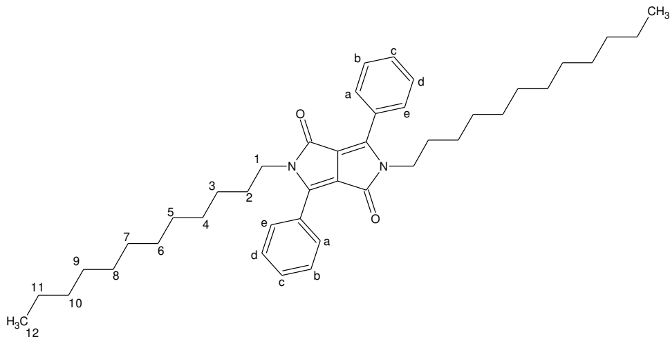
Şekil 3.80 3,6-difenil-2,5-didodesilpirolo[3,4-c]pirol-1,4-dion (Dodesil-DPP-Dodesil)
