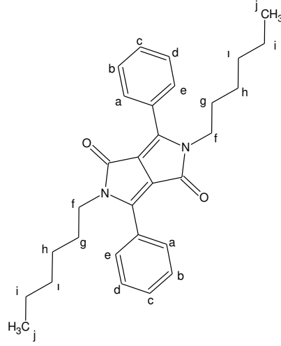
Şekil 3.73 3,6-difenil-2,5-dihekzilpirolo[3,4-c]pirol-1,4-dion (Hekzil-DPP-Hekzil)
