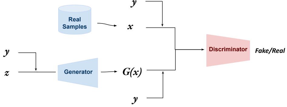
Figure 2.2: Overall architecture of Conditional Generative Adversarial Networks.
