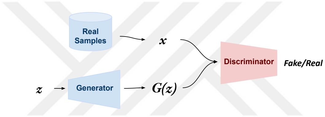
Figure 2.1: Overall architecture of Generative Adversarial Networks.
