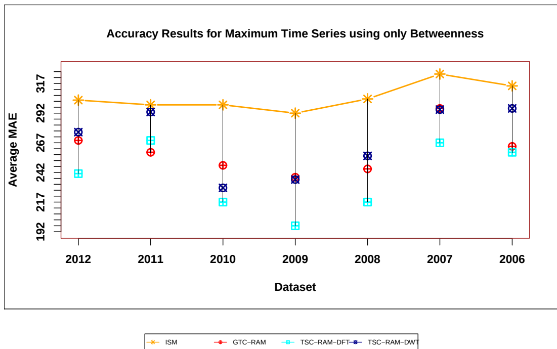
Figure 6.23: Performance of methods for maximum time series measured by MAE
