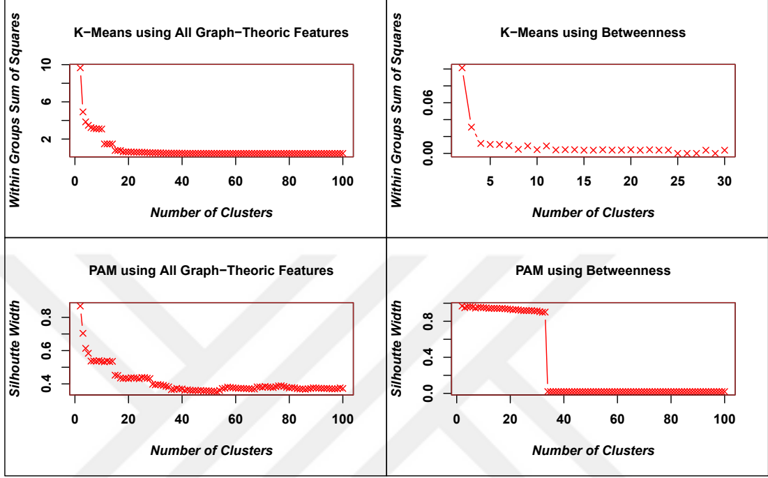
Figure 6.1: Cluster quality behavior changing according to number of clusters
