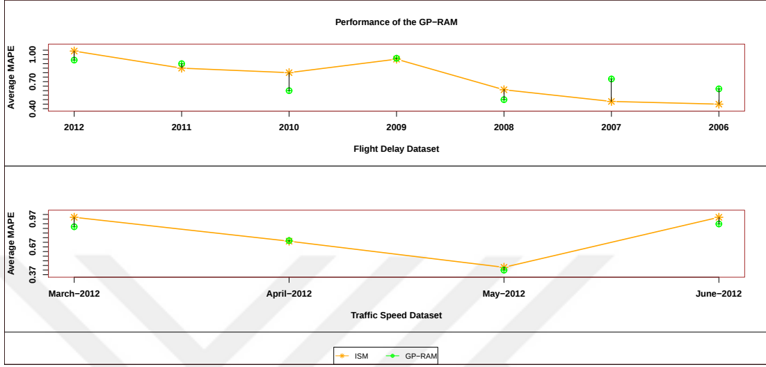
Figure 6.6: Comparison of GP-RAM with individual baseline model
