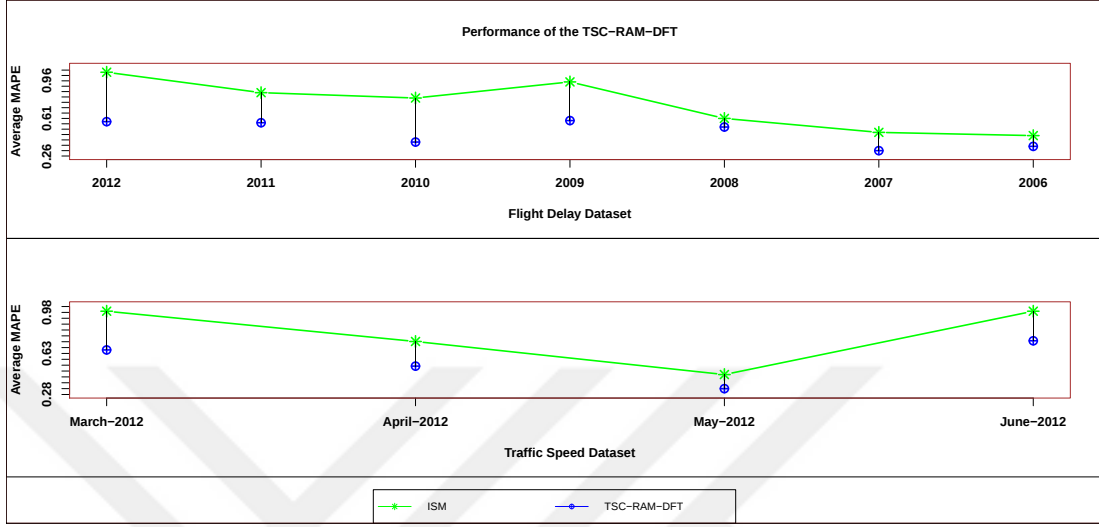
Figure 6.9: Comparison of TSC-RAM-DFT with individual baseline model
