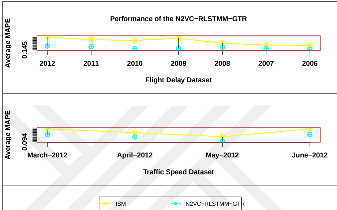
Figure 6.16: Comparison of N2VC-RLSTMM-GTR with individual baseline model
