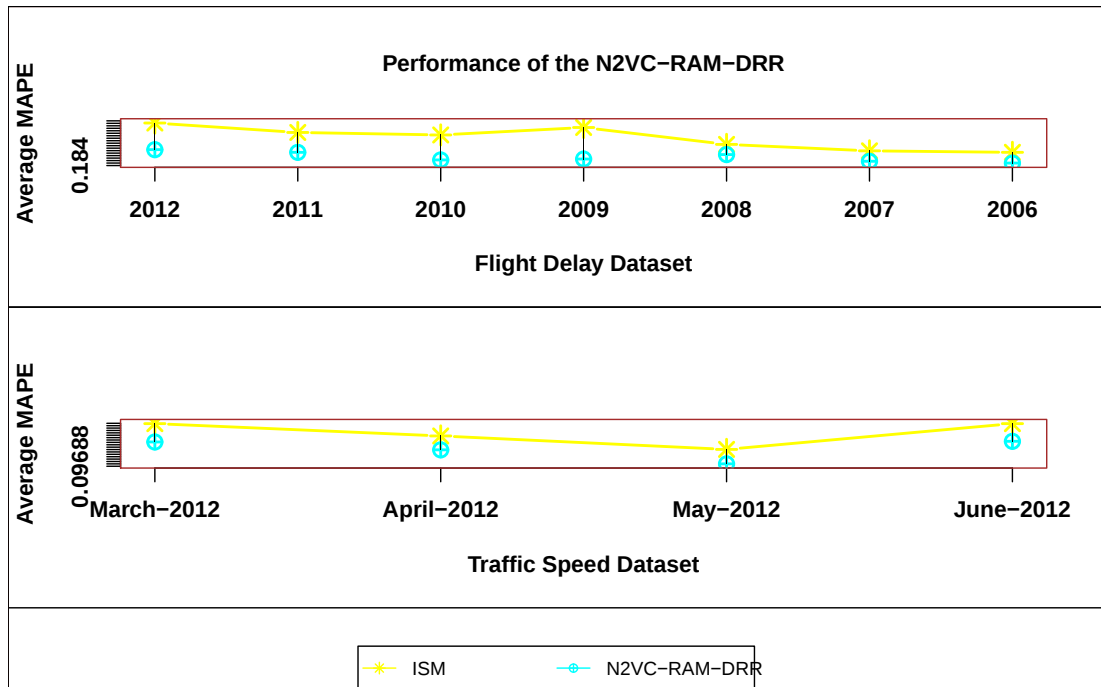
Figure 6.17: Comparison of N2VC-RAM-DRR with individual baseline model
