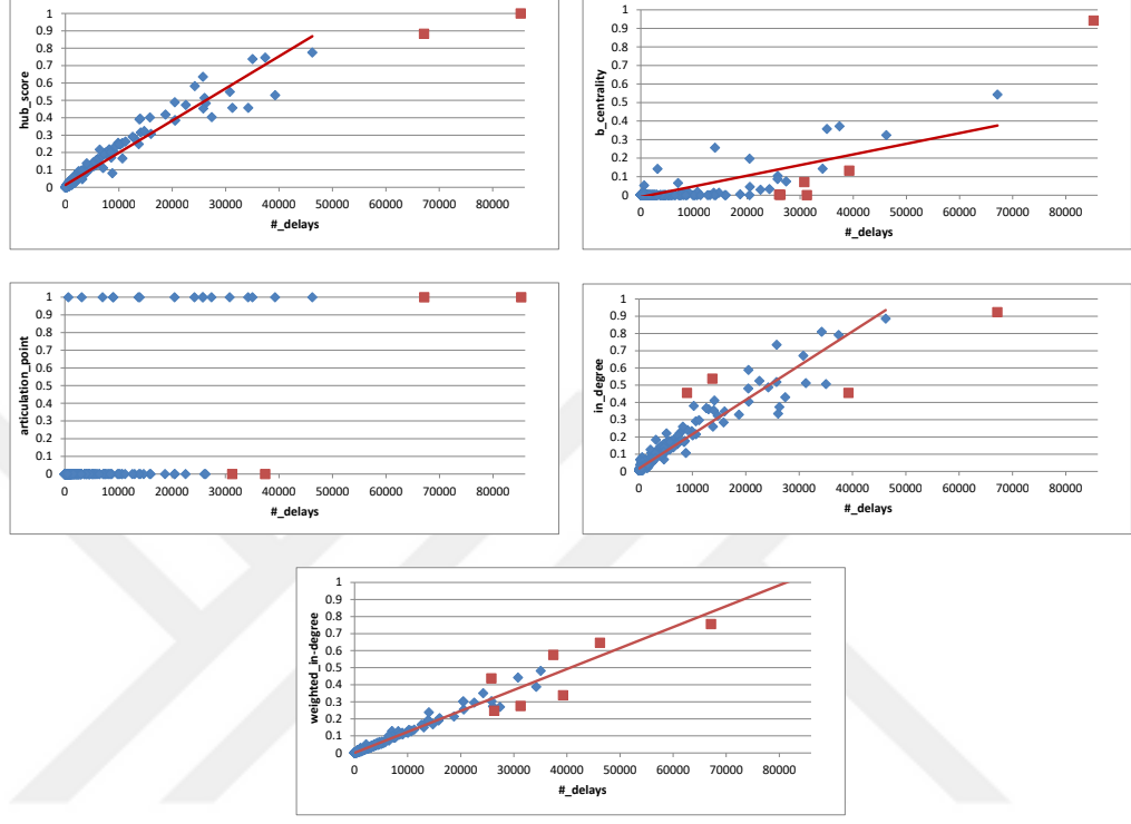
Figure 3.5: Graph-based scores vs. number of delays
