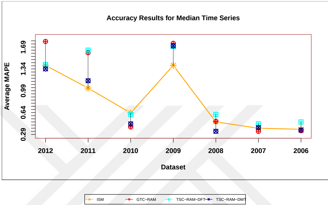
Figure 6.20: Accuracy comparison of proposed approaches using all features for median time series
