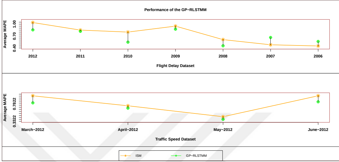
Figure 6.7: Comparison of GP-RLSTMM with individual baseline model
