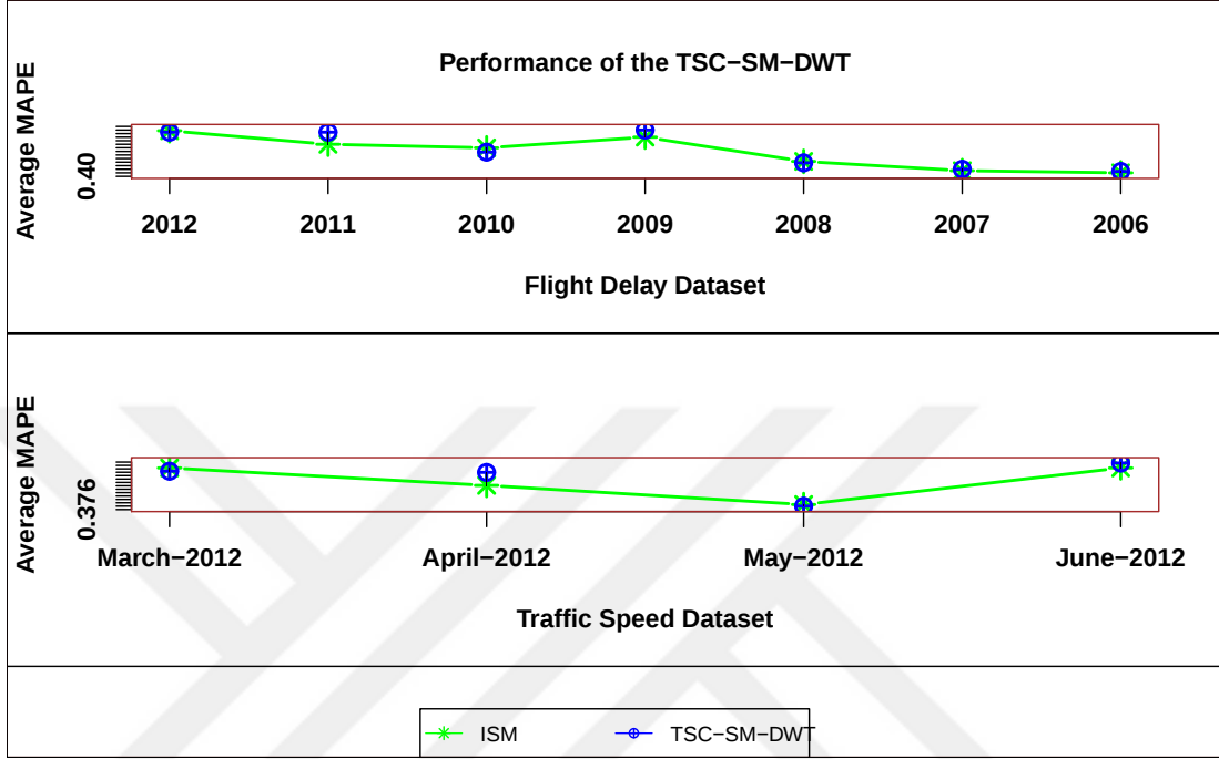
Figure 6.11: Comparison of TSC-SM-DWT with individual baseline model
