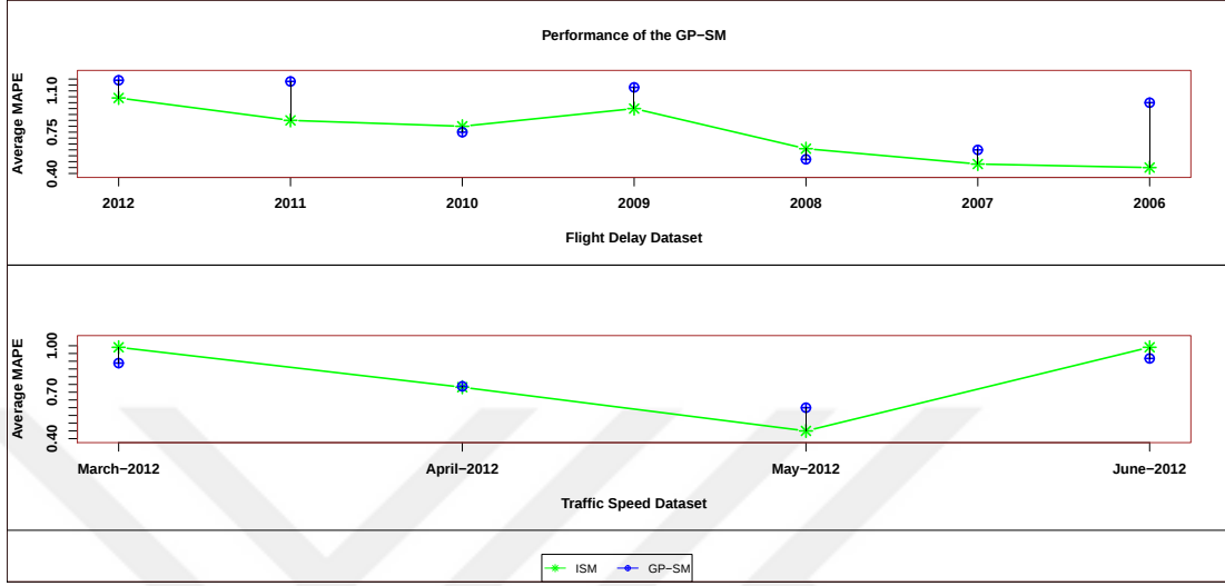
Figure 6.5: Comparison of GP-SM with individual baseline model
