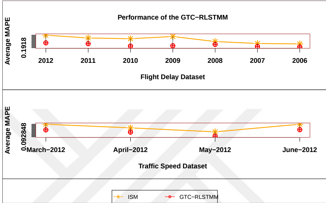
Figure 6.4: Comparison of GTC-RLSTMM with individual baseline model
