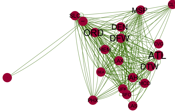
Figure 3.4: Top-20 airports with highest betweenness centrality scores
