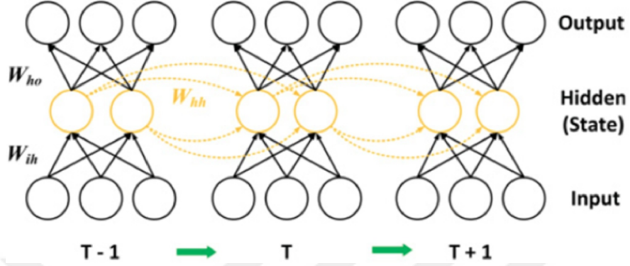
Figure 4.1: Time sequence processing in recurrent neural network
