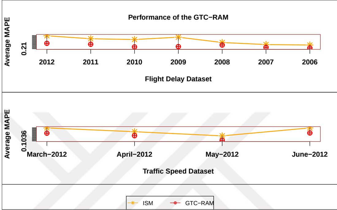
Figure 6.3: Comparison of GTC-RAM with individual baseline model
