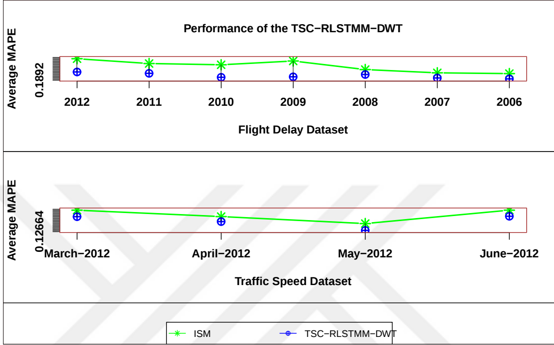
Figure 6.13: Comparison of TSC-RLSTMM-DWT with individual baseline model
