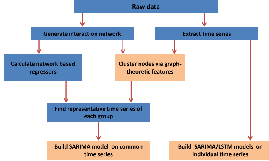
Figure 5.2: Flowchart of proposed GTC-SM
