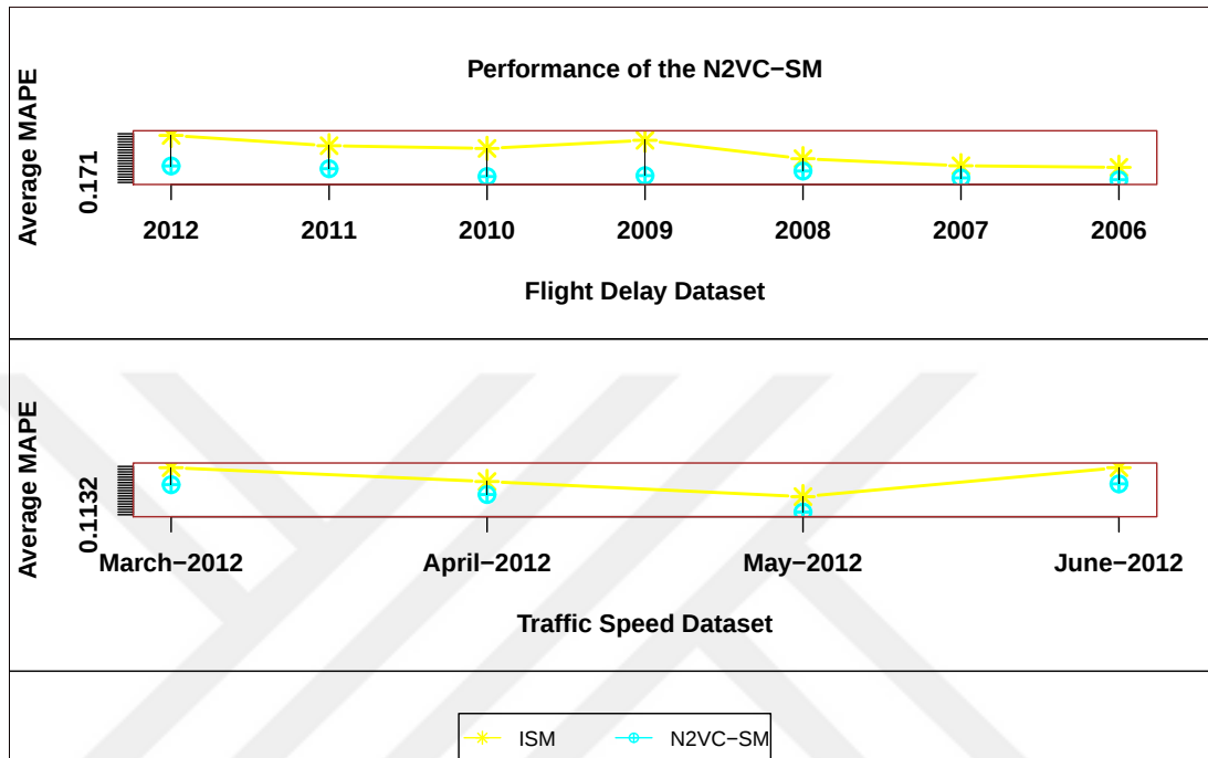
Figure 6.14: Comparison of N2VC-SM with individual baseline model
