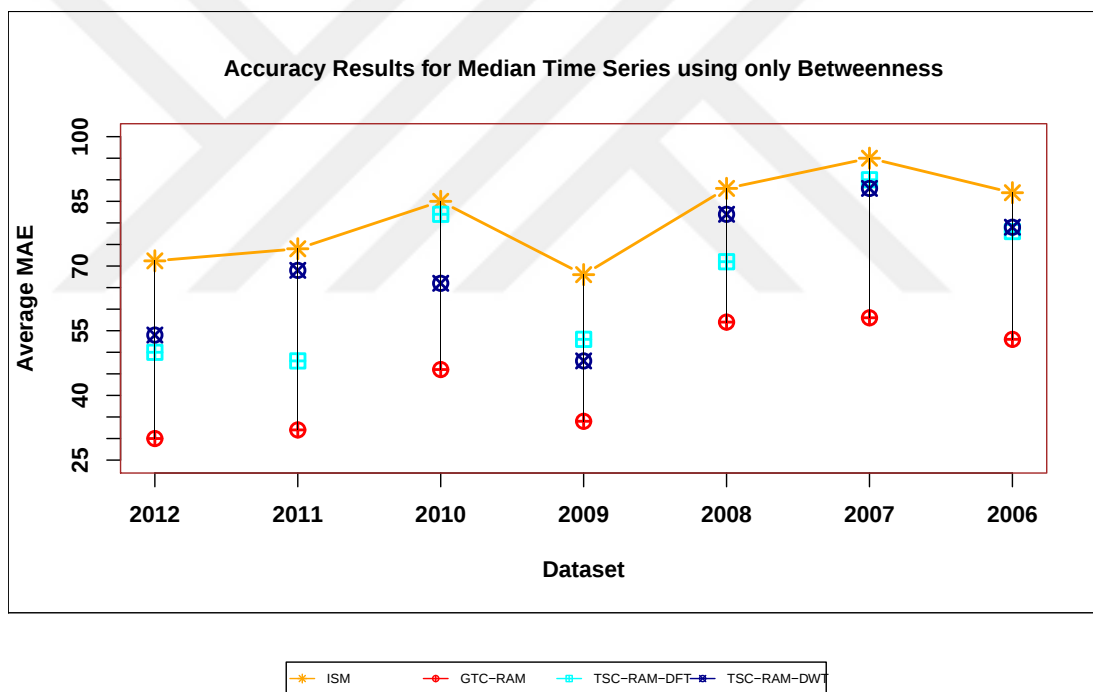
Figure 6.24: Performance of methods for median time series measured by MAE
