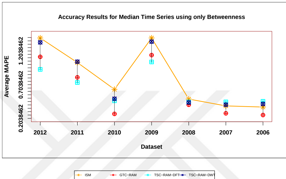
Figure 6.22: Effect of using only betweenness centrality feature on accuracy for median time series
