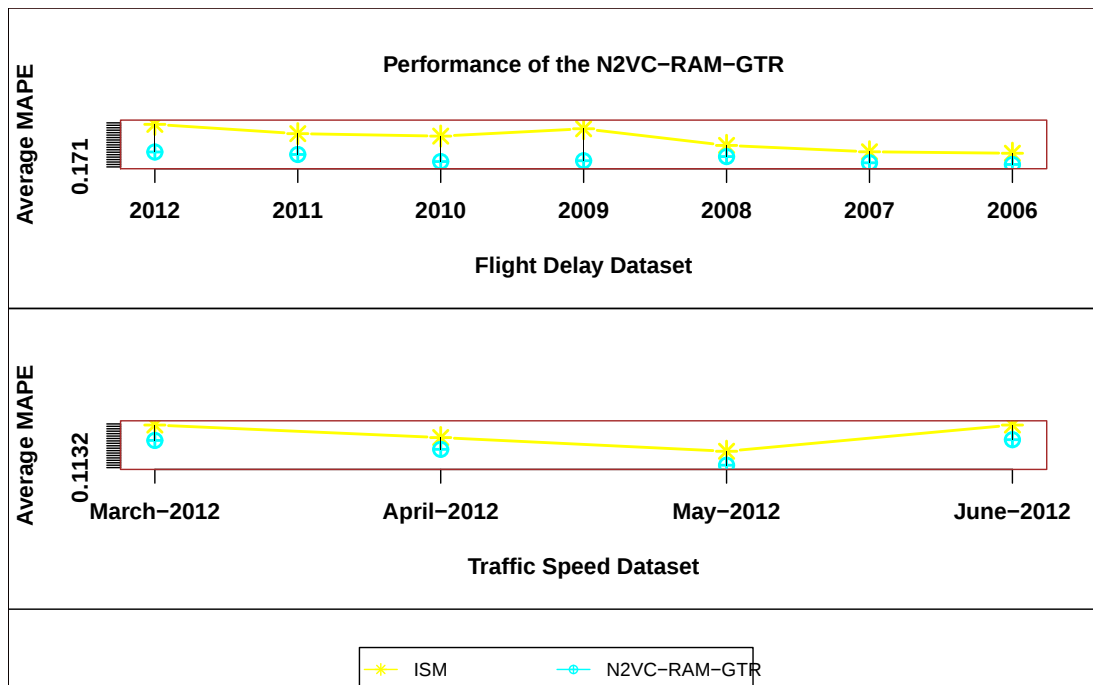
Figure 6.15: Comparison of N2VC-RAM-GTR with individual baseline model
