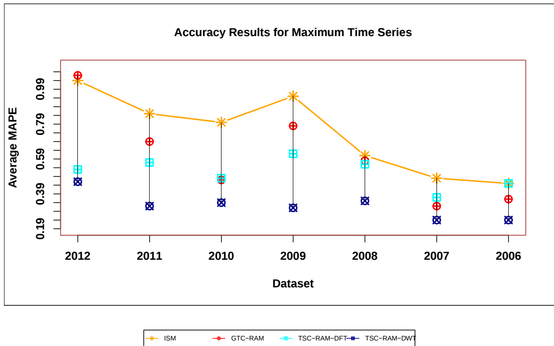
Figure 6.19: Accuracy comparison of proposed approaches using all features for maximum time series
