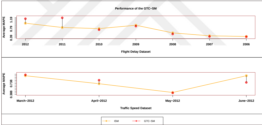
Figure 6.2: Comparison of GTC-SM with individual baseline model
