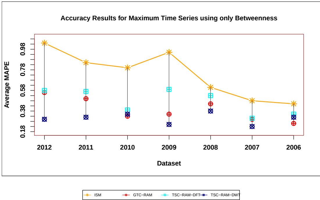
Figure 6.21: Effect of using only betweenness centrality feature on accuracy for maximum time series
