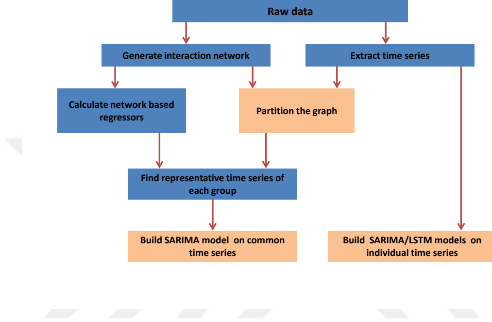
Figure 5.5: Flowchart of proposed GP-SM
