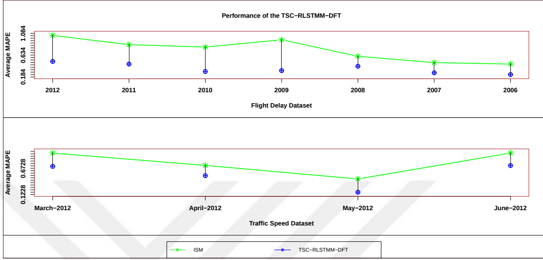
Figure 6.10: Comparison of TSC-RLSTMM-DFT with individual baseline model
