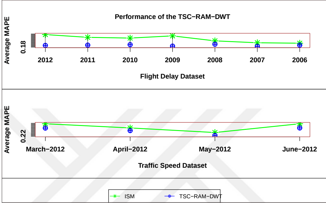
Figure 6.12: Comparison of TSC-RAM-DWT with individual baseline model
