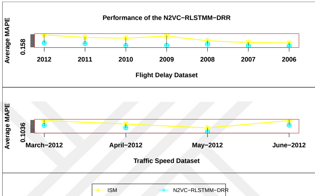
Figure 6.18: Comparison of N2VC-RLSTMM-DRR with individual baseline model
