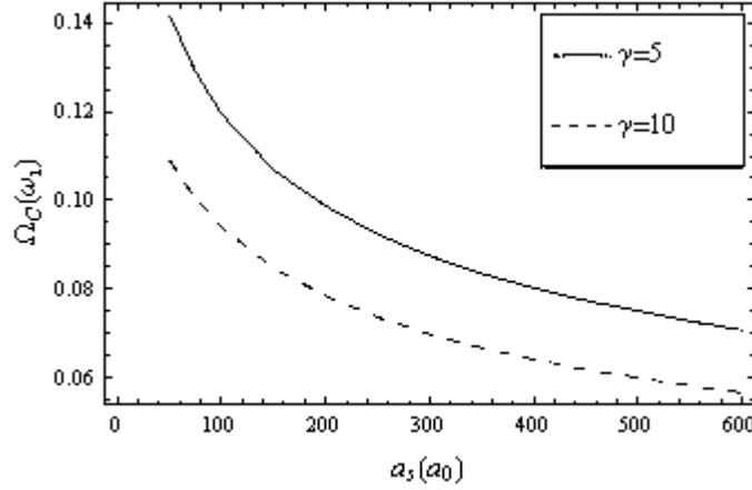
Fig. 5.7. The critical angular velocity of a condensate with a vortex for \gamma = 5 and \gamma = 10 as a function of the scattering length. \Omega_C is measured in units of \omega_\perp .
