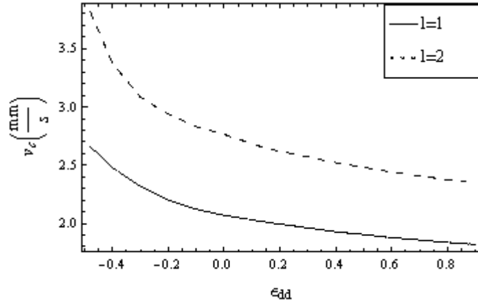
Fig. 5.9. The critical velocity, v_c (mm/s), for d = 1 in units of h.o.u. as a function of \epsilon_{dd} for an oblate trap. The solid (dashed) curve is for singly (doubly) quantized vortex dipole, and \gamma = 5 .
