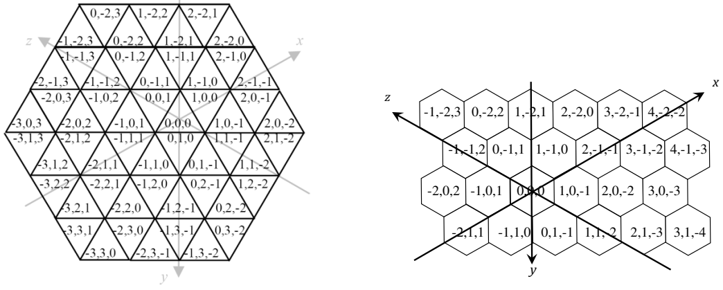
Figure 2.2: The triplet coordinate system for the triangular grid (left) and the hexagonal grid (right).
