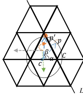
Figure 3.14: Blue point c indicates the center of the rotation where the orange point p and p' indicate the center of the right neighbor pixel and its image after rotation, respectively.
