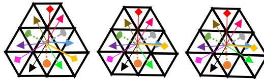
Figure 3.15: The first 3 neighborhood motion maps of rotations centered at the left edge midpoint of an even triangle with 12-neighbors.
