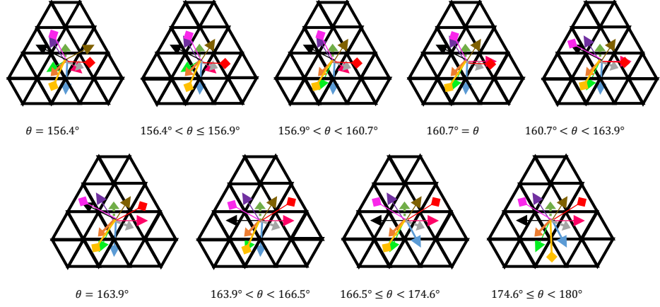
Figure 3.13: Neighborhood motion maps for rotation around lower edge midpoint.
