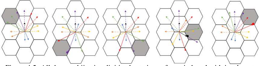
Figure 4.5: All the non-bijective digitized rotations of a main hexel with its closest neighbors on the hexagonal grid, when the center of rotation is the lower edge midpoint.
