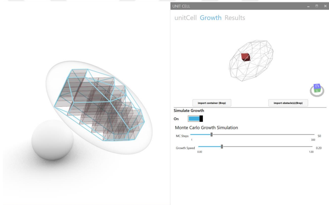
Figure 4.6. Growth tab of the computational model developed by author
