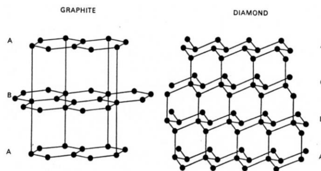
Figure 4.17. Crystal structure of graphite and diamond (Mallika, DeVries and Komanduri 1999)
