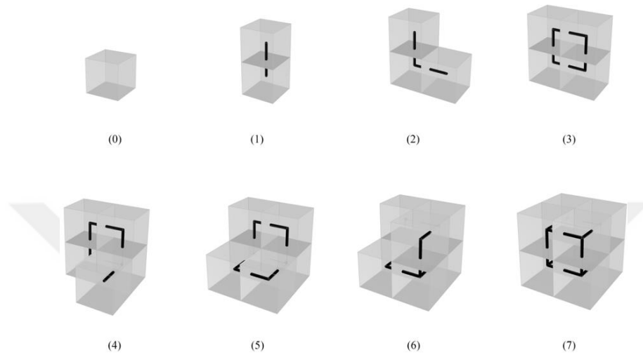
Figure 4.12. Sequential growth process of crystal formation as a result of proposed growth mechanism
