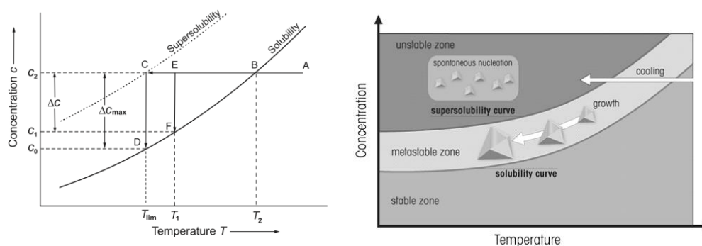
Figure 3.20. The relation between temperature and concentration during cooling (retrieved from https://syrris.co.jp/applications/what-is-crystallization-and-what-are-the-methods-of-crystallization/ on 15.11.2020)
