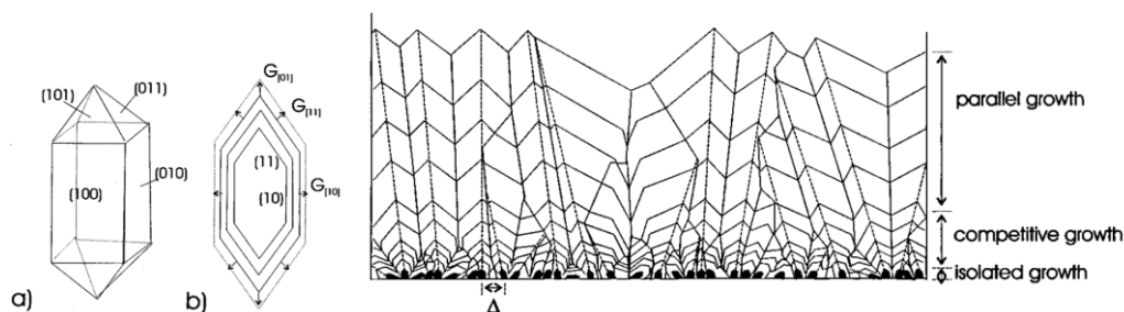
Figure 4.27. (1) Schematic single crystal growth and (2) Simulation of crystal growth starting with 35 crystals (Garcia-Ruiz and Garcia-Ruiz 2002)
