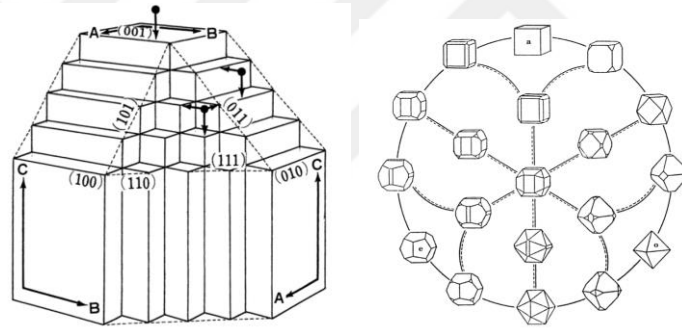
Figure 3.17. (a) F (flat), S (stepped) and K (kinked) faces based on Hartman and Perdok’s Periodic Bond Chain (PBC) analysis, (b) Tracht variation of pyrite crystals (Sunagawa 2005)
