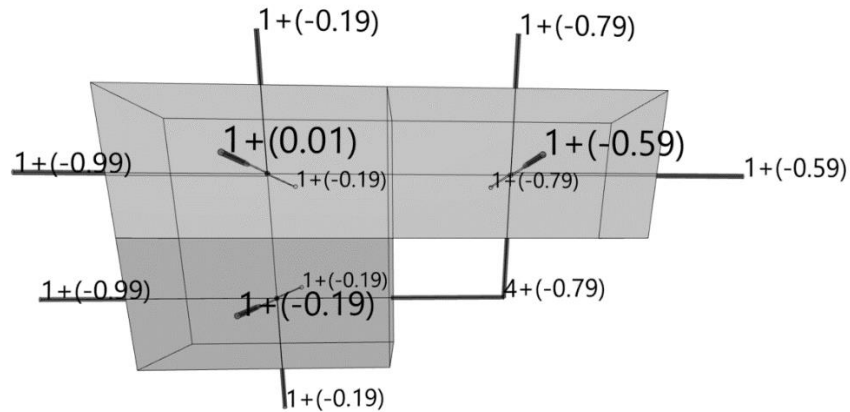
Figure 4.8. Score calculation of growth algorithm proposed by author
