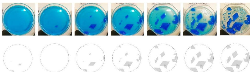
Figure 3.23. Deciphering the record of Chalcantite crystal growth
