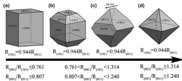
Figure 3.18. Morphological evolution of Al 6 Mn IMCs dependent on the growth-rate ratios of (001), (011), and (101) planes (a)–(d).
