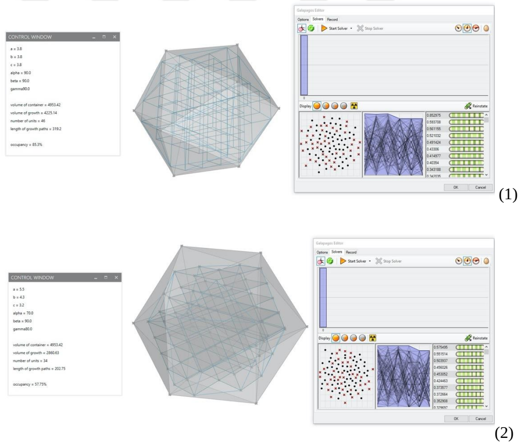
Figure 4.31. Two different runs of algorithm started with different initial variables: (1) started with benchmark module, (2) started with 90^{\circ}90^{\circ}120^{\circ} degrees module
