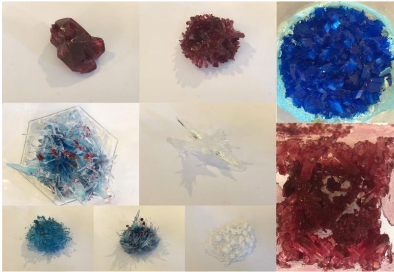
Figure 3.19. Potassium sulfate crystals are produced as initial observations
