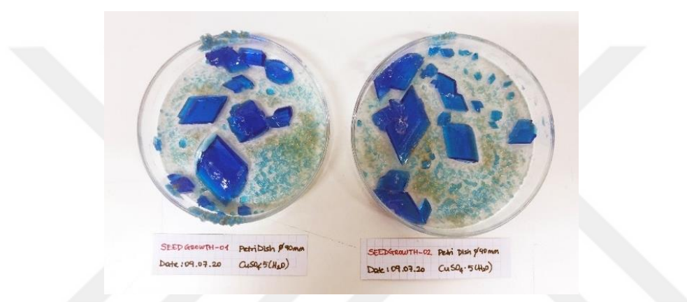
Figure 3.22. Growth of Chalcantite ( \text{CuSO}_4 \cdot 5\text{H}_2\text{O} ) Crystals
