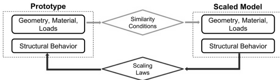
Figure 3.10. Conceptual diagram for prototype and scaled model. (Coutinho 2017)
