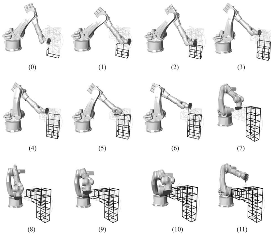
Figure 4.14. Generated path for robotic additive manufacturing process computed within the model designed by author
