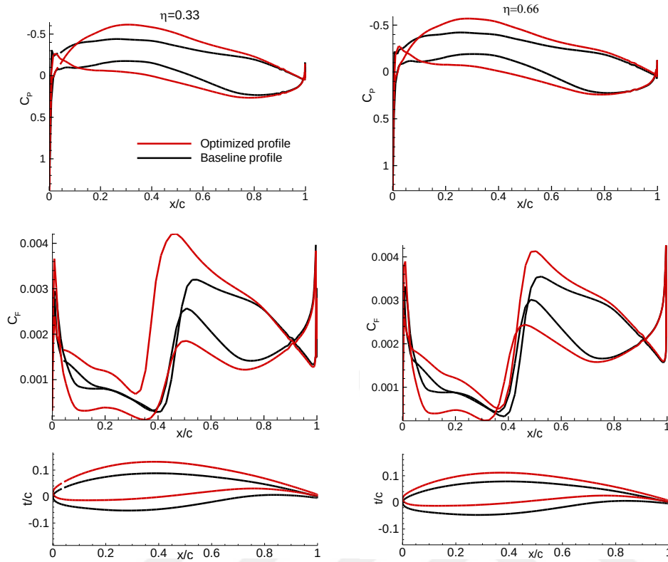
Figure 3-50 The wing sections of the baseline wing and the optimized wing
