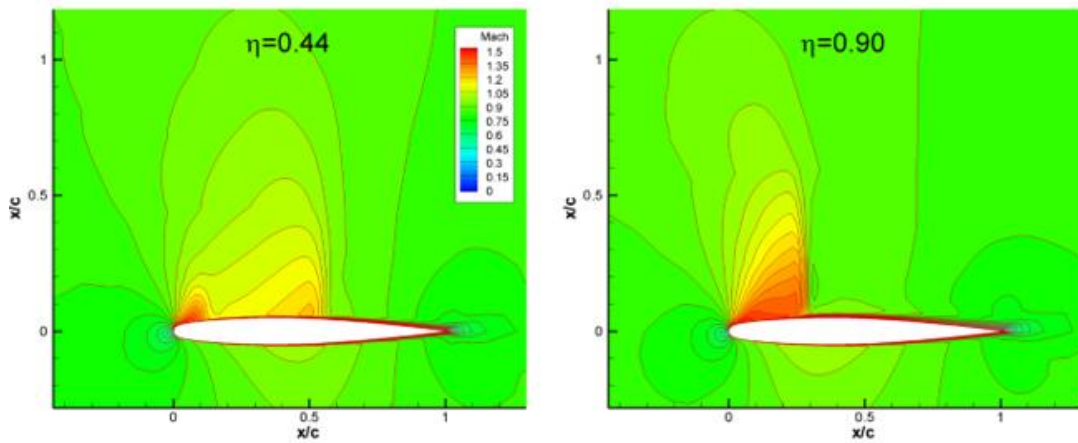
Figure 3-14 Mach contours
