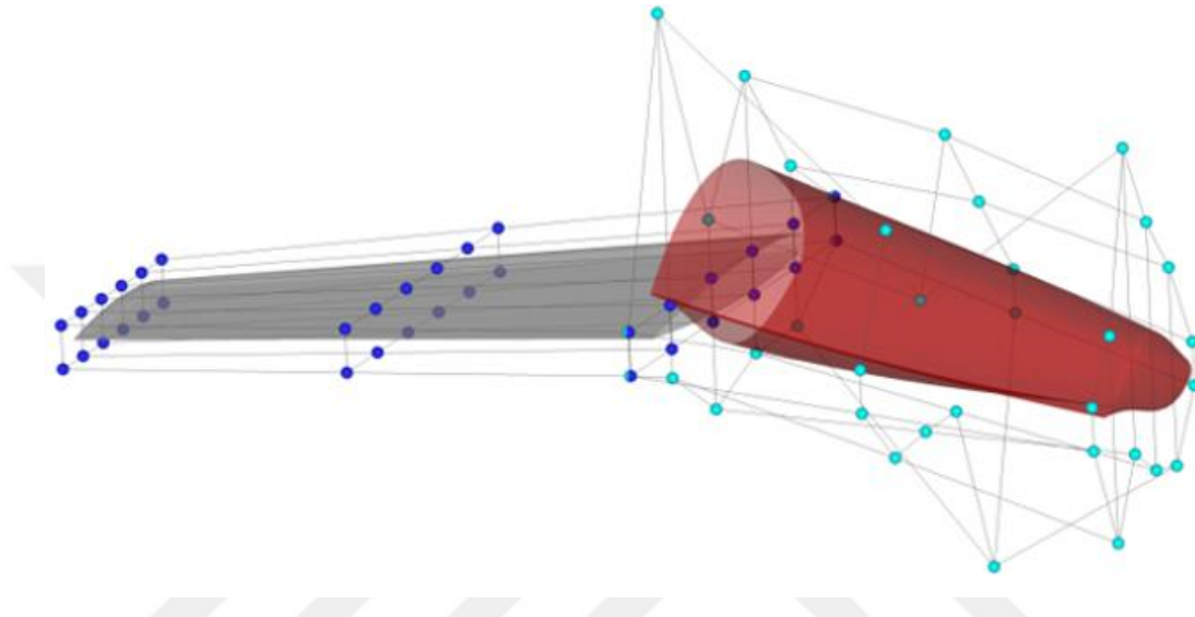
Figure 2-8 A sample deformation carried out by SU2_DEF employing FFD approach
