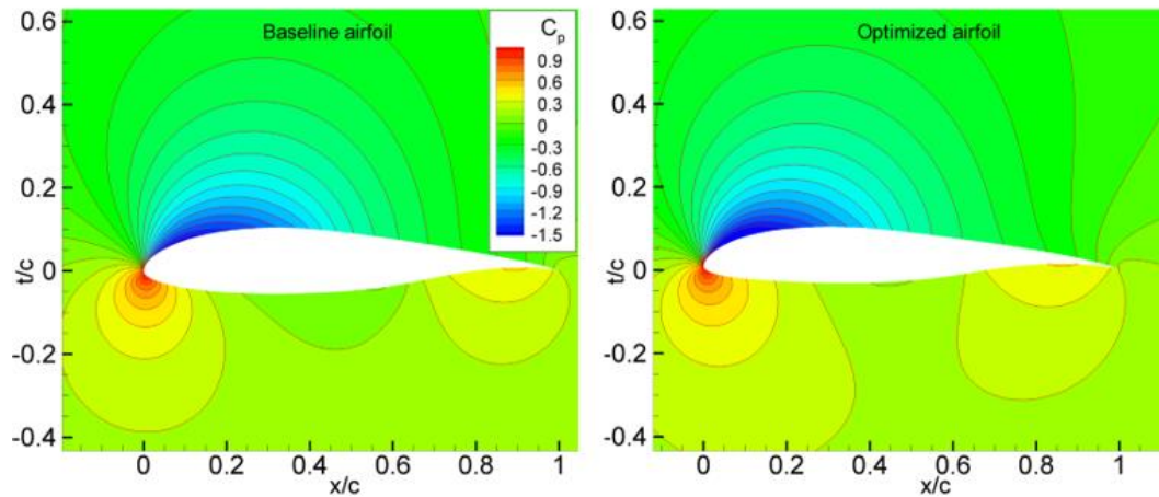
Figure 3-41 Pressure coefficient distributions on the baseline and optimized airfoils
