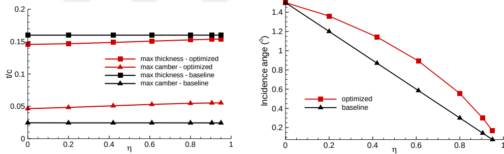
Figure 3-53 Maximum thickness and maximum camber to chord ratio distribution on the baseline and optimized wing along the span
