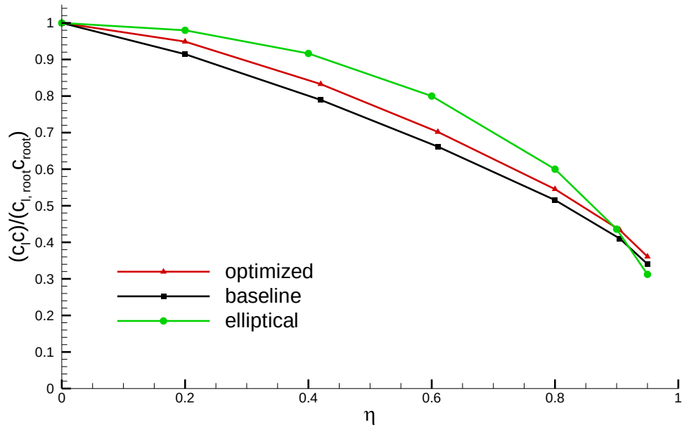
Figure 3-54 The lift distribution along the span
