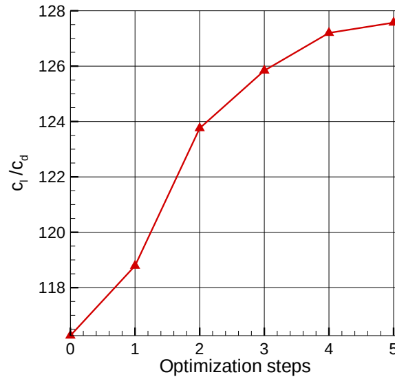
Figure 3-39 Evolution of c_l/c_d along the optimization steps
