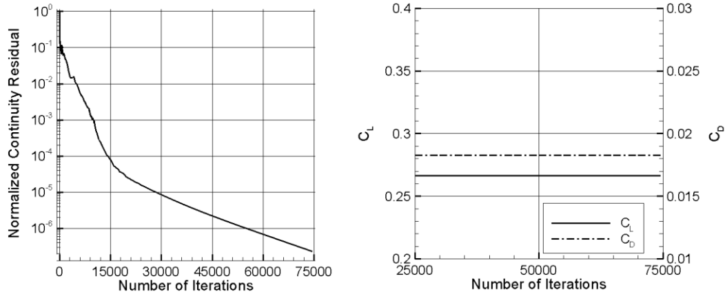
Figure 3-15 Convergence history for ONERA M6 analysis
