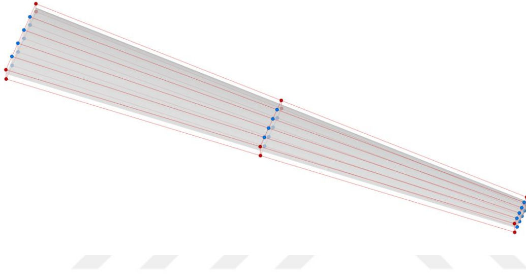
Figure 3-33 FFD box and control points (blue spheres depict active control points)
