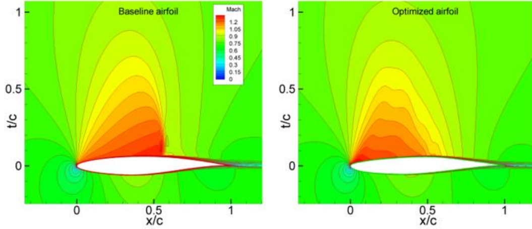
Figure 3-38 Mach distributions
