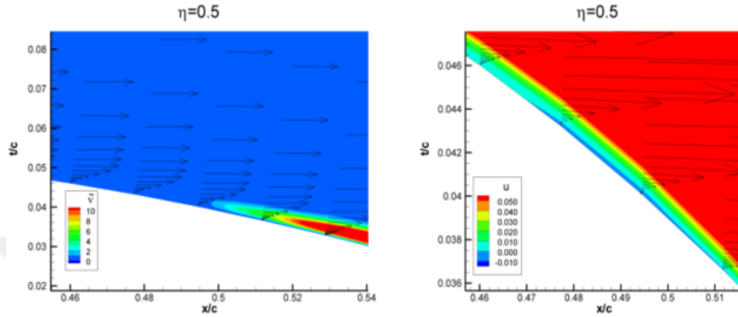
Figure 3-23 The turbulent working variable \tilde{\nu} and x-velocity u distribution at the midspan wing section
