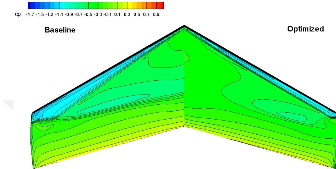
Figure 3-45 Pressure coefficients for baseline geometry and optimized geometry Reducing the maximum thickness and incidence angles of the wing sections resulted in that the aft shock is either removed or weakened along the spanwise (Figure 3-44, Figure 3-45). Furthermore, the lift decrease due to the reduction of the incidence angle has been compensated by alleviating the lift loss occurring due to shock.
