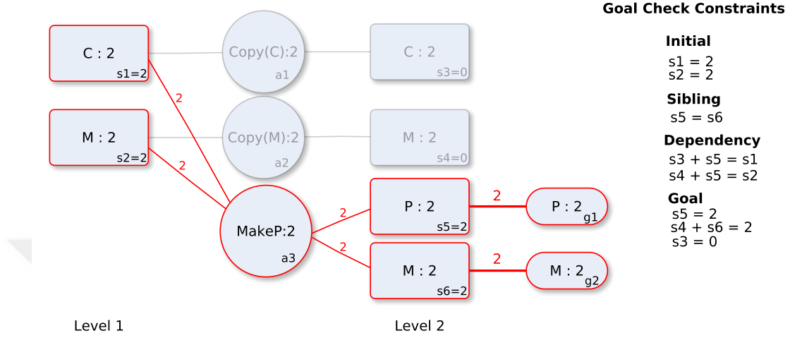
Figure 5.7: Final state of the LinGraph for the planning problem of (5.10), showing all constraints used for the last successful goal check step with all goals satisfied.
