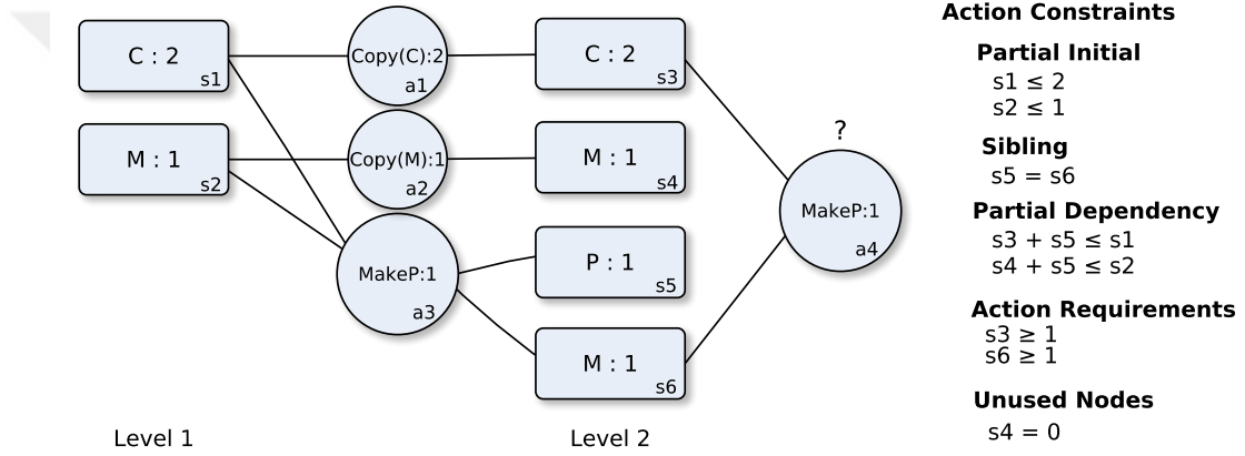
Figure 5.8: LinGraph expansion step checking for feasibility of a new instance of the MakeP action through action constraints .
