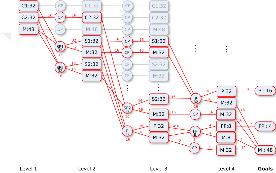
Figure 5.13: Final LinGraph for the complex assembly planning example of (5.13). Some actions and nodes for levels larger than 2 were omitted for visual clarity. Nodes that are part of the final plan are shown in red.
