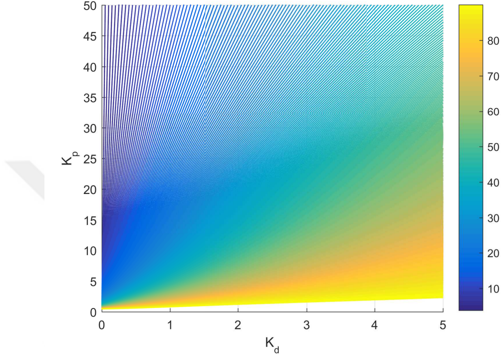
Figure 4.25: Phase margin of closed loop stable Mathieu system with respect to K_p and K_d values.
