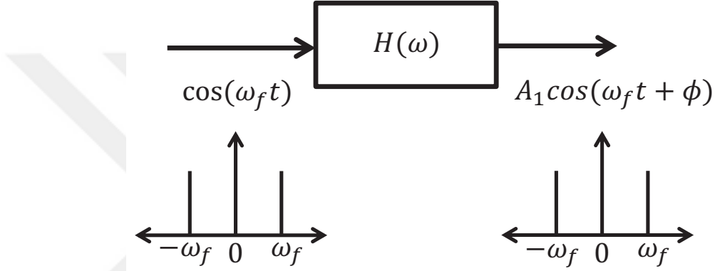
Figure 3.2: Input-output relation of LTI systems when single cosine signal is applied
