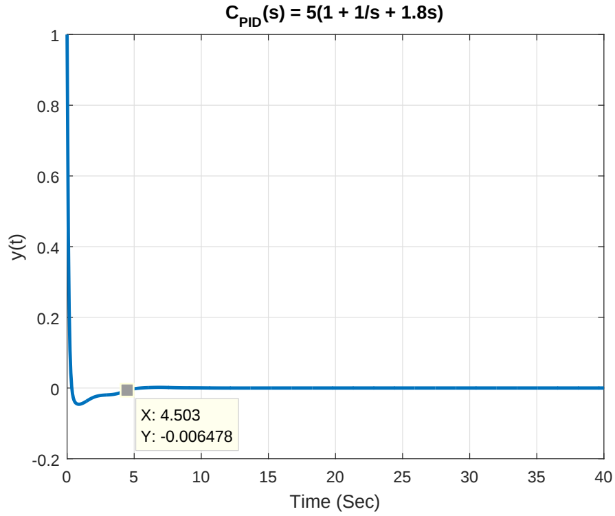
Figure 4.20: Output response of LTP System with C_{PID} = 5(1 + \frac{1}{s} + 1.8s) .
