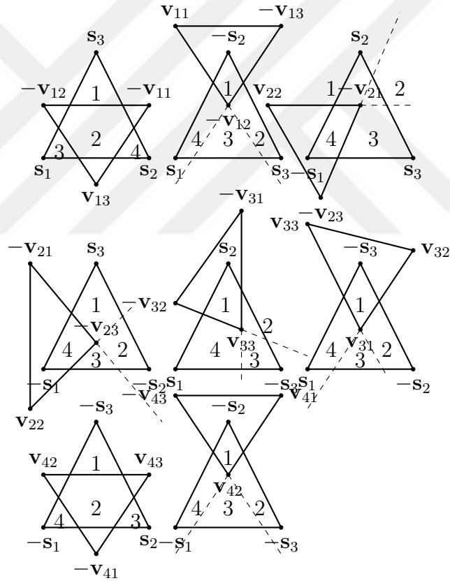
Figure 4.5: Positions of the \text{cone}\{\mathbf{v}_{i1}, \mathbf{v}_{i2}, \mathbf{v}_{i3}\} relative to \text{cone}\{\mathbf{s}_{i1}, \mathbf{s}_{i2}, \mathbf{s}_{i3}\} .
