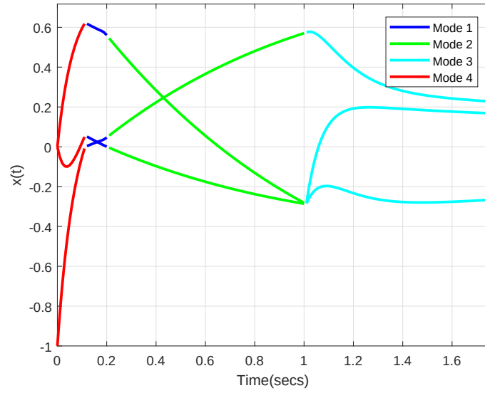
Figure 3.15: State trajectories for GAS CLS (zoomed).
