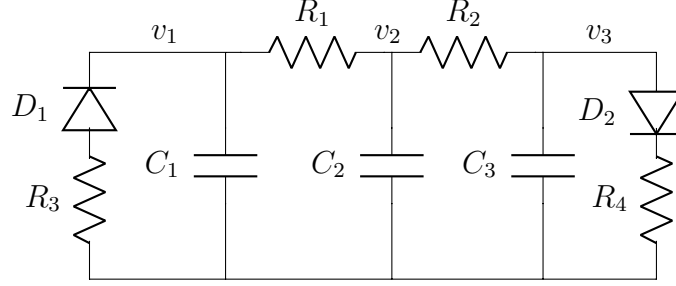
Figure 4.1: RC circuit with ideal diodes.
