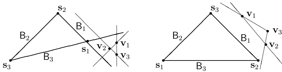
Figure 3.4: Two mutually exclusive \mathbf{S} and cone \{\mathbf{v}_1, \mathbf{v}_2, \mathbf{v}_3\} cases with sign patterns of CV , WS matrices.
