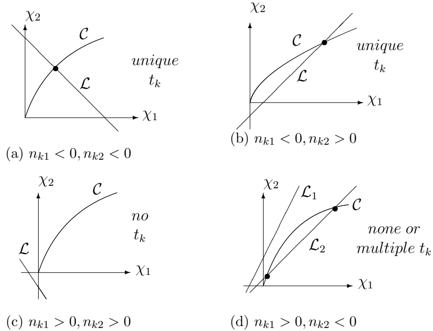
Figure 3.3: Existence of t_k when \mathbf{c}_k^T \mathbf{b} > 0 .
