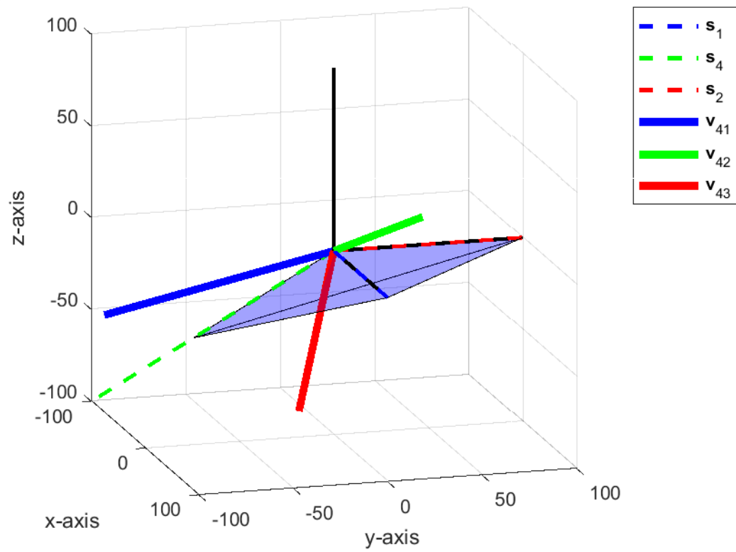
Figure 3.12: Position of the \text{cone}\{v_{41}, v_{42}, v_{43}\} relative to \text{cone}\{s_1, s_4, s_2\} for the source in 3D.
