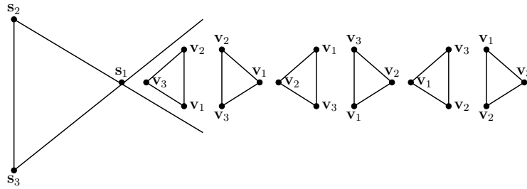
Figure 3.8: Further mutually exclusive orientations of the cone\{\mathbf{v}_1, \mathbf{v}_2, \mathbf{v}_3\} relative to cone\{\mathbf{s}_1, \mathbf{s}_2, \mathbf{s}_3\} . Third and fourth configurations are not structural but the others are structurally one or two-transitive.
