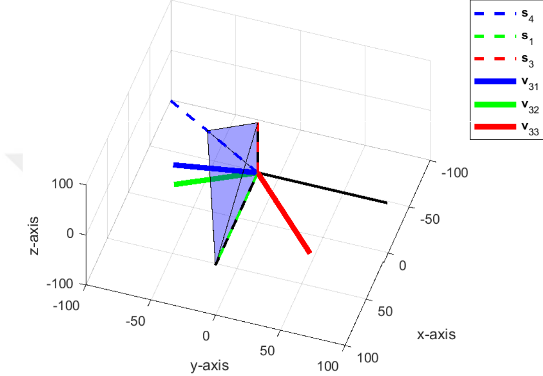
Figure 3.11: Position of the \text{cone}\{\mathbf{v}_{31}, \mathbf{v}_{32}, \mathbf{v}_{33}\} relative to \text{cone}\{\mathbf{s}_4, \mathbf{s}_1, \mathbf{s}_3\} for the sink in 3D.
