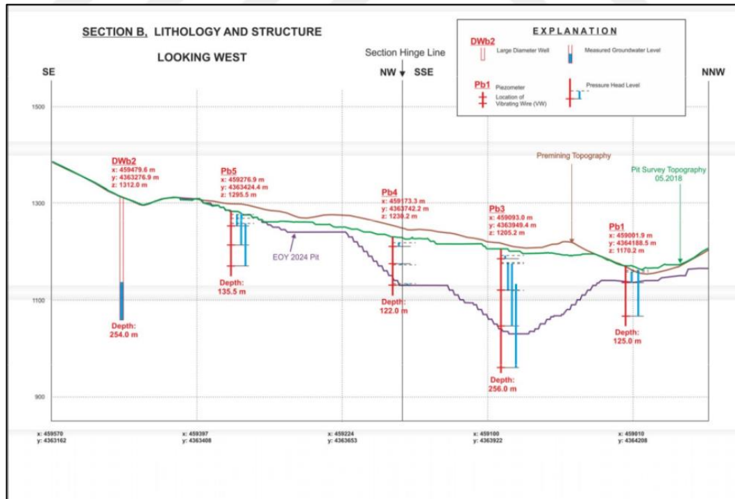
Figure 4.20. Pressure heads recorded at VWP on cross- section B (from Ekmekçi et al., 2018)
