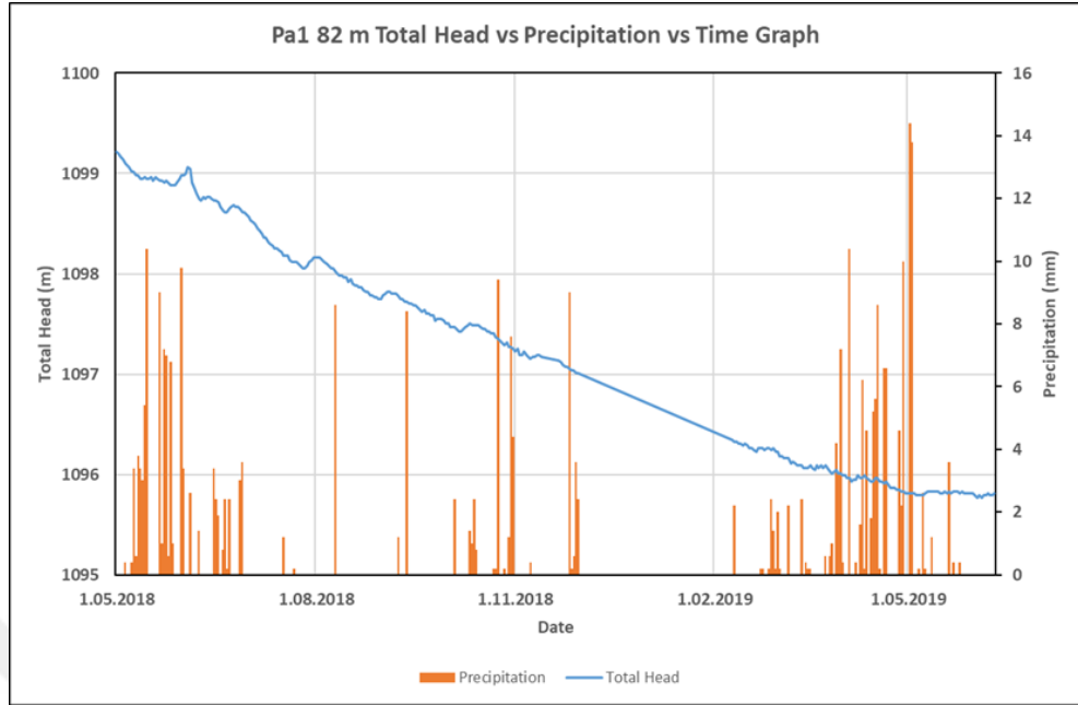
Figure 4.25. Hyetograph and hydrograph of VWP no Pa1_82 (enlarged view) (from Ekmekçi et al., 2019)
