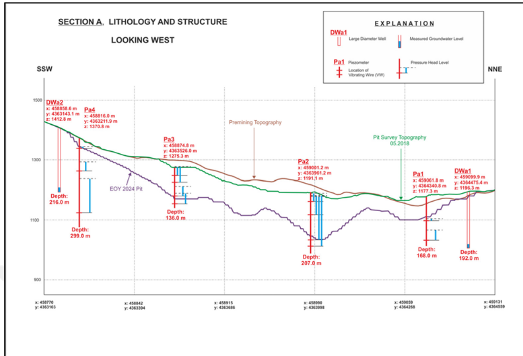
Figure 4.19. Pressure heads recorded at VWP on cross- section A (from Ekmekçi et al., 2018)
