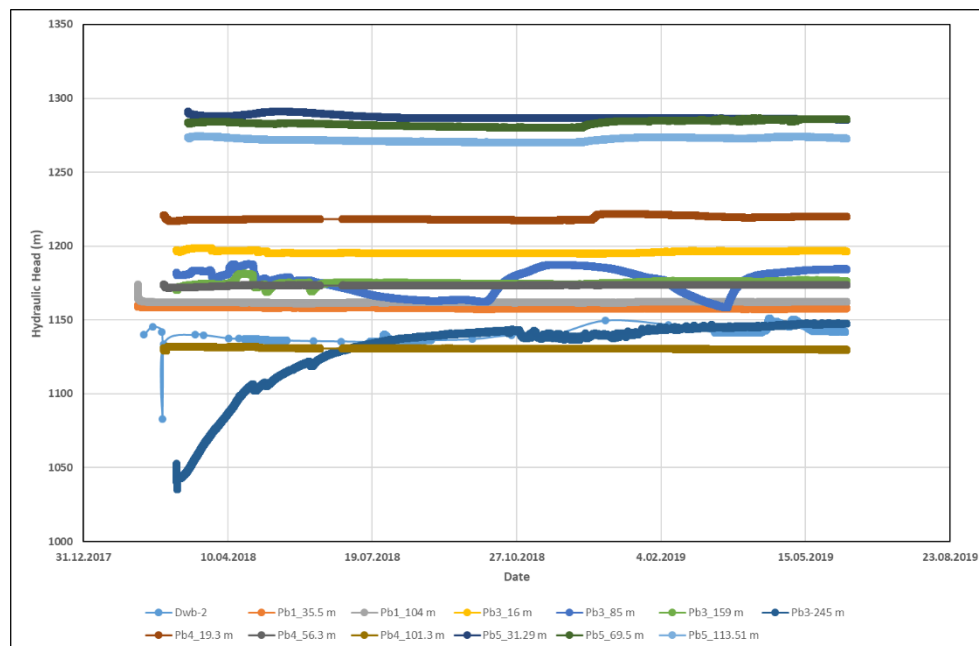
Figure 4.15. Hydraulic head distribution at cross- section B
