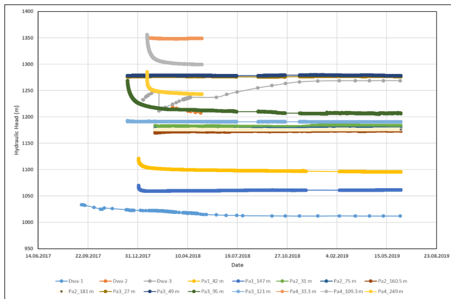
Figure 4.14. Hydraulic head distribution at cross- section A
