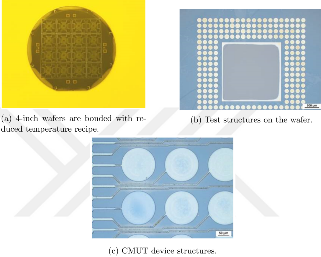
Figure 2.48: The third anodic wafer bonding of the 4-inch Pyrex - SOI wafer pair. Reduced temperature recipe was used for this bonding process.
