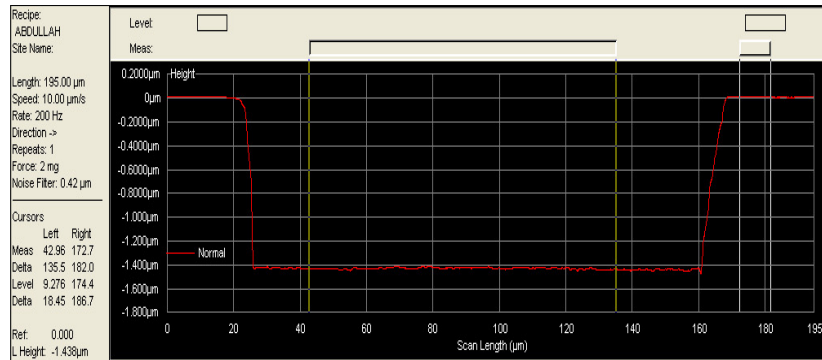
Figure 2.19: Stylus profilometer measurement of Pyrex chip after ICP argon and SF_6 plasma with the initial base recipe. Height difference is measured as 1438 nm
