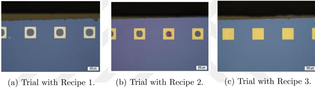
Figure 2.44: Wafer bonding results of Region 3 after 3 different recipe trials.
