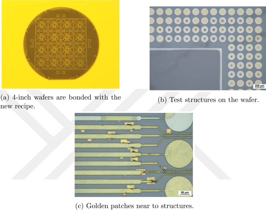
Figure 2.46: The second anodic wafer bonding of the 4-inch Pyrex - SOI wafer pair. New recipe was used for this bonding process.
