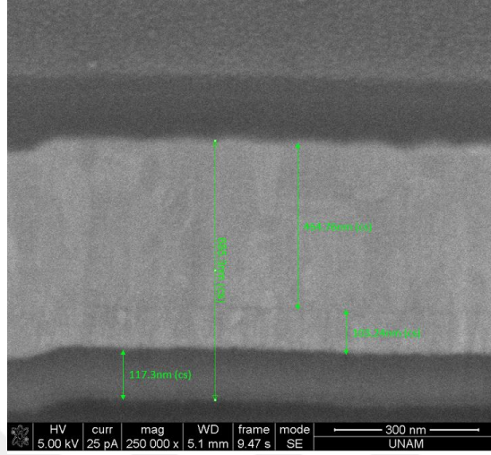
Figure 2.23: Focused Ion Beam (FIB) micrograph of the cross-section of the Ti/Pt/Au metal stack deposited on Pyrex wafer. Titanium thickness is measured as 117,30 nm , platinum thickness is measured as 103,24 nm , gold thickness is measured as 454,26 nm
