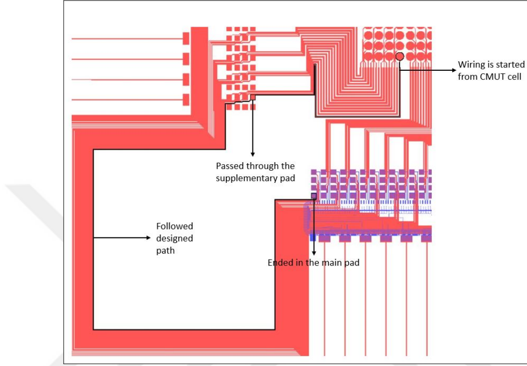
Figure 2.7: The path of wiring between CMUT cell and CMUT main pad using supplementary CMUT pad.
