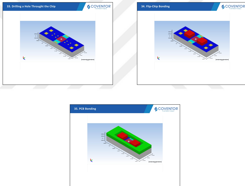
Figure 2.61: 3D process flow drawn by Coventor SEMulator 3D software when the software license was given free of charge due to the COVID-19 pandemic constraints.
