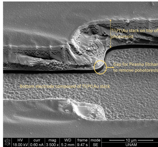
Figure 2.26: Entry regions for the piranha etchant to remove photoresist on top of the Pyrex surface to reveal bottom electrode.
