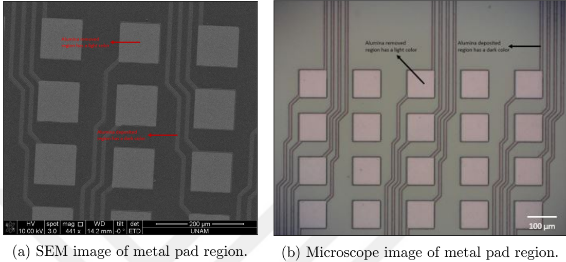
Figure 2.37: Metal pad regions after alumina etch, etched areas are brighter than other regions.
