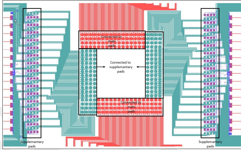
Figure 2.9: Half of the CMUT elements are connected to main CMUT metal pads, while the other half are connected to supplementary CMUT metal pads.
