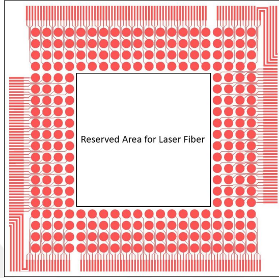
Figure 2.13: 12×12 CMUT subtracted from 20×20 CMUT elements in a square array pattern.
