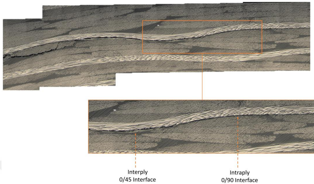
Figure 5.14. Post-mortem micrograph taken from the horizontal arm of Fabric 1.
