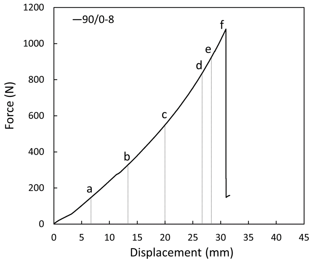
Figure 4.7. Six displacement values indicated at the load-displacement curve of experiment 90/0-8.
