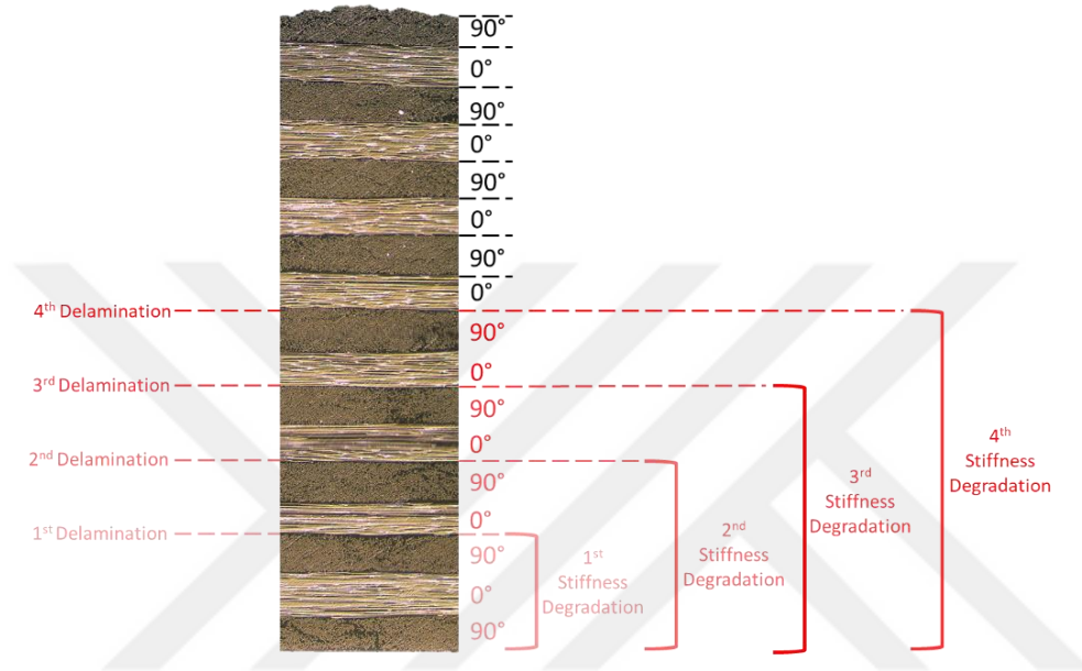
Figure 4.19. Interfaces where the delamination occurs and the plies whose stiffness are degraded.
