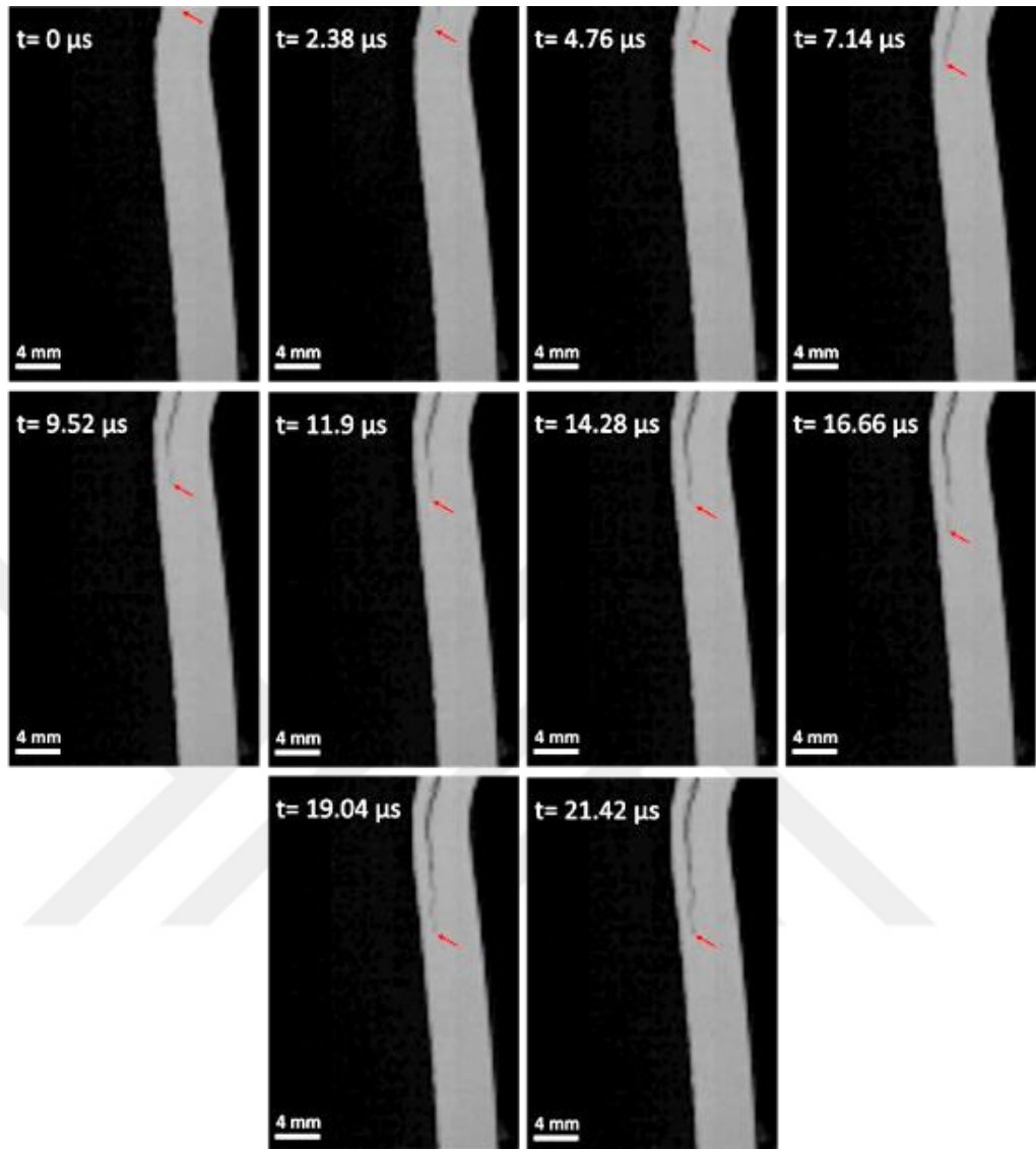
Figure 5.4. Propagation of the crack during the first load drop for the fabric specimen Fabric 1
