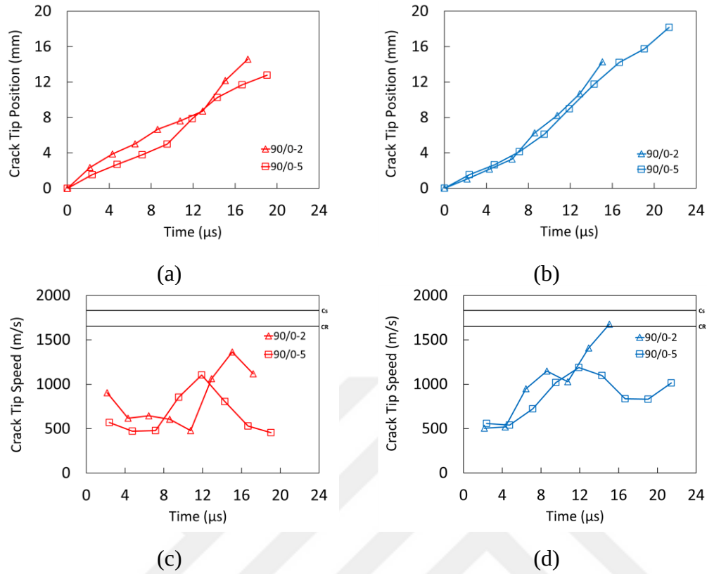
Figure 4.6. Crack tip position and speed history for cross-ply laminates: (a) upper crack tip position, (b) lower crack tip position, (c) upper crack tip speed, (d) lower crack tip speed
