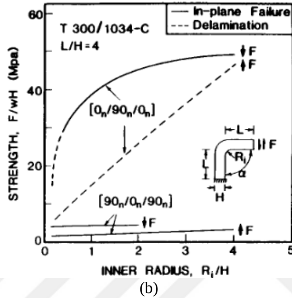
Figure 2.2. Effect of (a) the moment arm length and (b) stacking sequence on curved beam strength
