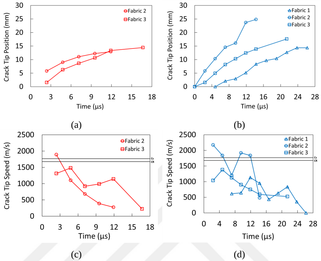
Figure 5.5. Crack tip position and speed history for fabric laminates: (a) upper crack tip position, (b) lower crack tip position, (c) upper crack tip speed, (d) lower crack tip speed.
