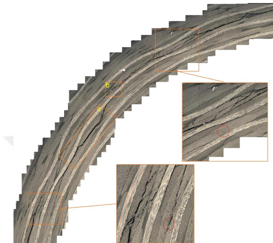
Figure 5.11. Post-mortem micrograph taken from the curved region of Fabric 1.
