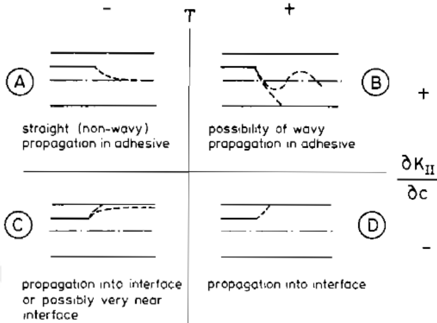
Figure 4.29. Possible crack paths in a brittle adhesive layer
