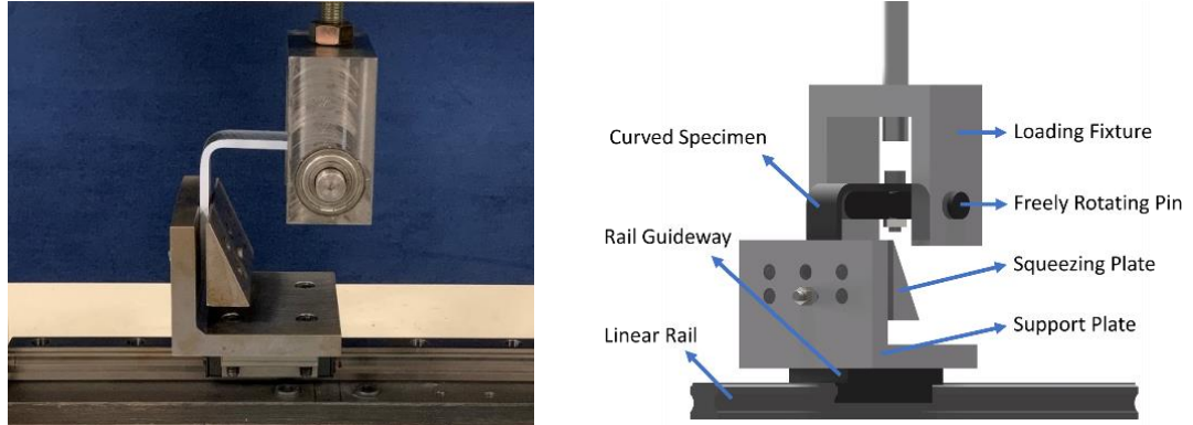
Figure 3.5. (Left) Novel test fixture designed for pure transverse loading and (Right) CAD Drawing of fixture
