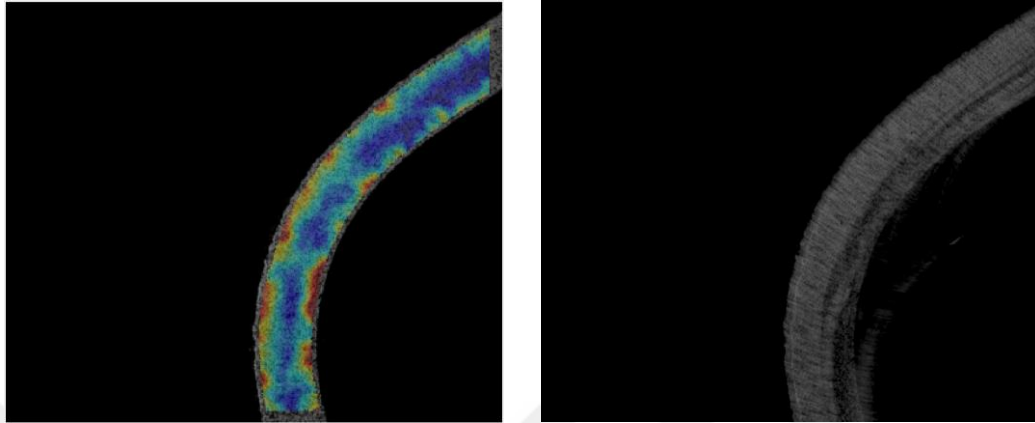
Figure 4.9. (a) von Mises strain field just before the failure and (b) High-speed camera images just after the failure
