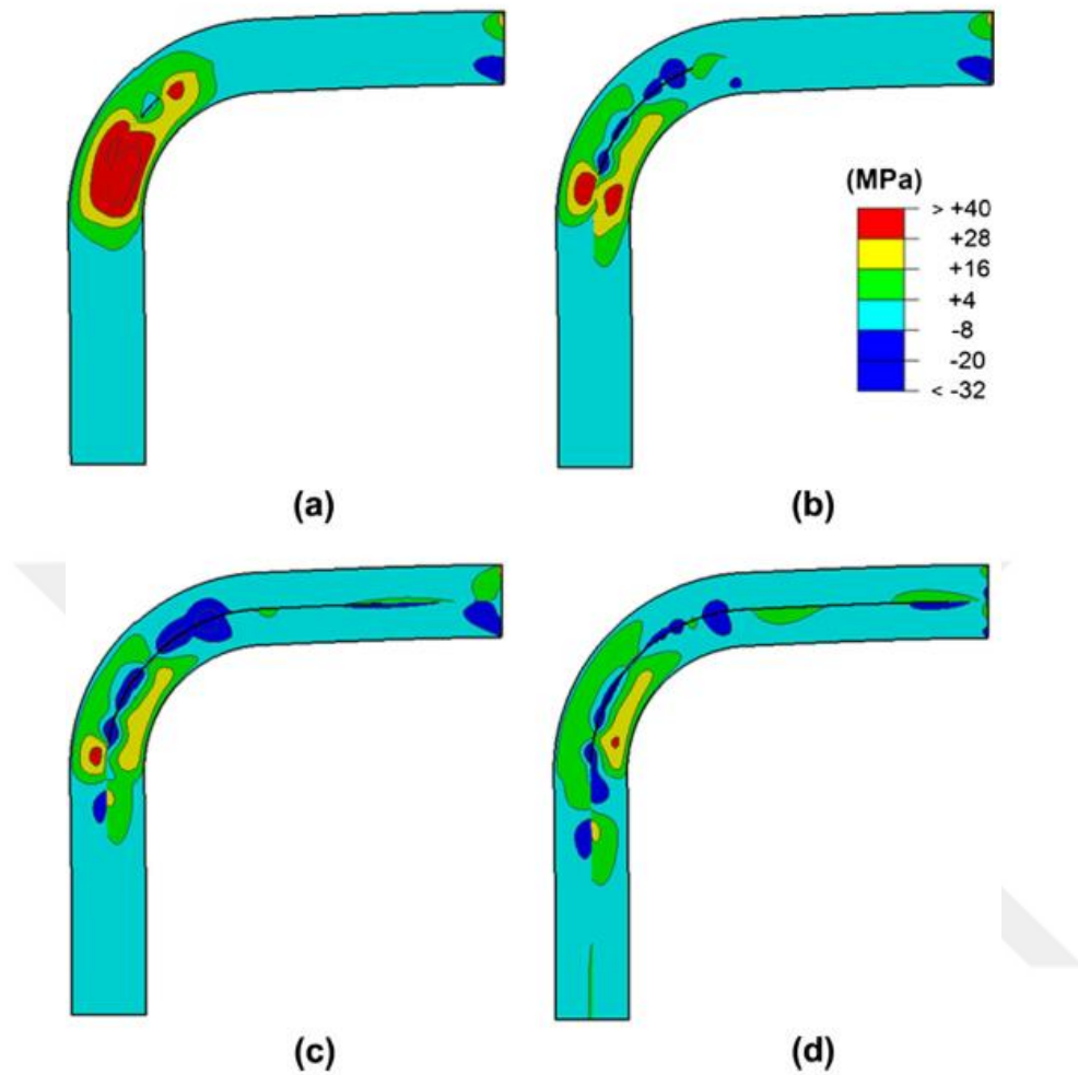
Figure 2.13. The propagation of the initial crack through both arms
