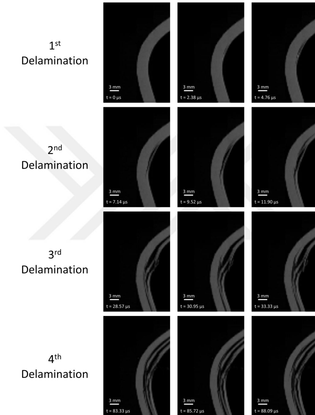
Figure 4.4. High-speed camera images corresponding to sequential delaminations occurring during the course of the load drop in the cross-ply specimen 90/0-9.
