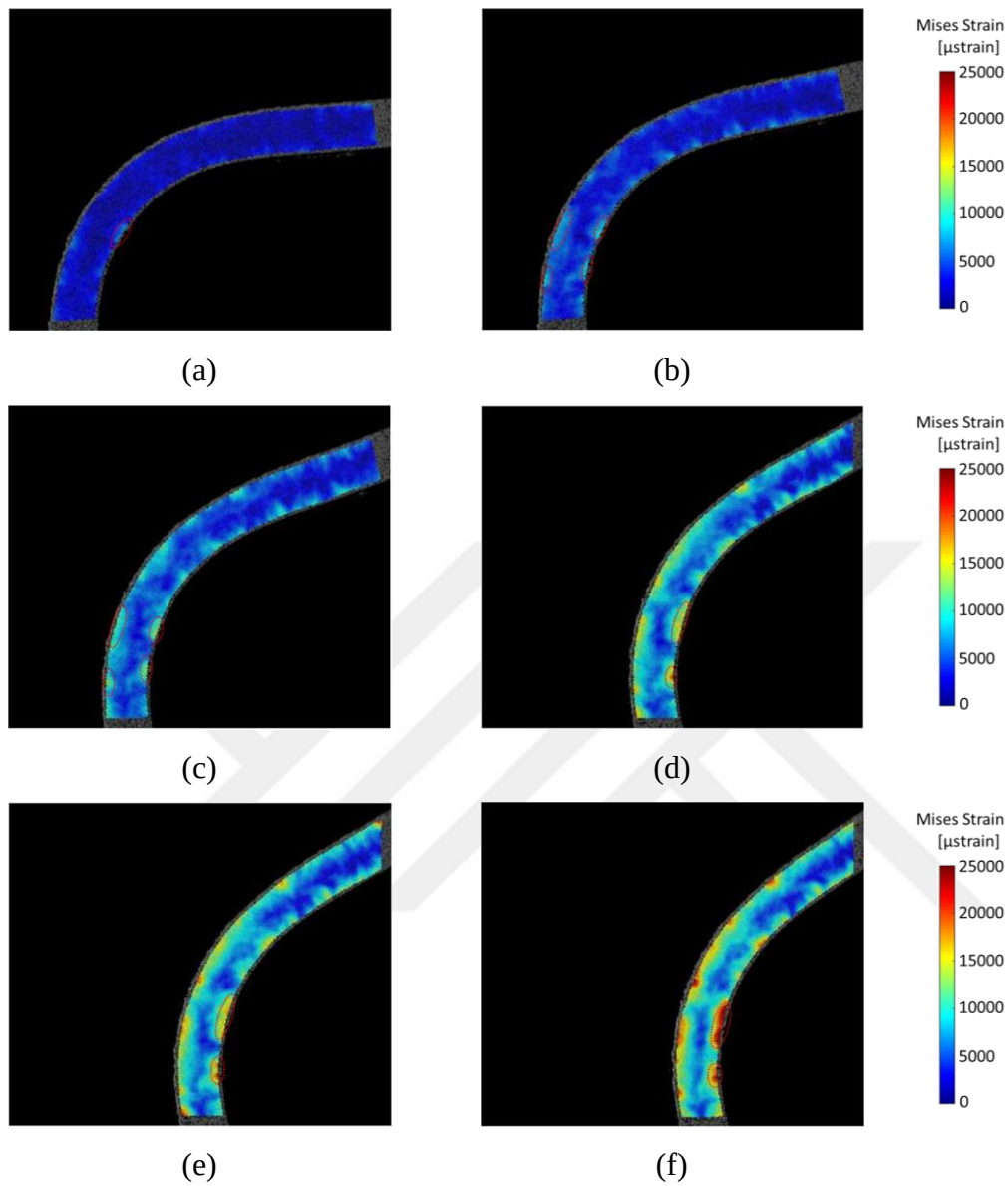
Figure 4.8. Von Mises strain field over the curved region of specimen 90/0-8 at six displacement values of (a) 6.67 mm, (b) 13.3 mm, (c) 20 mm, (d) 26.7 mm, (e) 28.3 mm and (f) 30.1 mm
