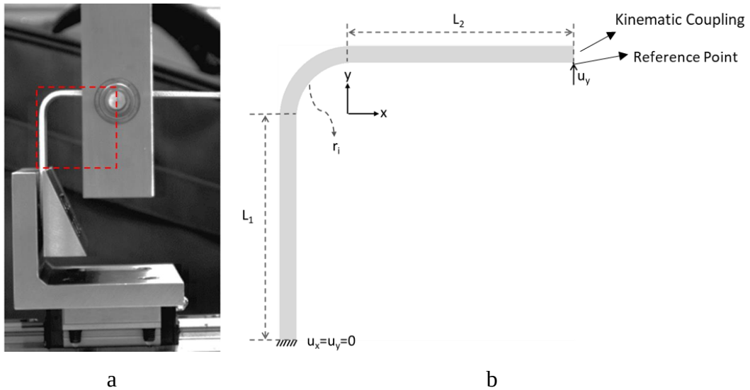
Figure 3.7. a) Experimental boundary conditions and b) 2D finite element model generated
