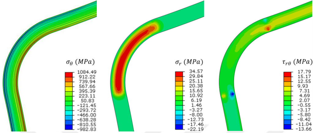
Figure 4.16. Stress field obtained for the cross-ply curved composite laminates: (a) Tangential Stress (b) Radial Stress (c) Shear Stress
