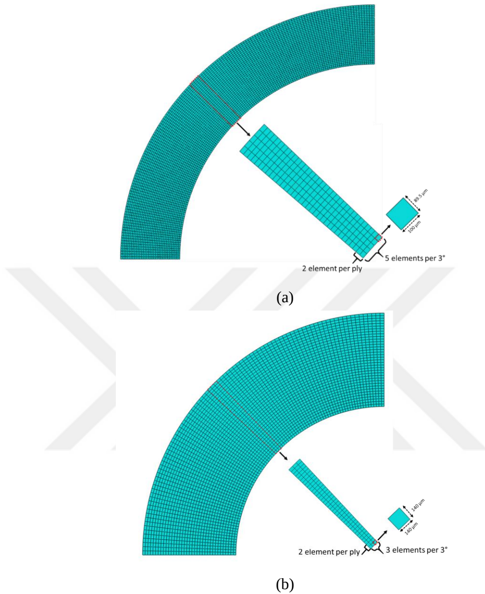
Figure 3.8. Mesh refinement in the curved region for (a) cross-ply and (b) fabric curved specimens
