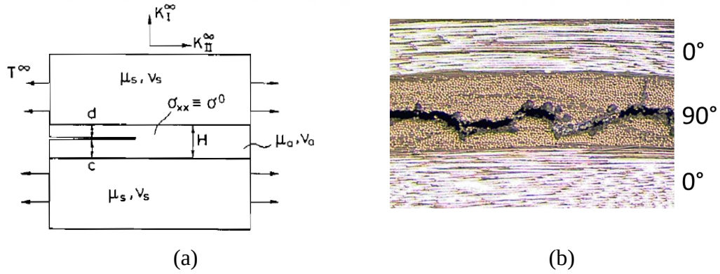
Figure 4.28. (a) Crack inside an adhesive layer constrained by solid layer and (b) Crack in brittle matrix inside the 90° ply constrained by the 0° plies
