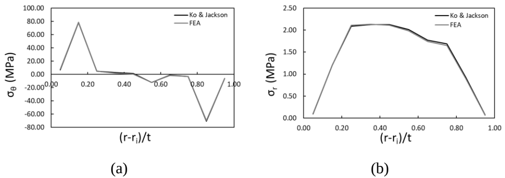
Figure A.1. Comparison of the analytic solution with finite element results for pure bending case: (a) tangential stress, (b) radial stress.
