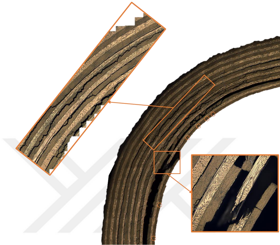
Figure 4.13. Post-mortem micrograph taken from the curved region of specimen 90/0-6
