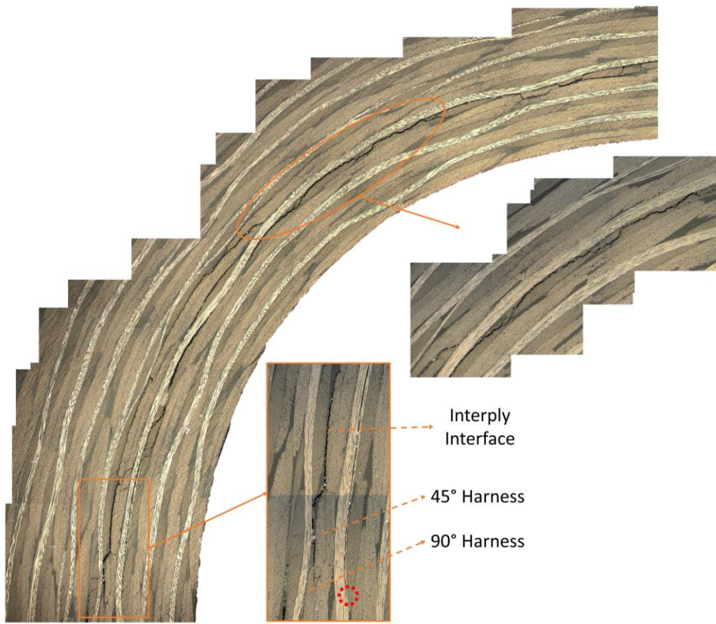
Figure 5.15. Post-mortem micrograph taken from the curved region of Fabric 3.
