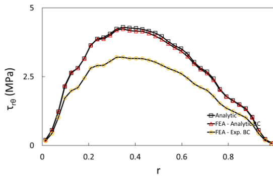
Figure D. 3. Shear stress distribution obtained from analytic solution and finite element results for plane stress case
