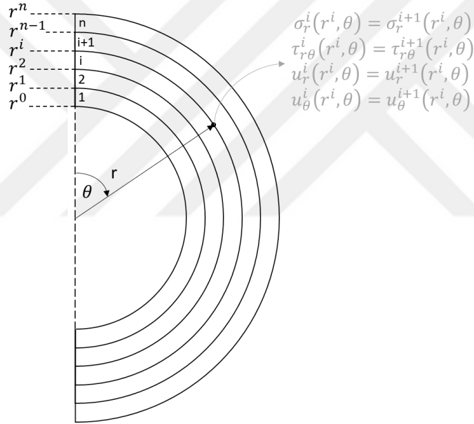
Figure 3.15. Boundary conditions and notations used in multilayered theory
