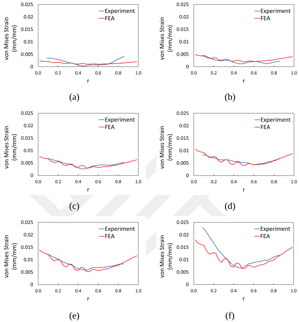
Figure 4.32. Comparison of the von Mises strain distribution obtained from the experiment and finite element analysis at different displacement values of : (a) 5mm, (b) 10 mm, (c) 15 mm, (d) 20 mm, (e) 25 mm and (f) 30 mm
