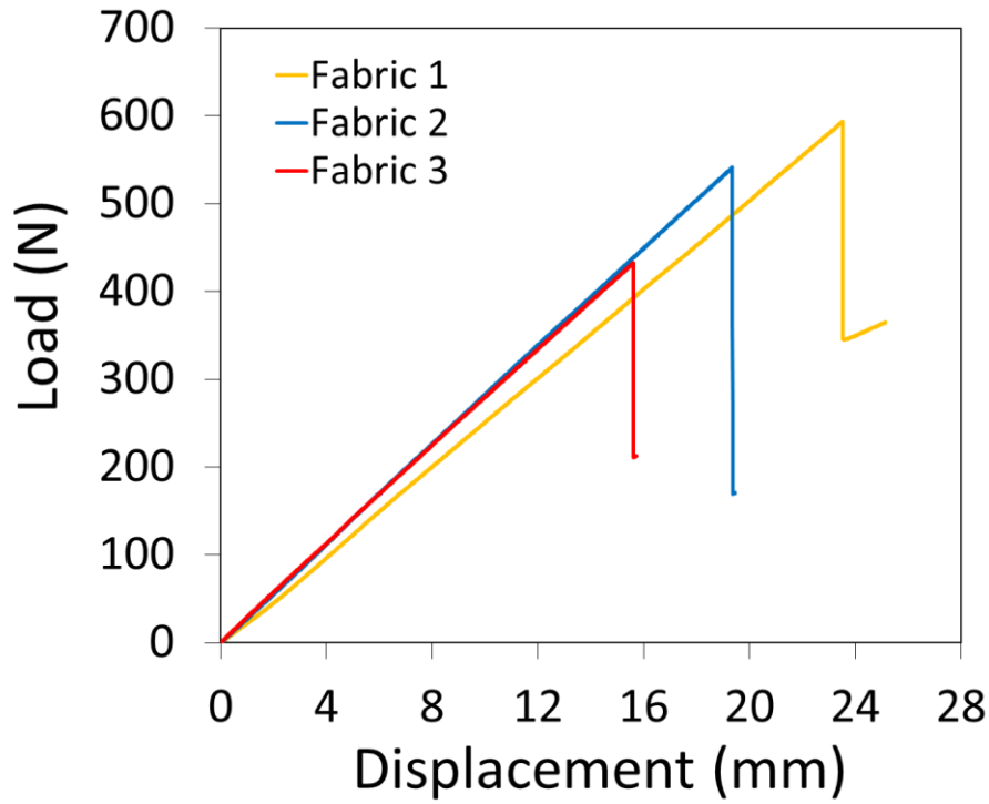
Figure 5.1. Load-displacement curves of fabric curved composite laminates.
