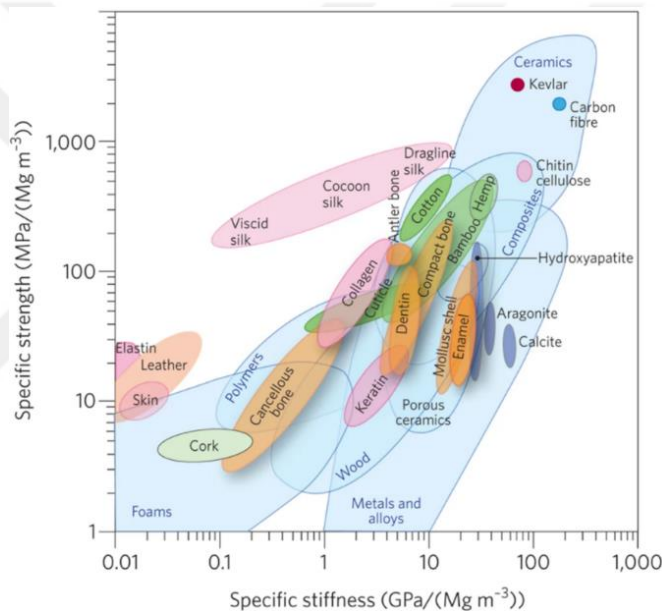
Figure 1.2. Ashby chart which shows the specific stiffness and strength of the materials [5]
