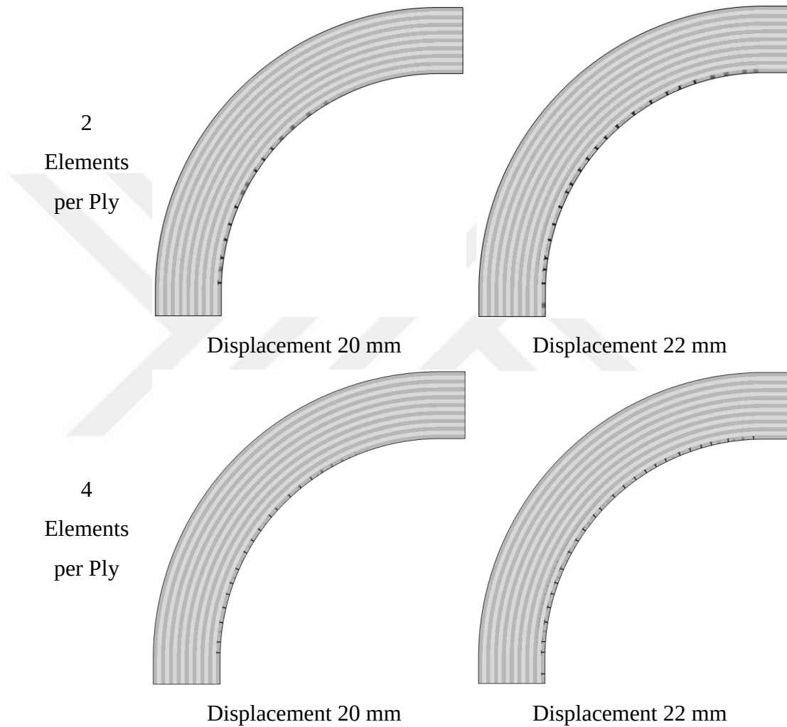
Figure 4.23. Progression of the tensile matrix damage at 2-direction for the mesh refinement of 2 elements per ply and 4 elements per ply
