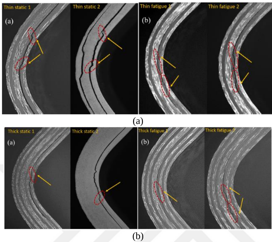
Figure 2.17. (a) damage pattern observed in thin laminates under static and fatigue loading (b) damage pattern observed in thick laminates under static and fatigue loading
