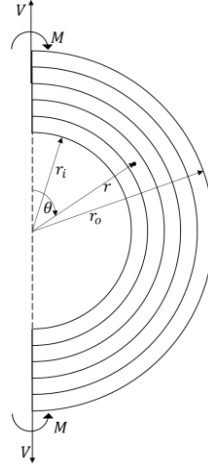
Figure 3.14. Curved beam under pure bending moment
