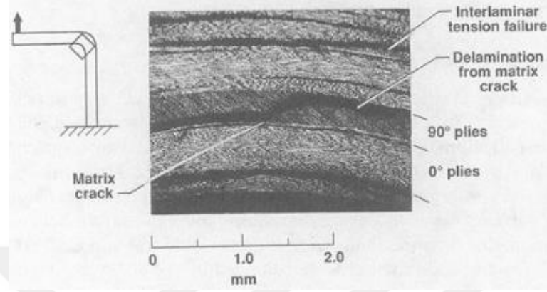
Figure 2.7. Failure modes observed in the tested specimen
