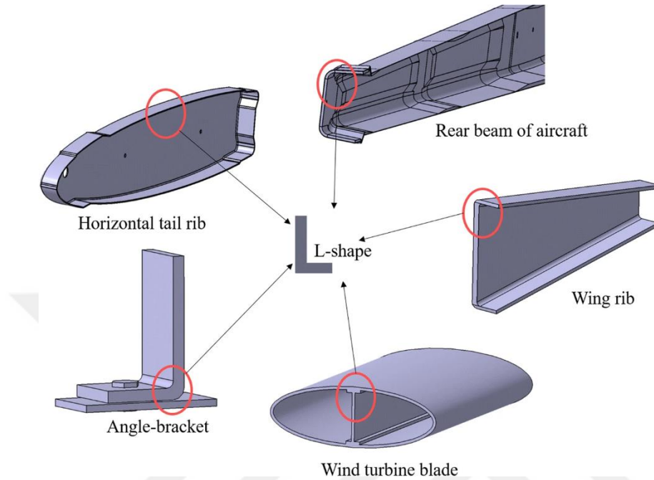
Figure 1.5. Curved sub-components in wing turbine blade or aircraft wing [10]
