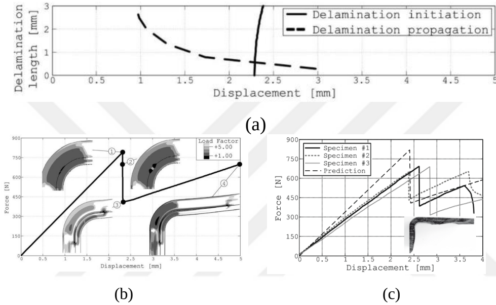
Figure 2.11. (a) Delamination initiation and delamination propagation curve (b) Load-displacement curve obtained from finite element analysis (c) comparison of load displacement curve obtained from experiment and finite element analysis
