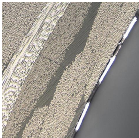
Figure 5.10. Detailed micrographs of the matrix cracks observed in the Fabric 1.
