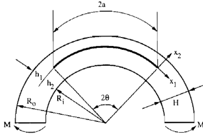
Figure 4.30. Curved beam with an initial crack length under pure bending moment
