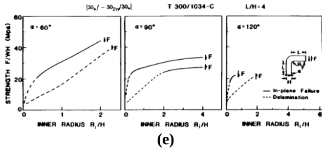
Figure 2.1. Strength versus Inner radius to thickness ratio for 5 different stacking sequence: (a) [0 n ], (b) [0 n /90 n /0 n ], (c) [0 2n /45 n /-45 2n /45 n /0 2n ], (d) [0 n /45 n /-45 n /90 2n /-45 n /45 n /0 n ], (e) [30 n /-30 2n /30 n ]
