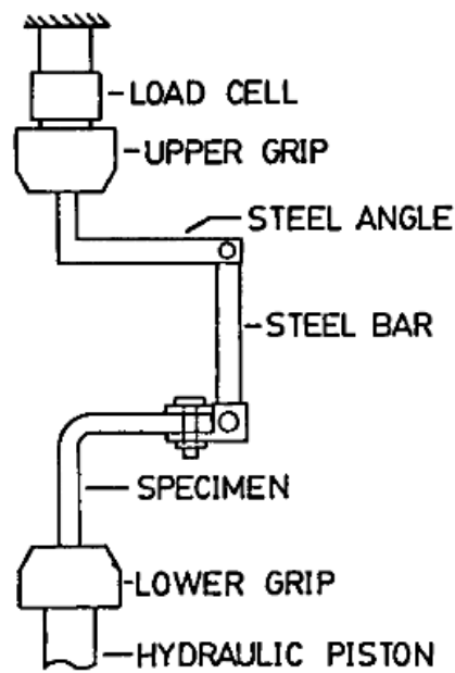
Figure 2.3. Schematic of the experimental setup
