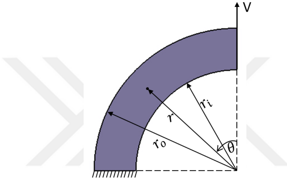
Figure 3.11. Curved beam under shear load
