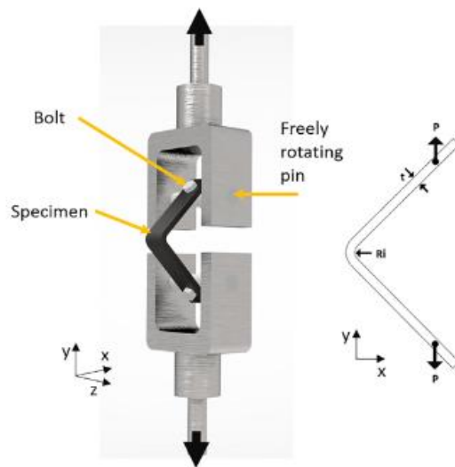
Figure 2.16. Experimental fixture designed.
