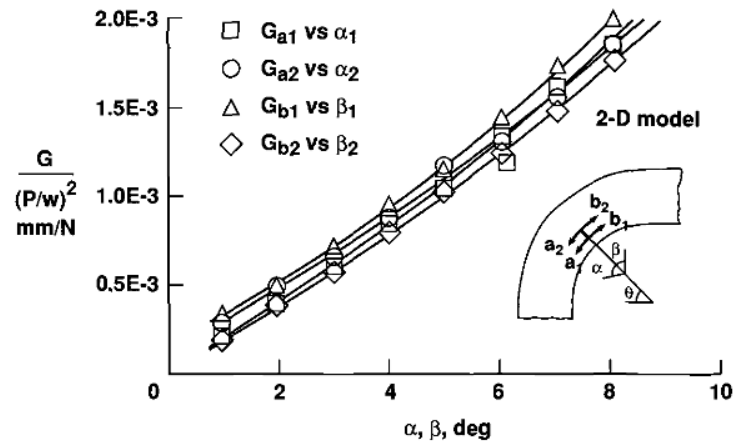
Figure 2.8. Strain energy release rate versus crack length growth for the possible crack branches
