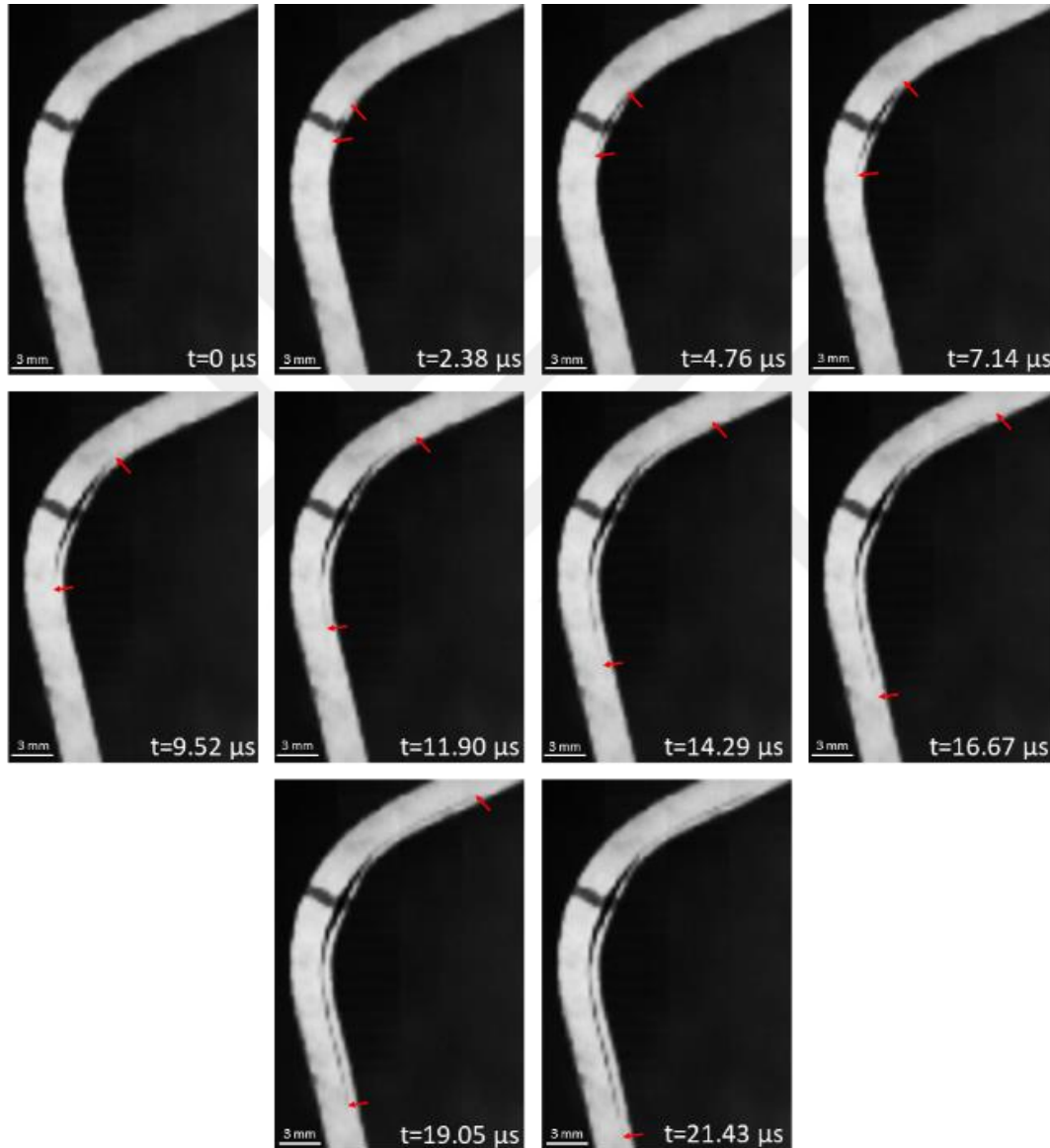
Figure 4.5. Propagation of the crack during the first load drop for the cross-ply specimen 90/0-5
