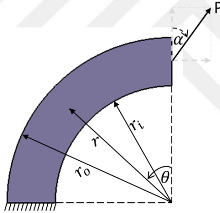
Figure 3.13. Curved beam under normal and shear load
