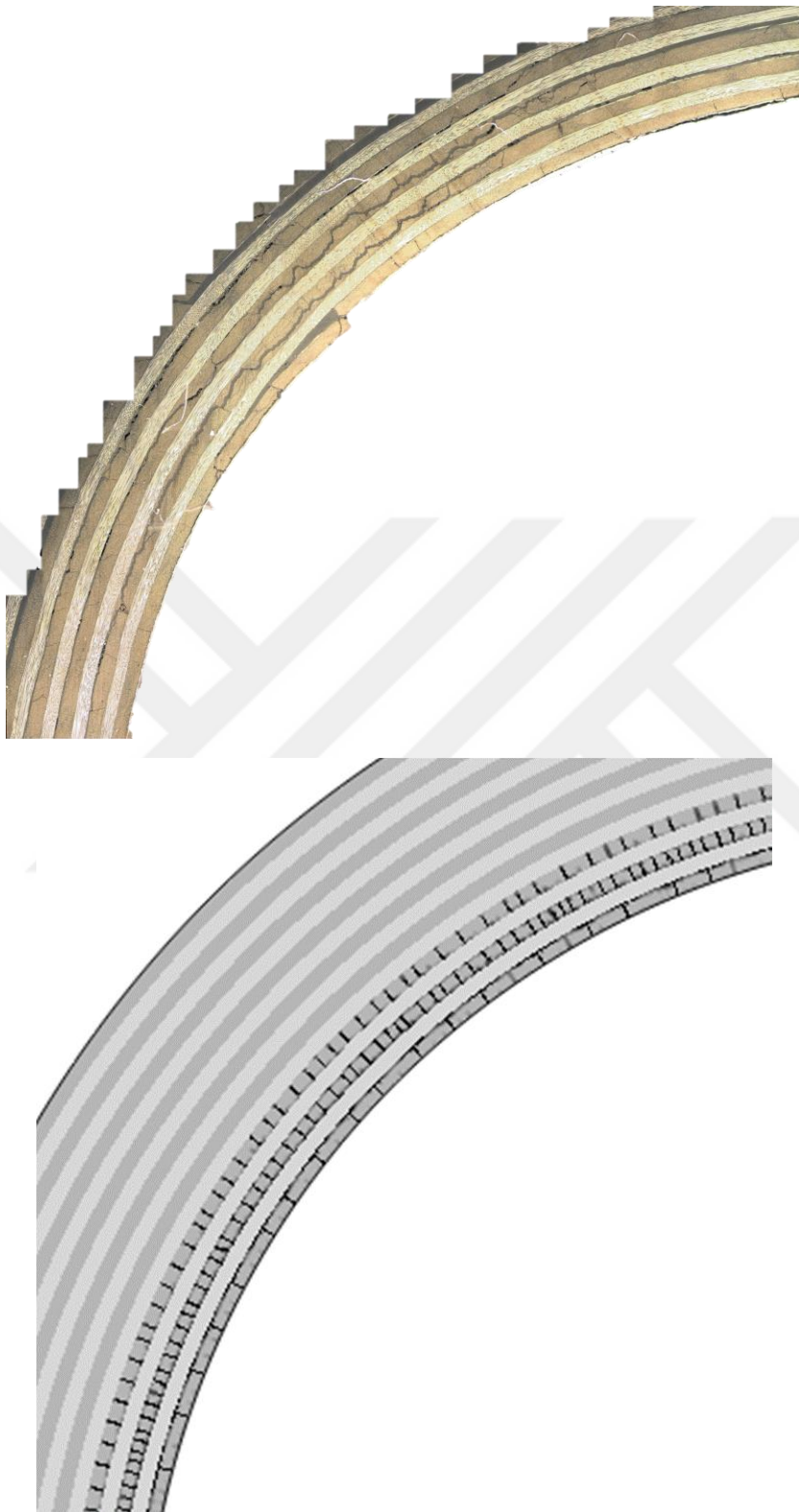
Figure 4.27. Damage pattern observed in the experiment and finite element analysis for the cross-ply curved composite laminates
