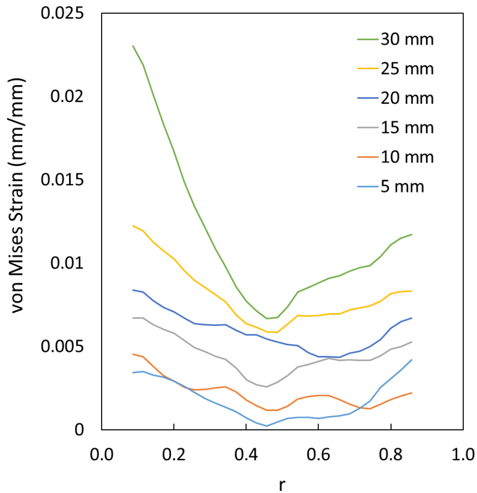
Figure 4.11. Through-the-thickness von Mises strain distribution obtained from digital image correlation method at six different displacement values.
