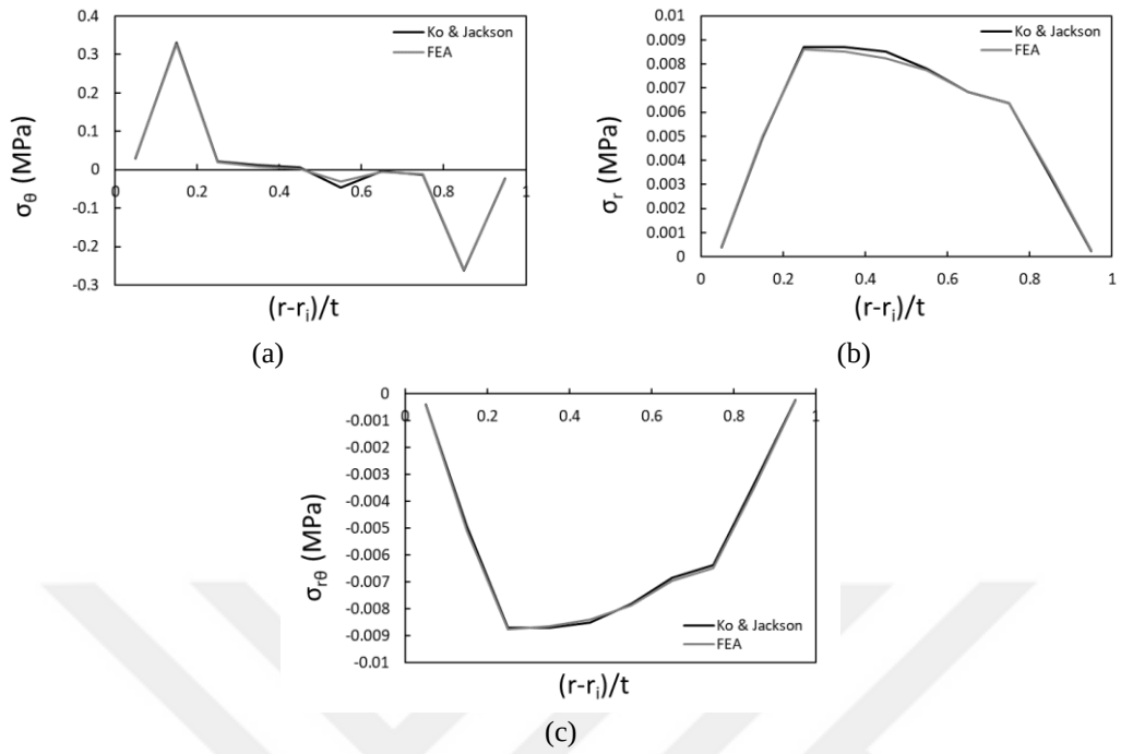
Figure A.2. Comparison of the analytic solution with finite element results for end shear load case: (a) tangential stress, (b) radial stress, (c) shear stress.
