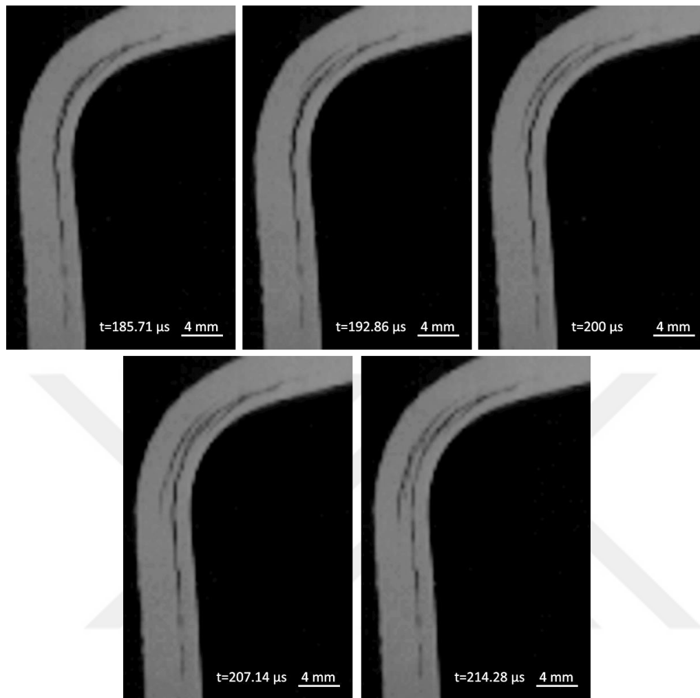
Figure 5.3. Secondary crack initiation 185.71 \mu\text{s} after the 1 st failure occurs in the fabric specimen Fabric 2
