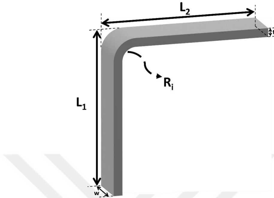
Figure 3.3. Geometry of the curved beam specimen
