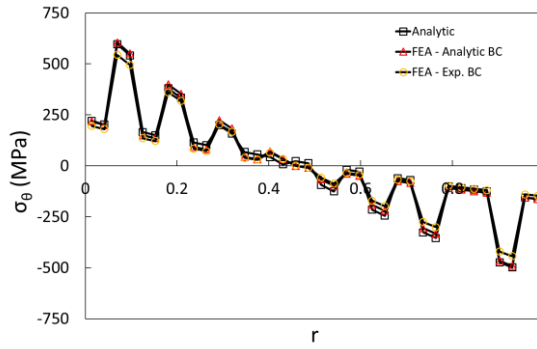
Figure D. 1. Tangential stress distribution obtained from analytic solution and finite element results for plane stress case
