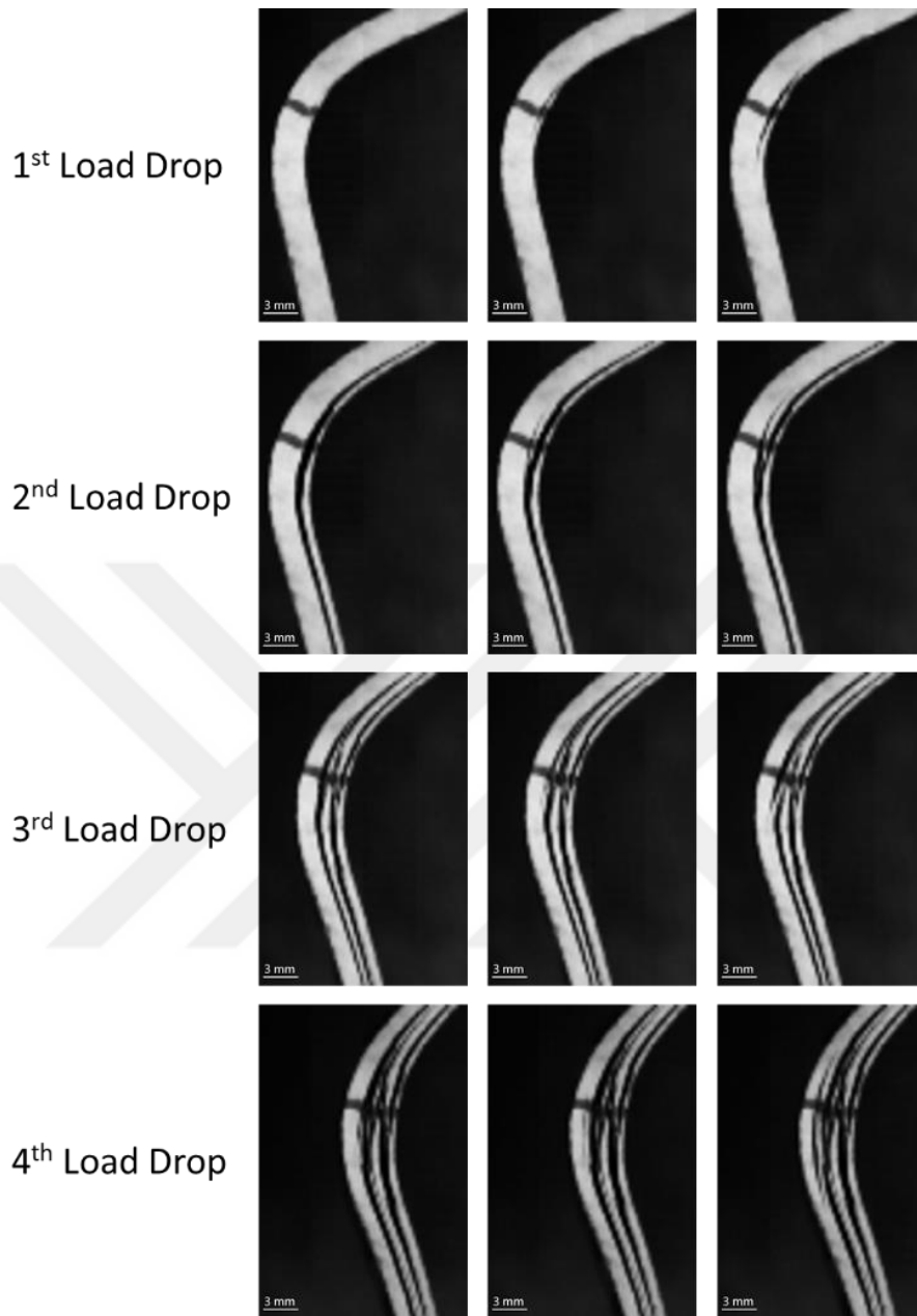
Figure 4.3. High-speed camera images corresponding to load drops observed in the cross-ply specimen 90/0-5.
