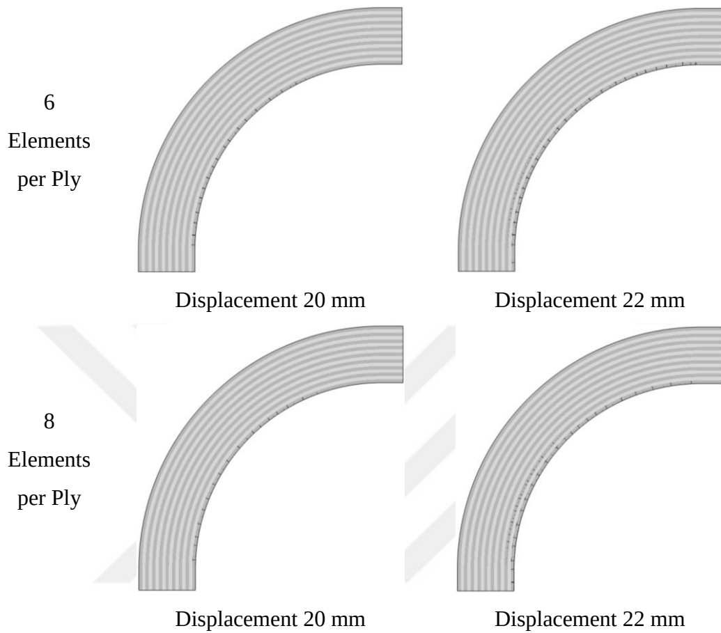
Figure 4.24. Progression of tensile matrix damage at 2-direction for the mesh refinement of 6 elements per ply and 8 elements per ply
