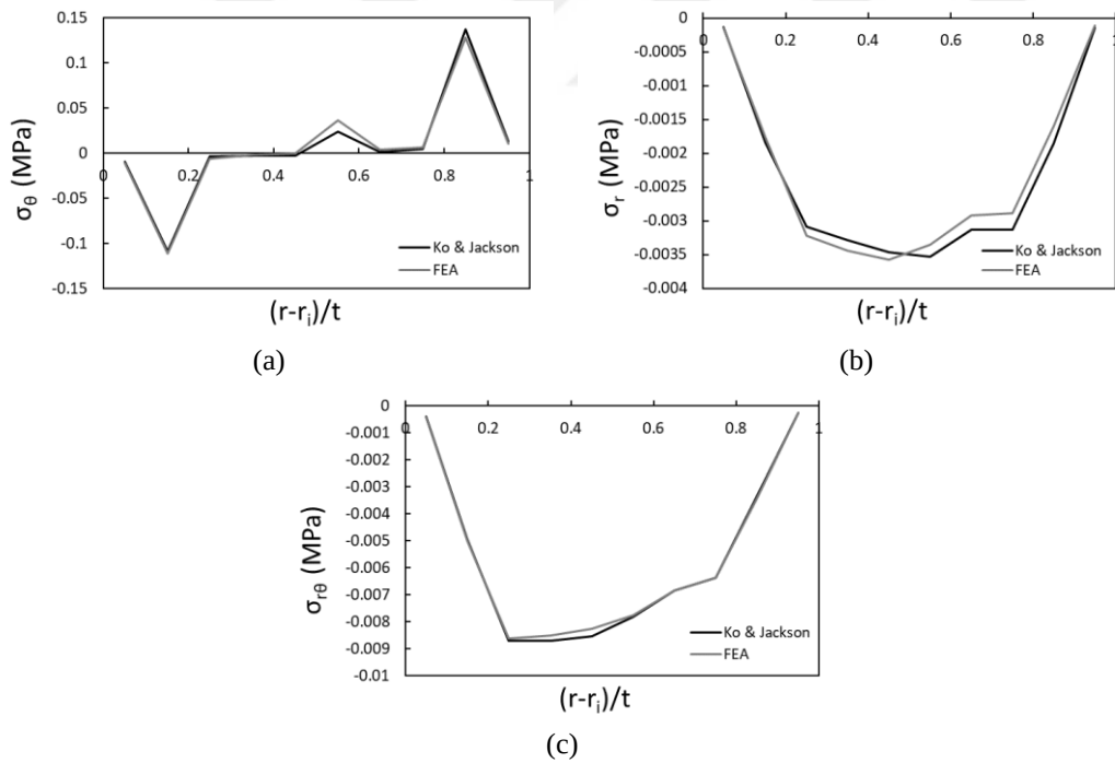
Figure A.3. Comparison of the analytic solution with finite element results for end normal load case: (a) tangential stress, (b) radial stress, (c) shear stress.
