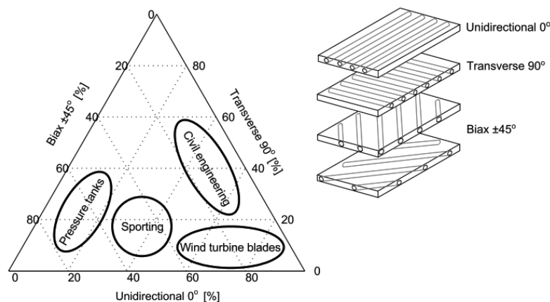
Figure 1.1. Stacking of the composite plies with different orientation [4]
