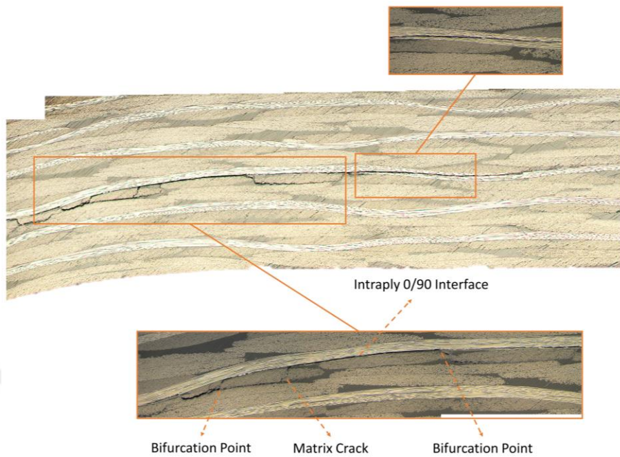
Figure 5.17. Post-mortem micrograph taken from the horizontal arm of Fabric 3. through the intra-ply +45/-45 interface. When it comes to the end of the harness, it propagates backward by surrounding the harness. It jumps to the intra-ply 0/90 interface by causing to resin and matrix cracking.
