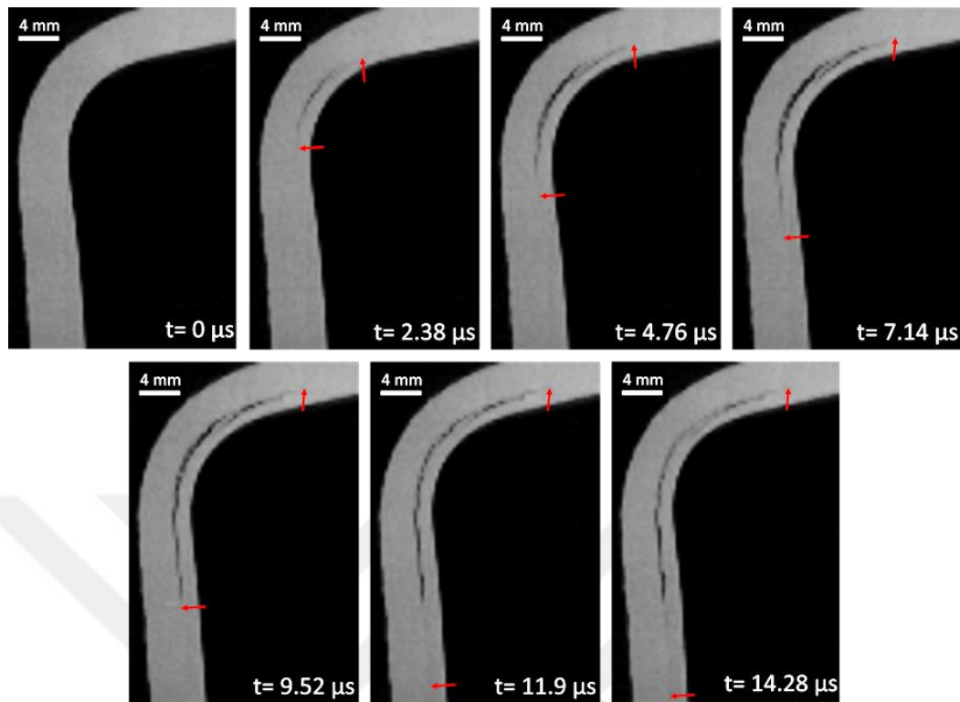
Figure 5.2. Propagation of the crack during the first load drop for the fabric specimen Fabric 2
