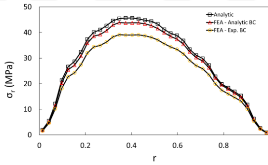
Figure D. 2. Radial stress distribution obtained from analytic solution and finite element results for plane stress case
