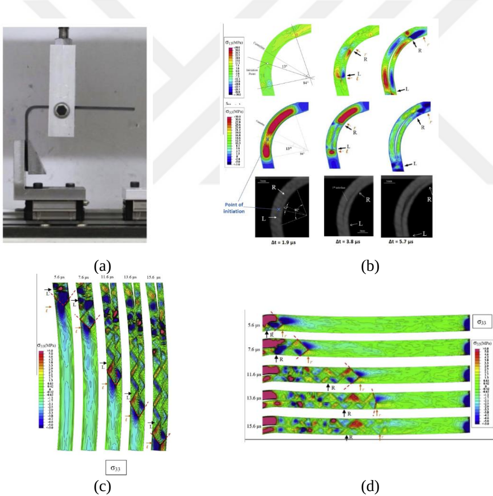
Figure 2.15. (a) Novel experimental setup designed (b) Comparison finite element result with numerical results in terms of crack initiation and propagation (c-d) shear Mach waves emanating from the crack tip where damage parameter is 0.6 at vertical and horizontal arm.
