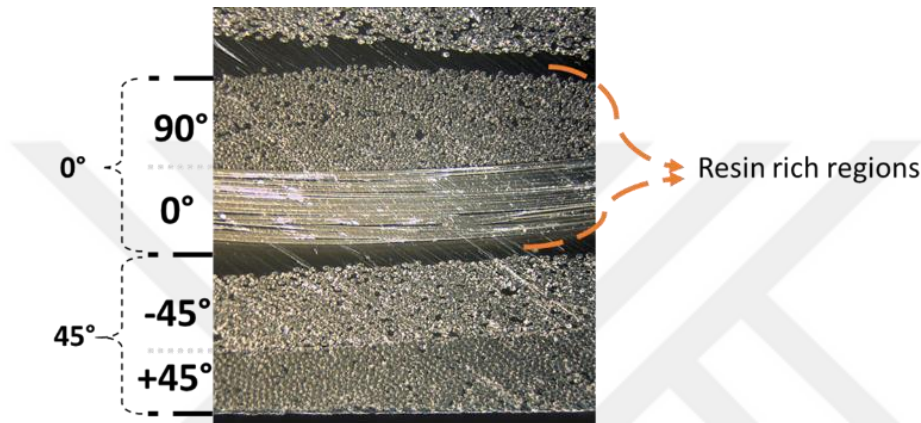
Figure 5.7. Resin rich regions and intra-ply interfaces.
