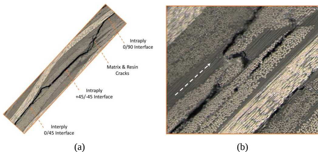
Figure 5.12. Close-up pictures of the curved region of Fabric 1.
