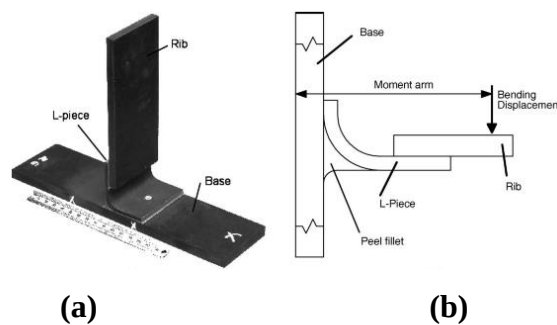
Figure 2.9. (a) Single L-joint (b) Schematic of the test setup
