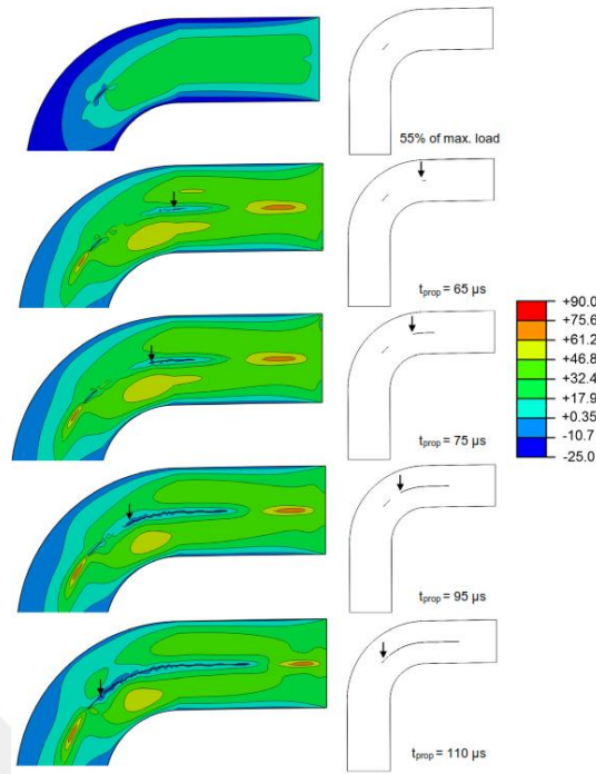
Figure 2.14. Failure sequence observed in the thicker curved composite laminate with an initial crack
