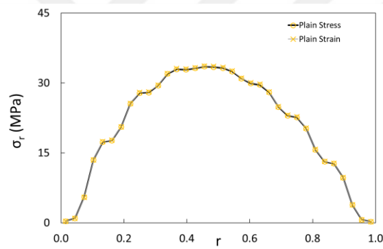
Figure C. 2. Radial stress distribution for plane stress and plain case in cross-ply specimen
