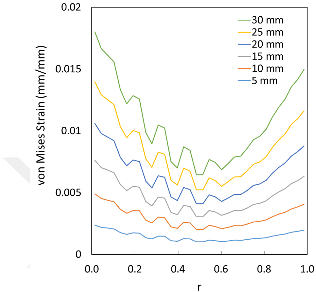
Figure 4.18. Through-the-thickness von Mises strain distribution obtained from finite element analysis at six different displacement values.
