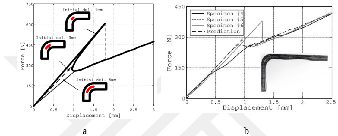
Figure 2.12. (a) Load displacement curves obtained from the models with different initial crack length (b) comparison of load displacement curves obtained from experiment and finite element analysis with a 3 mm initial crack length
