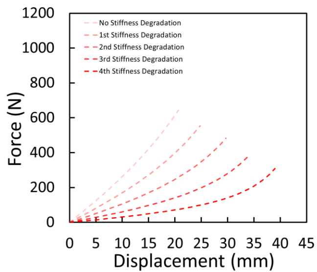
Figure 4.21. Load-displacement curves obtained from the finite element analysis with degraded material property.
