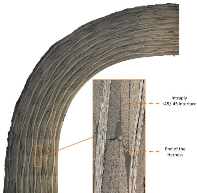
Figure 5.18. Post-mortem micrograph taken from the curved region of back surface of Fabric 3.
