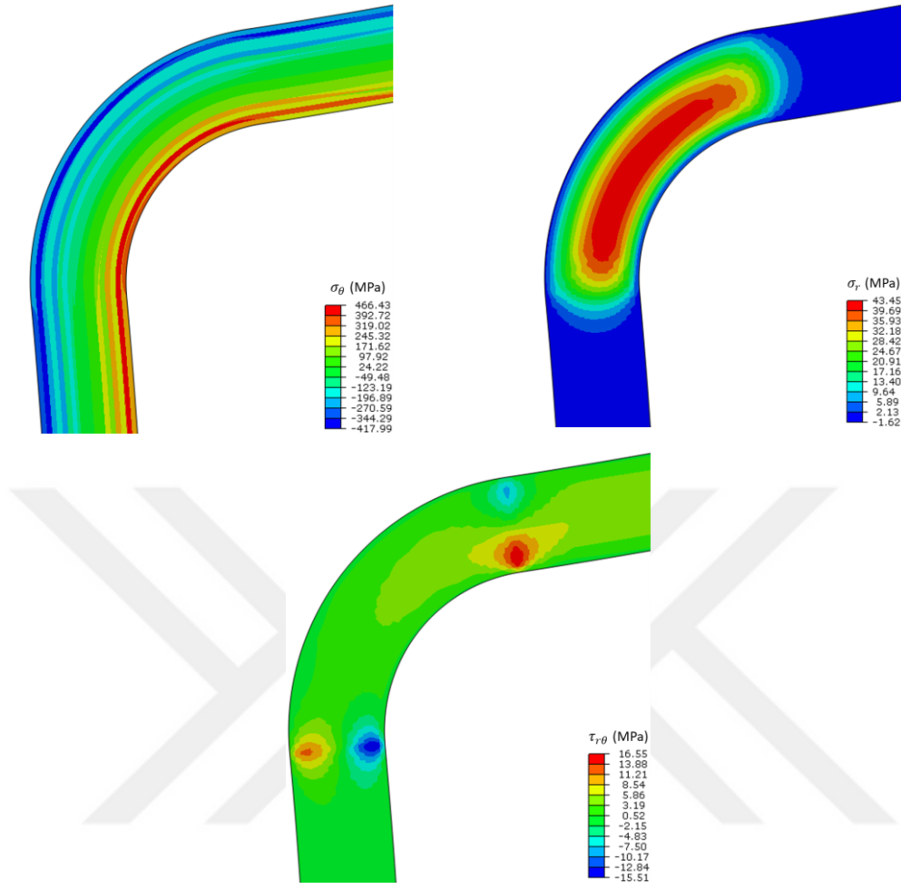
Figure 5.19. Stress field obtained for the fabric curved composite laminates: (a) Tangential Stress (b) Radial Stress (c) Shear Stress.
