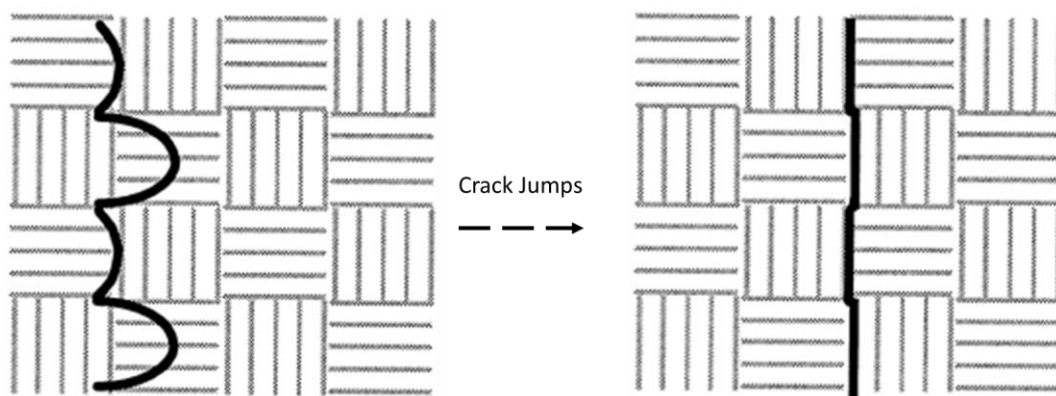
Figure 5.21. The effect of the weave pattern on the crack propagation and crack jumps occurs at a sudden load drop.
