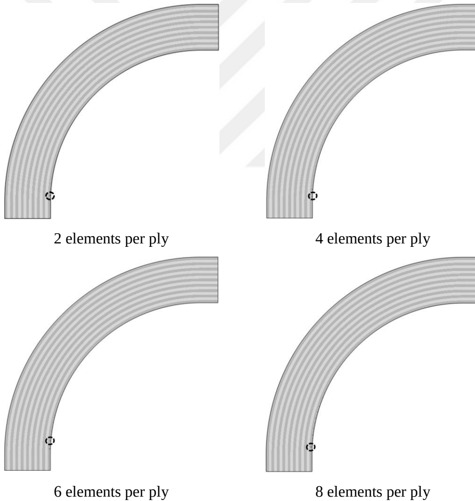
Figure 4.22. Initiation of tensile matrix damage at 2-direction for different mesh refinement
