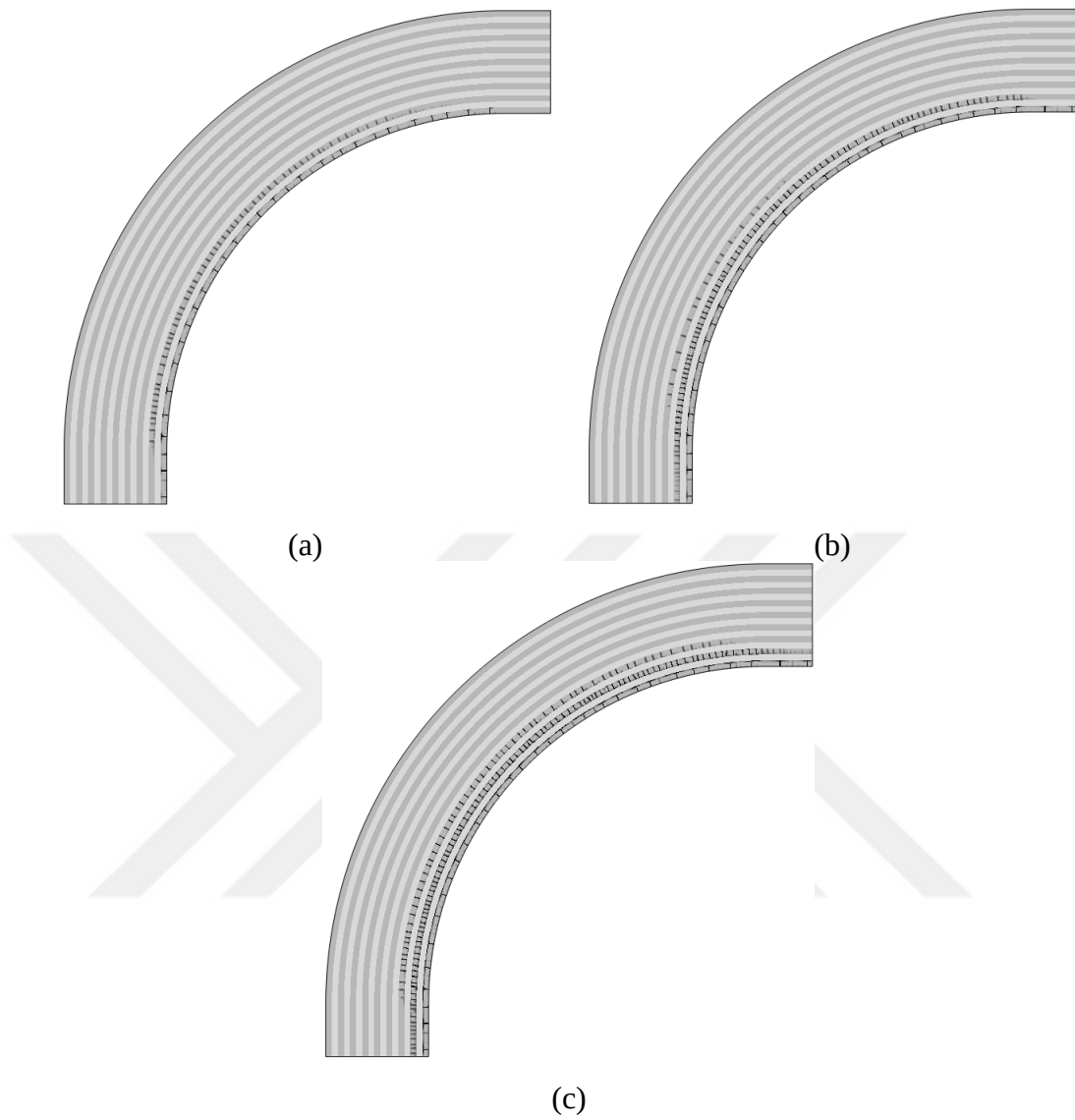
Figure 4.25. Progression of the tensile matrix damage at 2-direction for the mesh refinement of 8 element per ply at a displacement value of: (a) 24 mm, (b) 27 mm and (c) 30 mm
