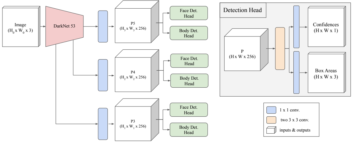
Figure 3.3: Complete model architecture
