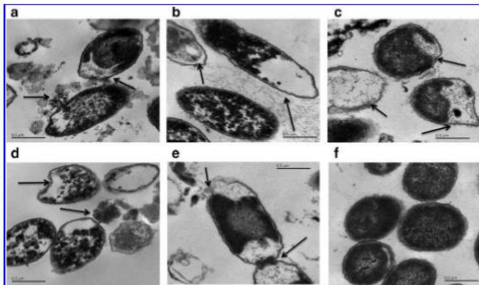
Figure 2.3. Micrographs of E.coli O157:H7 at 46,000x treated with 5%v/v of blueberry fractions: (a) total phenolics, (b) monomeric phenolic acids, (c) anthocyanins plus proanthocyanidins, (d) anthocyanins, (e) proanthocyanidins, and (f) control. Arrow indicates areas of significant damage (Lacombe et al. 2013).
