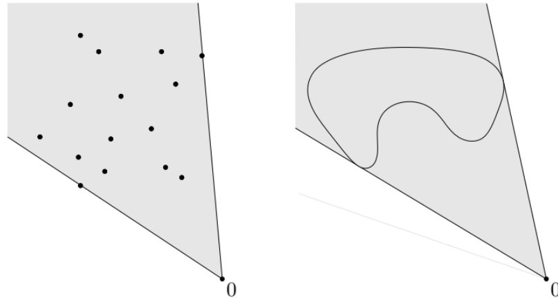
Figure 1.4: Conic hulls of two non-convex sets
