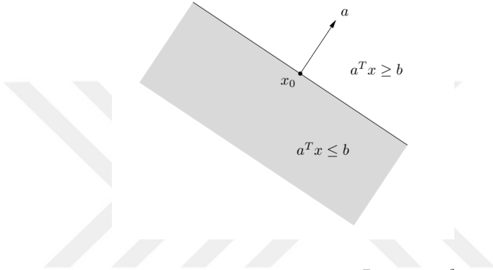
Figure 1.5 illustrates the hyperplane defined by a^T x = b in \mathbb{R}^2 . The hyperplane creates two halfspaces as a^T x \geq b and a^T x \leq b .
