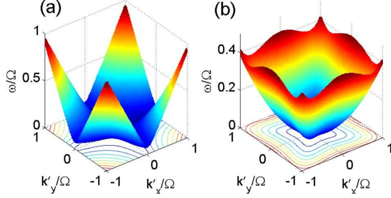
Figure 4.7: Dispersion relation of the acoustic Tkachenko modes for the square lattice, Eq. (4.71) for \alpha = 0.4 (a), and \alpha = 0.85 (b). Underlying contour plots are given to illustrate the anisotropy of the modes.
