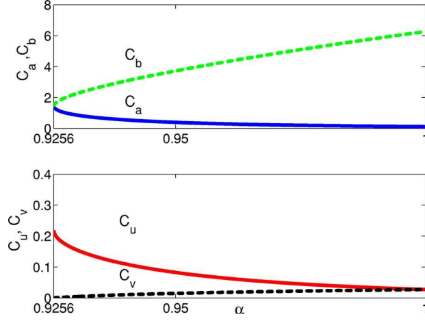
Figure 4.8: Elastic constants (C_a, C_b, C_u, C_v) of rectangular lattice. The upper figure shows optical elastic constants (C_a, C_b) . As \alpha \rightarrow 1 , C_a vanishes. The lower figure shows acoustic elastic constants (C_u, C_v) . As \alpha \rightarrow 1 , C_u \rightarrow C_v and there remains only one acoustic elastic constant similar to the one-component triangular lattice.
