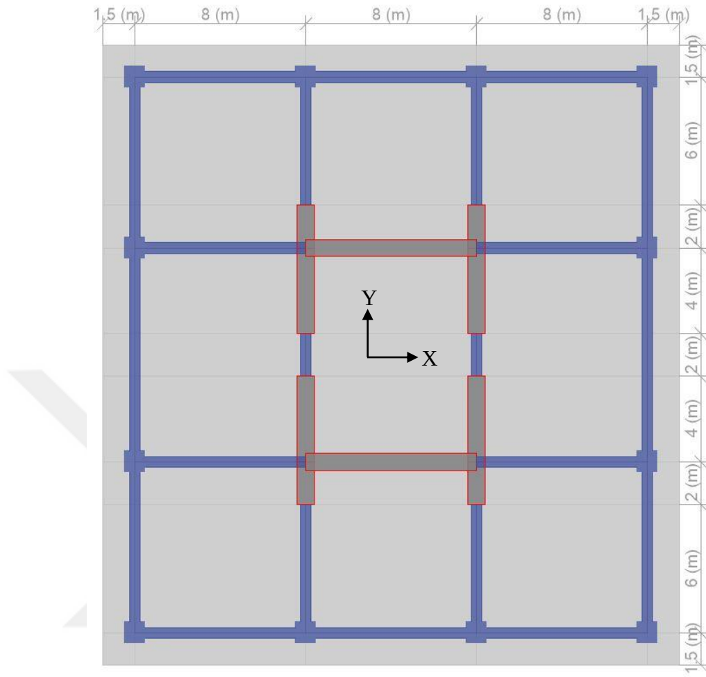
Figure 2.2. Typical Floor Plan
