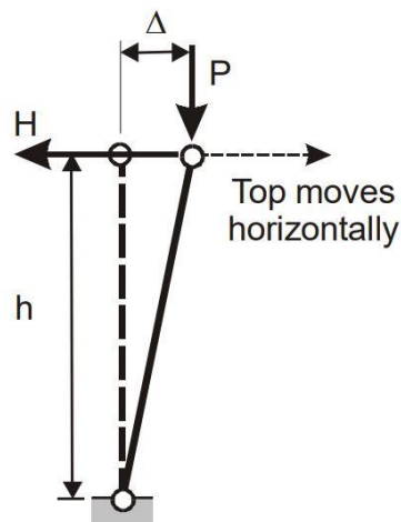
Figure 4.8. Schematic Representation of the P – \Delta Effect (Hill & Mallais, 2004)
