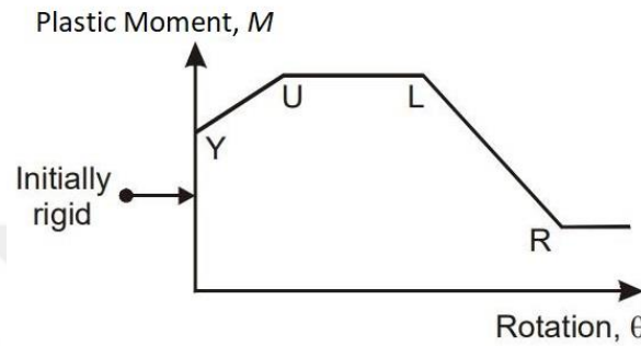
Figure 4.4. Plastic Hinge Moment – Rotation Relationship (Hill & Mallais, 2004)
