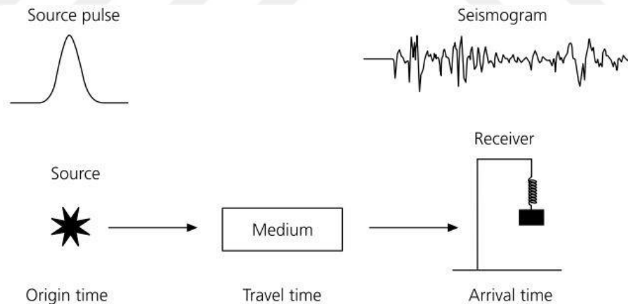
Figure 3.1. Schematic Geometry of Wave Propagation (Stein & Wyssession, 2009)
