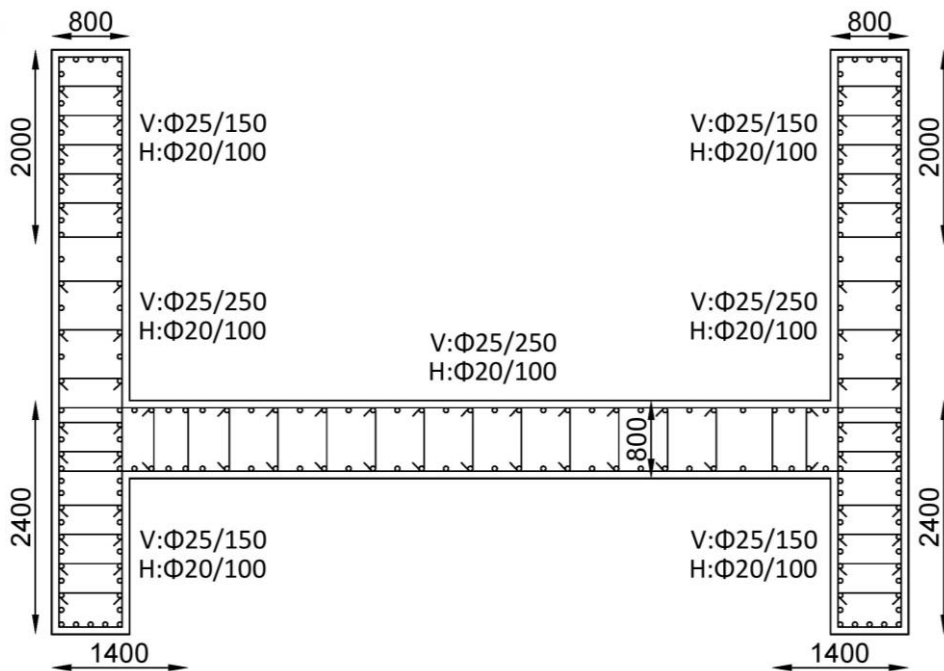
Figure 2.5. Shear Wall Longitudinal Reinforcement for Stories Between 1 - 10
