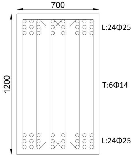
Figure 2.12. Coupling Beam Longitudinal Reinforcement
