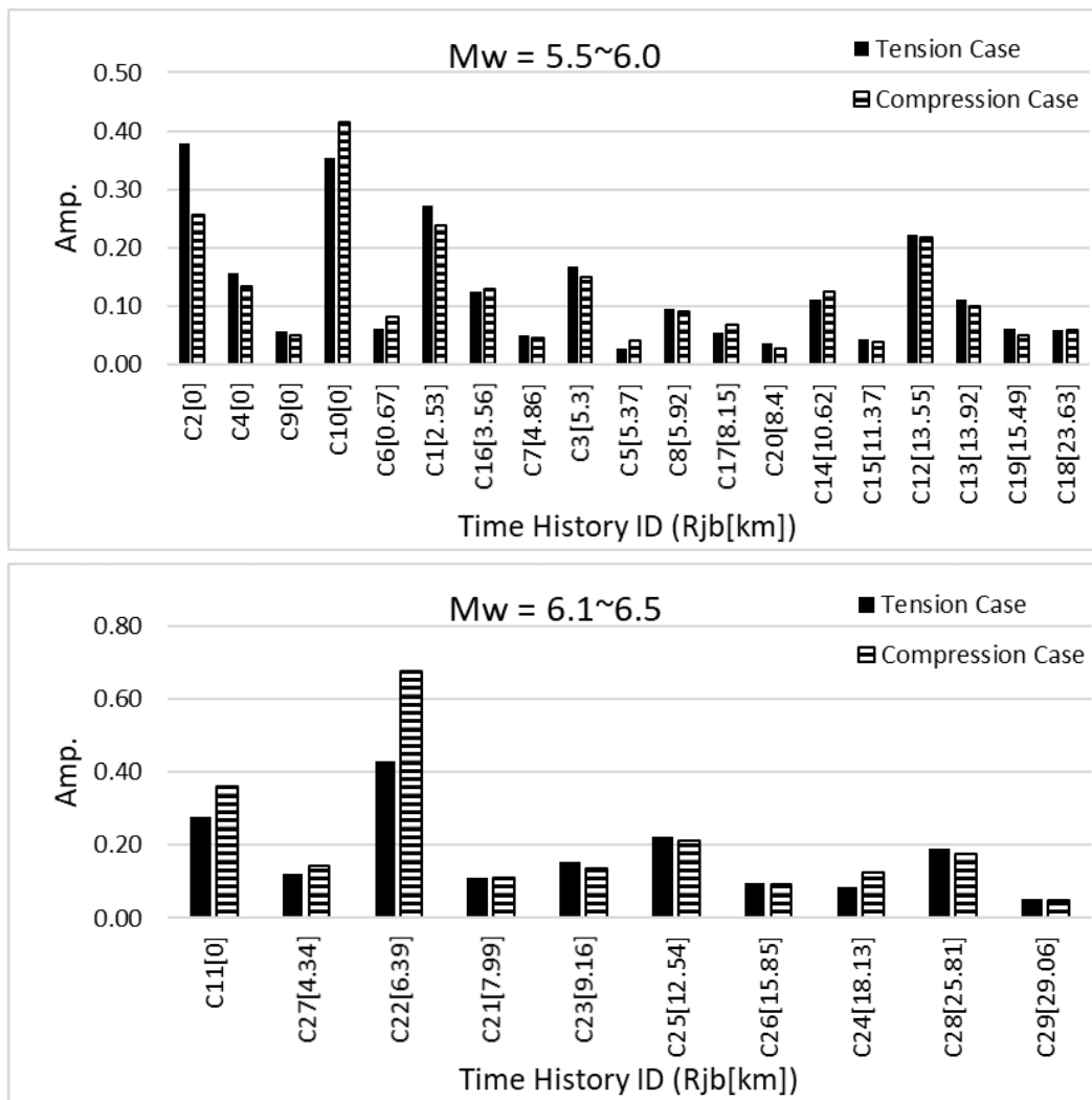
Figure B9. Column Axial Force Results for Site Class C
