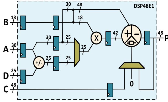
Figure 3.8 Xilinx DSP48E1 Block
