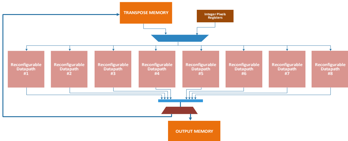
Figure 4.2 Proposed VVC Fractional Interpolation Hardware
