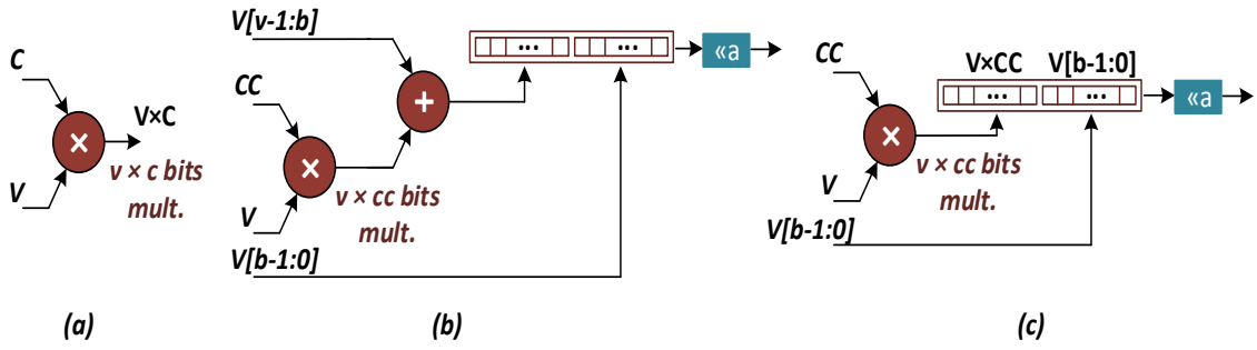
Figure 5.6 Constant Multiplication Hardware (a) Exact Constant Multiplication, (b) Exact Constant Multiplication with Proposed Manipulation, (c) Proposed Approximate Constant Multiplication
