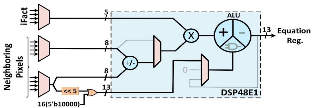
Figure 2.10 Proposed HEVC Intra Prediction Datapath
