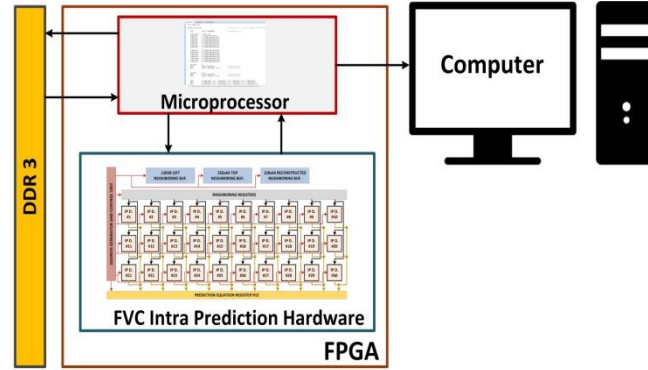
Figure 3.4 FPGA Implementation
