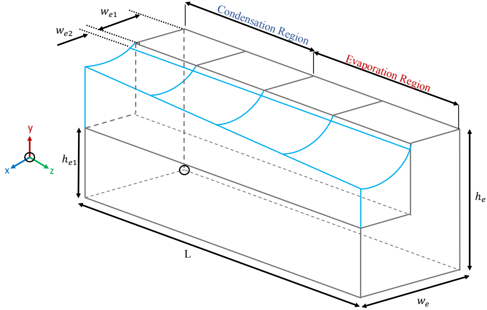
Figure 2.5: Energy solution domain
