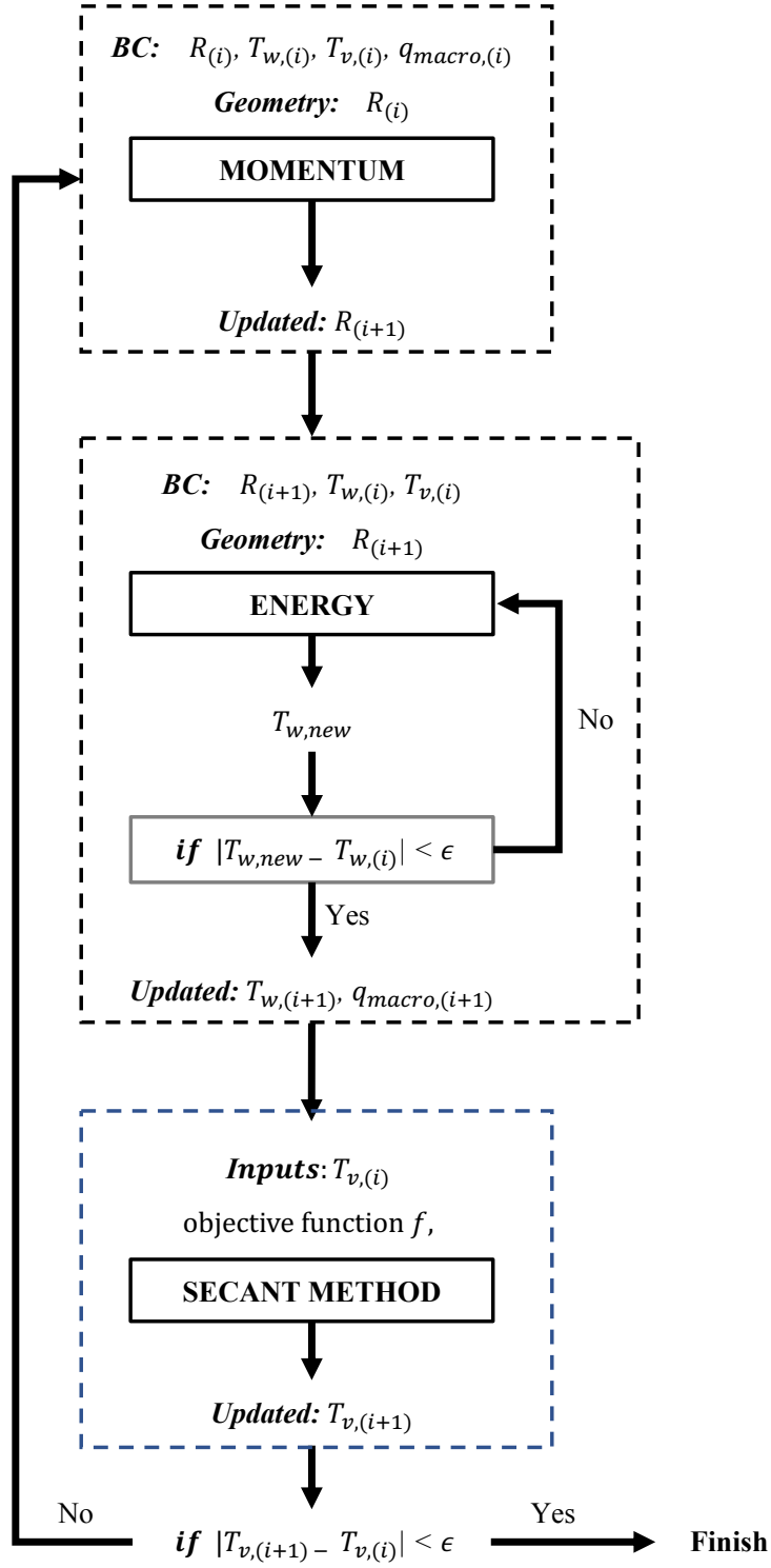
Figure 2.10: Flow chart of the model (BC and i mean phase change boundary condition and iteration index respectively.)
