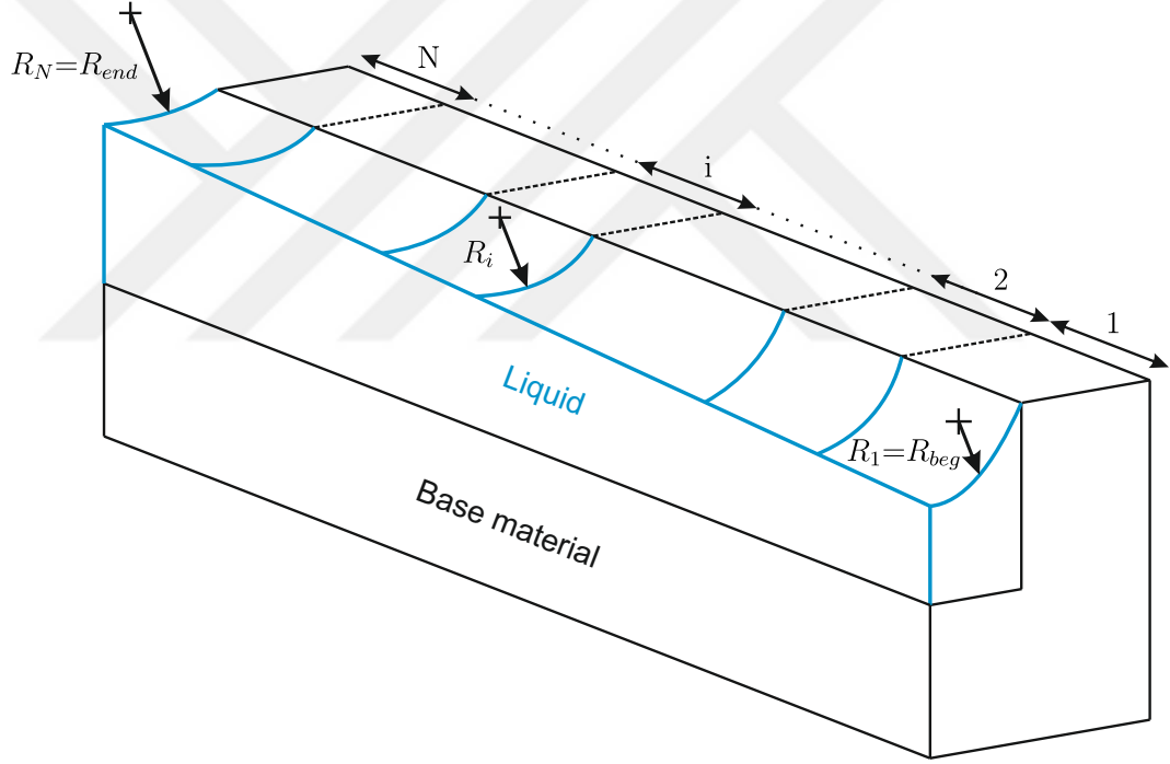
Figure 2.2: Solution domain with joined N-many cross-sections
