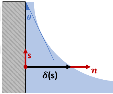
Figure 2.7: Coordinate system for the evaporating thin film calculations
