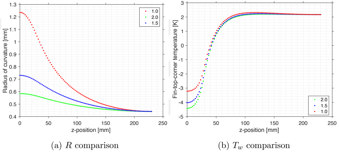
Figure 3.11: Effect of groove width on various parameters
