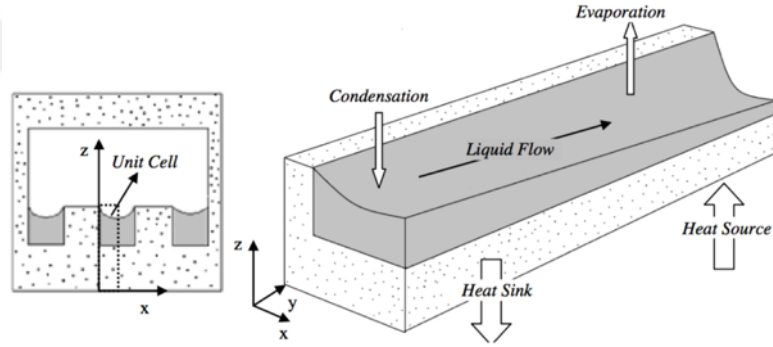
Figure 1.1: Working principle of a micro-grooved heat pipe [15]
