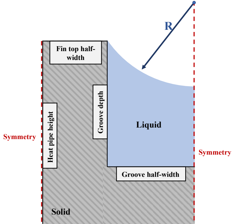
Figure 2.1: A cross-section of the solution domain
