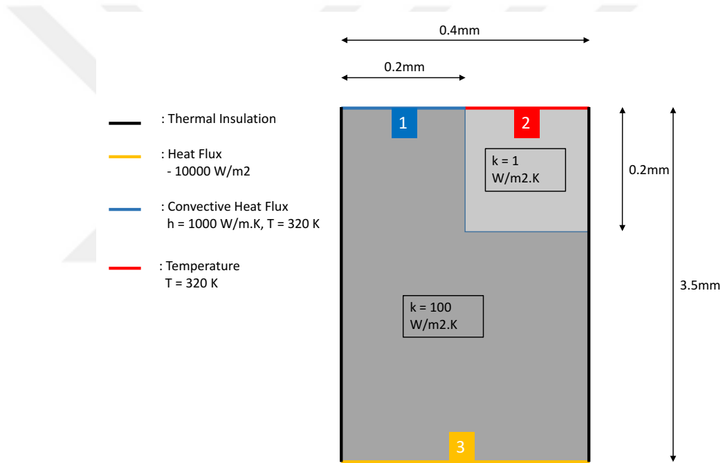
Figure 3.3: Boundary condition for COMSOL / ANSYS comparison
