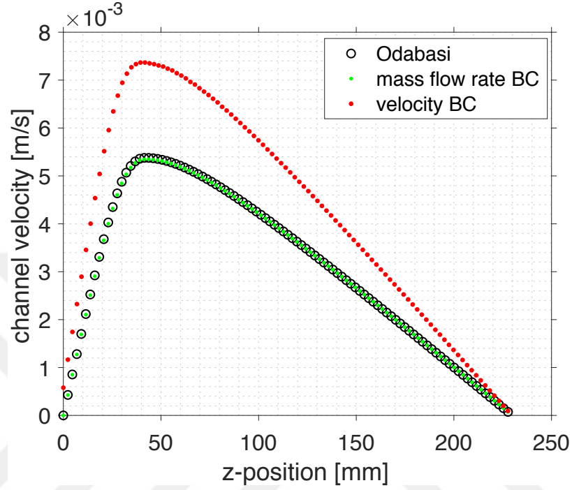
Figure 3.2: Comparison of velocity and mass flow rate boundary conditions (channel velocity)
