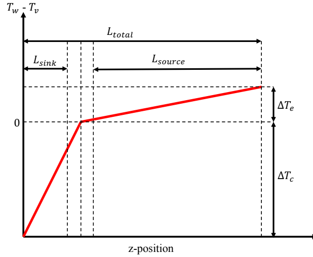
Figure 2.9: Initial guess procedure for T_w
