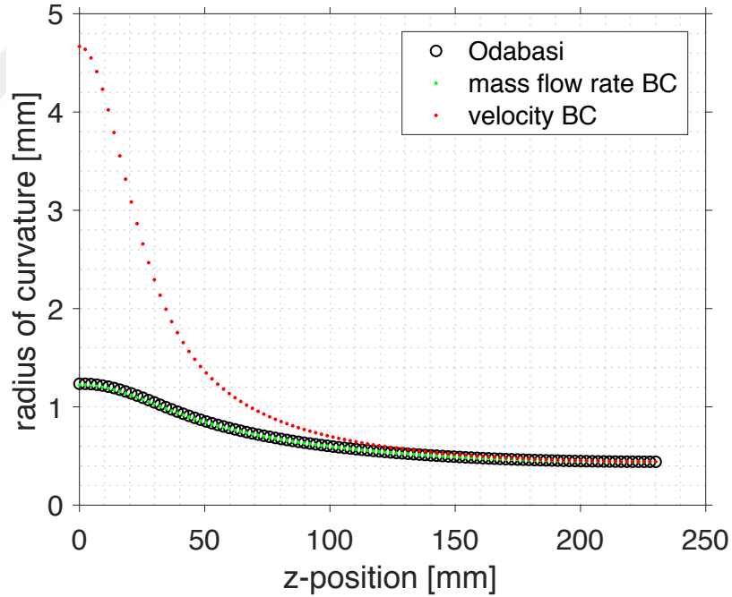
Figure 3.1: Comparison of velocity and mass flow rate boundary conditions ( R )
