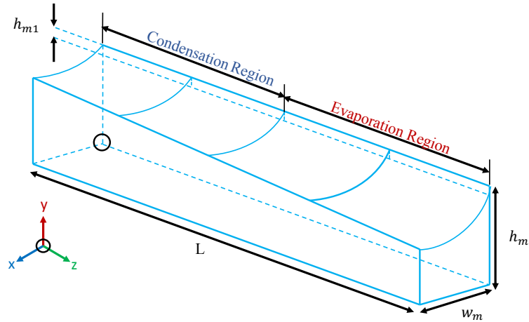
Figure 2.3: Momentum solution domain
