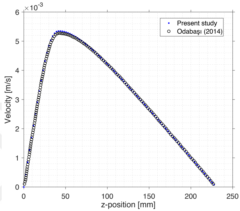
Figure 3.7: Channel velocity verification
