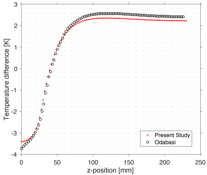
Figure 3.8: Wall temperature verification
