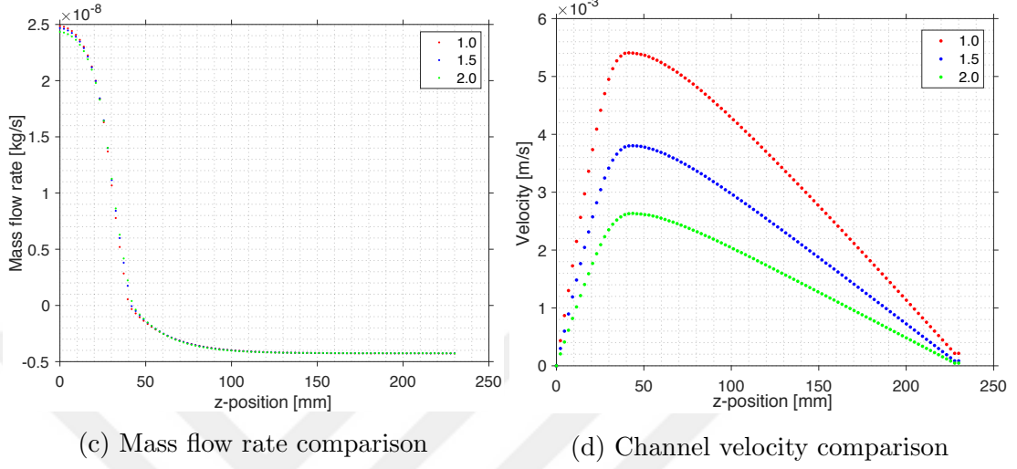
Figure 3.11: Effect of groove width on various parameters
