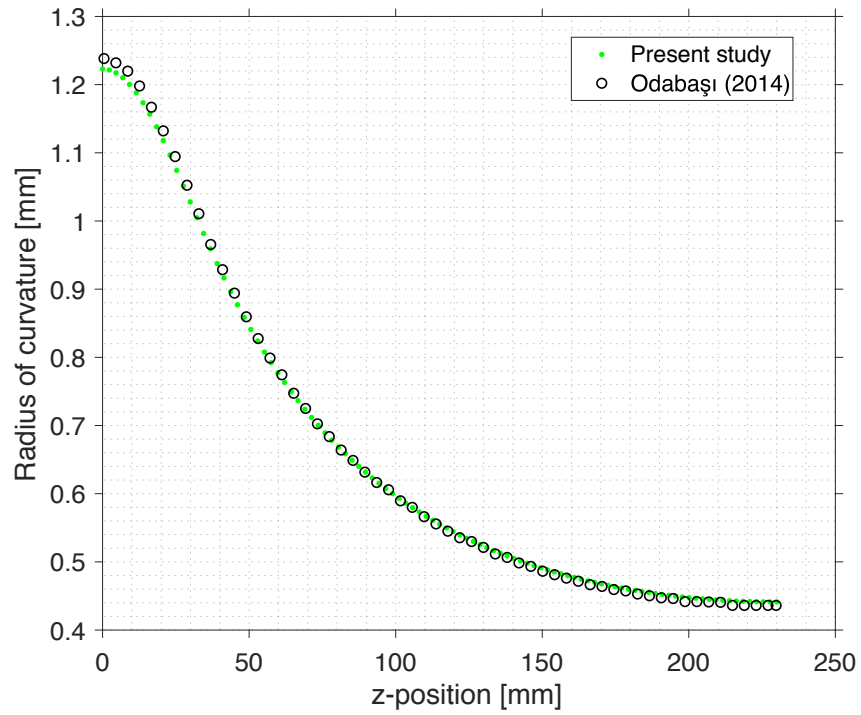
Figure 3.6: Radius of curvature verification
