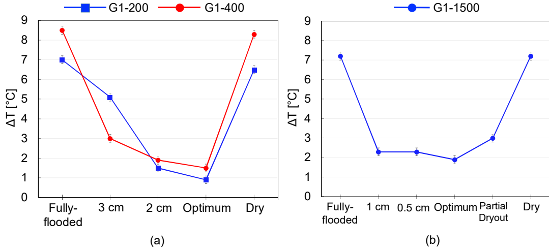
Figure 3.3: \Delta T for different operating conditions for first generation heat pipes: (a) G1-200 and G1-400, (b) G1-1500
