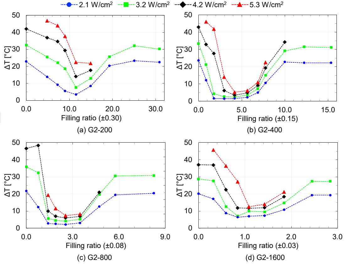
Figure 3.4: Variation of \Delta T with filling ratio under different input heat fluxes for second generation aluminum heat pipes
