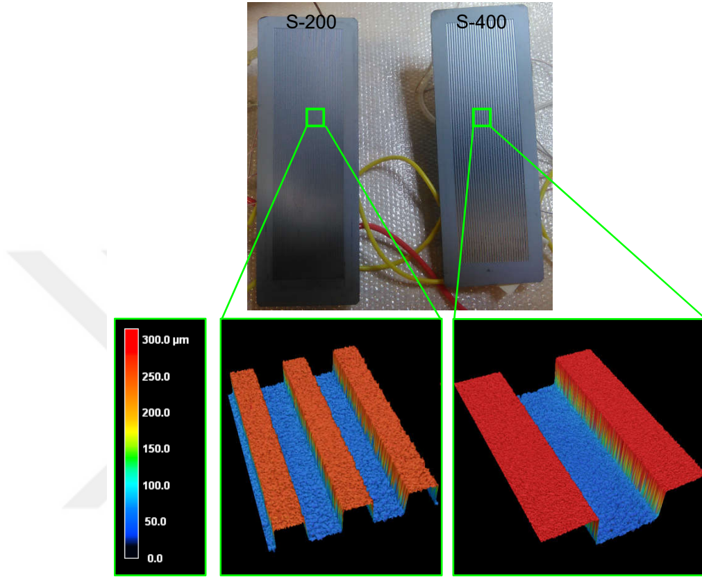
Figure 2.16: Fabricated silicon heat pipes and groove profiles
