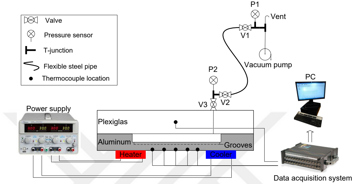
Figure 2.5: Vacuuming station for the first generation prototype aluminum heat pipes (Not to scale.)
