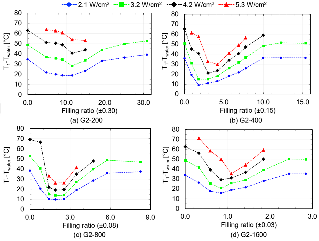
Figure 3.5: Variation of T_1 - T_{water} with filling ratio for second generation aluminum heat pipes for different input heat flux values
