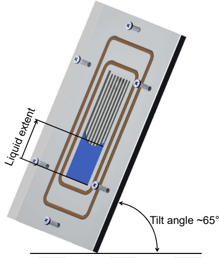
Figure 2.7: Orientation of first generation prototype aluminum heat pipes during the measurements of the liquid extent
