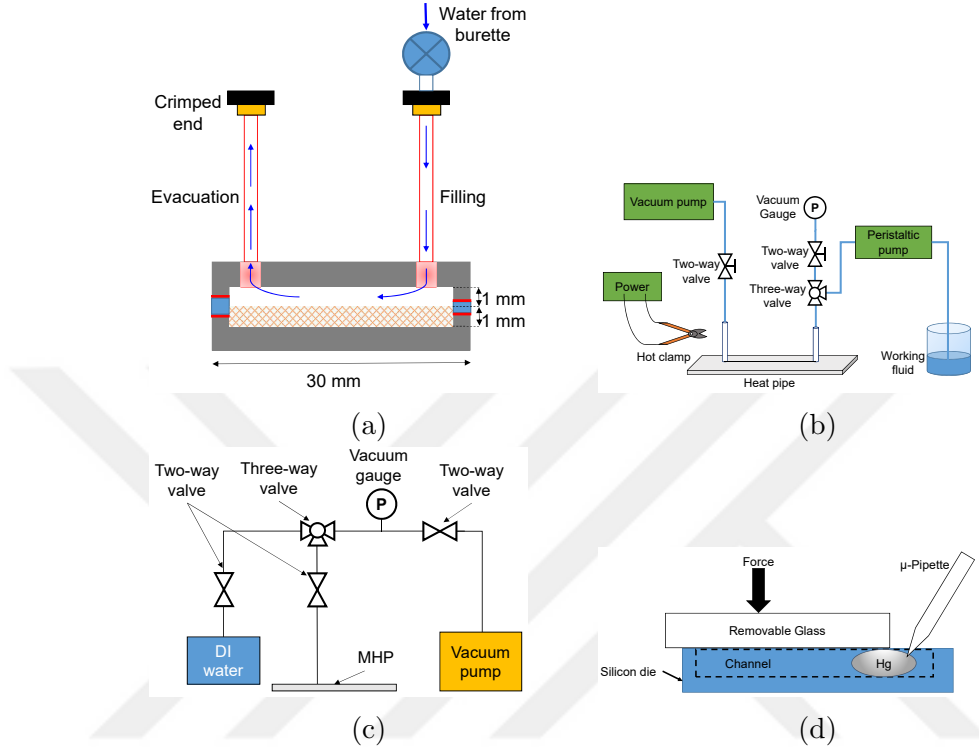
Figure 1.4: Schematic of different charging methods: (a) charging of a planar miniature heat pipe (adapted from [32]), (b) charging of a micro heat pipe (adapted from [33]), (c) charging of a pyrex-silicon heat pipe (adapted from [34]), (d) charging of a heat pipe with liquid metal (adapted from [22])
