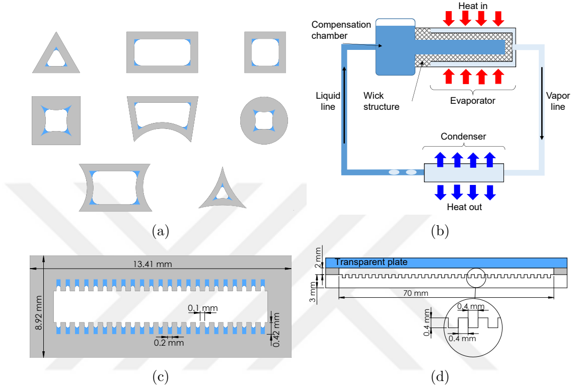
Figure 1.3: Different types of heat pipes: (a) common micro heat pipe cross-sections (adapted from [12]), (b) schematic of a loop heat pipe (adapted from [13]), (c) cross-section of a flat heat pipe with axial rectangular grooves (adapted from [14]), (d) cross-section of a flat plate heat pipe with axial rectangular grooves (adapted from [15])
