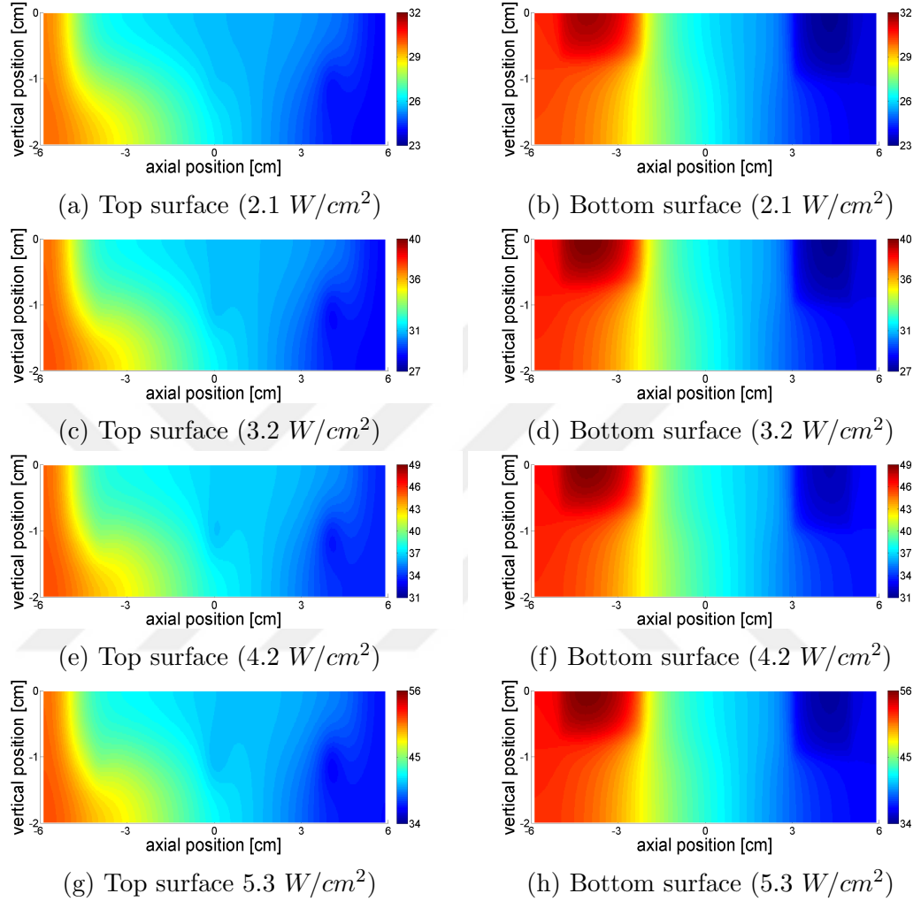
Figure 3.11: Temperature distribution of top and bottom surfaces of G2-800 heat pipe by the computational model under different input heat flux values
