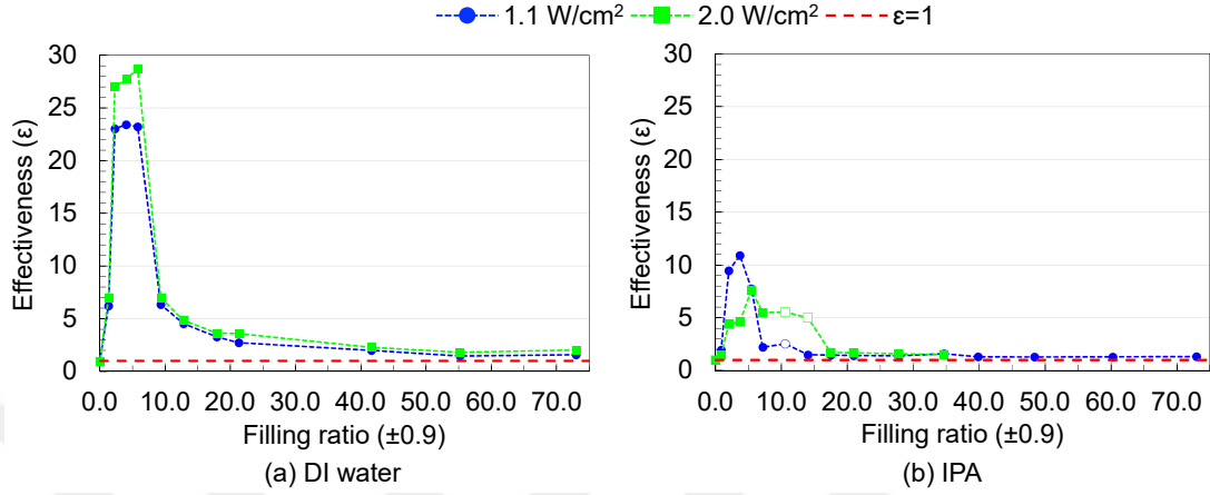
Figure 3.14: Variation of heat pipe effectiveness with filling ratio for heat pipe S-200 under different input heat fluxes (Note: the hollow data points correspond to unsteady operation of the heat pipe.)
