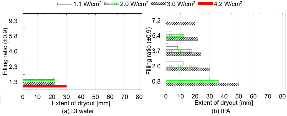
Figure 3.15: Variation of dryout extent with filling ratio for heat pipe S-200 under different input heat fluxes
