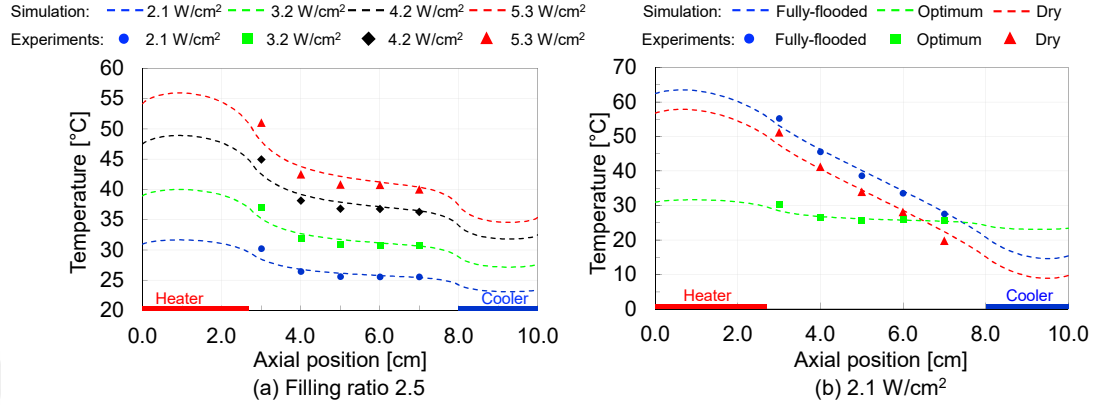
Figure 3.9: Experimental verification of computational model of heat pipe G2-800
