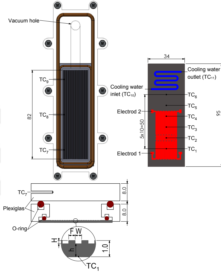
Figure 2.18: Top, bottom, and cross-sectional views of heat pipe S-400
