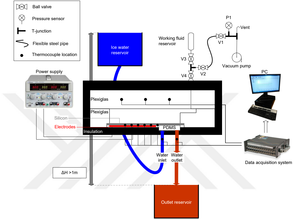
Figure 2.21: Charging and vacuuming station for silicon heat pipes
