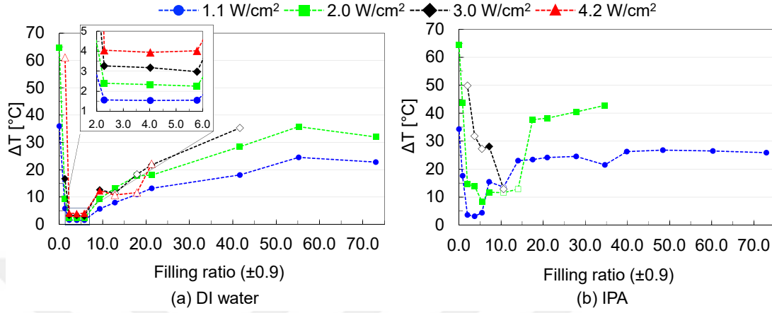
Figure 3.12: Variation of \Delta T with filling ratio for heat pipe S-200 under different input heat fluxes (Note: the hollow data points correspond to unsteady operation of the heat pipe.)
