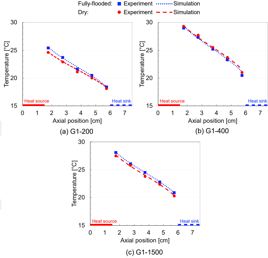
Figure 3.1: Simulated and measured temperatures of first generation prototype aluminum heat pipes
