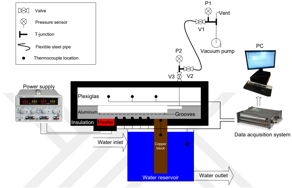
Figure 2.12: Vacuuming station for the second generation aluminum heat pipes (Not to scale.)
