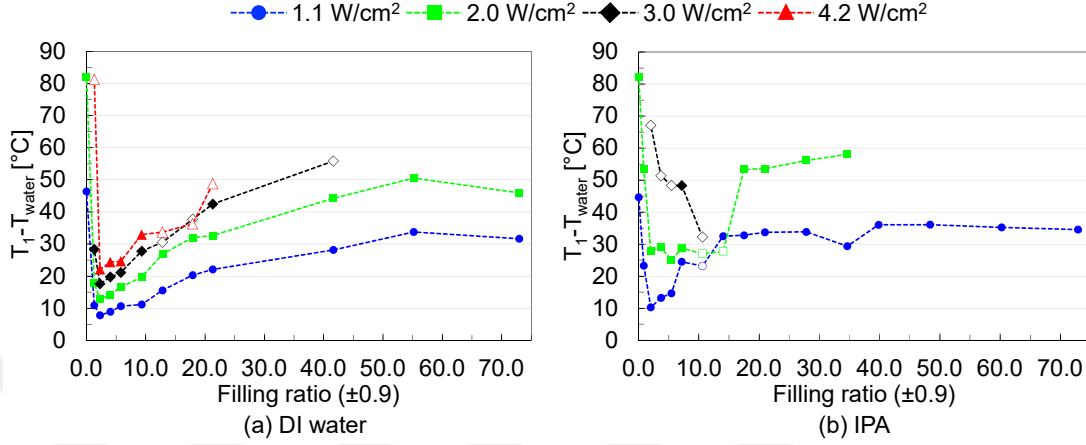
Figure 3.13: Variation of T_1 - T_{water} with filling ratio for heat pipe S-200 under different input heat fluxes (Note: the hollow data points correspond to unsteady operation of the heat pipe.)
