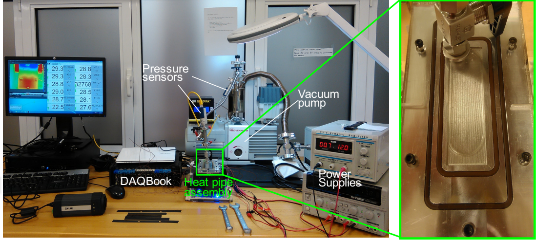
Figure 2.4: Experimental setup and close-up view of test section of the first generation prototype aluminum heat pipes
