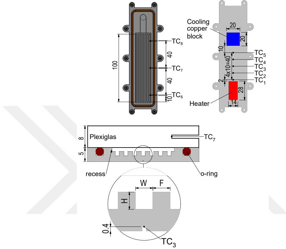
Figure 2.8: Top, bottom and mid cross-sectional views of G2-1600 (all units are in mm)
