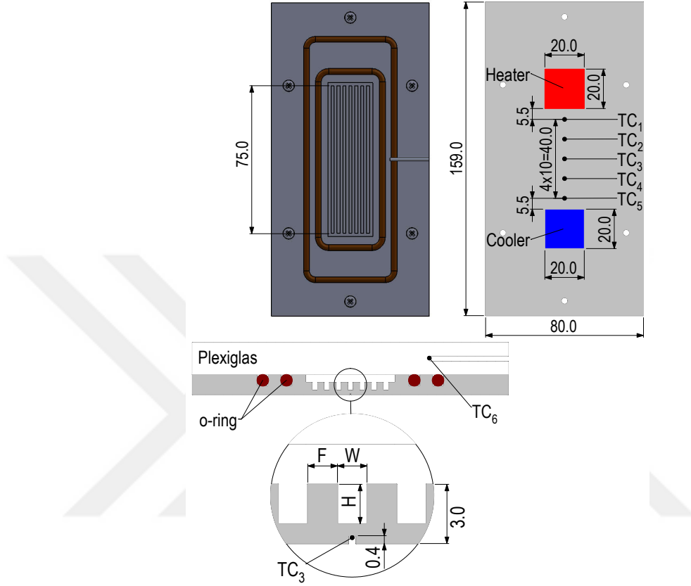
Figure 2.1: Top, bottom, and mid cross-sectional views of G1-1500, and the location of the thermocouples
