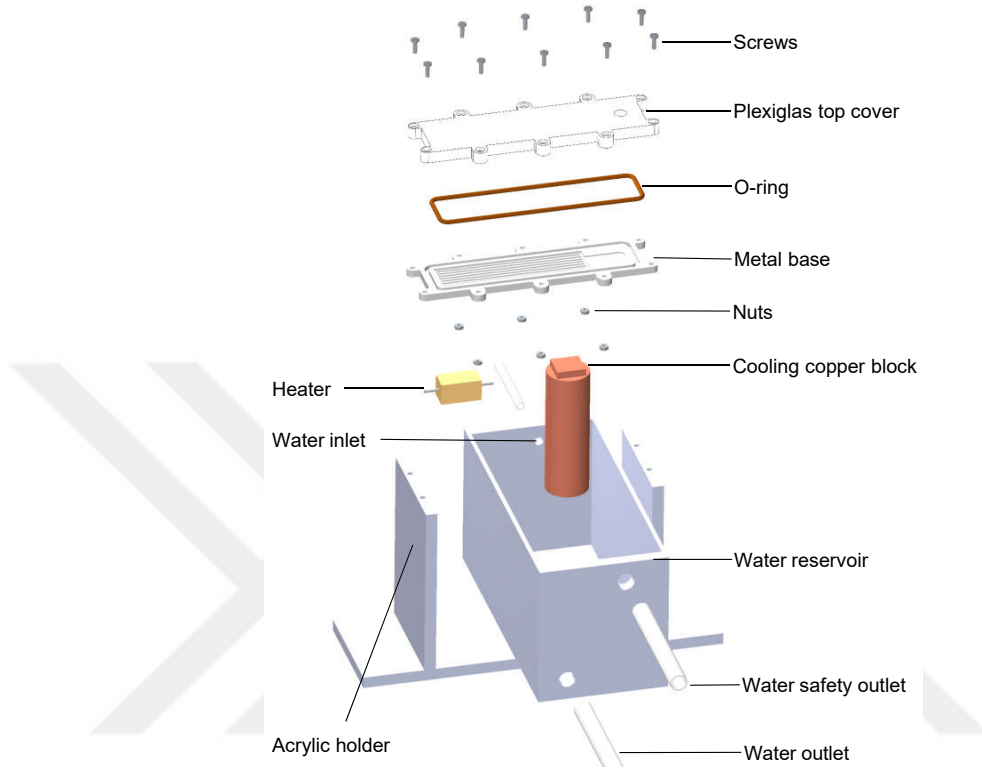
Figure 2.10: The disassembled components of the assembly of the second generation aluminum heat pipes
