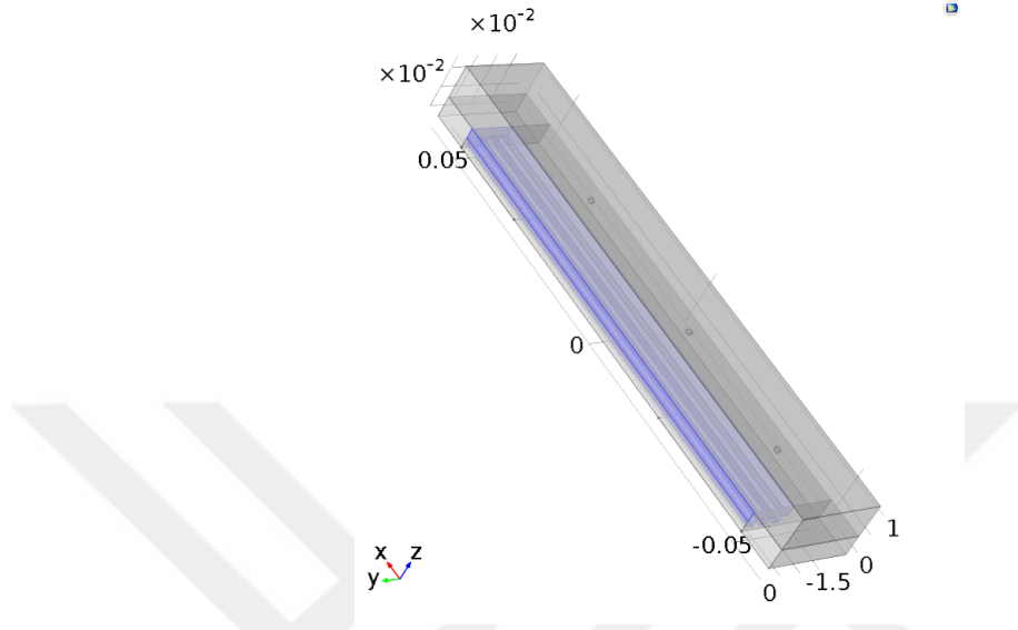
Figure 2.14: Computational domain of heat pipe G2-800 (all units are in m).
