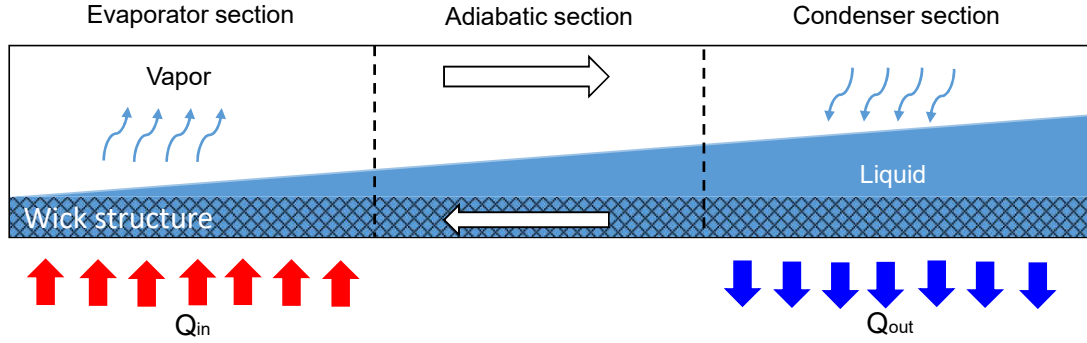
Figure 1.1: Schematic of the working principle and sections of a typical heat pipe, with direction of the vapor and liquid flows
