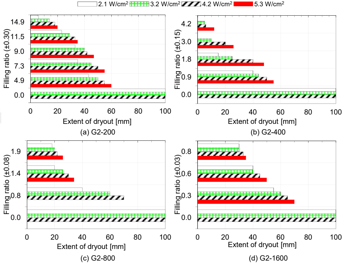
Figure 3.8: Variation of dryout extent with filling ratio for second generation aluminum heat pipes under different input heat fluxes
