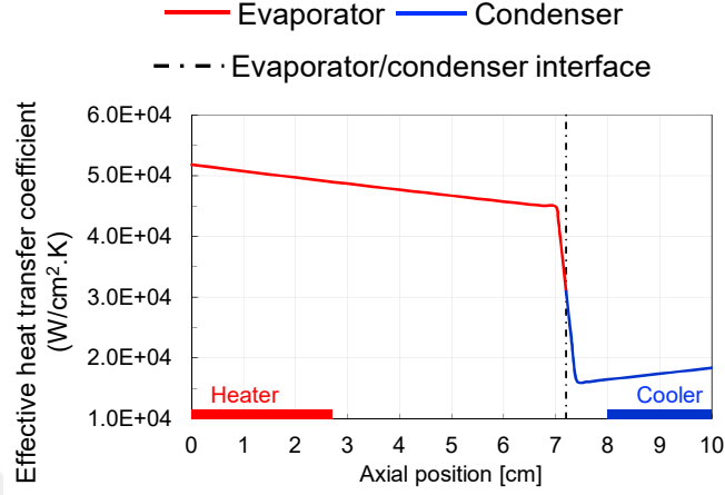
Figure 2.15: Phase change heat transfer coefficients of the evaporator and condenser sections of heat pipe G2-800
