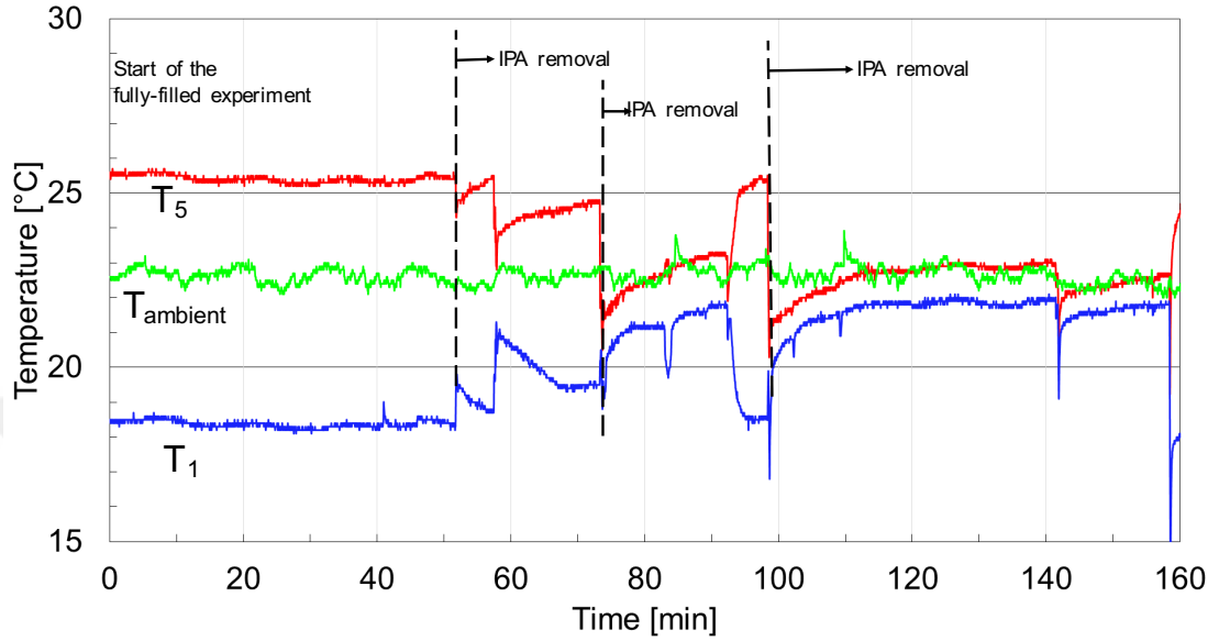
Figure 2.6: Transient temperature variation of heat pipe G1-200
