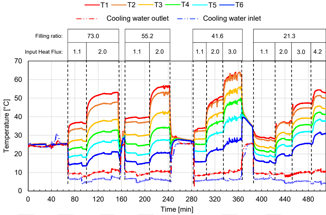
Figure 2.22: Transient temperature variation of heat pipe S-200 charged with DI water
