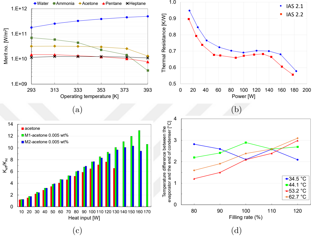
Figure 1.5: Different parameters to characterize the thermal performance of heat pipes: (a) Merit number (adapted from [49]), (b) total thermal resistance (adapted from [24]), (c) effective thermal conductivity (adapted from [20]), (d) temperature difference between the evaporator and condenser (adapted from [43])
