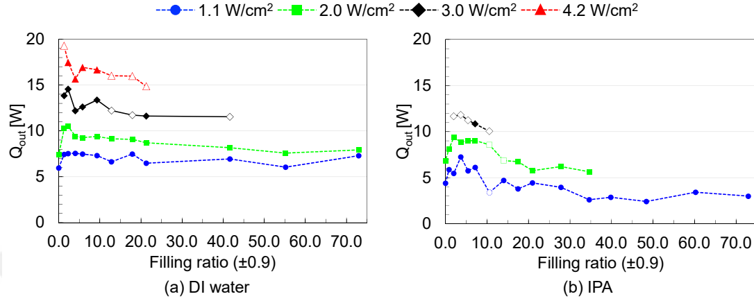
Figure 3.16: Variation of heat output with filling ratio under different input heat loads for heat pipe S-200 (Note: the hollow data points correspond to unsteady operation of the heat pipe.)
