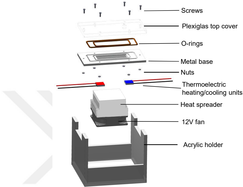
Figure 2.3: The disassembled components of the assembly of the first generation prototype aluminum heat pipes
