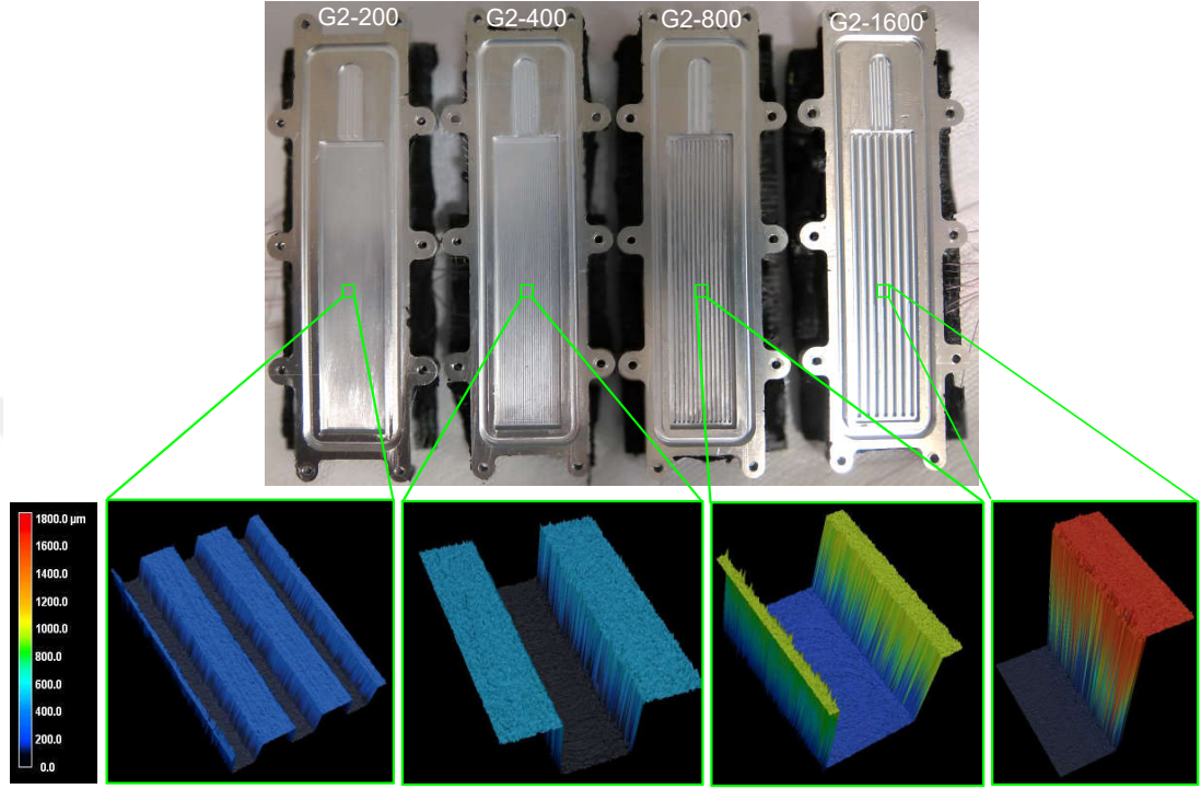
Figure 2.9: Fabricated metal pieces and the groove profiles of the second generation aluminum heat pipes
