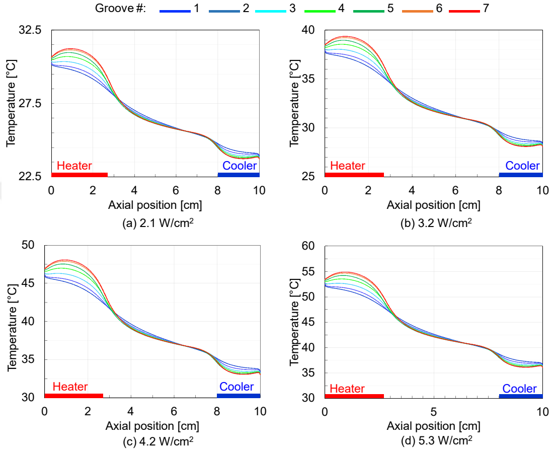
Figure 3.10: Simulated temperature distribution along the grooves of heat pipe G2-800 for different input heat flux values
