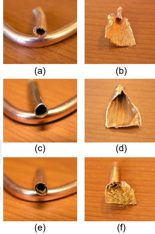
Figure 1.2: Three types of wick structures [4], sineterd wick: (a) cross-sectional view, (b) cut-up heat pipe, groove wick: (c) cross-sectional view, (d) cut-up heat pipe, mesh wick: (e) cross-sectional view, (f) cut-up heat pipe.
