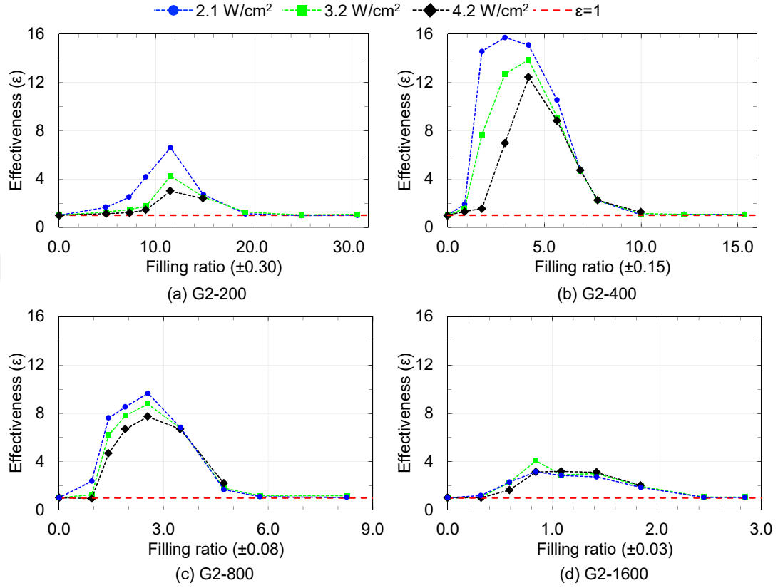
Figure 3.6: Variation of effectiveness with filling ration for second generation aluminum heat pipes under different input heat flux values
