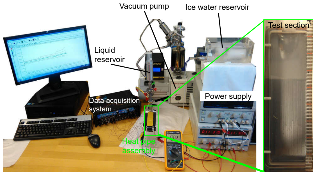
Figure 2.20: Experimental setup table of silicon heat pipes
