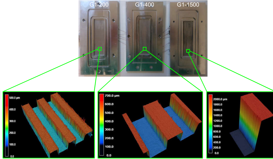
Figure 2.2: Fabricated metal pieces and the groove profiles of the first generation prototype aluminum heat pipes
