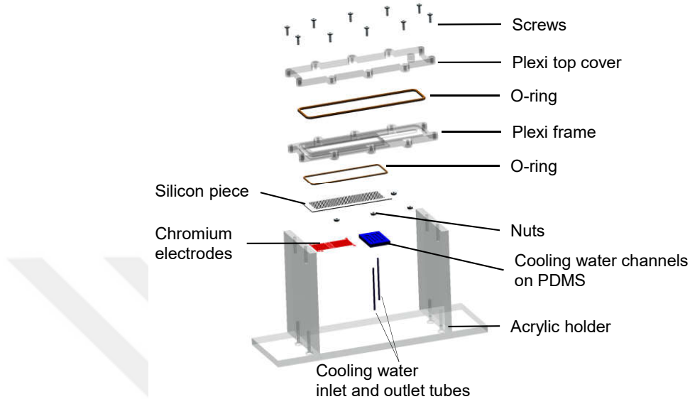
Figure 2.19: The disassembled components of the assembly of silicon heat pipes
