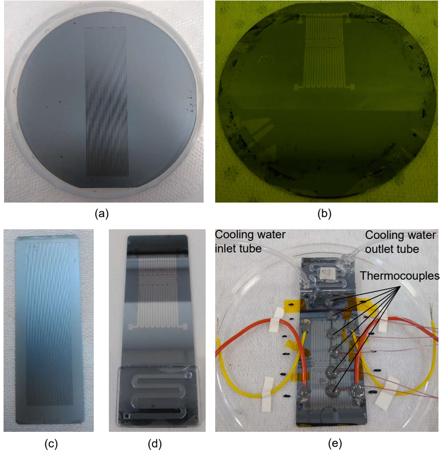
Figure 2.17: Fabrication steps of silicon heat pipes
