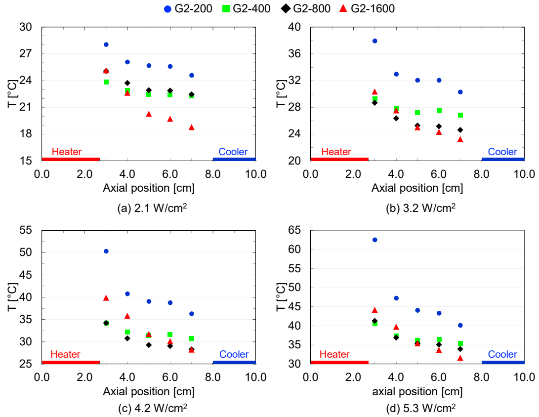
Figure 3.7: Variation of temperature with axial position under different input heat fluxes for second generation aluminum heat pipes working at their optimum filling ratios
