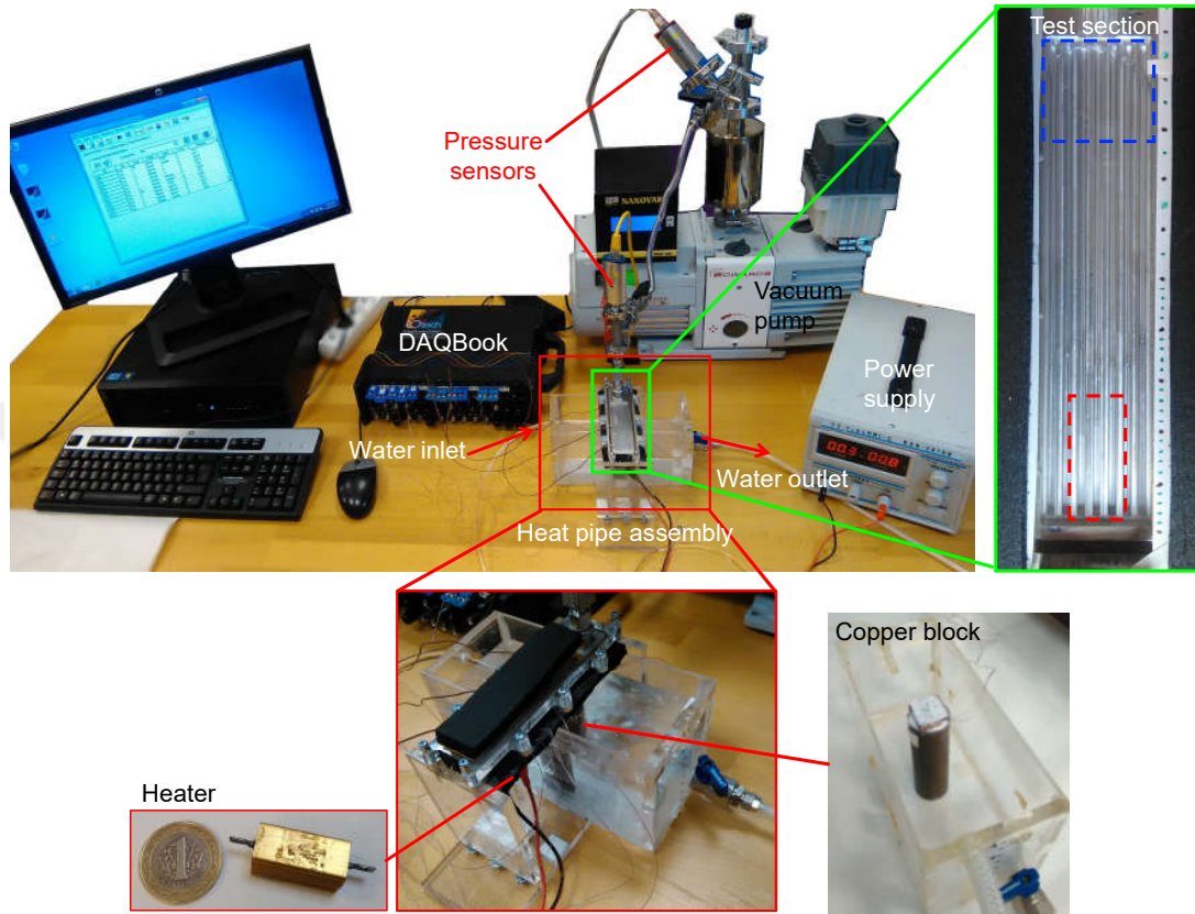
Figure 2.11: Experimental setup table of the second generation aluminum heat pipes
