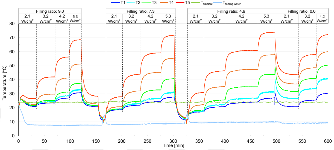
Figure 2.13: Transient temperature variation of heat pipe G2-200
