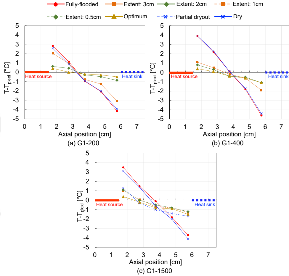
Figure 3.2: Temperature differences between thermocouples on the bottom of the metal base ( T_1 through T_5 ) and the one on plexiglas ( T_6 ) for first generation prototype aluminum heat pipes
