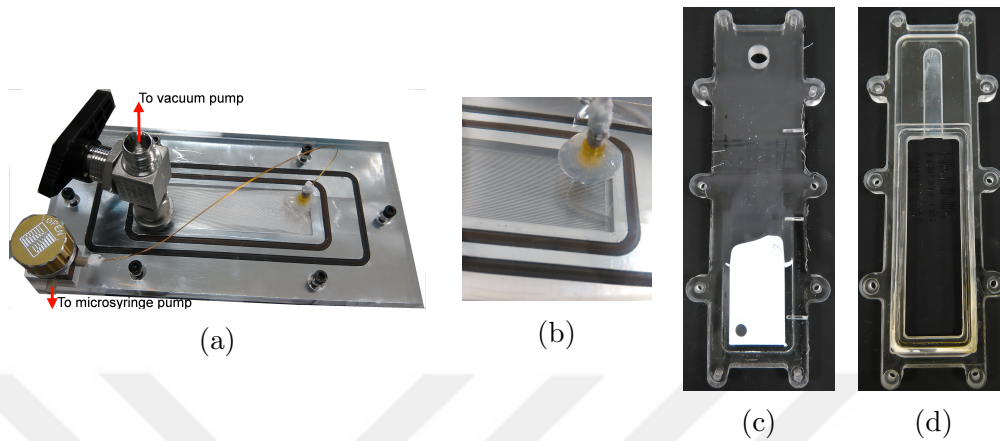
Figure 2.23: Examples of failures during the experiments: (a) the first charging method, (b) incompatibility of water with aluminum surface, (c) and (d) burnt plexiglas cover pieces (Note: the scale of the photographs are not identical.)
