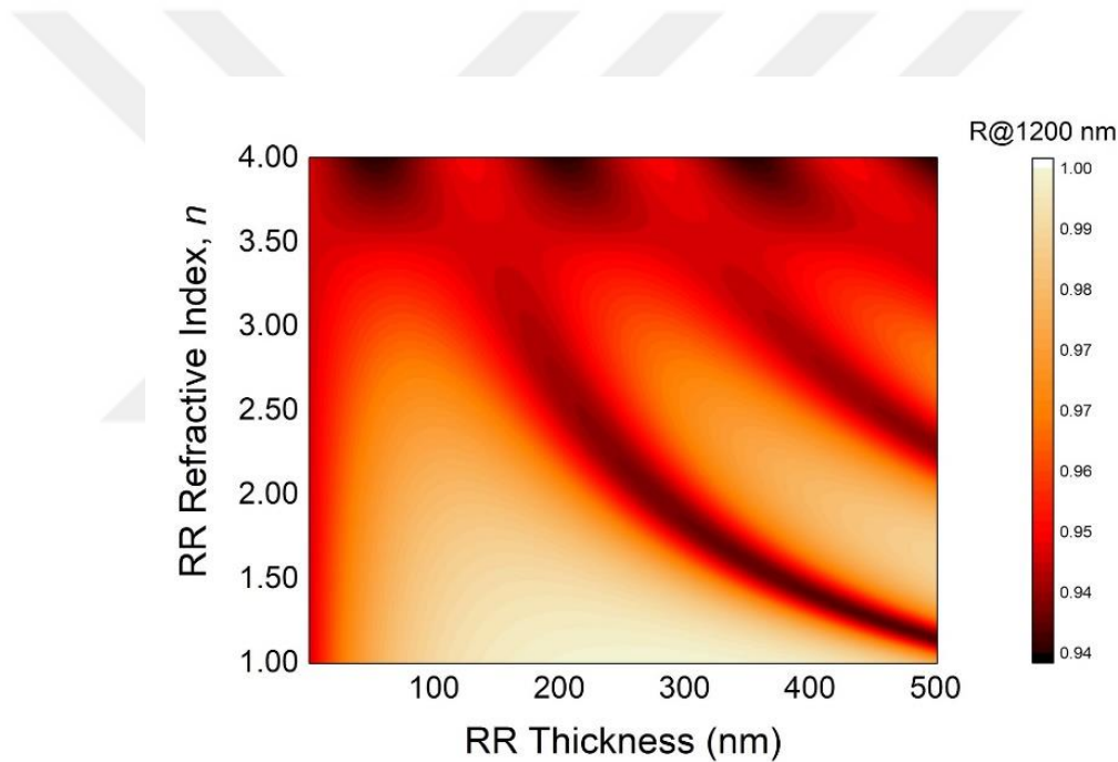
Figure 60 Internal reflectance at the rear interface at 1200 nm wavelength as a function of the RR refractive index and thickness.
