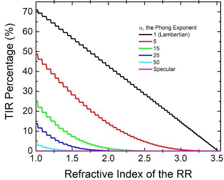
Figure 61 The percentage of the TIR as a function of the refractive index of the RR for various Phong exponents at normal incidence.
