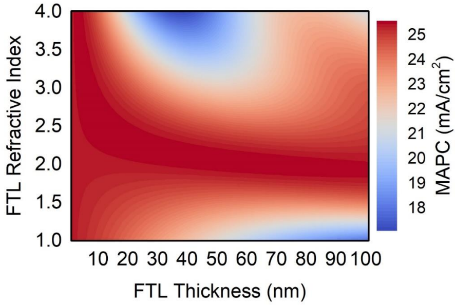
Figure 36 MAPC as a function of the refractive index and thickness of the front transport layer. PTB7:PCBM is used with a thickness of 400 \mu\text{m} and no RTL and metal layers are used.
