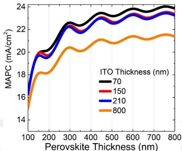
Figure 28 Variation of MAPC with perovskite thickness for various ITO thicknesses, \text{NiO}_x and PCBM thicknesses are taken as 30 nm and 50 nm, respectively. MAPC decreases with the thickness and the extinction coefficient (Figure 116, see Appendix B) of TCO due to enhanced parasitic absorption.
