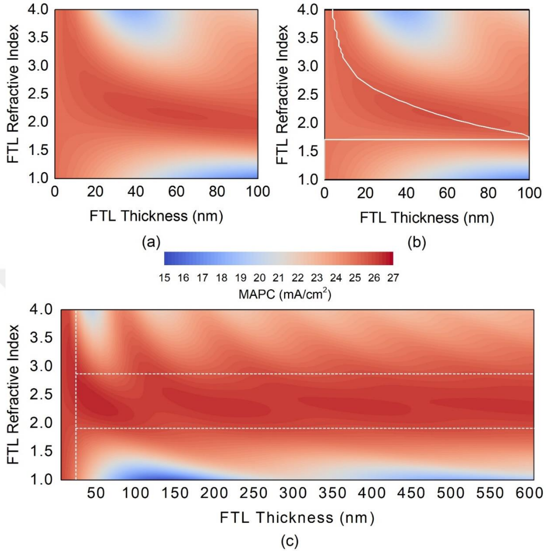
Figure 12 MAPC for a semi-infinite perovskite as a function of FTL thickness and refractive index for ITO thicknesses of (a) 150 nm, (b) 210 nm, and (c) 70 nm (extended). The white solid line in (b) indicates the optimum FTL thickness for FTL refractive index calculated with Equation 56. White dashed lines in (c) separate three regions with distinct behaviors.
