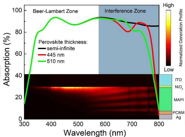
Figure 19 Absorption spectra of perovskite at thicknesses of semi-infinite, 445 nm and 510 nm for \text{NiO}_x , PCBM and Ag thicknesses of 30 nm, 50 nm, 100 nm, respectively. Inset: The weighted spectral absorption rate of photon profile within the depth of 445 nm perovskite.
