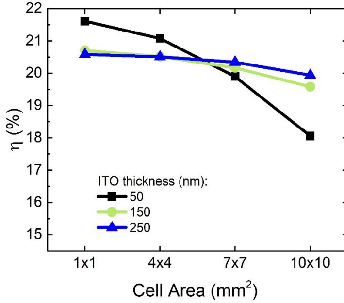
Figure 50 Variation of lab-type solar cell efficiency as a function of the cell length with 50, 150, and 250 nm thick ITO layers. J_0 , n , \rho , R_{sh} are assumed to have values of 2.8 \times 10^{-11} mA/cm², 1.5, 2.025 \times 10^{-4} Ω.cm, and infinity, respectively.
