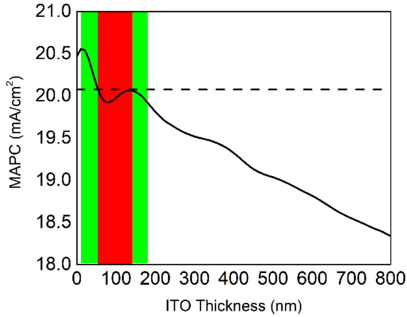
Figure 42 MAPC as a function of ITO thickness for a 240 nm-thick active layer. Recommended (green) and non-recommended regions (red) are highlighted
