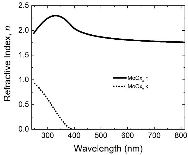
Figure 115 Measured refractive index spectra of \text{MoO}_x .
