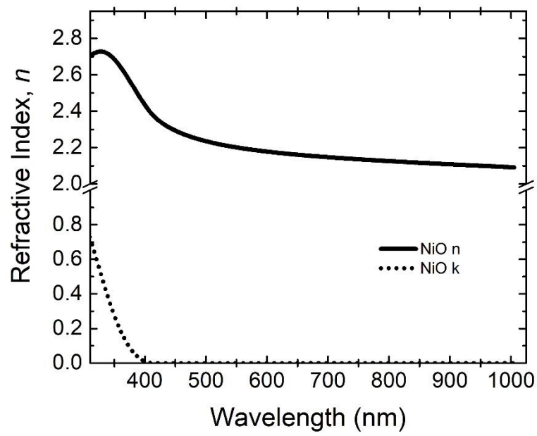
Figure 111 Measured refractive index spectra of \text{NiO}_x .
