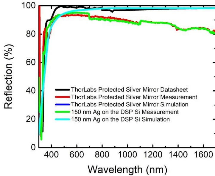
Figure 68 Measured and supplied reference reflection spectra of the protected silver coated mirror from ThorLabs and fabricated 150nm-thick Ag coated DSP silicon substrate. Along with the corresponding simulated reflection spectra.
