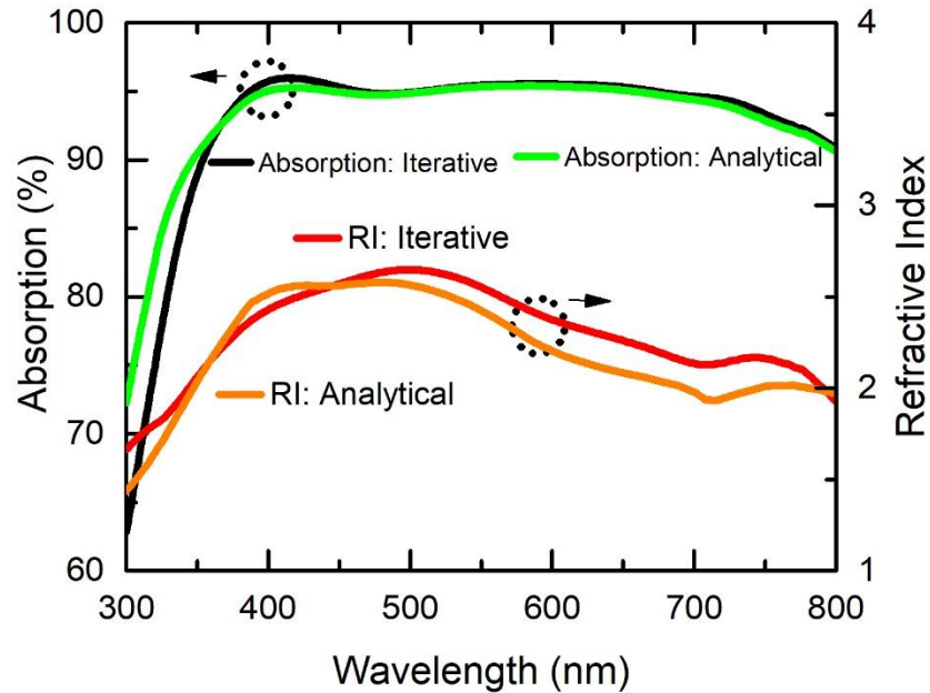
Figure 15 Absorption spectra of computed champion refractive index profile, optimum thicknesses (40nm TL and 70nm ITO) are given with numerically and iteratively found champion refractive index profiles.
