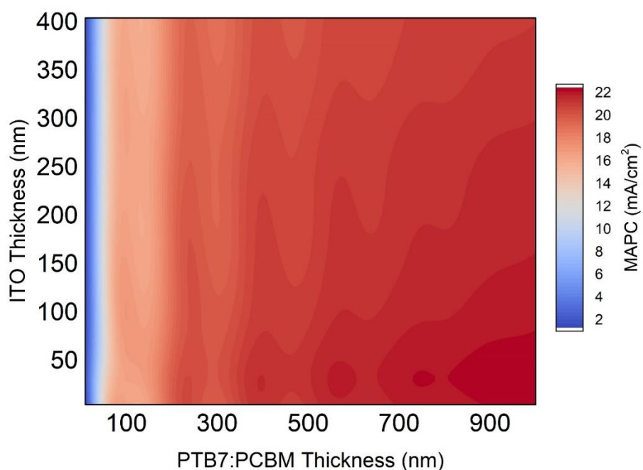
Figure 38 MAPC as a function of ITO and the active layer thicknesses.
