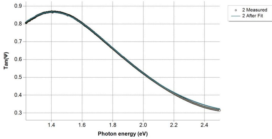
Figure 89 Fitted and measured \tan(\psi) data of aerogel.
