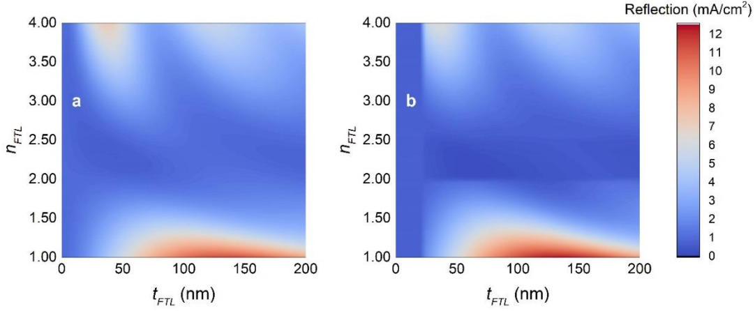
Figure 14 Comparison of weighted reflections obtained by simulations (a) and analytical calculations (b). Reflection losses are presented as current flux as a function of the thickness and refractive index of FTL.
