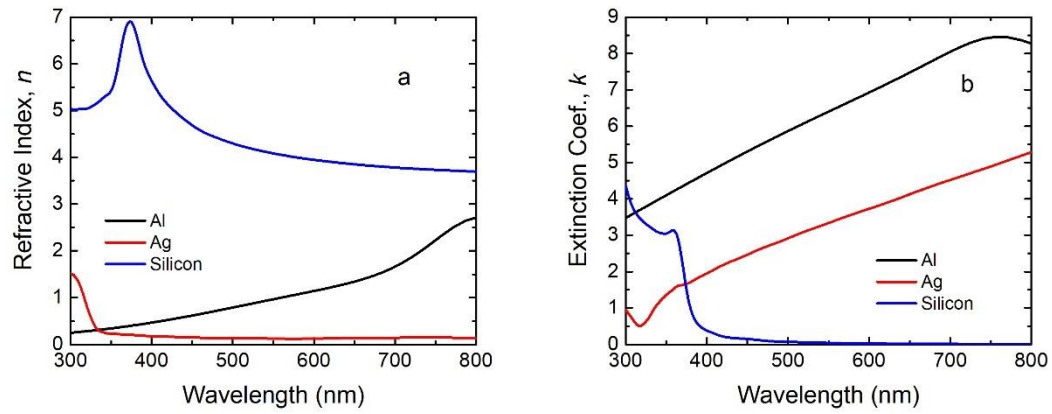
Figure 117 Adopted refractive index (a) and extinction coefficient (b) spectra of Al, Ag, and silicon used in Chapter 4.
