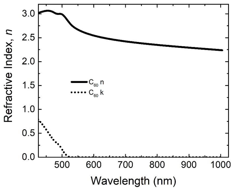
Figure 114 Measured refractive index spectra of C_{60} .
