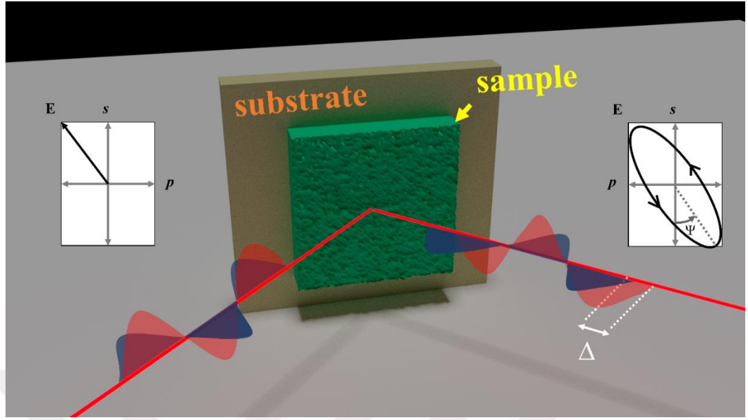
Figure 6 Illustration of a typical spectroscopic ellipsometry measurement.
