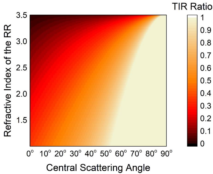
Figure 62 The ratio of the TIR as a function of the refractive index of the RR and the central scattering angle for the Lambertian scattering profile.
