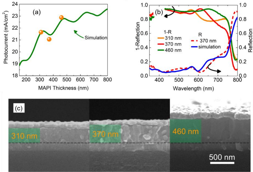
Figure 33 (a) Available photocurrent (in wavelengths between 350 and 800 nm) calculated using Equation 1 where A is replaced by 1-R as a function of perovskite thicknesses for a perovskite solar cell with 115 nm ITO, 33 nm NiO x , 25 nm C 60 , 7 nm BCP and 100 nm Ag. Orange circles, extracted from 1-reflection measurements, are the total available photocurrent of fabricated solar cells with perovskite thicknesses of 310, 370 and 460 nm. (b) Measured 1-Reflection spectra for perovskite solar cells with thicknesses of 310, 370 and 460 nm, and measured and simulated reflection spectrum for the perovskite solar cell with a thickness of 370 nm. (c) Cross-section SEM images of fabricated solar cells.
