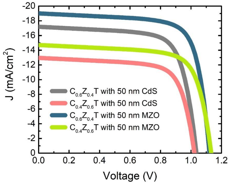
Figure 88 Top cell J-V curves of selected C_{1-x}Z_xT cases ( x = 0.4, 0.6 ) with 50 nm ETL (CdS and MZO).
