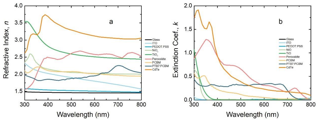
Figure 116 Refractive index (a) and extinction coefficient (b) spectra of adopted materials used in Chapter 3.
