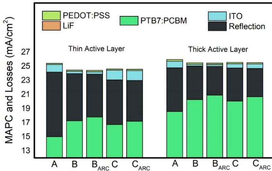
Figure 45 MAPCs and losses of the reference (A), optimized with the optically best ITO (B) and optimized with optically favorable and low sheet resistance layer for the thin and thick active layer cases and along with the ARC coated structures.
