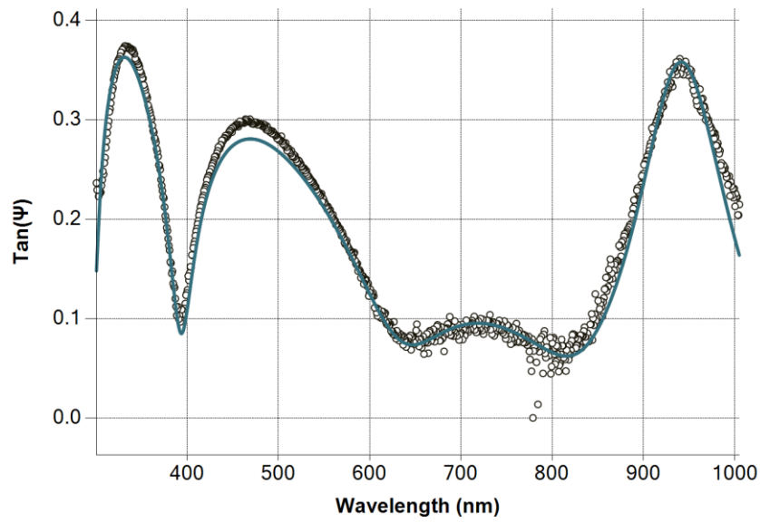
Figure 99 \tan(\psi) spectra of ITO with fitted dispersion law (line) and measurement (dots).
