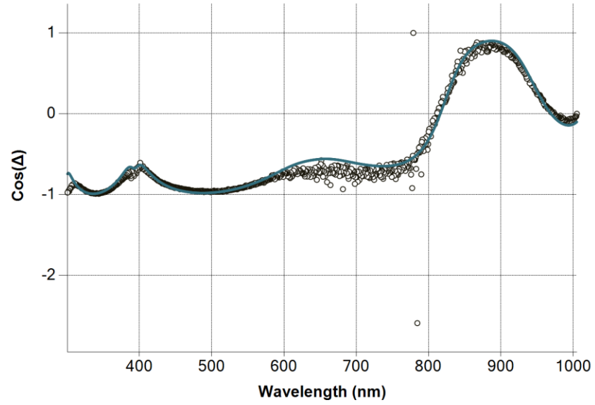
Figure 100 \cos(\Delta) spectra of ITO with fitted dispersion law (line) and measurement (dots).
