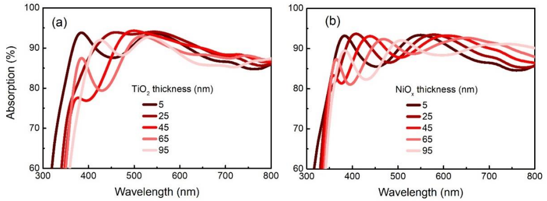
Figure 17 Absorption spectra of semi-infinite perovskite for various \text{TiO}_2 and \text{NiO}_x thicknesses.
