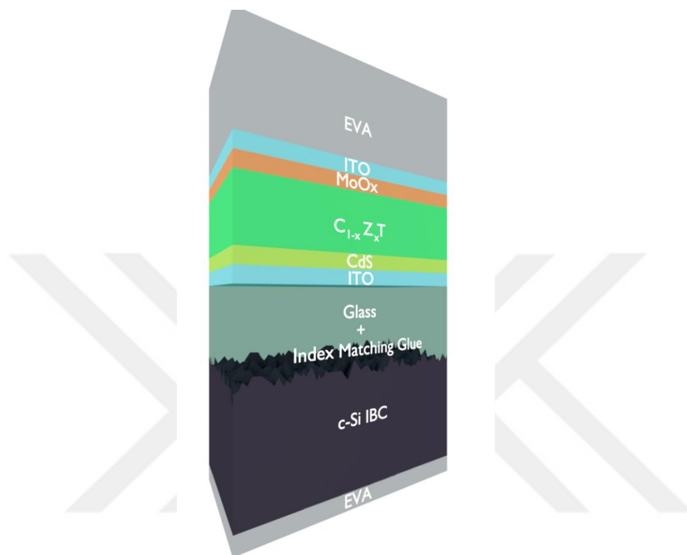
Figure 82 Schematic of the inverted structure. Front and rear TCO is ITO, ETL is CdS, HTL is MoO x , index matching glue is employed between two cells. EVA is used to protect IBC Si cell contacts; glass is employed as the substrate.
