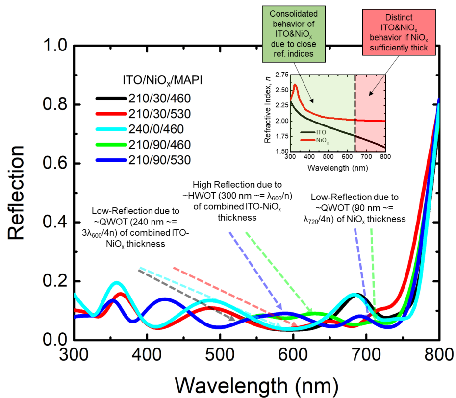
Figure 122 Reflection spectra of perovskite solar cell with various ITO, NiO x , and perovskite thickness combinations. Inset: Refractive index spectra of ITO and NiO x .
