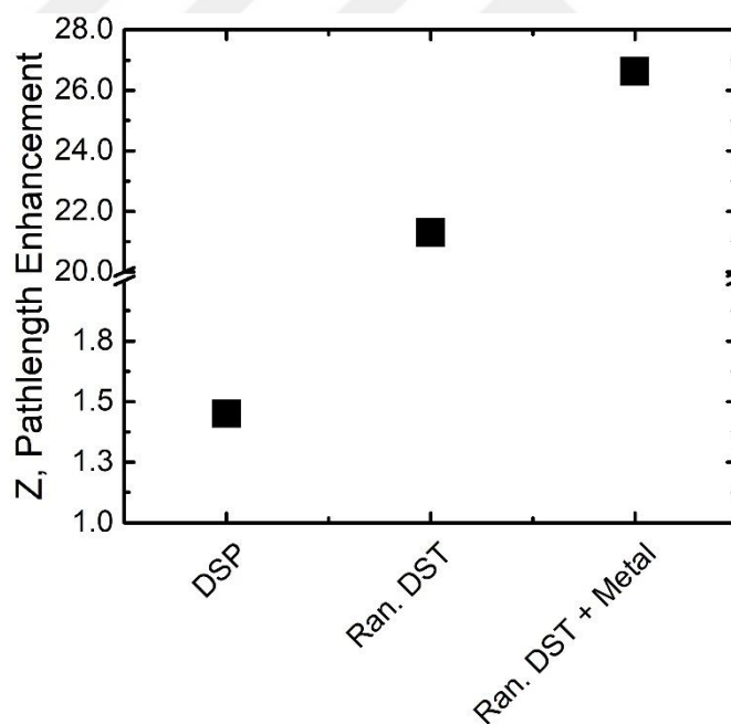
Figure 69 Path length enhancements for various front and rear surface morphologies at 1200 nm wavelength.
