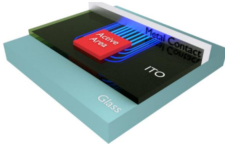
Figure 49 Illustration of the photogenerated charge collection in a lab-type perovskite solar cell with the current spreading phenomenon.
