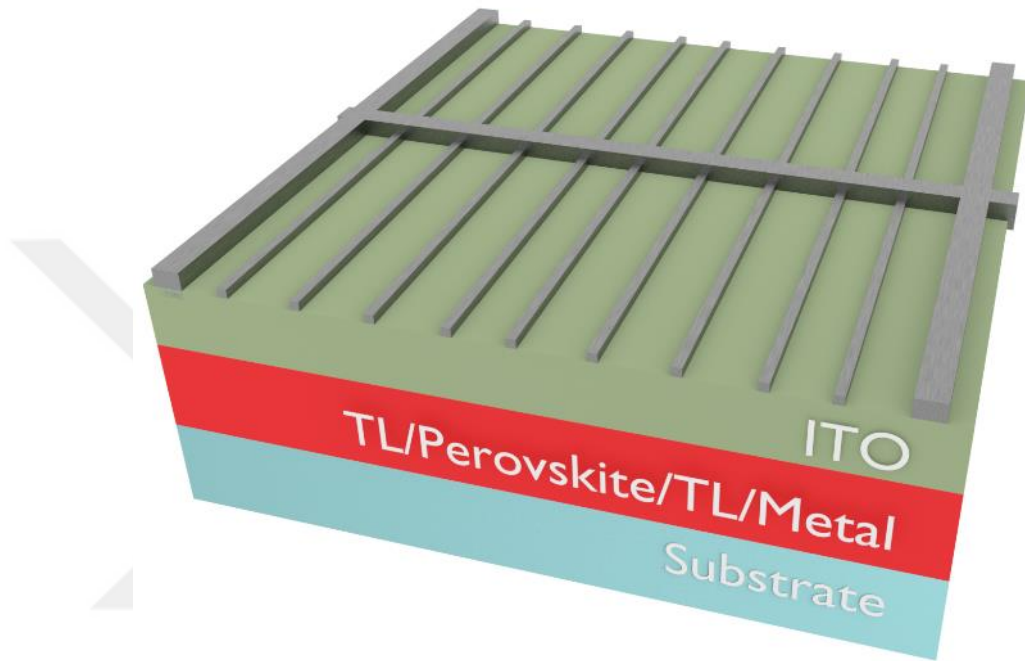
Figure 51 Scheme of the industrial type module design with metal grid network atop the ITO layer.
