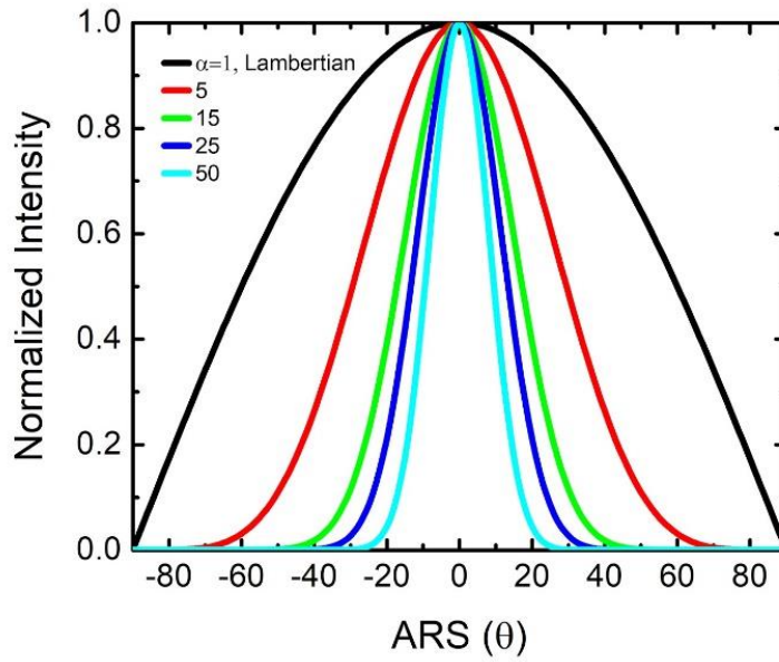
Figure 64 The angle-resolved spectroscopy of the Phong scattering for various Phong exponents.
