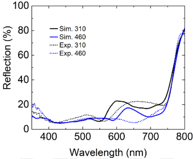
Figure 34 Measured and simulated reflection spectrum for the perovskite solar cells with thicknesses of 310 nm and 460 nm.
