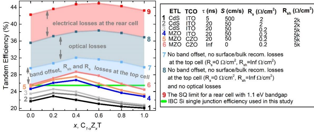
Figure 87 C_{1-x}\text{ZnTe}/\text{IBC Si} tandem efficiency as a function of various x values for different ETL (CdS and MZO) and rear TCO (ITO and CZO) combinations, along with different shunt-series resistances (2000–2 and 5000–0.2 \Omega/\text{cm}^2 ), minority carrier lifetimes (5 and 20 ns), and surface recombination velocities (50 and 500 cm/s): Curves 1–5. Curve 6 is the case for the eliminated bulk and surface recombination at the top cell with MZO ETL and CZO rear TCO for R_s = 0.2 and R_{sh} = 5 \text{ k}\Omega/\text{cm}^2 . The single-junction efficiency of IBC Si cell, 25.2 %, is illustrated as a reference (horizontal green line). The estimated share of efficiency losses with respect to the SQ limit. Curve 7 represents the most ideal electrical case for the top cell with no series/shunt resistance losses and no energy band offset at interfaces, tailored for each absorber composition. Curve 8 represents the ideal electrical case for the top cell and eliminated optical losses, parasitic absorptions, reflection, and transmission for both cells. Curve 9 is the SQ limit for the double-junction tandem solar cell with a rear cell with 1.1 eV bandgap.
