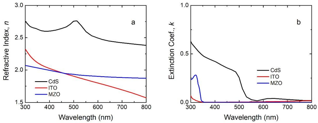
Figure 118 Adopted refractive index (a) and extinction coefficient (b) spectra of CdS, ITO, and MZO used in Chapter 5.
