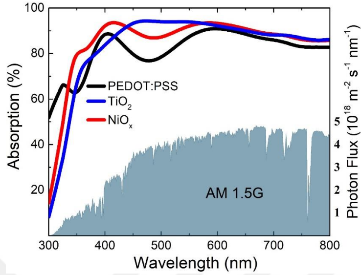
Figure 18 Absorption spectra of semi-infinite perovskite when a 30 nm TL and 210 nm ITO are used (d) together with the AM 1.5G spectrum for the photon flux (green shaded area). The simulated structure (e).
