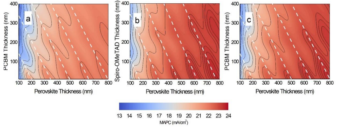
Figure 22 MAPCs varied with perovskite and RTL thicknesses (a, b and c), for PEDOT:PSS, \text{TiO}_2 and \text{NiO}_x FTLs, respectively.
