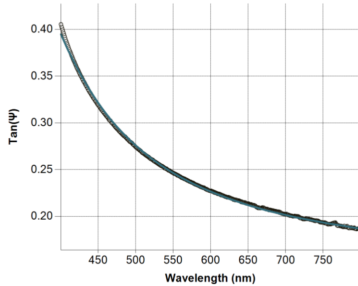
Figure 101 \tan(\psi) spectra of ITO with fitted dispersion law (line) and measurement (dots).
