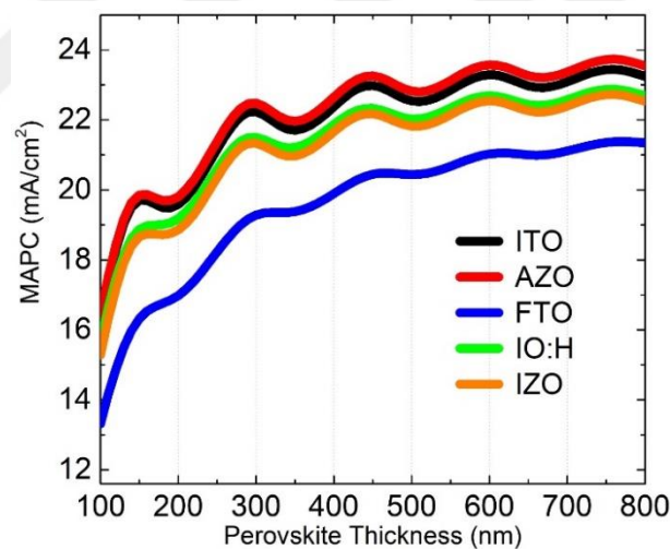
Figure 29 Variation of MAPC with perovskite thickness for different TCO materials with 210 nm thickness. 37,39 \text{NiO}_x and PCBM thicknesses are taken as 30 nm and 50 nm, respectively. The extensive parasitic loss in FTO smooths out MAPC variation with perovskite thickness. 38,40
