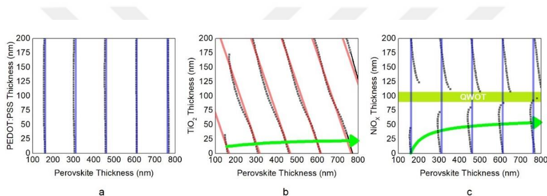
Figure 25 Local maxima regions in MAPC for different interference orders when (a) PEDOT:PSS, (b) \text{TiO}_2 and (c) \text{NiO}_x is used as FTL (black squares). Local maxima regions predicted using Equation 54 and Equation 55 are shown by solid blue and red lines. Green arrows in (b) and (c) indicated the optimum \text{TiO}_2 and \text{NiO}_x thicknesses in terms of ARC efficiency. Green band in (c) indicates \text{NiO}_x thickness range providing QWOT condition hindering occurrence of interference in perovskite solar cell.
