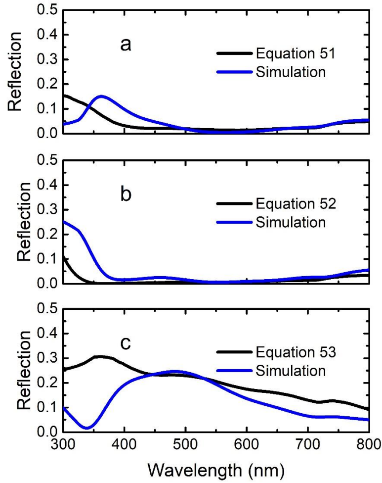
Figure 13 Reflection spectra of glass/ITO/NiO/perovskite stack with QWOT ITO for 15 nm \text{NiO}_x FTL (a), 30 nm \text{TiO}_2 FTL (b) and 80 nm PEDOT:PSS FTL (c) calculated with analytical (black) and simulation (blue).
