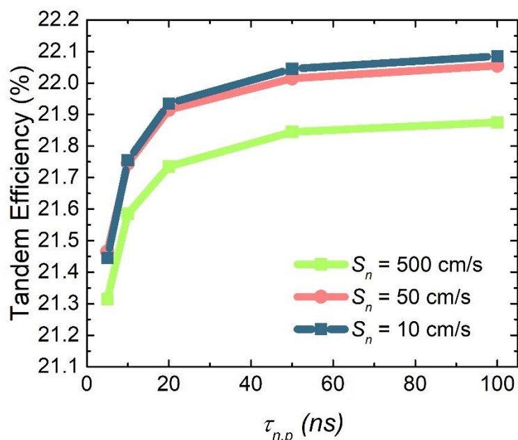
Figure 84 CdTe/IBC Si tandem efficiency as a function of lifetime for three surface recombination velocities (10, 50 and 500 cm/s) for a 3 \mu m CdTe absorber. CdS is used as the ETL.
