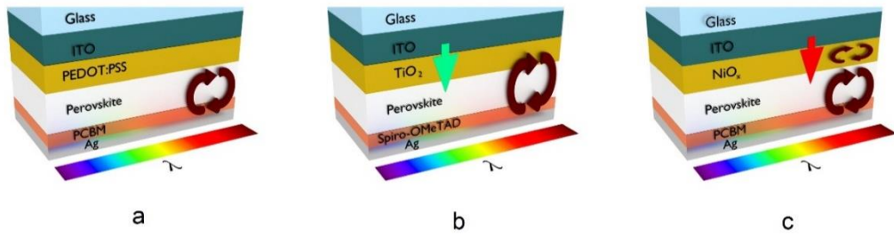
Figure 24 Light trapping (circular arrows) and ARC (vertical arrows) mechanisms in perovskite solar cells are presented for PEDOT:PSS (a), \text{TiO}_2 (b) and \text{NiO}_x FTLs (c).
