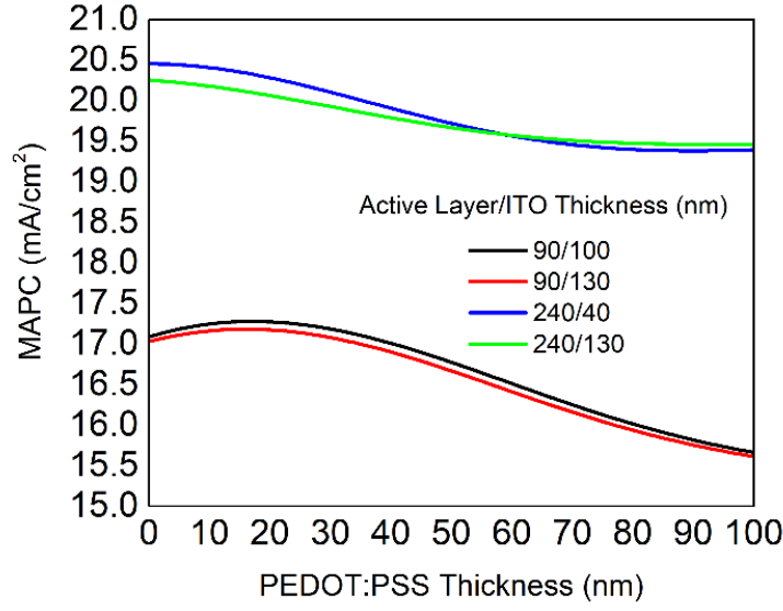
Figure 40 MAPC as a function of PEDOT:PSS thickness for various active layer and ITO combinations
