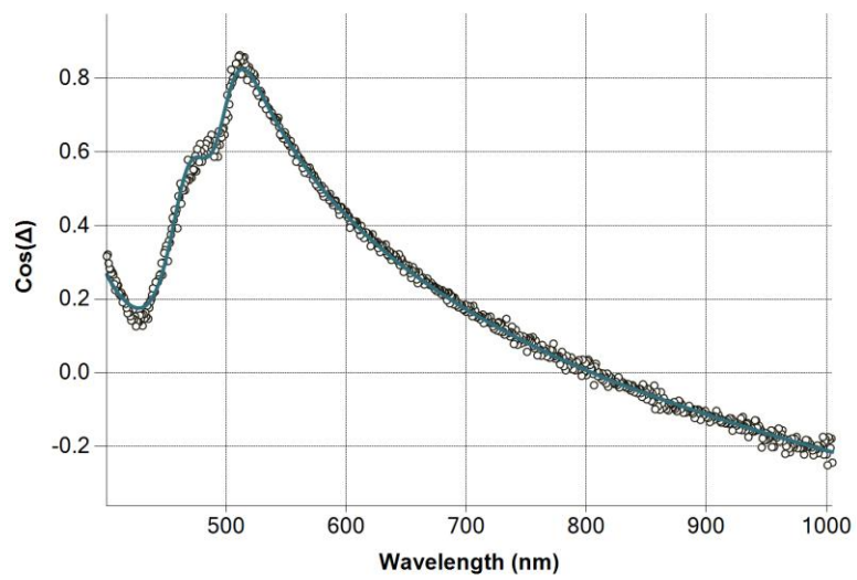
Figure 106 \cos(\Delta) spectra of C_{60} with fitted dispersion law (line) and measurement (dots).
