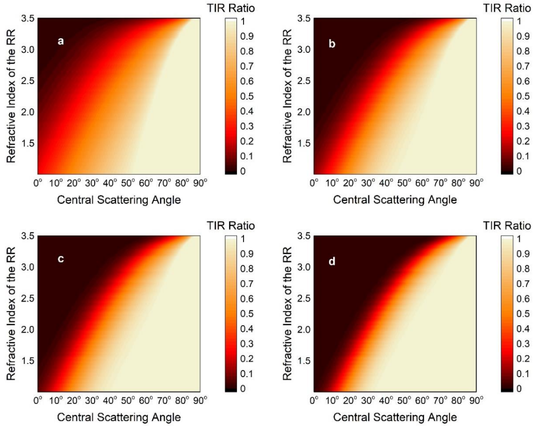
Figure 63 The ratio of the TIR as a function of the refractive index of the RR and the central scattering angle for various Phong exponents, 5 (a), 15 (b), 25 (c), and 50 (d).
