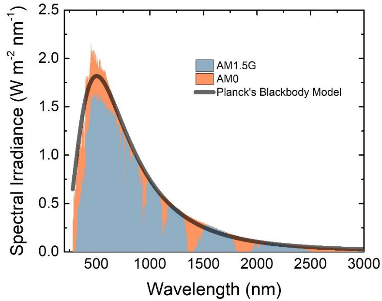
Figure 1 The solar spectral irradiance at the top of the Earth's atmosphere (AM 0) and surface (AM1.5G) along with the Planck's blackbody model at T = 5800 K.
