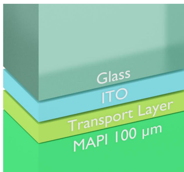
Figure 10 Illustration the structure used to probe anti-reflection of FTL and ITO layers on a very thick perovskite
