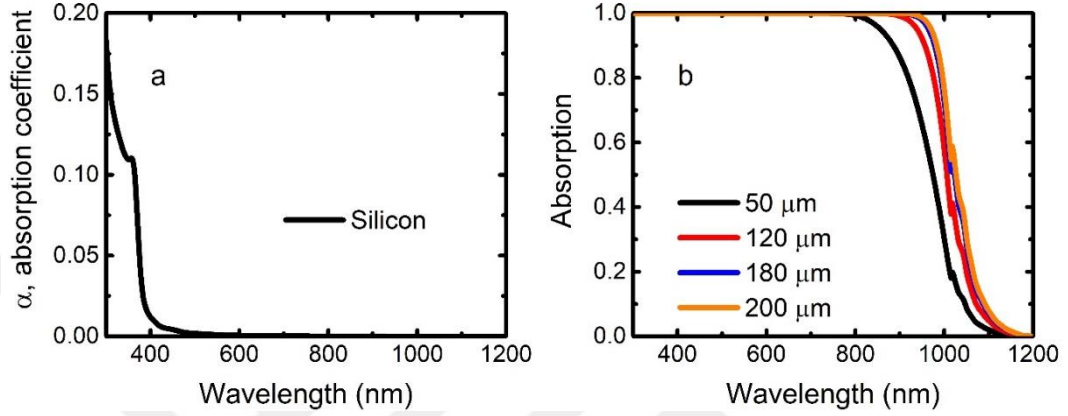
Figure 54 Absorption coefficient of silicon (a). Single-pass absorption spectra of 50, 120, 180, and 200 \mu\text{m} -thick silicon (b).
