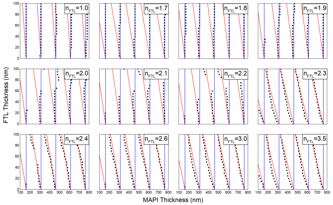
Figure 26 Computed maximal trends in MAPC for various interference orders for hypothetical FTLs with refractive indices between 1.0 and 3.5 and with no extinction coefficient. Maximal trends predicted using Equation 54 and Equation 55 are shown by solid blue and red lines.
