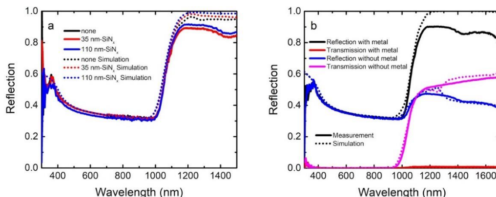
Figure 74 Measured and simulated reflection spectra of the DSP silicon with 35 and 110 nm thick SiN x RR layer, and without an RR layer (a). Measured and simulated reflection and transmission spectra of the DSP silicon with a planarized aerogel RR layer with and without the Ag layer (b).
