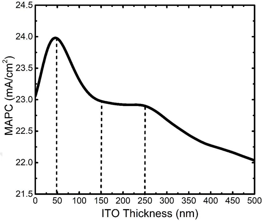
Figure 47 MAPC for various ITO thicknesses. The dashed lines indicated ITO thicknesses of 50, 150, and 250 nm, used in electrical and optical optimizations.
