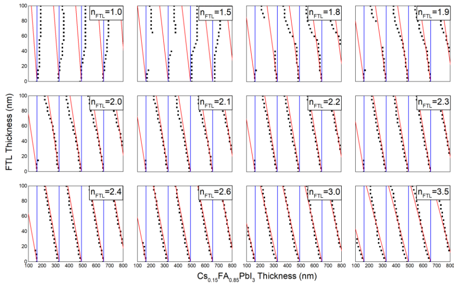
Figure 119 Maximal MAPC trends predicted with Equation 57 are shown as red and blue lines. Simulated maximal trends (black squares) for \text{Cs}_{0.15}\text{FA}_{0.85}\text{PbI}_3 in MAPC for various interference orders for hypothetical FTLs with refractive indices between 1.0 and 3.5 and with no extinction coefficient.
