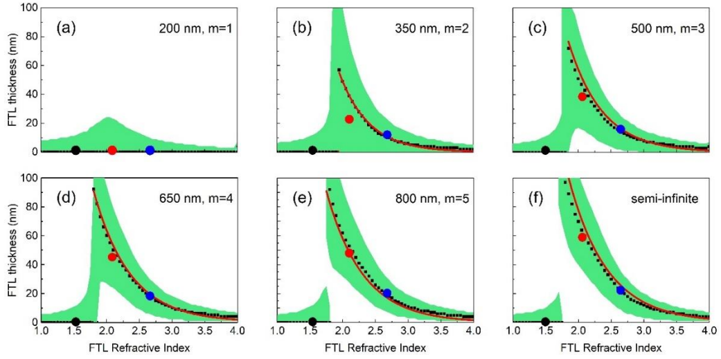
Figure 27 The optimum FTL thickness with respect to FTL refractive index for interference orders of (a) 1, (b) 2, (c) 3, (d) 4, (e) 5 and for semi-infinite perovskite. The RTL thickness is set to zero. Black, red and blue dots indicate the optimum FTL thickness of PEDOT:PSS, \text{NiO}_x and \text{TiO}_2 obtained using their experimental refractive index and extinction coefficients, respectively. The solid red line shows the optimum thickness prediction of Equation 56.
