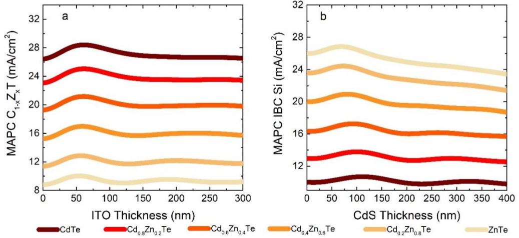
Figure 80 The MAPC of C_{1-x}Z_xT (a) and IBC Si (b) cells for various x values and C_{1-x}Z_xT thickness of 3 \mu\text{m} . In panel (a), the front ITO thickness is varied with no CdS and no rear ITO layers employed, whereas in panel (b), the CdS thickness is varied with 55 nm front ITO and no rear ITO layer employed.
