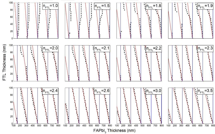
Figure 120 Maximal MAPC trends predicted with Equation 57 are shown as red and blue lines. Simulated maximal trends (black squares) for \text{FAPbI}_3 in MAPC for various interference orders for hypothetical FTLs with refractive indices between 1.0 and 3.5 and with no extinction coefficient.
