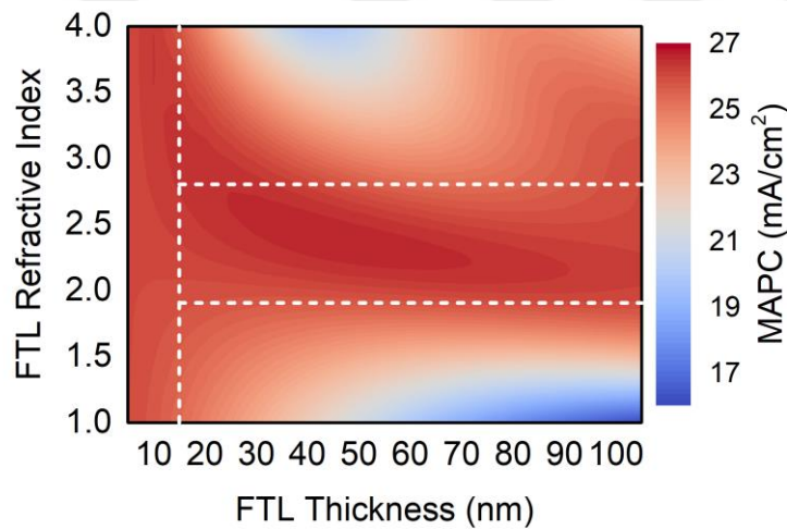
Figure 11 MAPC of semi-infinite perovskite as a function of the thickness and refractive index of a hypothetical FTL upon a 70 nm-thick ITO (a). Dashed lines separate three regions with distinct behaviors.
