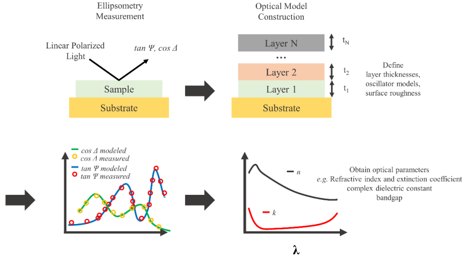
Figure 7 Data acquisition steps for a typical spectroscopic ellipsometry measurement.
