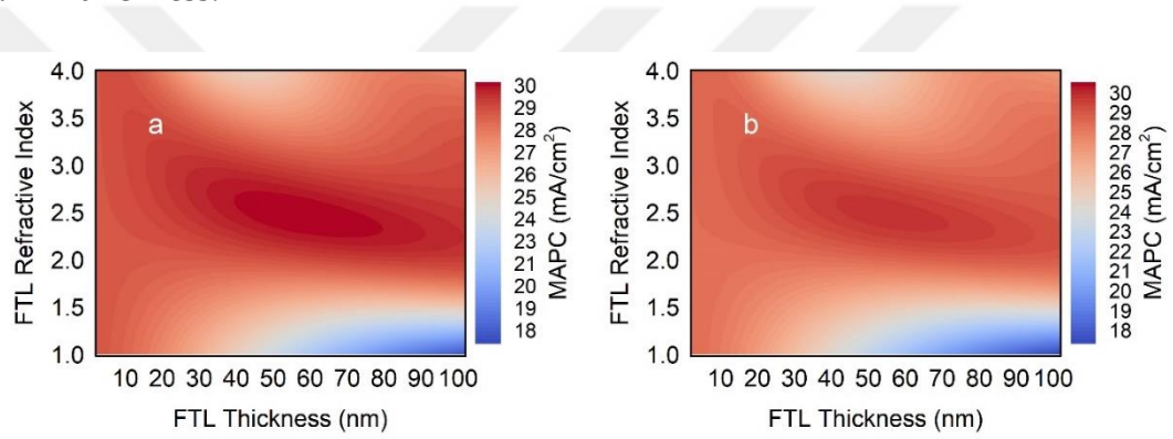
Figure 46 MAPC as a function of refractive index and thickness of FTL for (a) semi-infinite, and (b) 3 \mu\text{m} -thick CdTe layers. ITO is used as 70 nm, 5 nm-thick MoO x is used as RTL and Ag thickness is 150 nm.
