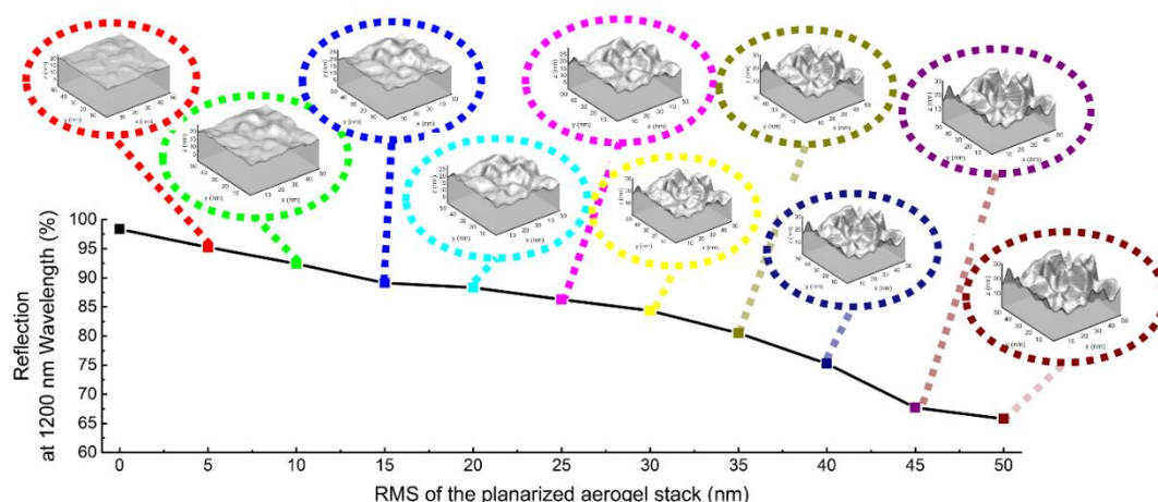
Figure 71 The internal reflection of the planarized aerogel RR layer and the Ag metal for various surface roughness values at the normal incidence at 1200 nm wavelength. Illustration of the metal surface is given as inset.
