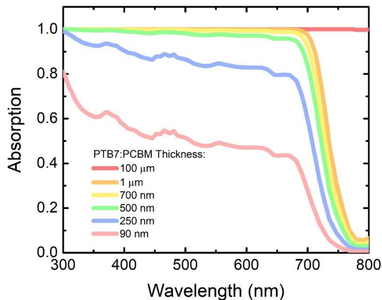
Figure 37 Single-Pass absorption spectra of PTB7:PCBM for various thicknesses.
