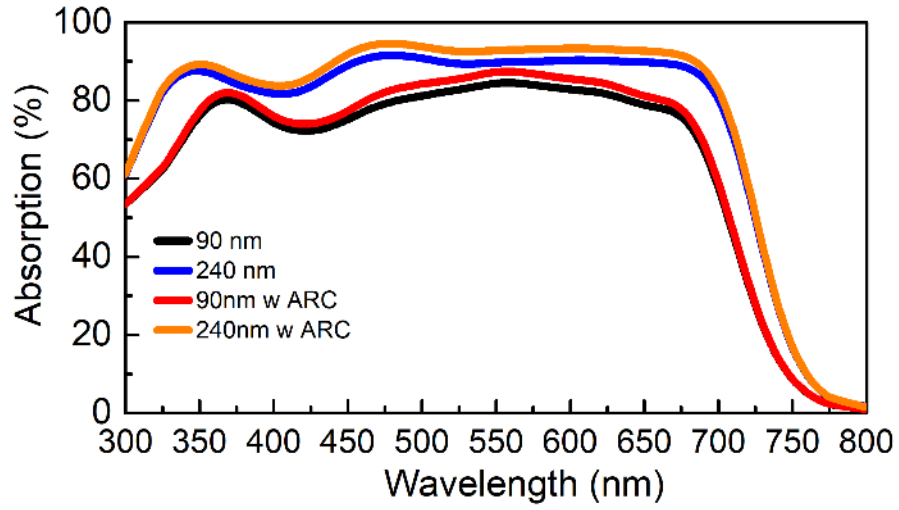
Figure 43 Absorption spectra of optimized structures for active layers 90 and 240 nm with and without the ARC layer. ITO and PEDOT:PSS are used as 130 and 20 nm.
