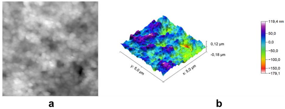
Figure 72 Illustration of AFM surface measurement of the planarized aerogel coated rear interface (a). The height map of the measured surface (b).
