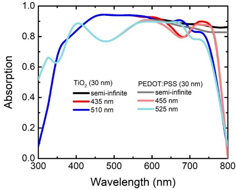
Figure 21 Absorption spectra of perovskite for perovskite thickness leading to local maxima and minima, and for semi-infinite perovskite. The thicknesses of TiO 2 and PEDOT:PSS are 30 nm. The thickness of PCBM is 50 nm in the case of finite perovskite layers.
