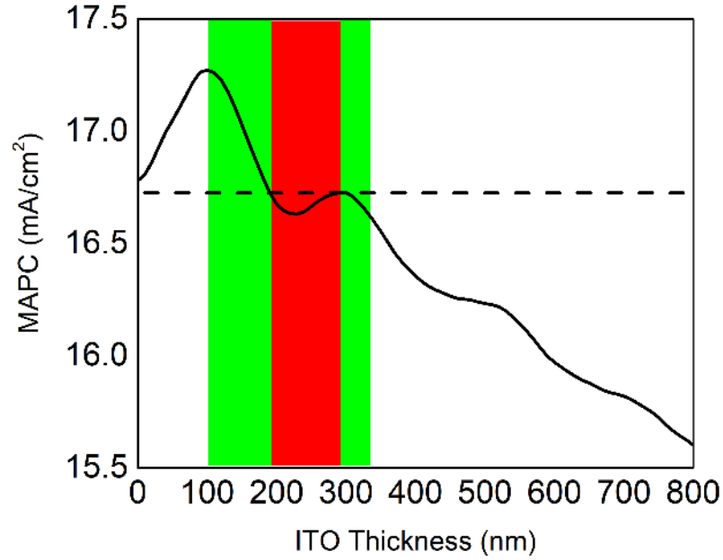
Figure 41 MAPC as a function of ITO thickness for a 90 nm-thick active layer. Recommended (green) and non-recommended regions (red) are highlighted
