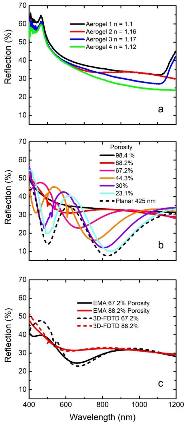
Figure 58 Measured reflection spectra of fabricated aerogel layers on a planar silicon substrate (a). Reflection spectra of aerogel layers for various porosities using 3D optical simulation (b). Comparison of selected porosity fractions using Bruggeman effective medium theory and 3D optical simulations.
