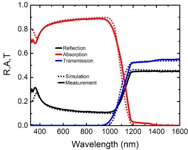
Figure 66 Reflection, absorption and transmission spectra of random DST silicon substrate with simulation (dotted line) and measurement (solid line).
