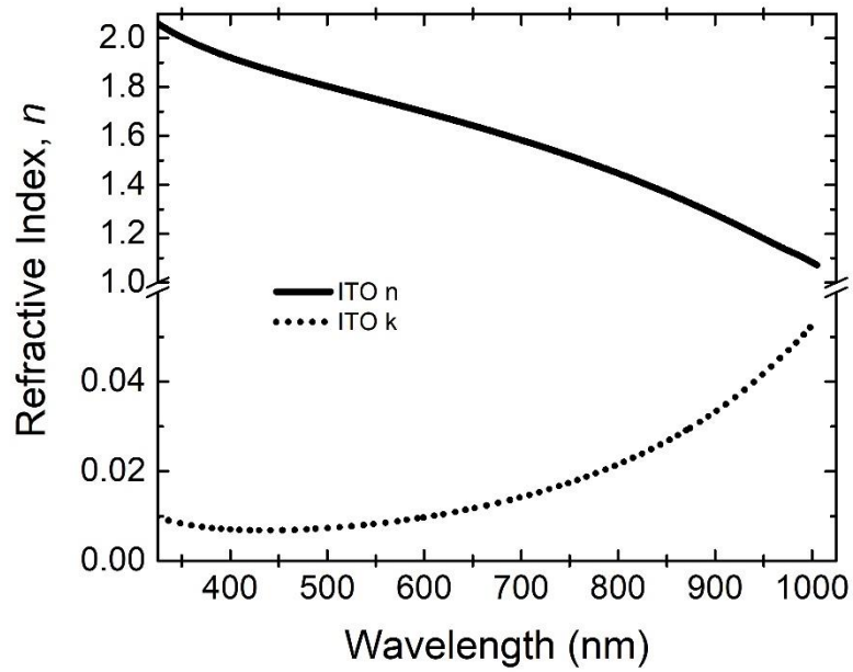
Figure 112 Measured refractive index spectra of ITO.
