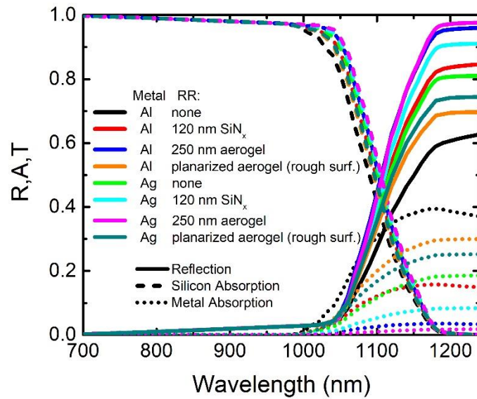
Figure 75 Reflection and absorption spectra of the DST silicon substrate with various RR and metal layer combinations (a).
