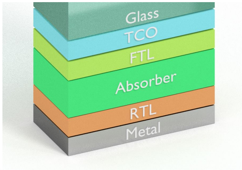
Figure 9 Illustration of the typical thin-film planar solar cell structure investigated in this thesis.
