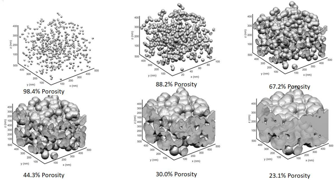
Figure 57 Illustration of aerogel layers with various porosities used in 3D optical computations.
