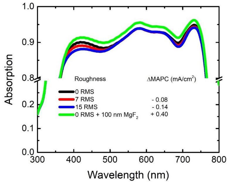
Figure 32 Absorption spectra of a perovskite solar cell with 50 nm \text{NiO}_x , 445 nm Perovskite and 50 nm RTL, and with no roughness (black), 7 nm RMS roughness (red) and 15 nm RMS roughness (blue). Roughness slightly reduces absorption in perovskite primarily in the UV part of the spectrum where scattering is more significant and therefore leads to an optical path length increase and parasitic absorption losses in FTL with relatively large extinction coefficients such as \text{NiO}_x and \text{TiO}_2 . The absorption spectrum of a perovskite solar cells with the same thicknesses of layers having no roughness but a 100 nm-thick \text{MgF}_2 ARC on glass (green line).
