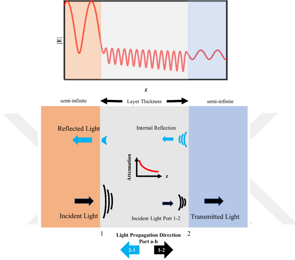
Figure 4 Reflection and transmission of light from a single layer. |E| as a function of depth is presented atop.
