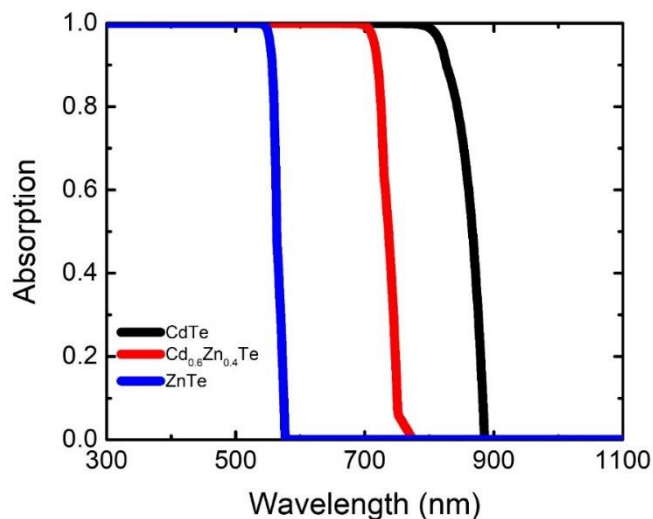
Figure 78 Single-pass absorption spectra for 3 \mu\text{m} thick top cell active absorber (CdTe, \text{Cd}_{0.6}\text{Zn}_{0.4}\text{Te} and ZnTe) obeying the Beer-Lambert Law for the incident light as a function of wavelength are given.
