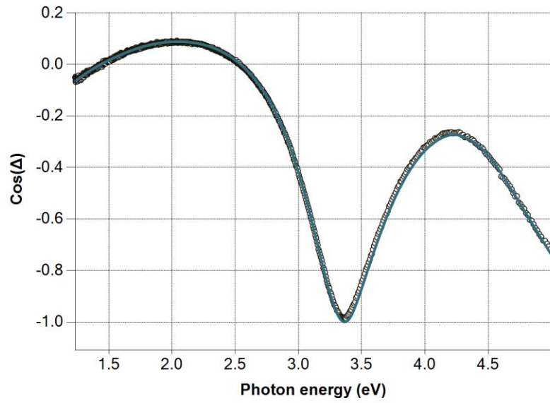
Figure 104 \cos(\Delta) spectra of \text{MgF}_2 with fitted dispersion law (line) and measurement (dots).
