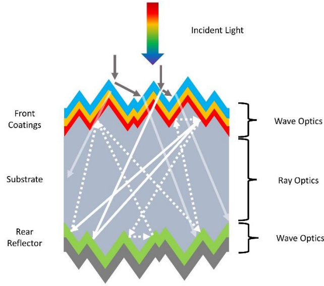
Figure 3 Scheme of the combined ray-wave optics simulation method.
