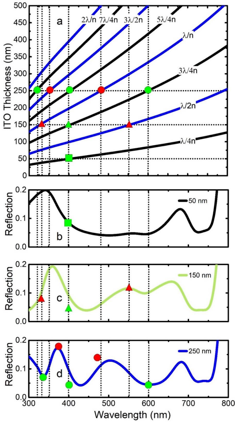
Figure 48 ITO thickness corresponding to QW and HW anti-reflection lines regarding the refractive index spectrum as a function of wavelength (a). Reflection spectra of 50 nm (b), 150 nm (c), and 250 nm thick ITO layer (d). Anti-reflective (green) and reflective (red) trends in line with (a) are presented for 50 nm (square), 150 nm (triangle), and 250 nm (circle).
