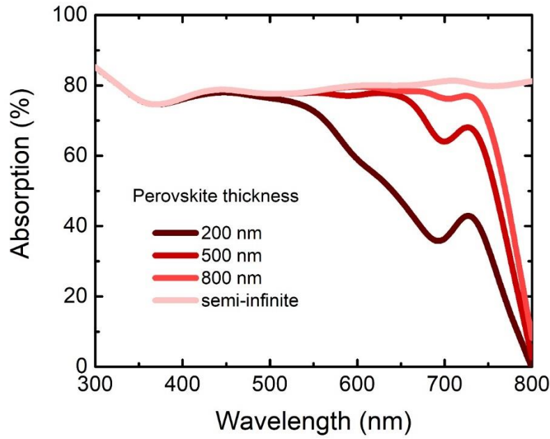
Figure 20 Absorption spectra of 200 nm-, 500 nm- and 800 nm-thick perovskite along with semi-infinite 100\ \mu\text{m} perovskite for a \text{NiO}_x thickness of 30 nm. The thickness of PCBM is 50 nm in the case of finite perovskite layers.
