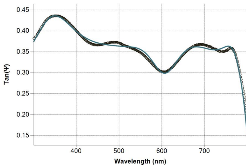
Figure 95 Fitted (line) and measured (dots) \tan(\psi) data of MAPI.
