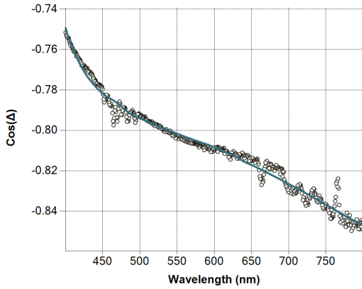
Figure 102 \cos(\Delta) spectra of ITO with fitted dispersion law (line) and measurement (dots).
