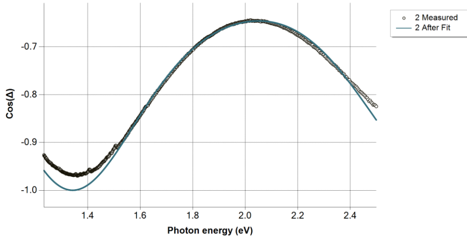
Figure 90 Fitted and measured \cos(\Delta) data of aerogel.
