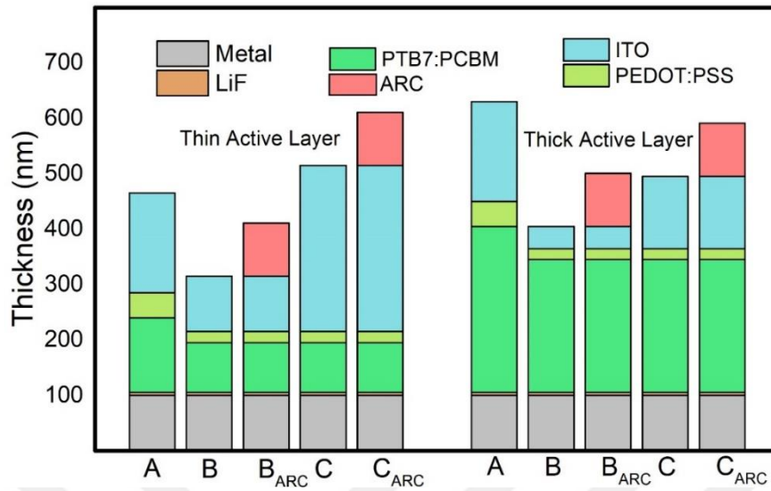
Figure 44 Thickness values of the reference (A), optimized using optically best ITO (B) and optimized using optically favorable ITO with low sheet resistance structures for the thin and thick active layer cases along with ARC coated.
