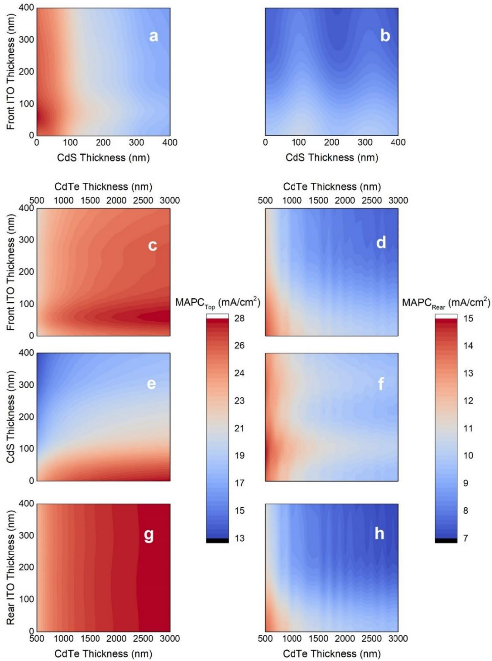
Figure 79 The maximum achievable photocurrent (MAPC) of CdTe and IBC Si cells for various front indium-tin-oxide (ITO) and CdS thicknesses for a constant CdTe thickness of 3000 nm, assuming no rear ITO layer is present (a,b); for various front ITO and CdTe thicknesses, assuming no CdS and rear ITO layers are present (c,d); for various CdS and CdTe thicknesses, assuming a front ITO layer thickness of 55 nm and no rear ITO is present (e,f); and for various rear ITO and CdTe thicknesses, assuming a front ITO layer thickness of 55 nm and no CdS layer is present (g,h), respectively.
