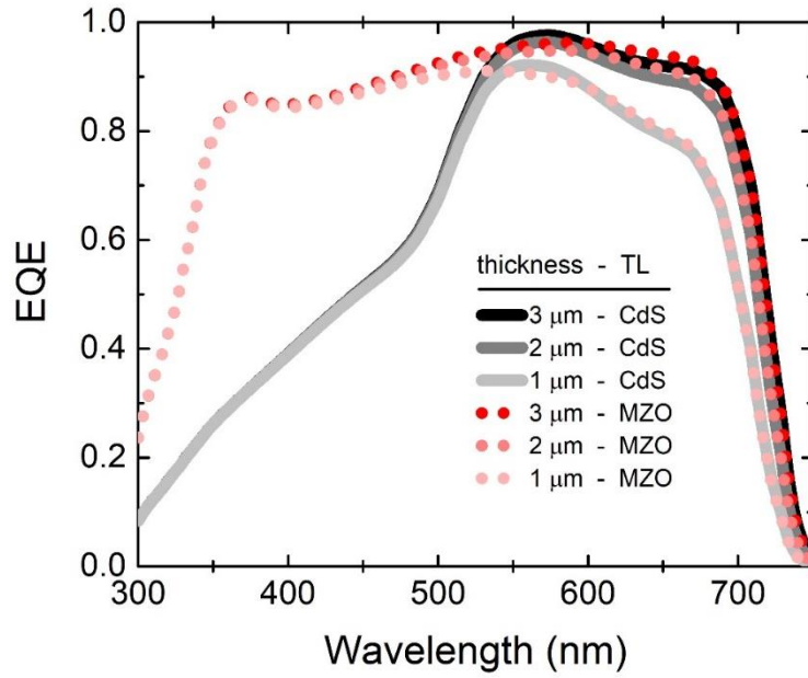
Figure 86 Calculated external quantum efficiency (EQE) spectra for the C_{1-x}Z_xT top cell as a function of the absorber thickness (1, 2, and 3 \mu\text{m} ) at x = 0.6 with 50 nm ETL of CdS and MZO.
