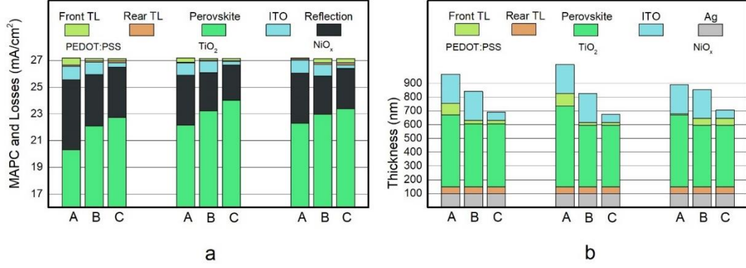
Figure 35 MAPC, and reflection and parasitic absorption losses are given in \text{mA/cm}^2 units for perovskite solar cells utilizing PEDOT:PSS, \text{NiO}_x and \text{TiO}_2 as FTL (a) and corresponding layer thicknesses are given in (b). A denotes the non-optimum perovskite, FTL and ITO thicknesses, B denotes the optimum perovskite and FTL thicknesses but non-optimum ITO thickness and C denotes the optimum perovskite, FTL and ITO thicknesses.
