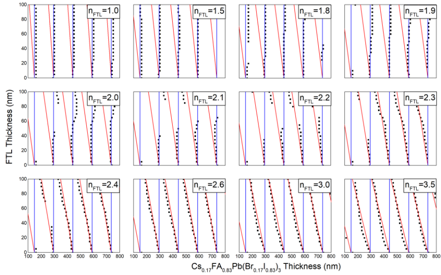
Figure 121 Maximal MAPC trends predicted with Equation 57 are shown as red and blue lines. Simulated maximal trends (black squares) for \text{Cs}_{0.17}\text{FA}_{0.83}\text{Pb}(\text{Br}_{0.17}\text{I}_{0.83})_3 in MAPC for various interference orders for hypothetical FTLs with refractive indices between 1.0 and 3.5 and with no extinction coefficient.
