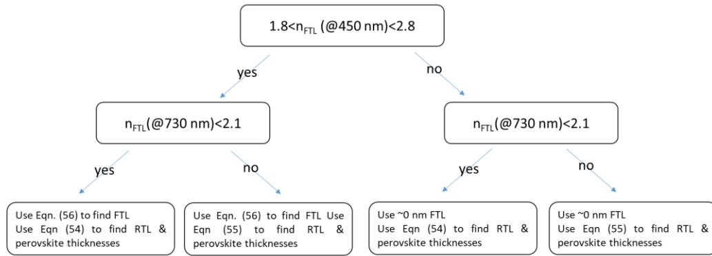
Figure 31 Decision tree for the thickness optimization guideline of FTL, perovskite, and RTL to achieve maximum MAPC.
