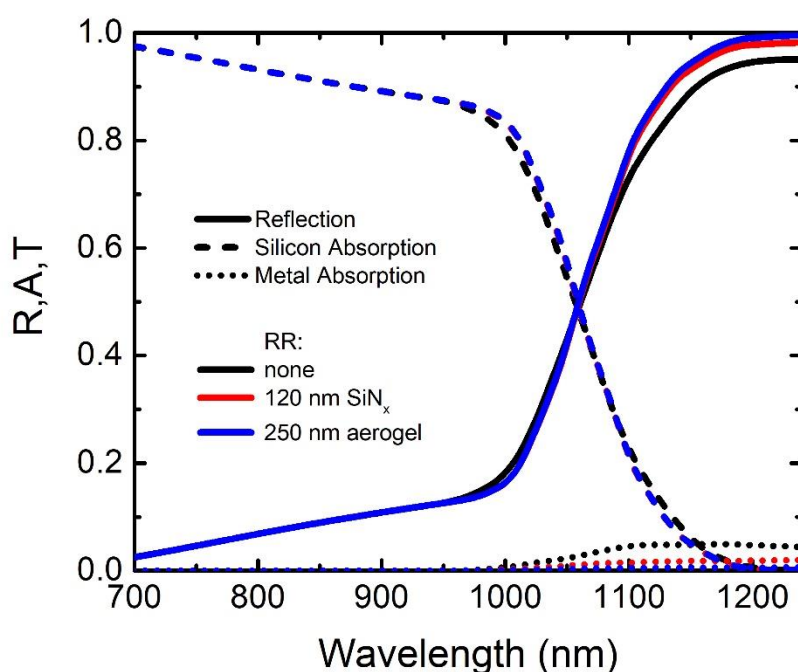
Figure 59 Reflection, and silicon and metal absorption spectra of DSP silicon substrate with various RR combinations (none, 120 nm \text{SiN}_x and 250 nm aerogel). Ag is used as the metal electrode.
