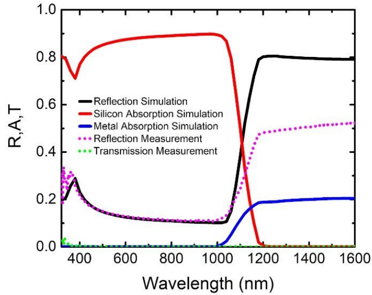
Figure 67 The measured reflection and transmission spectra (dotted line) of random DST silicon substrate with 300 nm-thick Ag metal layer along with simulated reflection, transmission, silicon and metal absorption spectra (solid lines).
