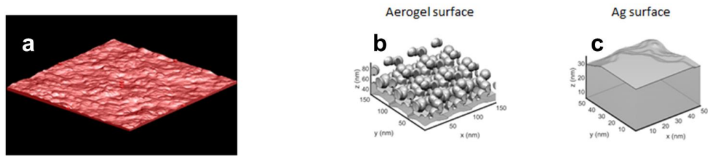
Figure 73 Corresponding simulation model of AFM surface (a) at the rear interface of planarized aerogel RR (b) and conformally coated Ag layer (c).
