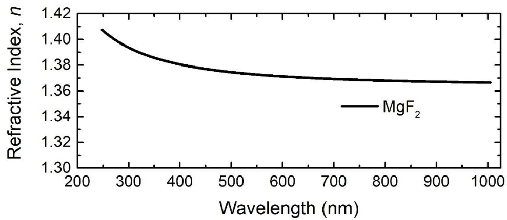
Figure 113 Measured refractive index spectra of \text{MgF}_2 .
