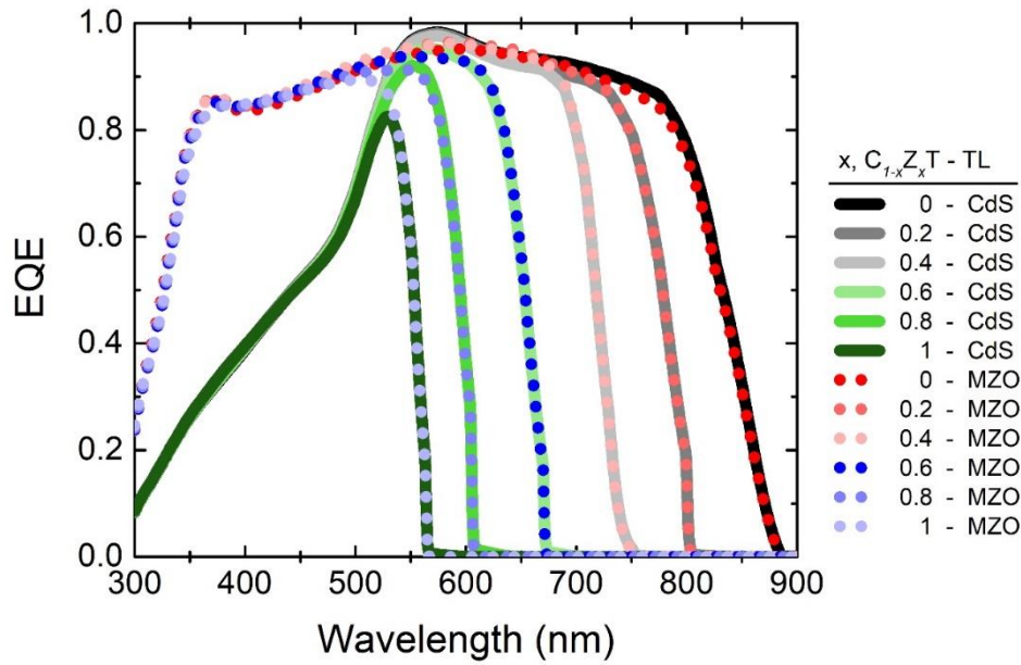
Figure 85 Calculated external quantum efficiency (EQE) spectra for the C_{1-x}Z_xT top cell as a function of the absorber composition ( x = 0, 0.2, 0.4, 0.6, 0.8 , and 1 ) at 3 \mu\text{m} thickness with 50 \text{ nm} ETL of CdS and MZO.
