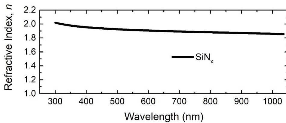
Figure 109 Measured refractive index spectra of \text{SiN}_x .
