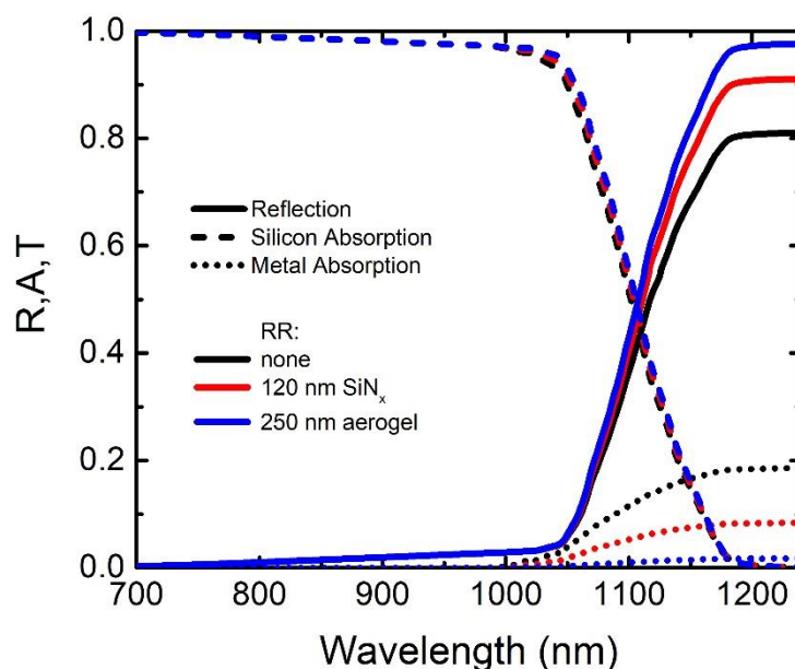
Figure 70 Reflection, and silicon and metal absorption spectra of random DST silicon substrate with various RR combinations (none, 120 nm SiN x and 250 nm aerogel). Ag is used as the metal electrode.
