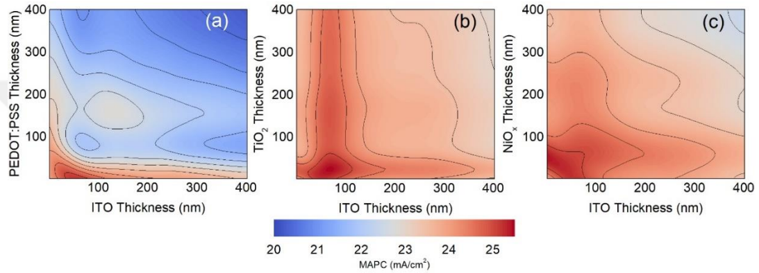
Figure 16 MAPC of semi-infinite perovskite at various thicknesses of ITO and (a) PEDOT:PSS, (b) \text{TiO}_2 , (c) \text{NiO}_x .
