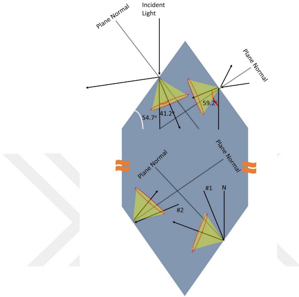
Figure 65 Illustration of the optical paths in the DST silicon substrates at the normal incidence for random distribution of pyramids.
