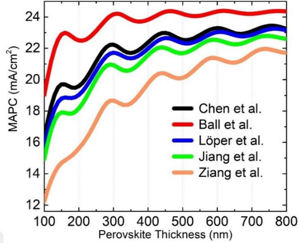
Figure 30 Variation of MAPC with perovskite thickness for various perovskites. 37 \text{NiO}_x and PCBM thicknesses are taken as 30 nm and 50 nm, respectively. The variations in optimum perovskite thicknesses are within a range of 10 nm for various perovskites.
