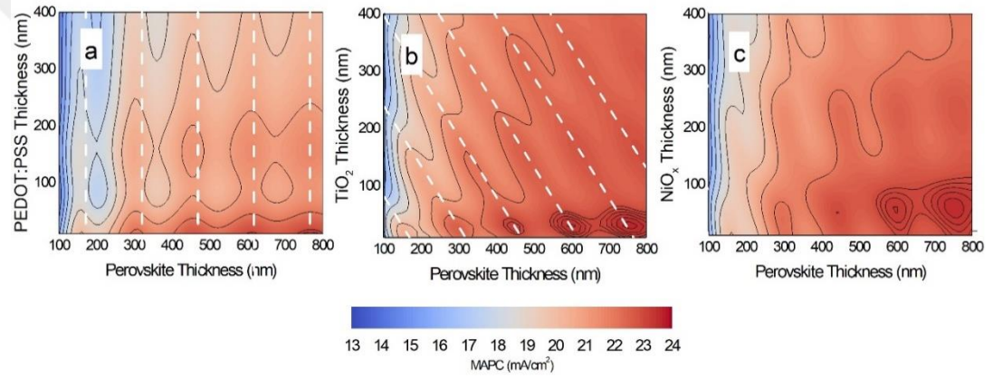
Figure 23 MAPCs varied with perovskite and FTL thicknesses (a, b and c) for PEDOT:PSS, \text{TiO}_2 and \text{NiO}_x FTLs, respectively.
