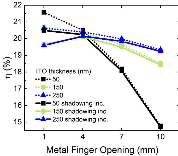
Figure 52 Efficiency of the industry-scale solar cell as a function of the metal finger opening with 50, 150, and 250 nm thick ITO layers. J_0 , n , \rho , R_{sh} are assumed to have values of 2.8 \times 10^{-11} mA/cm 2 , 1.5, 2.025 \times 10^{-4} Ω.cm, and infinity, respectively. Results are presented with (solid) and without (dot) the effect of metal finger shadowing.
