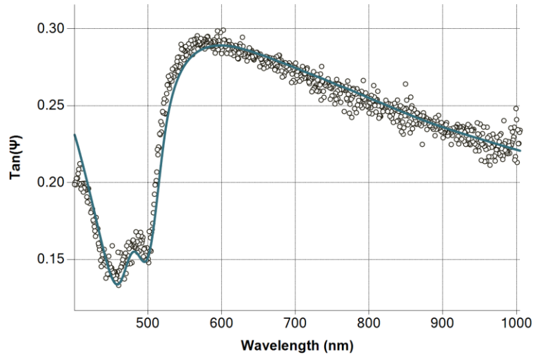
Figure 105 \tan(\psi) spectra of \text{C}_{60} with fitted dispersion law (line) and measurement (dots).
