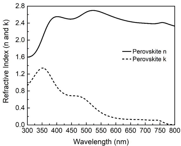
Figure 110 Measured refractive index spectra of MAPI.
