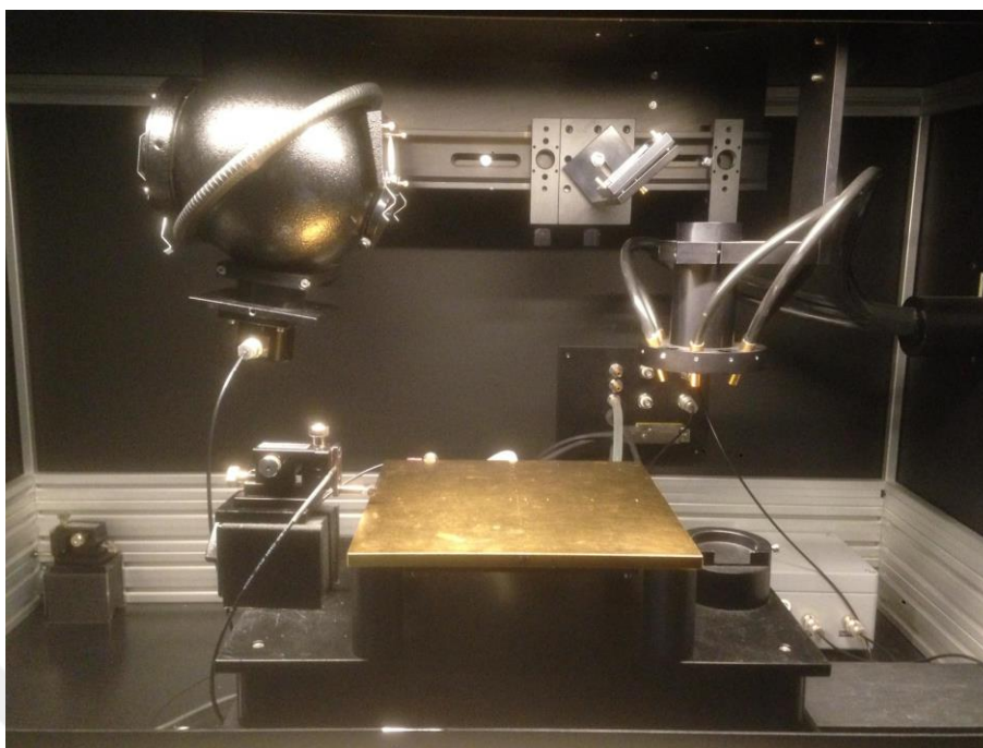
Figure 8 Photograph of the reflection-transmission measurement setup.
