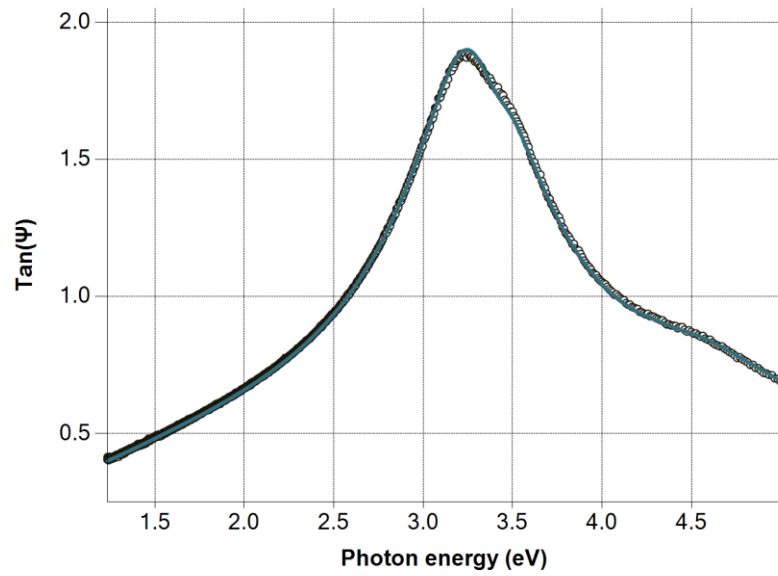
Figure 103 \tan(\psi) spectra of \text{MgF}_2 with fitted dispersion law (line) and measurement (dots).
