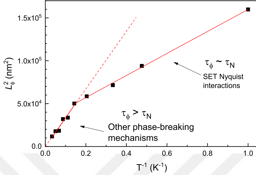
Figure 4.8: L_\phi^2 \propto \tau_\phi shows a linear behavior with inverse temperature ( T^{-1} ) as expected for inelastic phase breaking scatterings induced by e-e interactions. At low temperatures the SET Nyquist scattering is dominated while at higher temperatures the effective dephasing time is larger than the Nyquist time.
