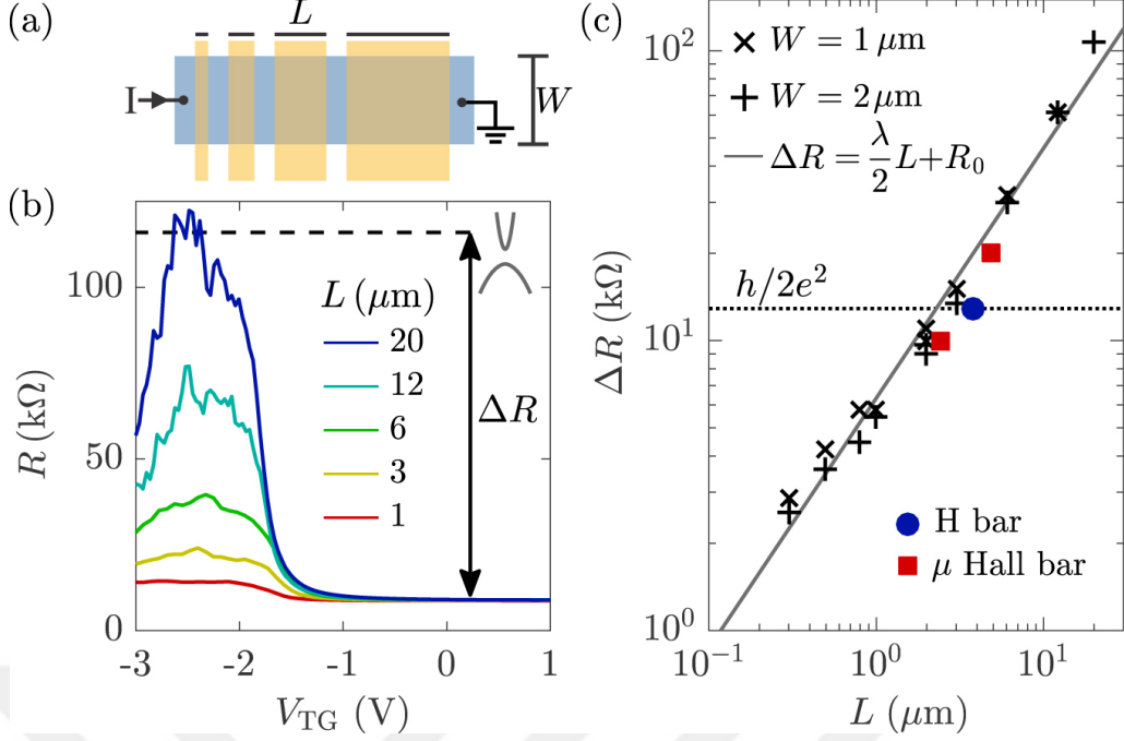
Figure 3.1: The edge resistance of an InAs/GaSb heterostructure in the trivial regime. (a) Schematic representation of finger gate device used to measure the length-dependent resistance of the edge channels. (b) Resistance of a finger gate device with a width of 2\mu\text{m} as a function of top gate voltage for gated regions of different lengths. (c) Resistance change vs gate length shows a linear behavior without saturation at short edge limits. Adapted from Ref. [27].
