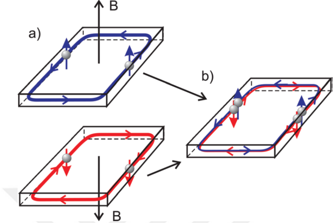
Figure 2.1: A combination of two \nu = 1 integer quantum Hall states with opposite magnetic field directions thus opposite chirality (a) is equivalent to a QSH state with helical edge channels at zero magnetic field (b). Adapted from Ref. [46].
