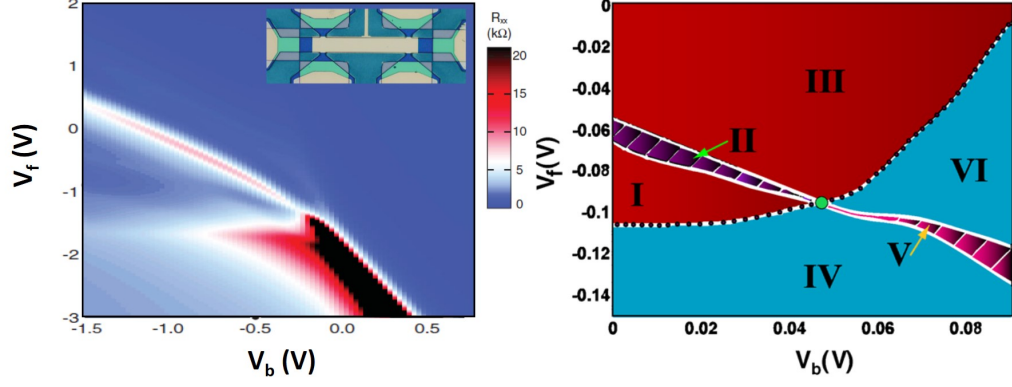
Figure 2.8: Right: The phase diagram as a function of top and bottom gate voltages calculated numerically. Adapted from Ref. [12]. Left: The phase diagram obtained in a transport experiment. Adapted from [23]
