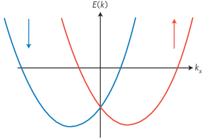
Figure 4.1: Splitting of the spin bands as a consequence of strong spin-orbit interaction.
