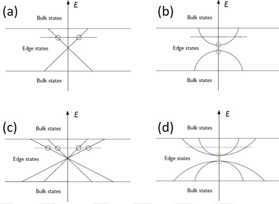
Figure 3.2: Schematic of topological and trivial edge states. (a) A single pair of Kramers pair forms the topological edge states crossing each other at \vec{k} = 0 . (b) Gapped trivial edge states when there is no Kramers pair inside the bulk gap. (c) Gap-less trivial channels as a result of even pair number of Kramers states. (d) Similar to (c) but with a gap in trivial edge states.
