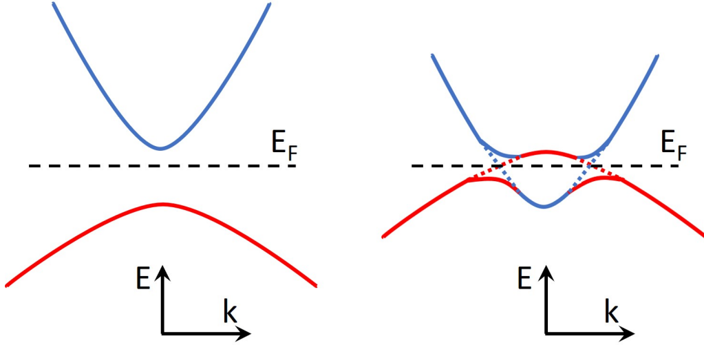
Figure 2.2: Band line-up for trivial (left) and non-trivial (right) insulators with normal and inverted bulk gaps, respectively. Conduction (electron) band is shown in blue and valence (hole) band is depicted in red color.
