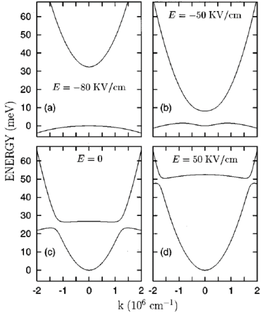
Figure 2.6: Band engineering of InAs/GaSb bilayer QWs using an external electric field. Adapted from Ref. [52].
