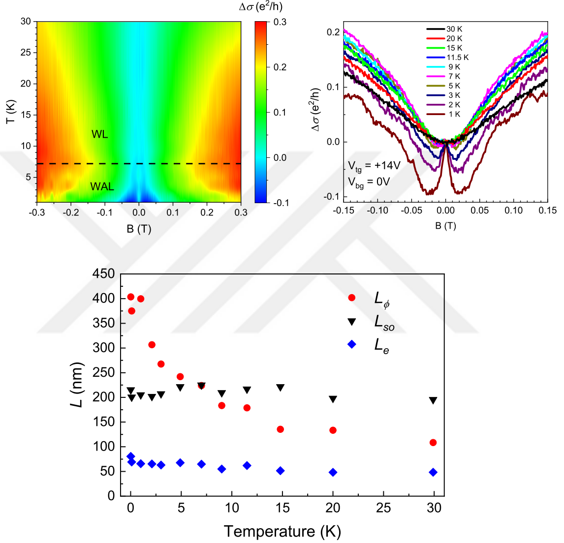
Figure 4.7: Temperature-induced WAL/WL crossover. (a) Magnetoconductance quantum correction measured at different temperatures when V_{bg} = 0 V and V_{tg} = +14 V. (b) The inelastic dephasing length L_\phi , spin relaxation length L_{so} , and elastic mean free path L_e as functions of temperature obtained from theoretical fits to the measurements shown in (a).
