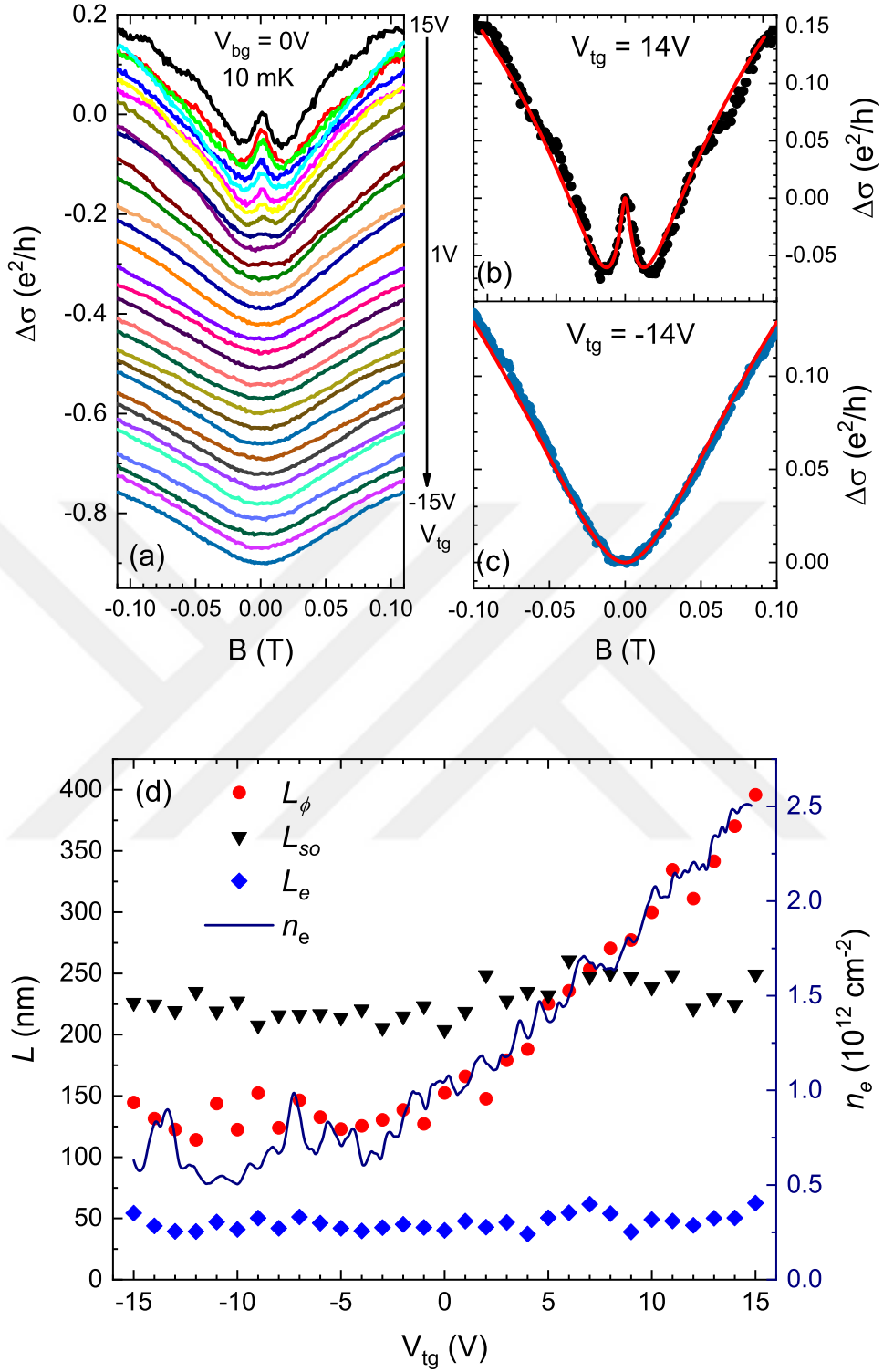
Figure 4.6: Magnetotransport measurements and the characteristic lengths of scatterings. (a) Magnetoconductance correction at different V_{tg} 's where the WAL behavior at V_{tg} = 15 V gradually suppresses at lowered gate voltages and converts to WL at V_{tg} \leq 4 V. (b) and (c) Magnetoconductance correction at V_{tg} = +14 V and V_{tg} = -14 V, respectively, showing WAL and WL features with fit curves (red) to the HLN equation. (d) Corresponding scattering lengths as functions of V_{tg} obtained from the HLN fits to the experimental data. The density modulation with V_{tg} is also shown, which is calculated by Hall resistance measurements at constant magnetic fields.
