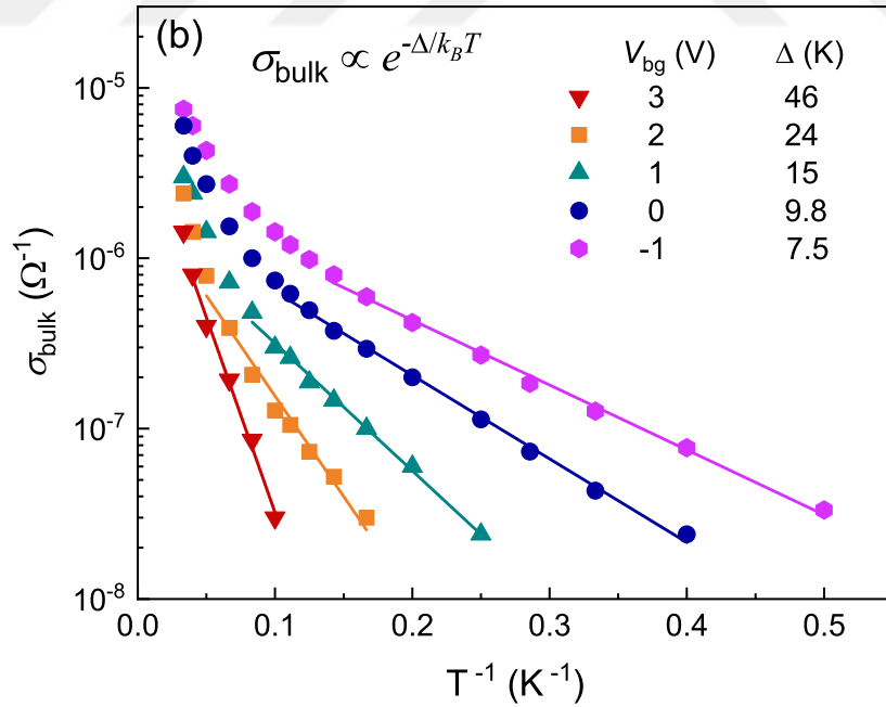
Figure 3.7: (a) The phase diagram of the Corbino disk measured with 100 \mu V AC bias at T = 4 K. (b) Temperature behavior of the minimum bulk conductivity inside the trivial gap for different bottom gate voltages. Solid lines are the fits to the Arrhenius equation giving the corresponding bulk gap for each bottom gate voltage.
