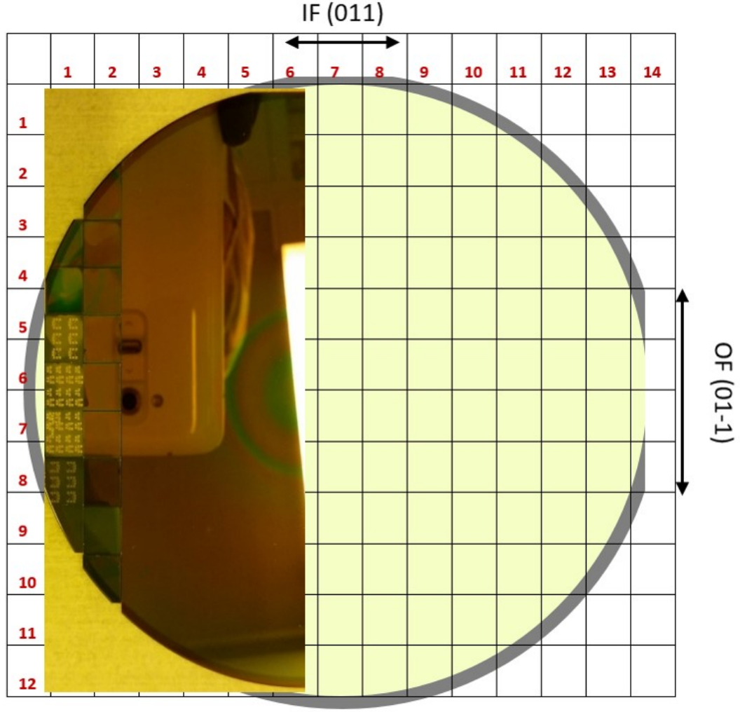
Figure B.1: The dicing map for a 4-inch wafer. Individual pieces are labeled as matrix elements with their corresponding row and column numbers.
