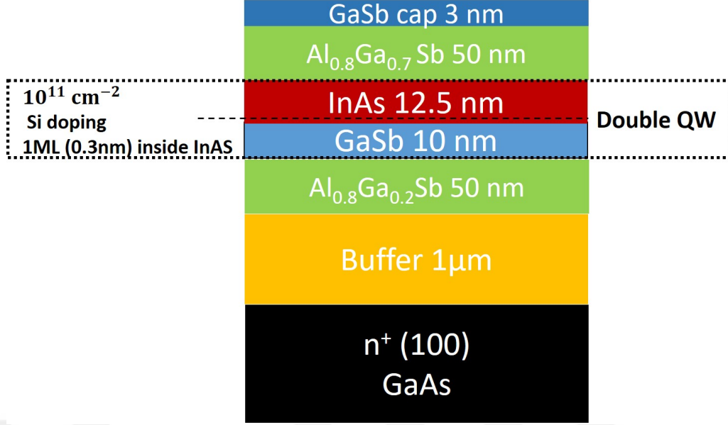
Figure 4.3: Wafer B: Schematic of the heterostructure measured and presented in this chapter with Si delta-dopants inside InAs QW at 1 monolayer distance from the InAs/GaSb interface.
