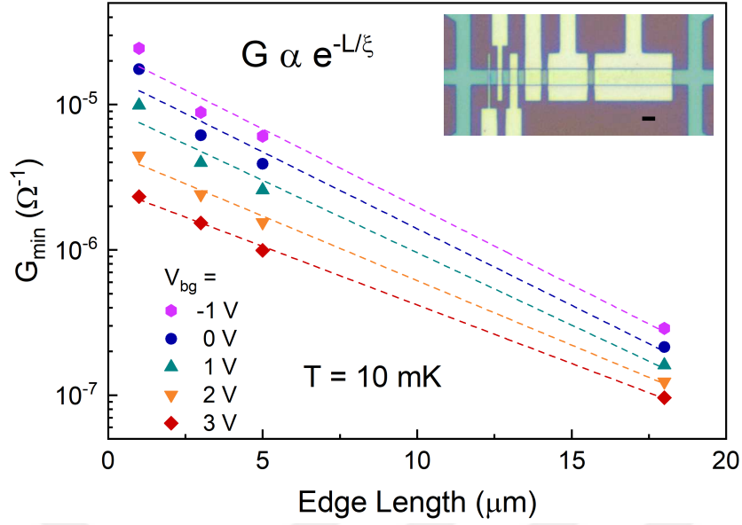
Figure 3.10: The conductance minimum vs edge length measured in the finger gated device. Optical microscope image is shown in the inset, the black scale bar indicates 10 \mu m length.
