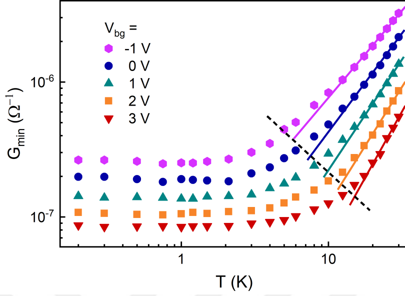
Figure 3.8: Temperature behavior of the Hall bar minimum conductance in top gate sweeps at different bottom gate voltages, characterized by saturation at low temperatures and power law increase at higher temperatures.
