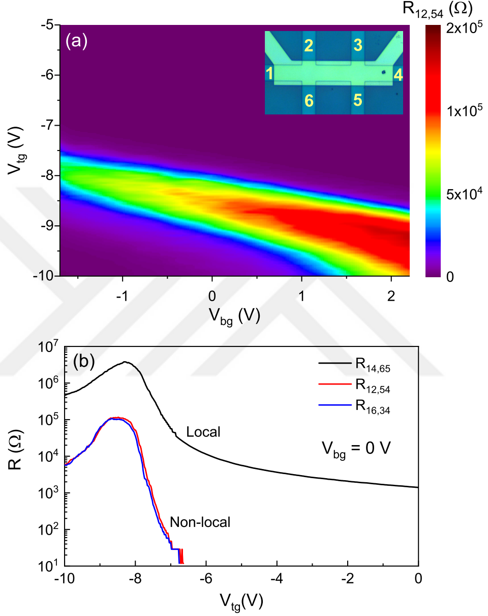
Figure 3.6: (a) Non-local resistance measured in the Hall-bar device as a function of top and bottom gate voltages at 10 mK. Inset shows the optical image of the device with labeled contacts. R_{ij,kl} is the resistance measured between k and l when the current applied between i and j . (b) Comparison of local and two different configuration of non-local resistances as functions of top gate voltage.
