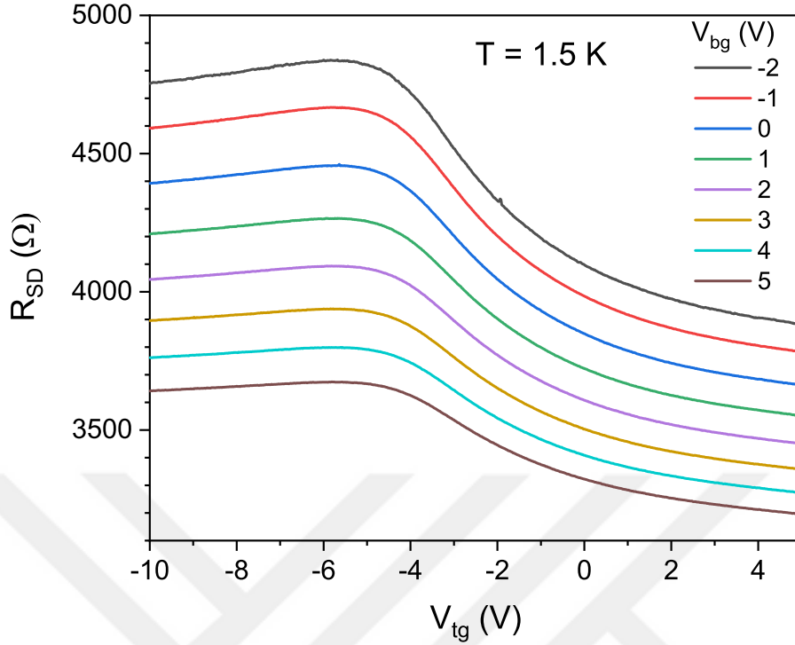
Figure 4.5: Two-terminal resistance of the Corbino device as a function of V_{tg} for different V_{bg} measured with 100 \mu V AC current between source and drain. The sample exhibits semi-metallic behavior with weak modulation of the resistance.
