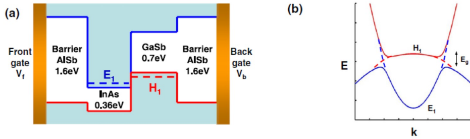
Figure 2.7: (a) A schematic of a dual gate configuration connected to top and bottom AlSb barriers. (b) Band structure diagram in the inverted regime with electron and hole subbands crossing and hybridize at a non-zero momentum. Adapted from Ref. [12].
