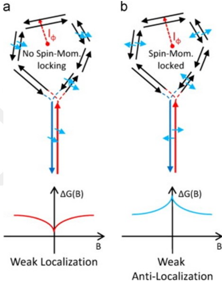
Figure 4.2: Schematic WL and WAL effects. (a) In a spin-degenerate system, the electron waves moving around identical intersecting trajectories interfere constructively thus increase the backscattering probability, i.e. WL phenomenon. (b) The SOC locks the electron spin to its momentum leading to a destructive interference in closed loop time-reversed trajectories. The net difference of the spin rotation between two counter-paths is 2\pi which results in a \pi phase difference between the two wavefunctions that is a destructive superposition (WAL effect). Adapted from [105].
