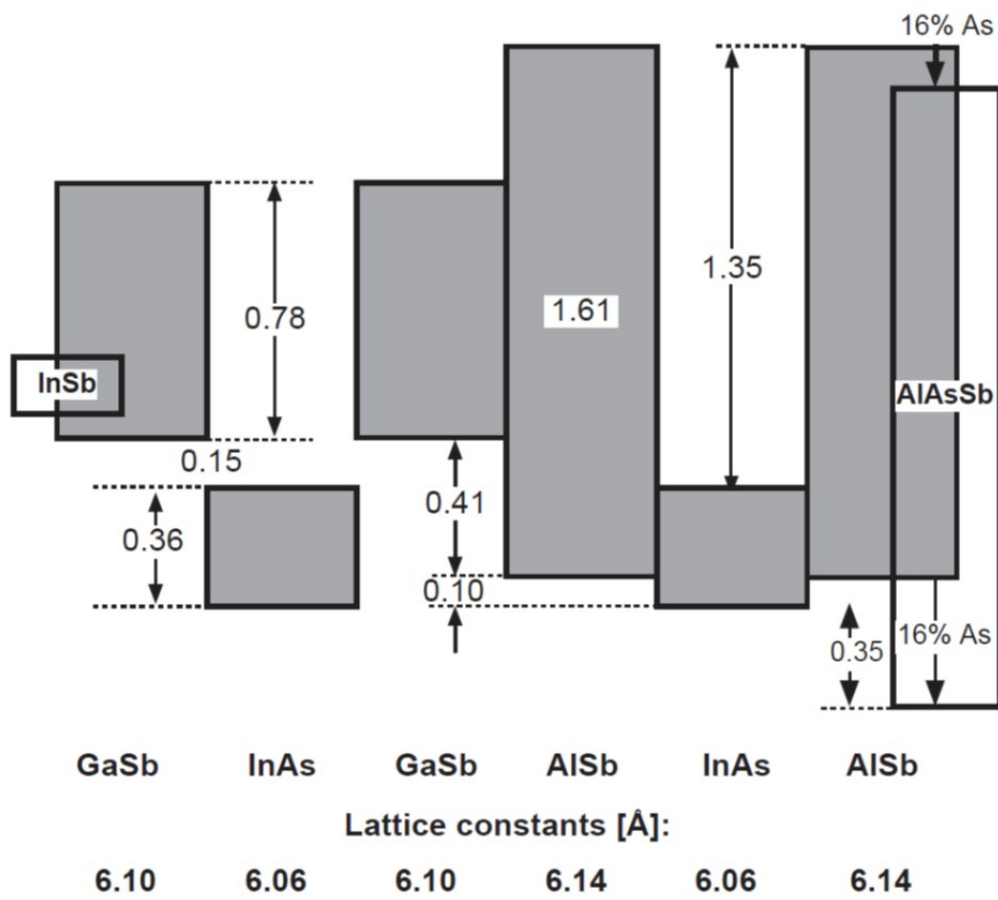
Figure 2.5: Band lineups for 6.1 Å family. The gray areas represent the energy gap and all energies are in eV unit. Adapted from Ref. [51].
