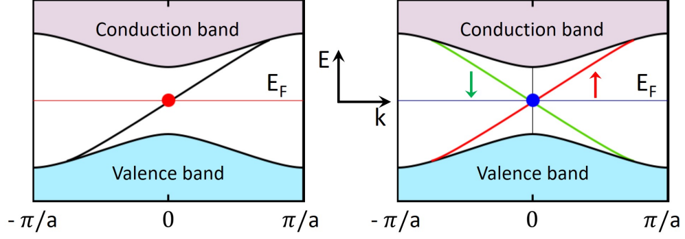
Figure 2.4: QH vs QSH insulators. Left: integer quantum hall is characterized by an insulating bulk with a single right-mover or left-mover edge state depending on the B field direction. Right: A QSHI with a bulk gap and two counterpropagating edge states which has to be spin-polarized due to time-reversal symmetry. Adapted from [1]
