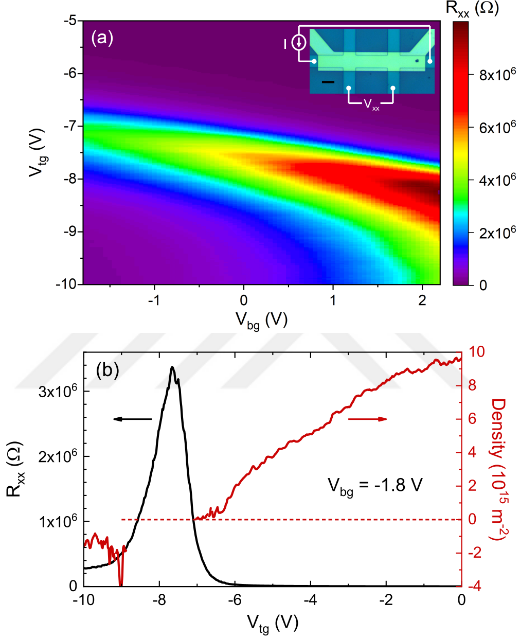
Figure 3.4: (a) Longitudinal resistance of the Hall bar device as a function of V_{tg} and V_{bg} measured at T = 10 \text{ mK} applying 10 \text{ nA} DC current. Inset shows the optical microscope image of the device with a 5\text{-}\mu\text{m} black scale bar. (b) Density modulation via top gate obtained from Hall measurements at 0.5 \text{ T} (red curve). The dashed guideline indicates the zero density. The black curve shows the corresponding longitudinal resistance at B=0 .
