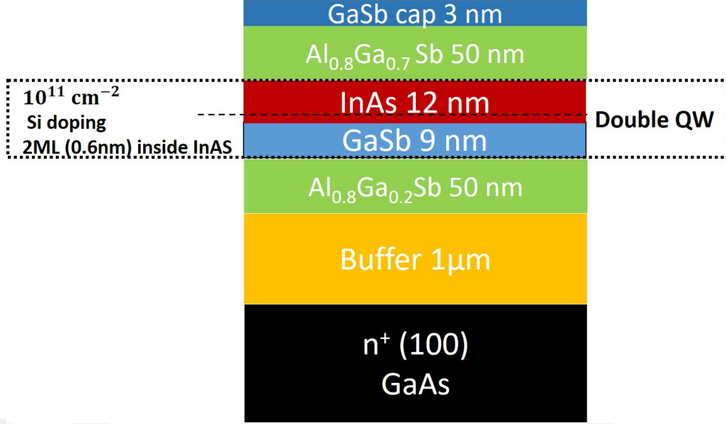
Figure 3.3: Wafer A: Schematic of the heterostructure measured and presented in this chapter with Si delta-dopants inside InAs QW at 2 monolayer distance from the InAs/GaSb interface.
