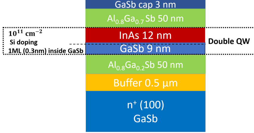
Figure A.2: Wafer C grown on GaSb substrate with a thinner buffer layer since the substrate is better matched with epilayers compared to GaAs substrates used for A and B.
