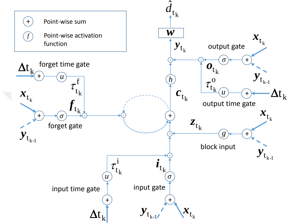
Figure 2.2: Detailed schematic of an LSTM block with additional time gates. Note that x_{t_k} , y_{t_{k-1}} and \Delta t_k are multiplied with their weights, W_{(\cdot)} and R_{(\cdot)} , according to (3.2)-(3.4) and (2.20)-(2.23). Also corresponding biases b_{(\cdot)} is added.
