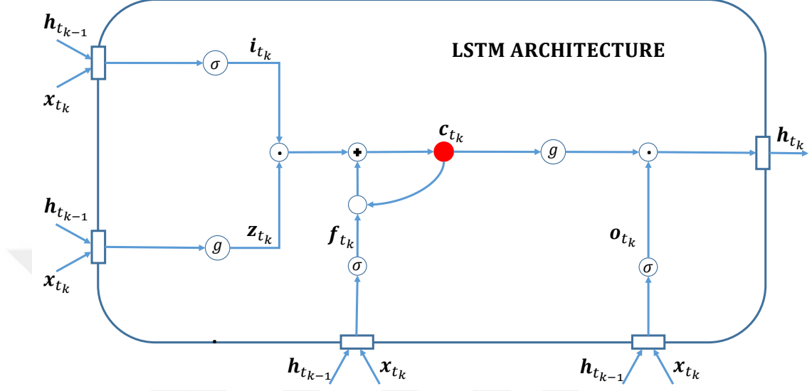
Figure 3.2: Detailed schematic of the LSTM architecture.
