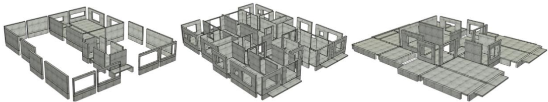
Figure 7.10 3D Locations of Infill Walls on a) 2 nd Floor, b) Normal Floor, c) 8 th Floor Beams
