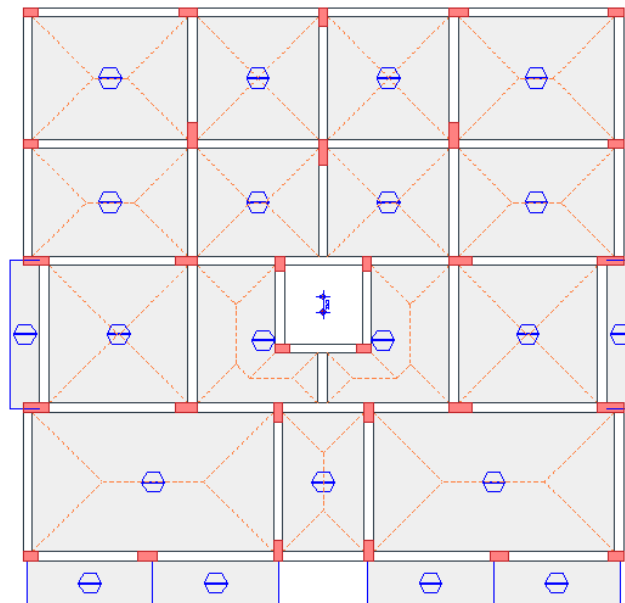
Figure 7.1 Floor Plan of the Building
