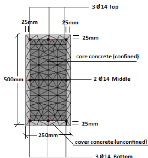
Figure 5.4 Beam Sections
