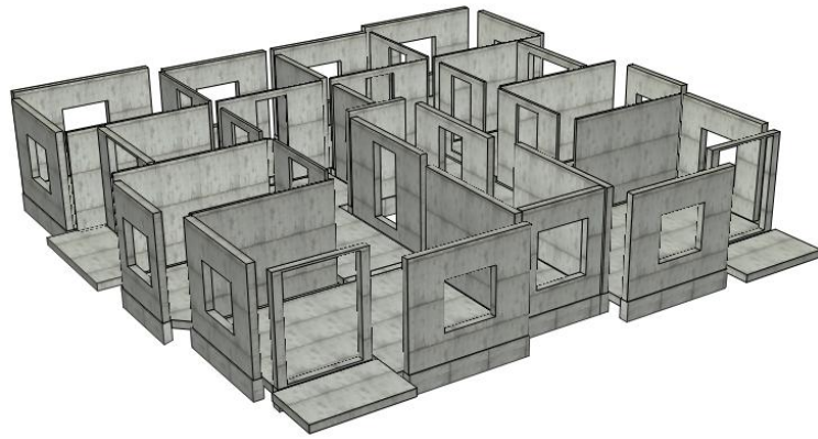
Figure 7.24 3D Locations of Infill Walls on the Beams
