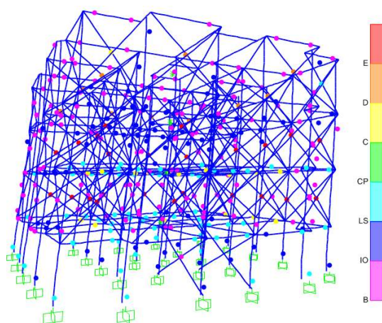
Figure 7.31 Frame with AAC Infill Wall Mechanism at the Collapse Point
