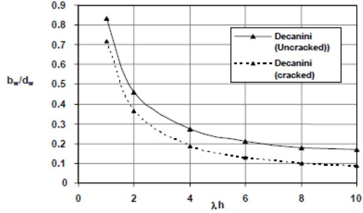
Figure 4.5 Variation of the Ratio b_w/d_w as a Function of the Parameter h \cdot \lambda (Decanini & Fantin, 1986)
