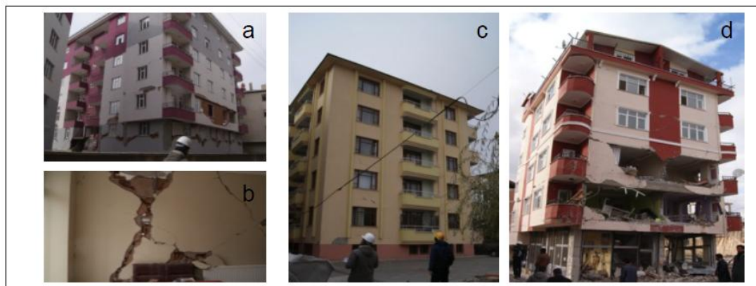
Figure 2.1 Infill Wall Damages Observed After the Earthquake in Van, 2011 a) in Plane Damage, b) Interior Wall Damage, c) Moderate Damage, d) Heavy Damage of the Inner and Outer Plane (Yakut et al., 2013).
