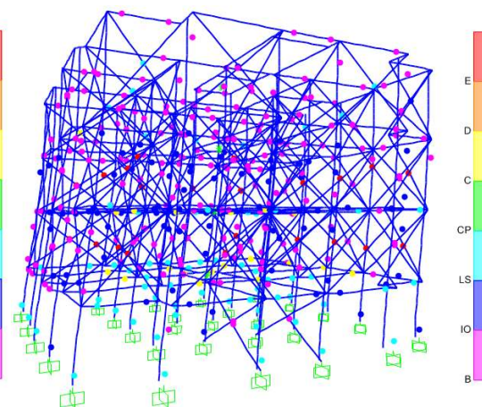
Figure 7.32 Frame with Brick Infill Wall Mechanism at the Collapse Point
