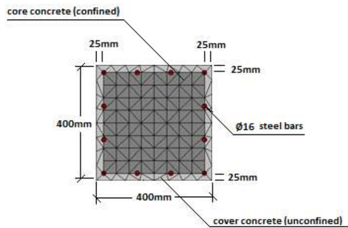
Figure 5.3 Column Sections
