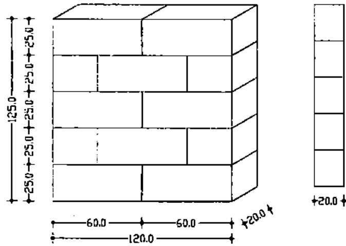
Figure 3.3 Wall Experiment Elements (Alakoç et al., 1999)
