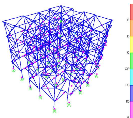
Figure 7.30 Frame with Brick Infill Wall Mechanism at the Performance Point
