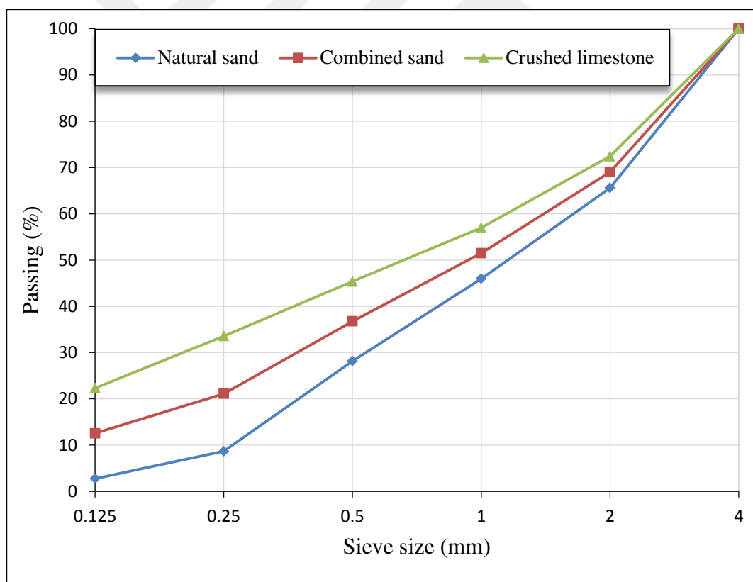
Figure 3.2 Grading curves for aggregates
