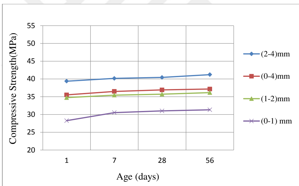
Figure 4.6 Effect of age on compressive strength of GPM with natural sand
