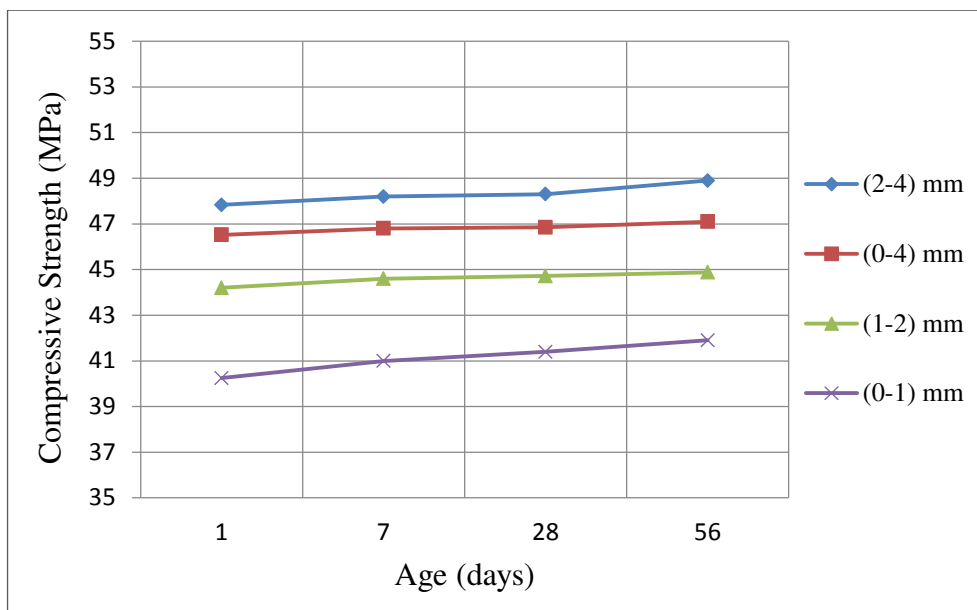
Figure 4.5 Effect of age on compressive strength of GPM with crushed limestone
