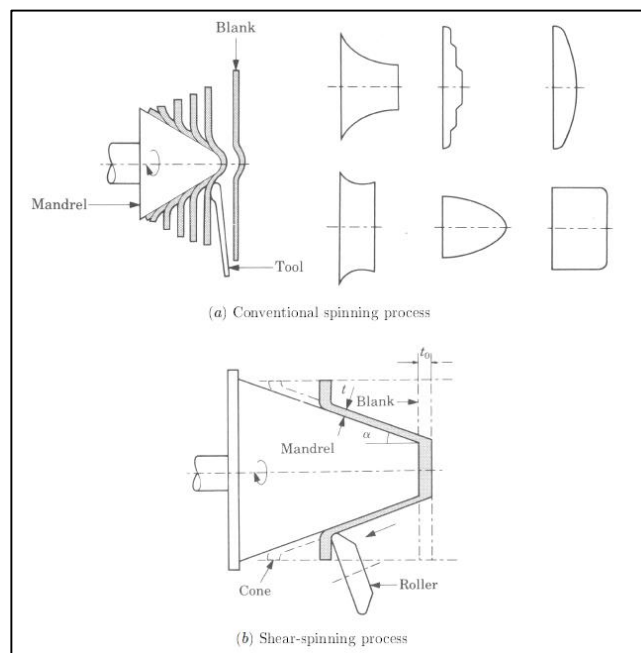
Figure 1.2: Schematics of conventional spinning and sheer spinning [2].
