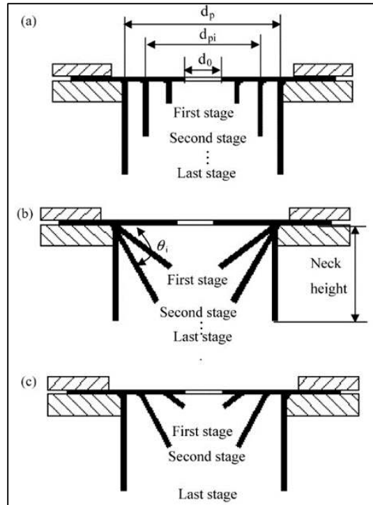
Figure 2.12: Different strategies for multistage incremental forming [28].
