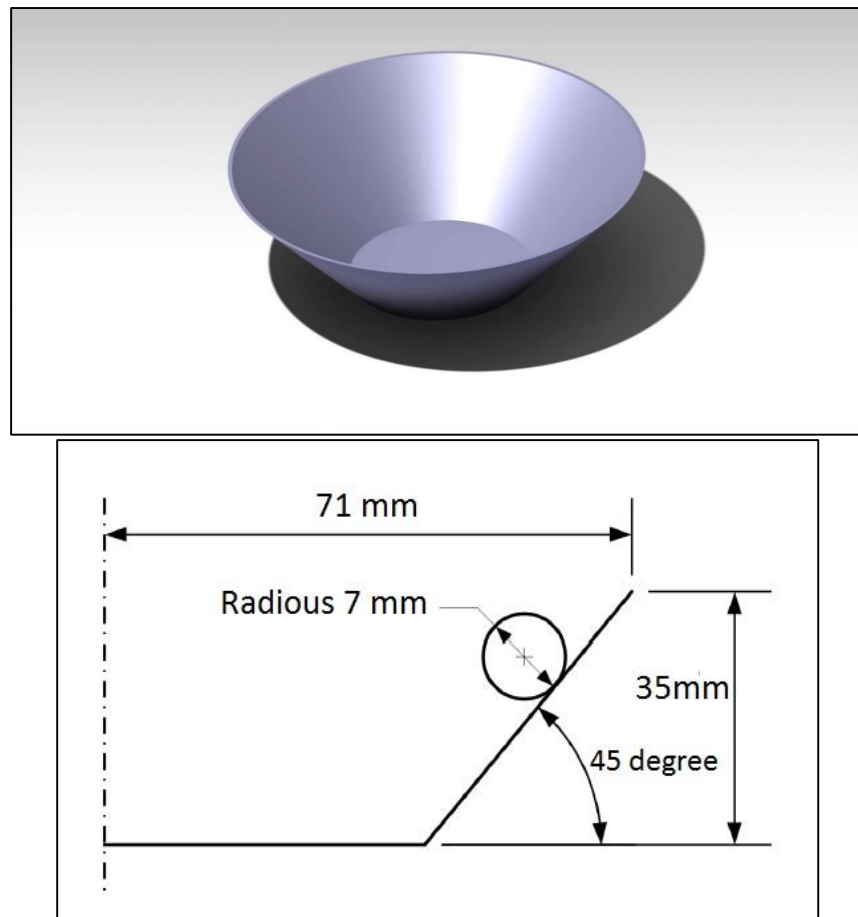
Figure 4.16: 3D view and dimensions of the test for 45^\circ cone. Illustrated using SIEMENS NX.
