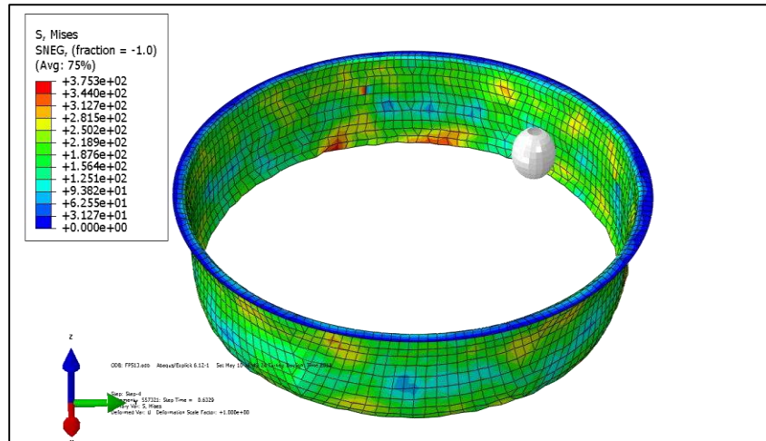
Figure 5.9: 90 mm holed part – Misses stress distribution (MPa).
