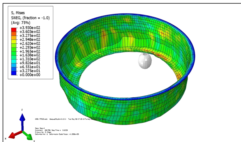
Figure 5.8: 80 mm holed part – Misses stress distribution (MPa).
