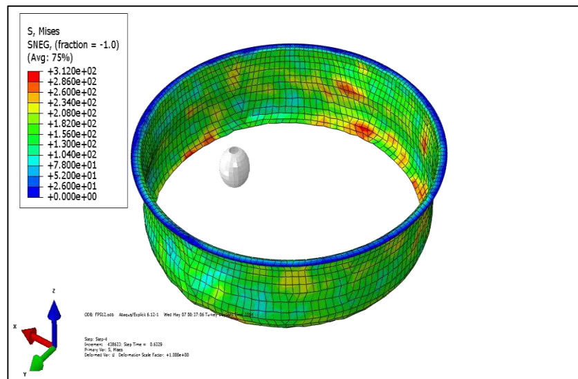
Figure 5.7: 85 mm holed part – Misses stress distribution (MPa).
