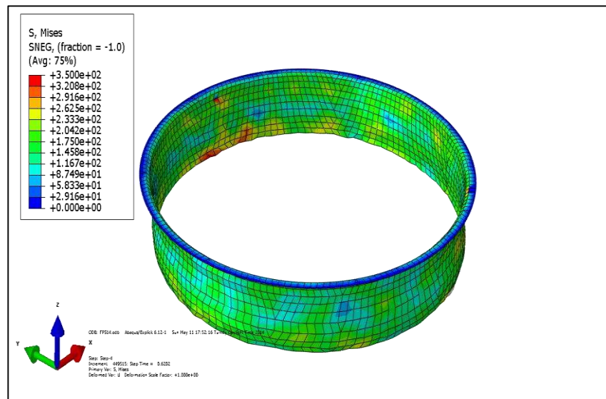
Figure 5.10: 95 mm holed part – Misses stress distribution (MPa).
