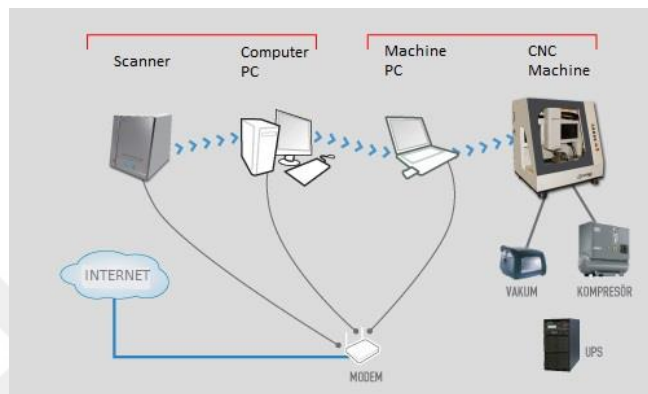
Figure 2.4 CAD-CAM algorithms
