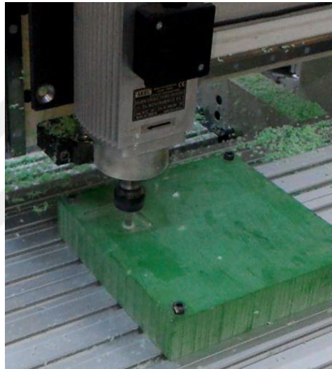
Figure 5.10 Sikablock milling process (Personal archive, 2017)
