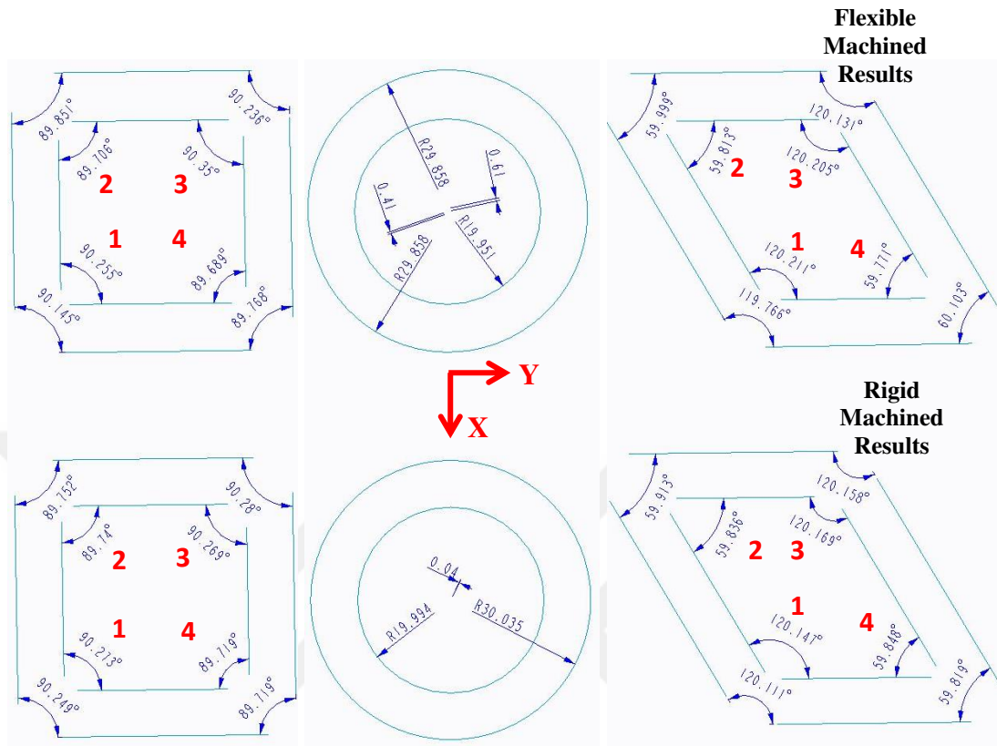
Figure 5.16 Angular measurement results
