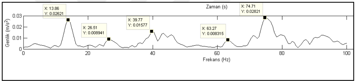
Figure 4.20 Frequency spectrum of the vibration signal generated in the Y direction with respect to the local axis-set of the applied in the Y direction
