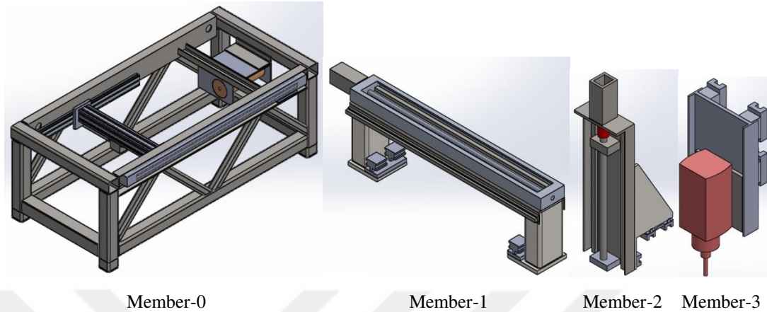
Figure 4.2 Undetailed CAD models of members
