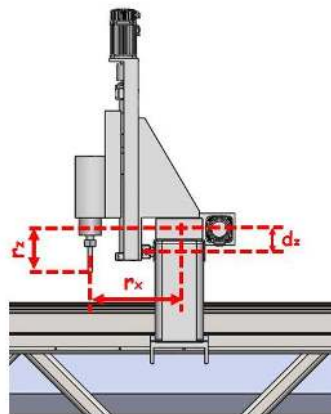
Figure 3.24 Force and moment calculation distances for Y-Axis
