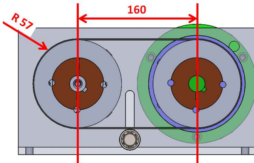
Figure 3.29 A-Axis dimensions
