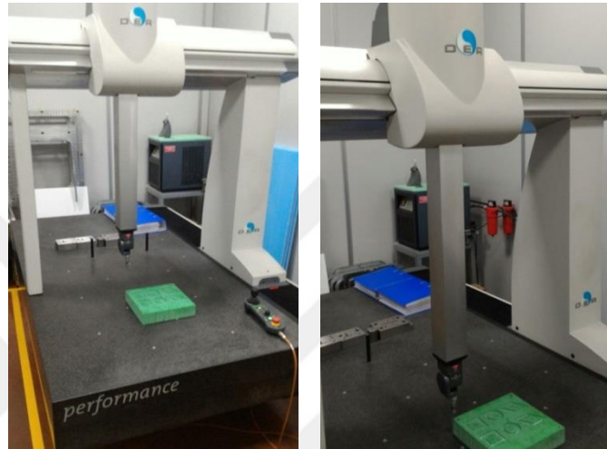
Figure 5.14 CMM measuring process (Personal archive, 2017)
