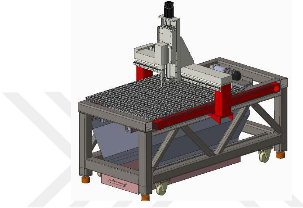
Figure 3.8 New design CNC machine view and X-Axis is colored with red
