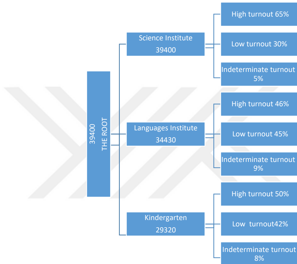
Figure 2.2 Neutrosophic decisions tree
