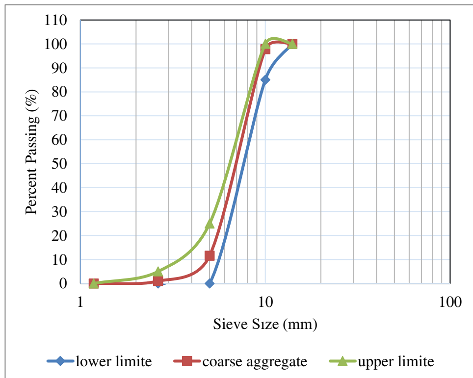
Figure 3.2: Grading of the Coarse Aggregate
