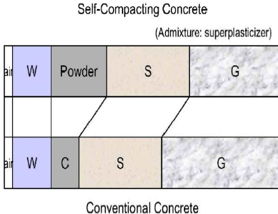
Figure 2.2: Comparison of Mixture Proportioning between SCC and Conventional Concrete (Okamura & Ouchi, 2003)
