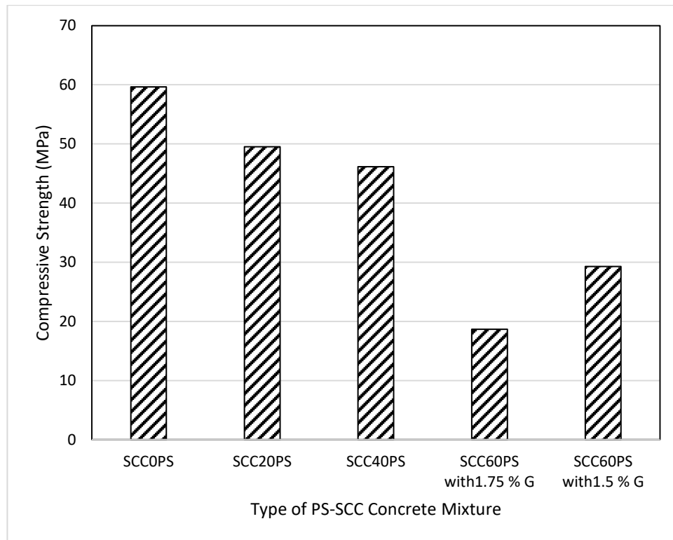
Figure 4.7: Compressive Strength Test Results of PS-SCC Concrete
