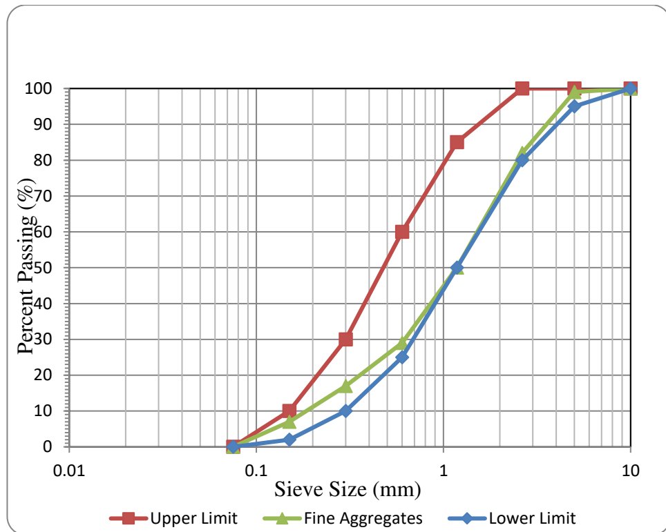
Figure 3.1: Grading of the Fine Aggregate
