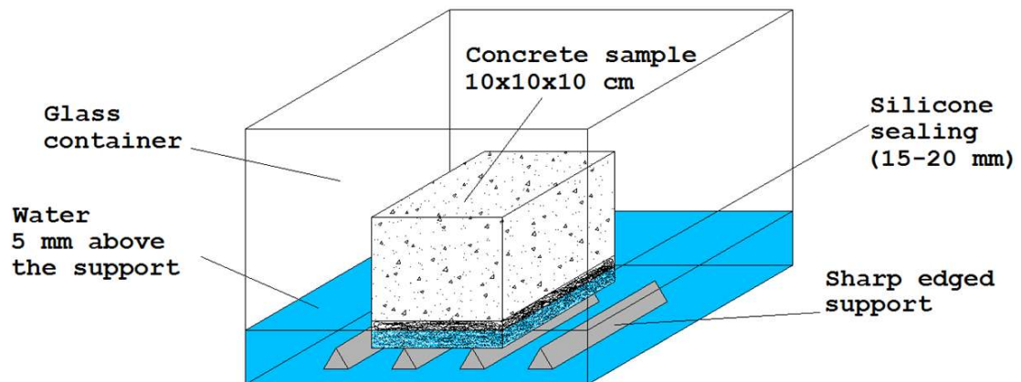
Figure 3.4: Sorptivity test set up
