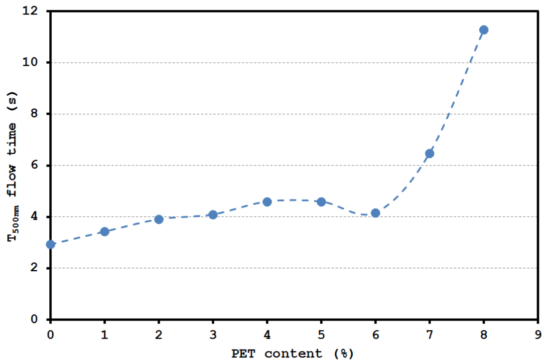
Figure 4.2: Variation of T_{500\text{mm}} slump flow time with PET content
