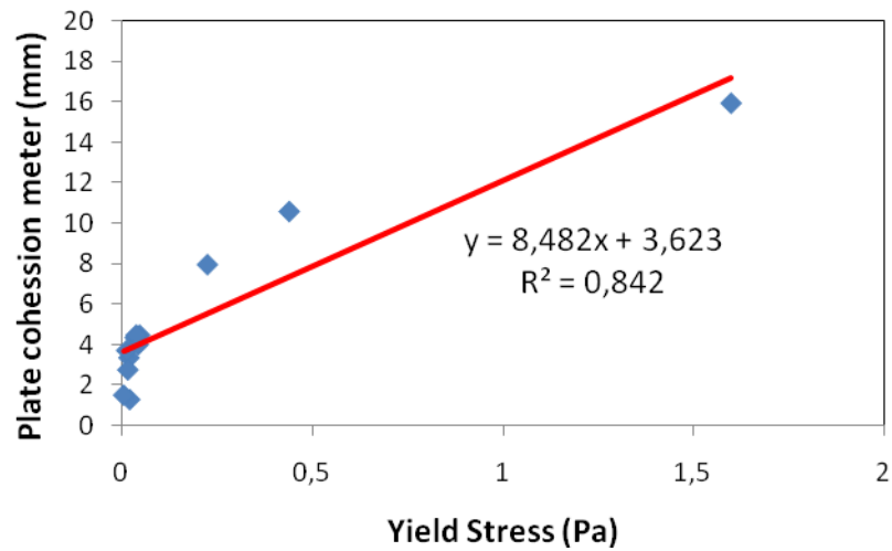
Fig. 4.5. Correlation between rheological and workability properties of grout.
