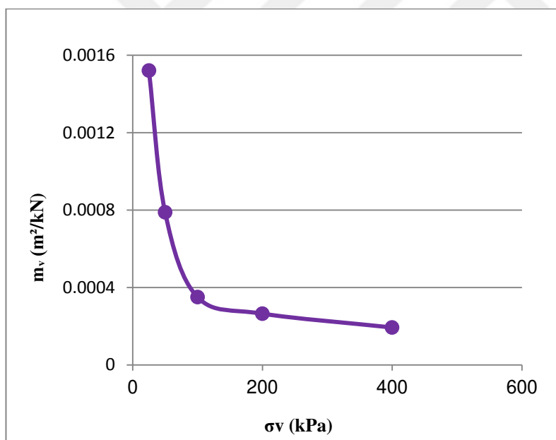
B11: \sigma versus m_v curve of sand colum 2.5 cm
