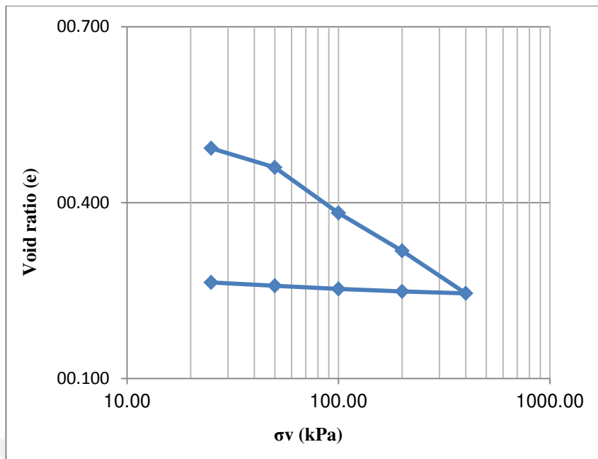
B6: e versus \log \sigma curve of sand colum 1.7 cm
