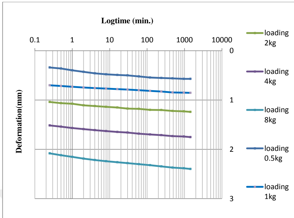
B13: Log time versus deformation curve of sand colum 3.5 cm
