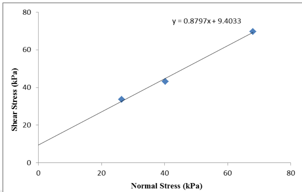
C18: Normal stress versus shear stress for sand colum 3.5(CU)
