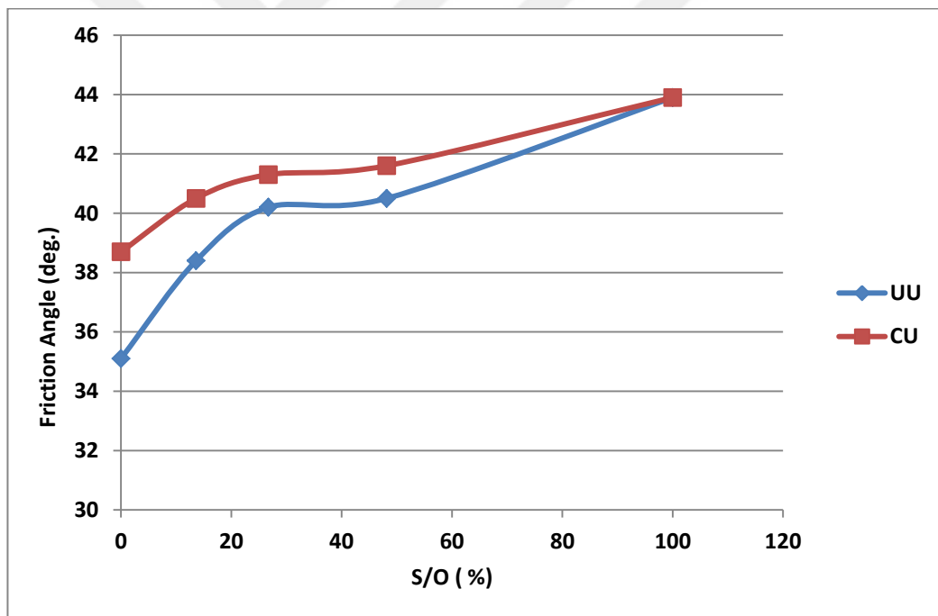
Figure 4.8: Sand column – Internal friction angle relation
