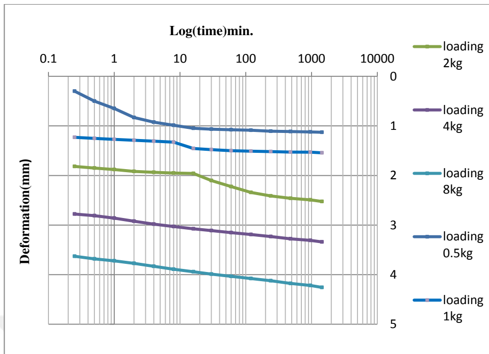
B5: Log time versus deformation curve of sand column 1.7 cm
