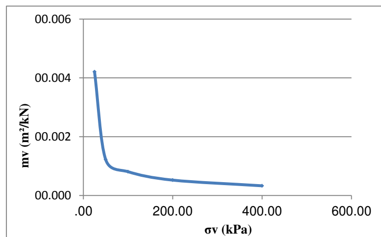
B3: \sigma_v versus m_v curve of organic soil
