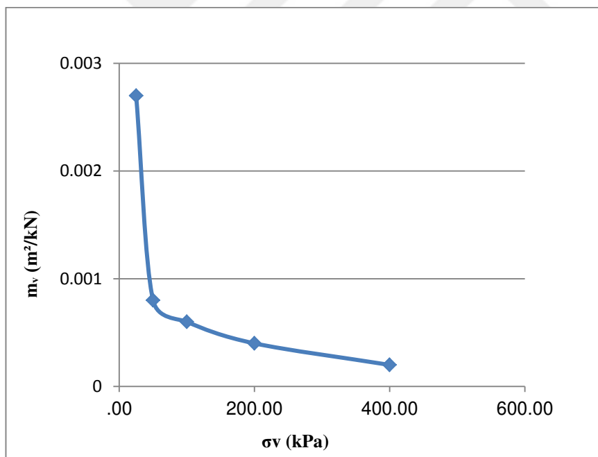
B7: \sigma versus m_v curve of sand colum 1.7 cm
