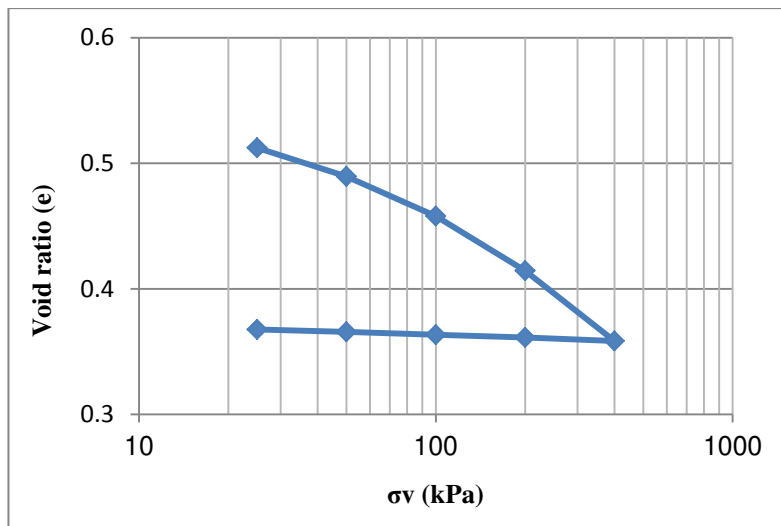
B10: e versus \log \sigma curve of sand colum 2.5 cm
