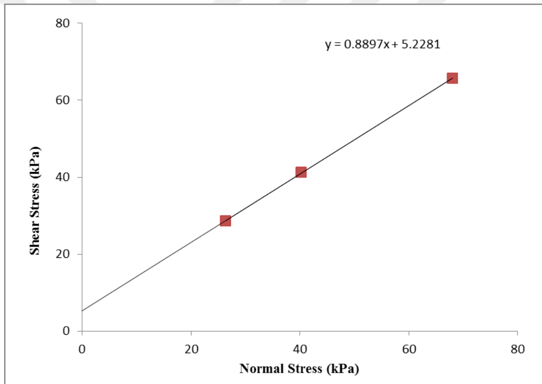
C20: Normal stress versus shear stress for sand colum 4.7 (CU)
