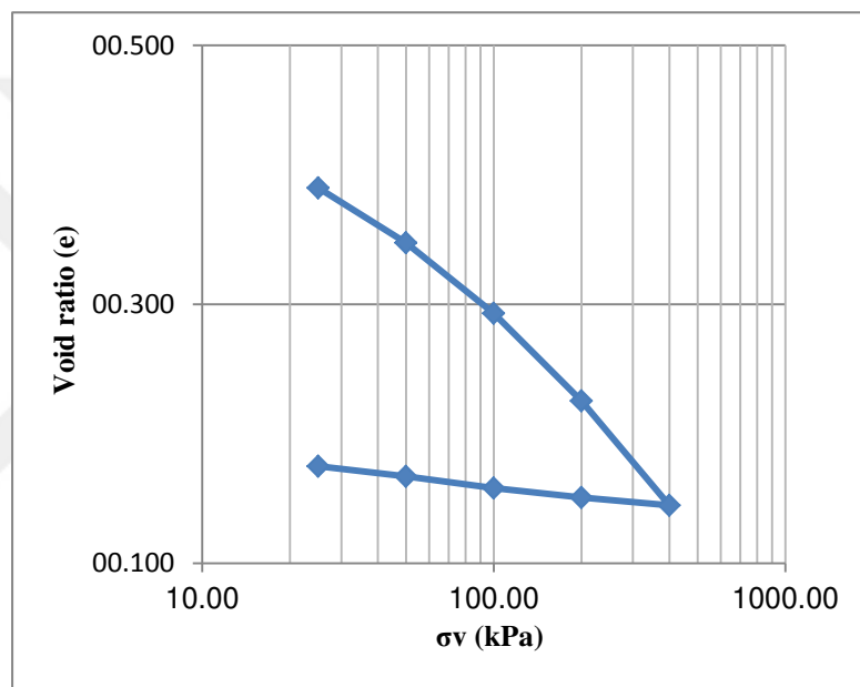
B2: e versus log \sigma_v curve of organic soil
