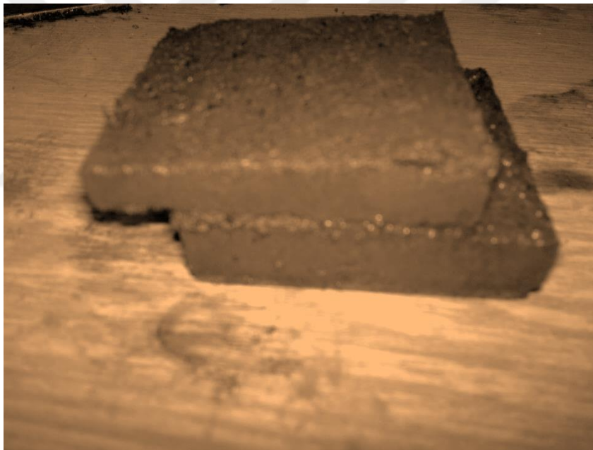
Figure 4.10: Samples of direct shear after testing
