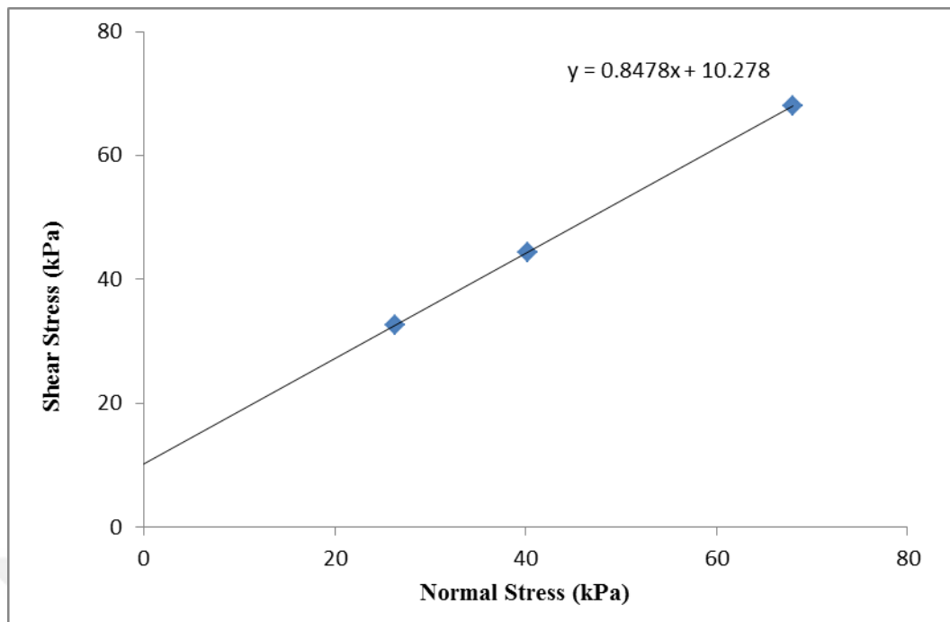
C6: Normal stress versus shear stress for sand colum 3.5 (UU)
