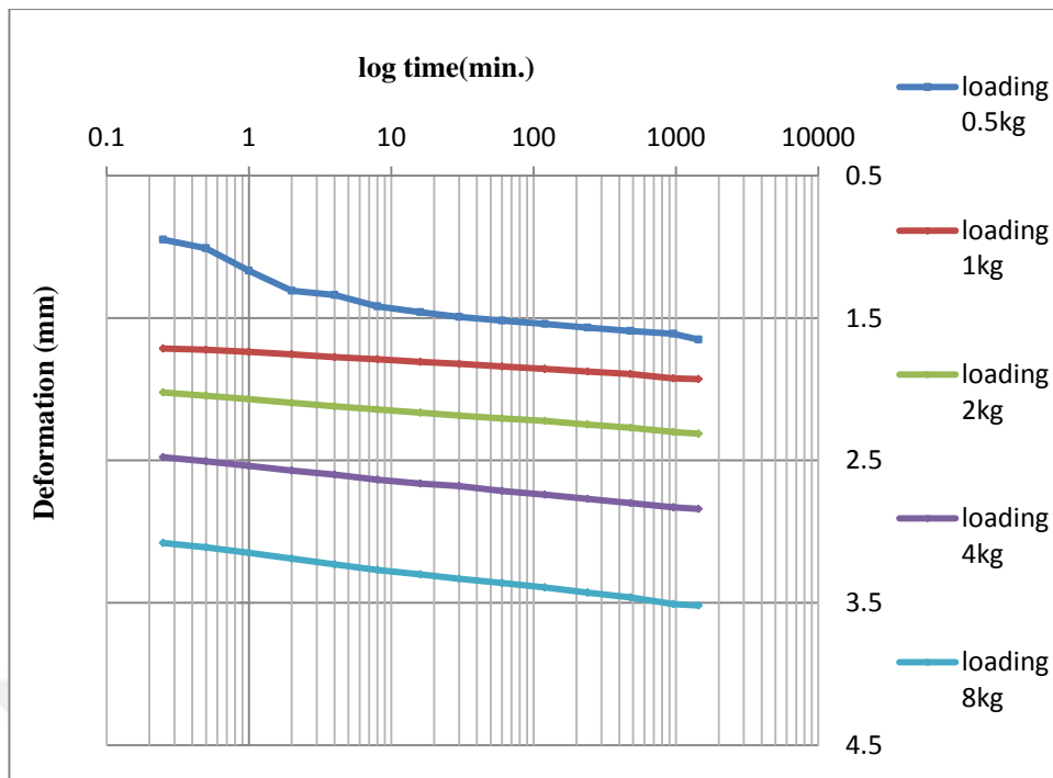
B9: Log time versus deformation curve of sand colum 2.5 cm
