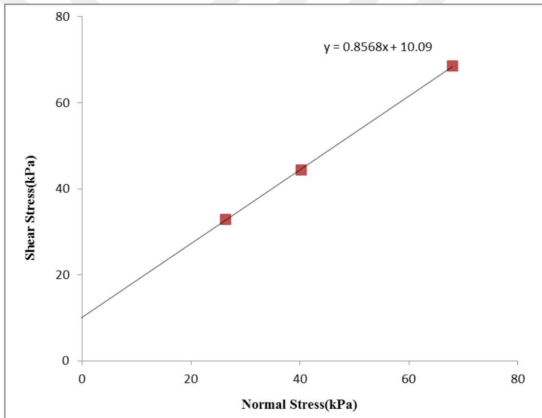
C16: Normal stress versus shear stress for sand colum 2.5 (CU)
