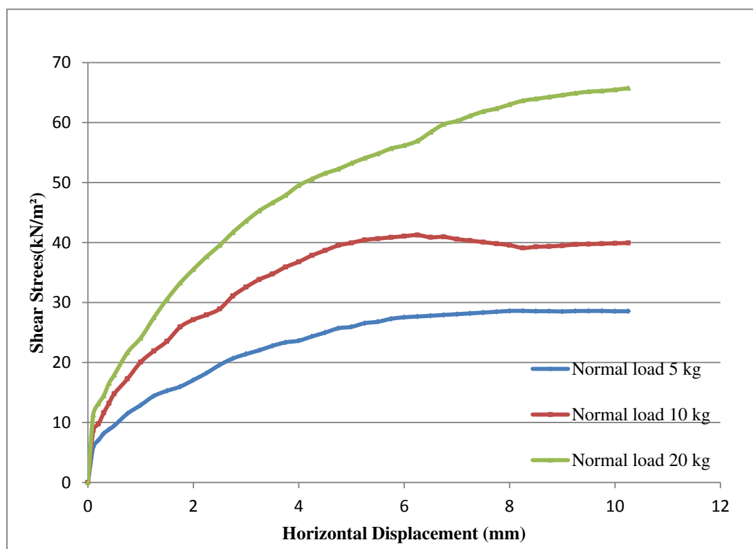
C19: Horizontal displacement versus shear stress for sand colum 4.7 (CU)
