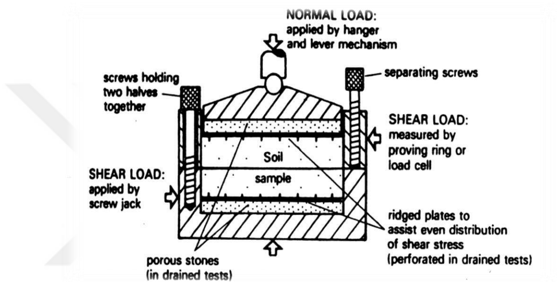
Figure 2.8: Direct shear apparatus (Whitlow, 2001)
