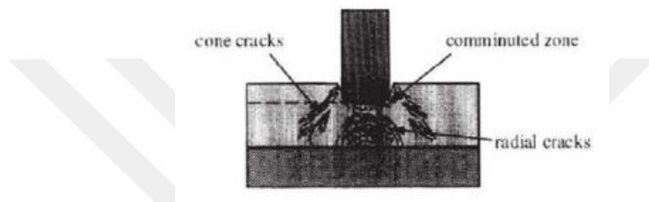
Figure 1.2. Cone and Radial Cracks in Ceramic Tile [1]
