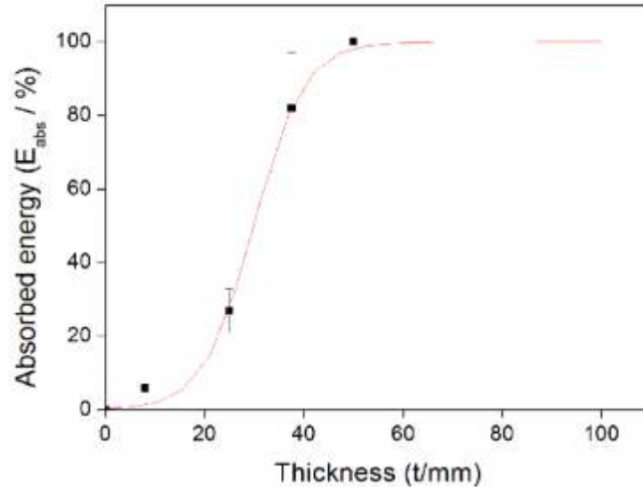
Figure 2.5. Test Results in Terms of Absorbed Energy and Thickness [4]
