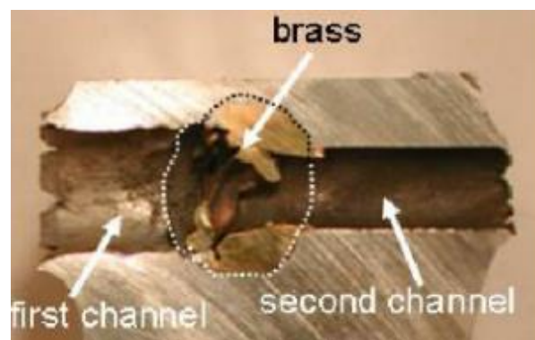
Figure 2.15. Cross Section of the Armor [10]
