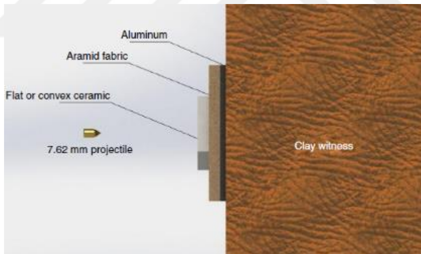
Figure 2.2. Schematic Diagram of the Multi-Layered Armor System [2]
