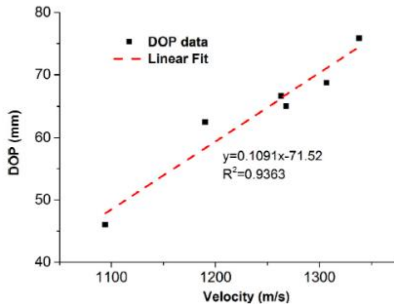
Figure 2.9. Test Results of Depth of Penetration Tests [9]
