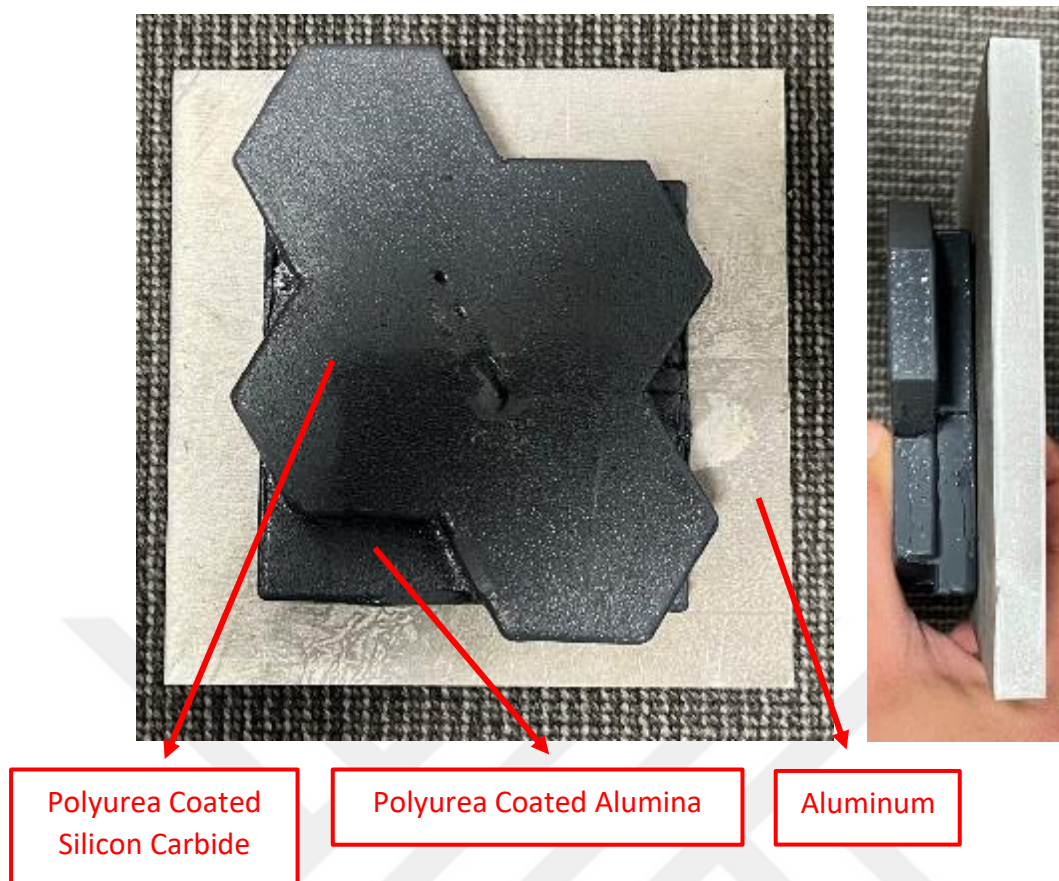
Figure 4.5. Physical Visual of Configuration – 4
