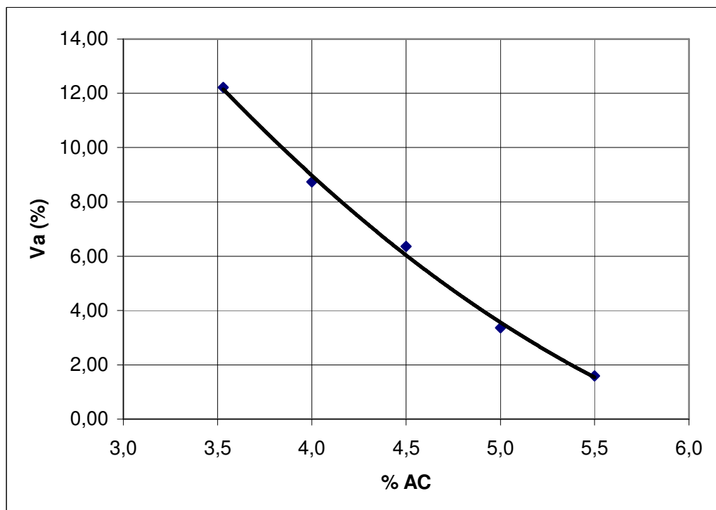
Figure 5.18 Air Voids vs. % AC Graph of Test 3
