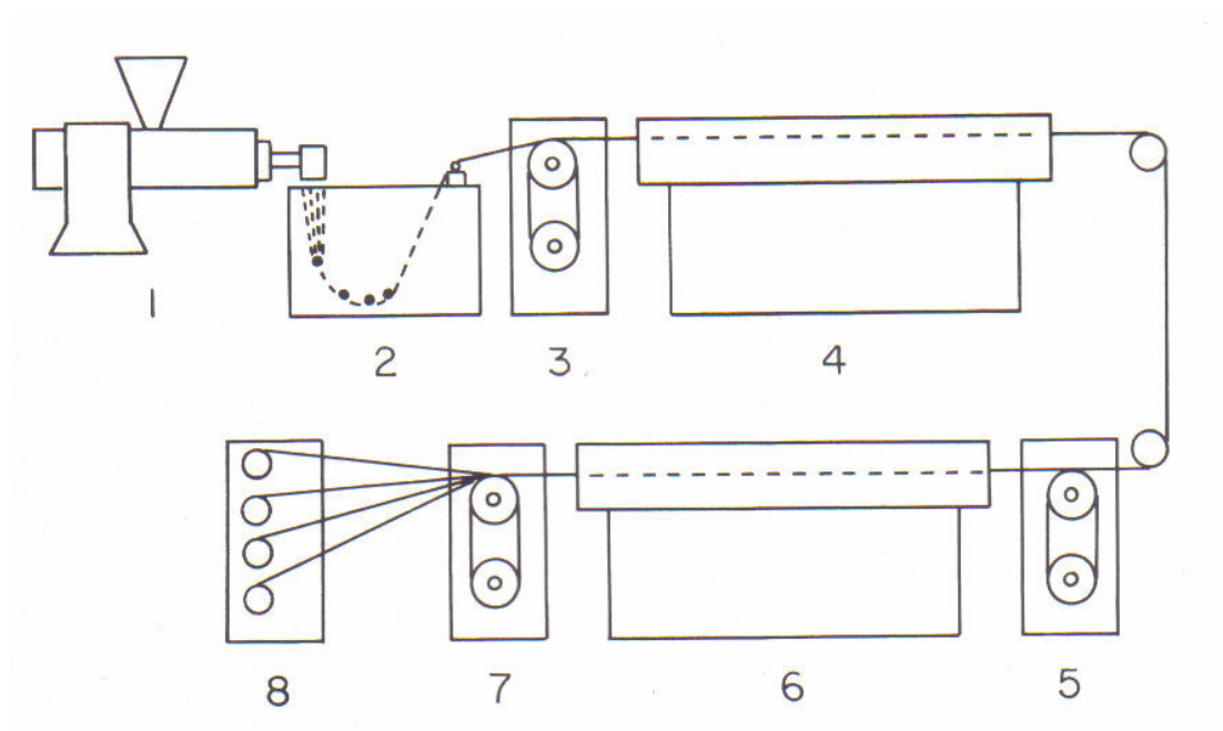
Figure 3.2 Typical Line Diagram For The Extrusion of Polypropylene Monofilaments: (1) Extruder, (2) Quench Tank, (3) Pull-Out Rolls (4) Draw Oven, (5) Draw Rolls, (6) Relax Oven, (7) Relax Rolls, (8) Wind-Up. [46]
