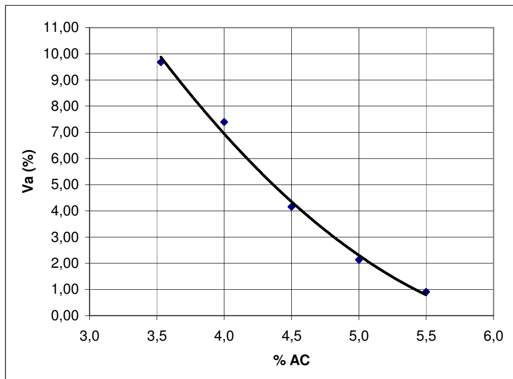
Figure 5.12 Air Voids vs. % AC Graph of Test 2
