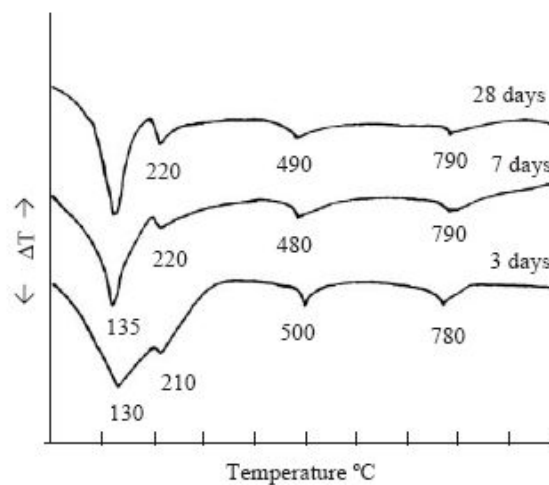
Figure 2.6 Differential thermograms of OPC-metakaolin mix hydrated for different periods [65]
