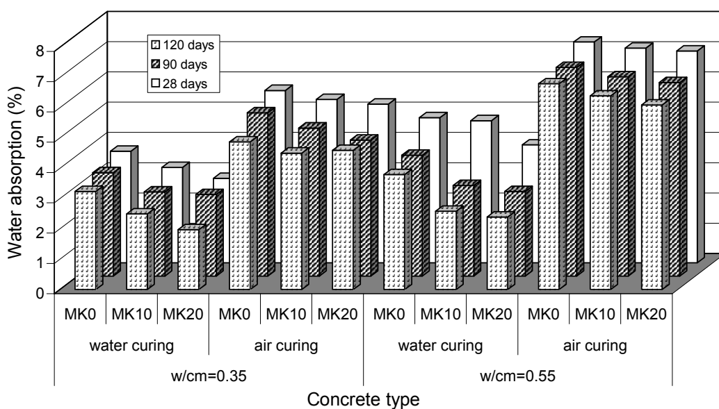
Figure 4.5 Variation in water absorption of plain and metakaolin-modified concretes to different curing regimes
