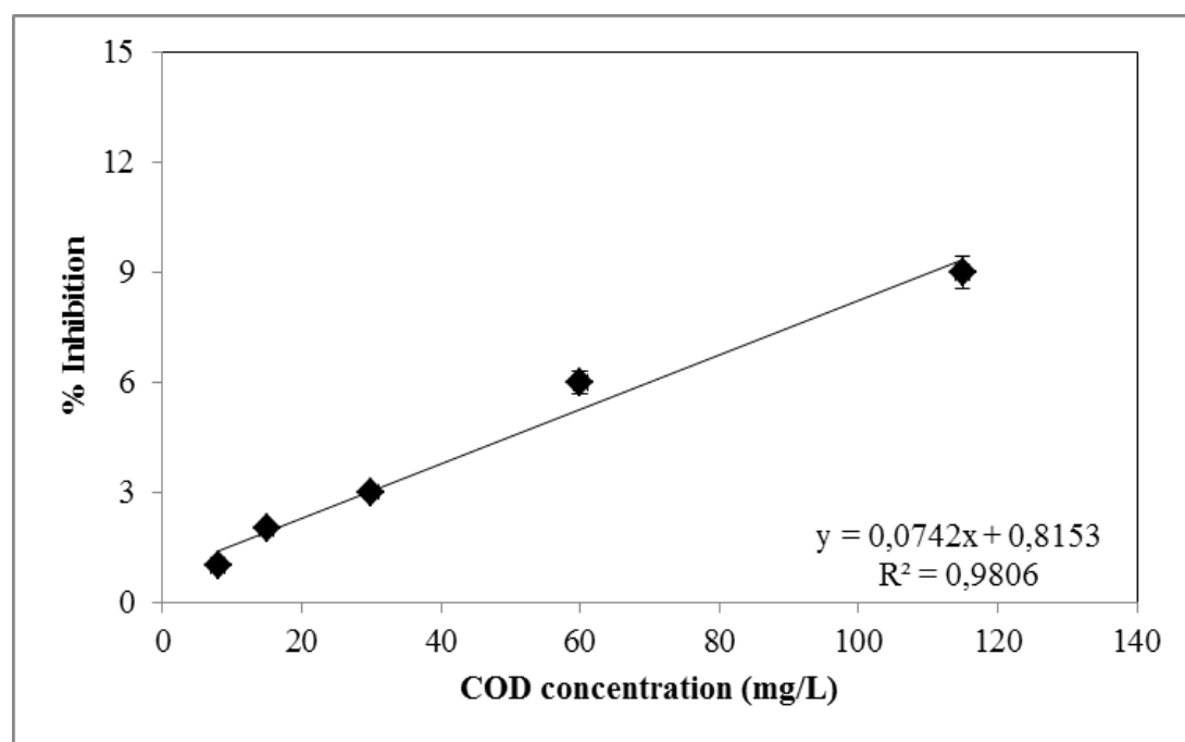
Figure 6.102 Variations of inhibition percentages versus COD_{dis} concentrations in the effluent of aerobic CSTR system at a HRT of 25 days with 15 mg/L RD ( EC_{50} = 663 mg/L, SRT=25 days)
