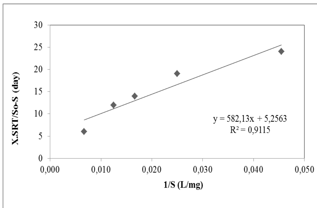
Figure 6.34 Determination of half saturation constant ( K_s ) and maximum rate of substrate utilization ( k ) for COD_{dis} without RD
