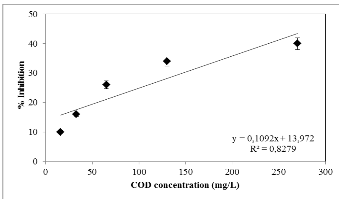
Figure 6.77 Variations of inhibition percentages versus COD dis concentrations in the effluent of aerobic CSTR system at a SRT of 40 days without RD (EC 50 = 330 mg/L, HRT=5 days)
