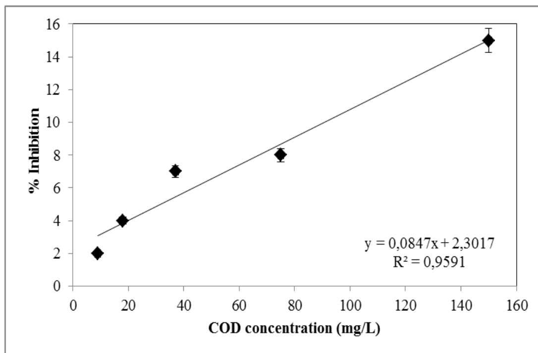
Figure 6.138 Variations of inhibition percentages versus \text{COD}_{\text{dis}} concentrations in the effluent of sequential anaerobic ITBR/aerobic CSTR system at a HRT of 11.00 days with 75 mg/L RD ( \text{EC}_{50} = 563 mg/L)
