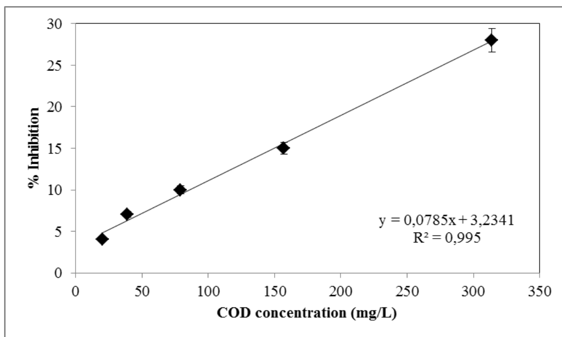
Figure 6.101 Variations of inhibition percentages versus COD_{dis} concentrations in the effluent of aerobic CSTR system at a HRT of 3.3 days with 15 mg/L RD ( EC_{50} = 595 mg/L, SRT=25 days)
