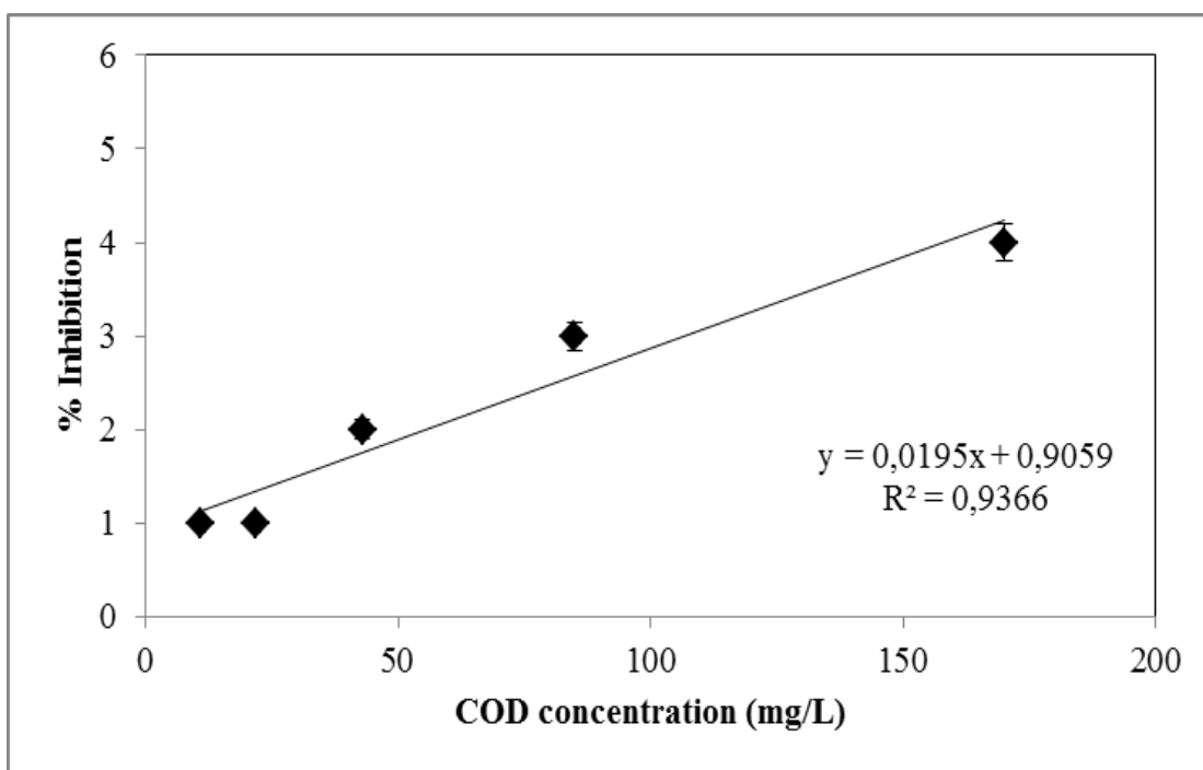
Figure 6.121 Variations of inhibition percentages versus \text{COD}_{\text{dis}} concentrations in the effluent of anaerobic ITBR system at a HRT of 2.75 days with 75 mg/L RD ( \text{EC}_{50} = 2511 mg/L)
