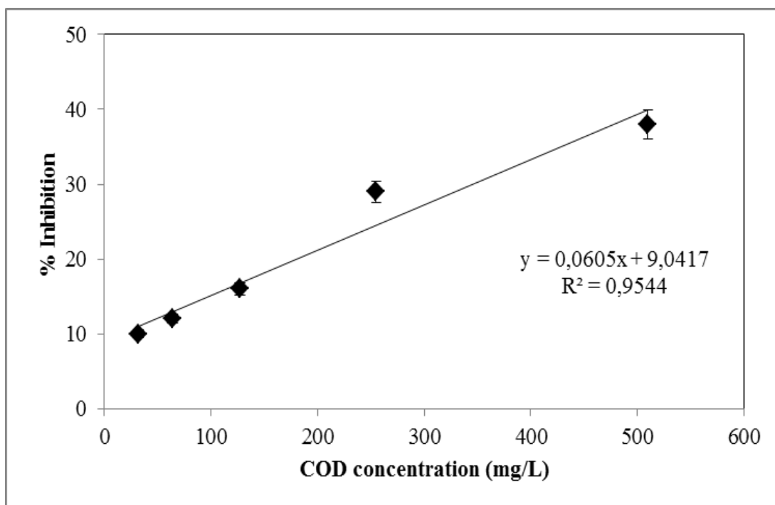
Figure 6.122 Variations of inhibition percentages versus COD_{dis} concentrations in the effluent of anaerobic ITBR system at a HRT of 5.5 days with 75 mg/L RD ( EC_{50} = 677 mg/L)
