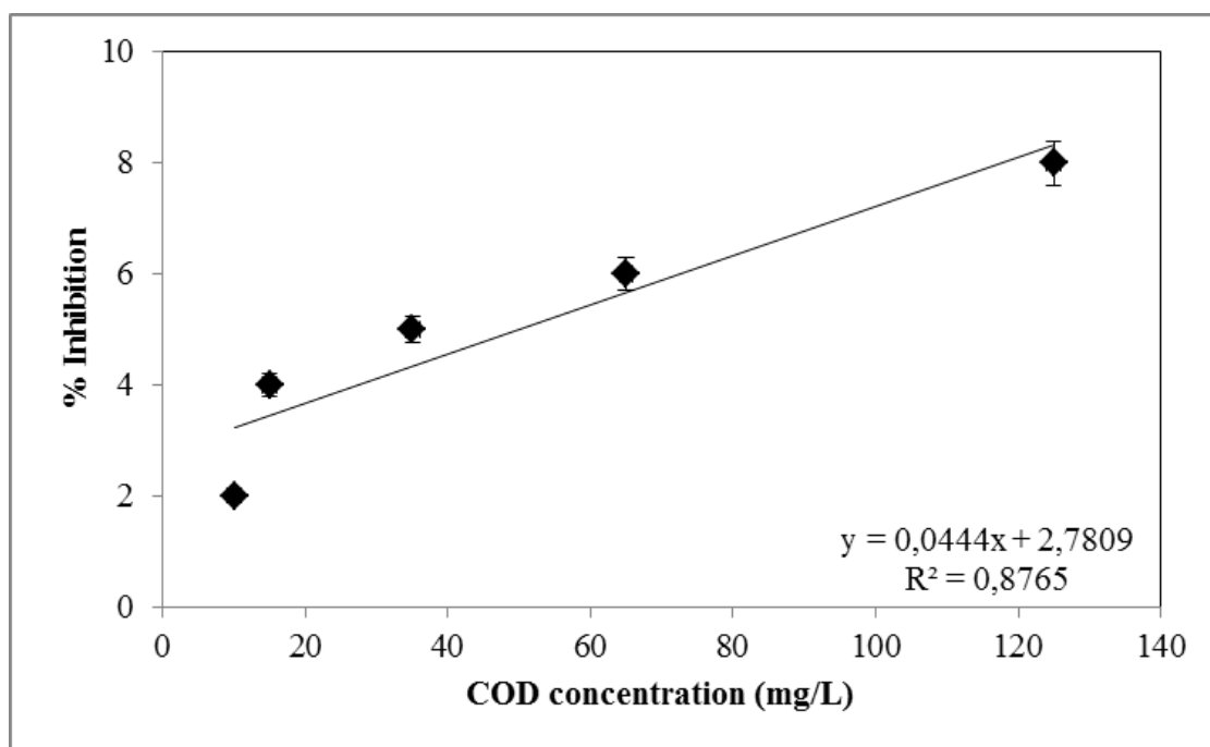
Figure 6.132 Variations of inhibition percentages versus COD_{dis} concentrations in the effluent of sequential anaerobic ITBR/aerobic CSTR system at a HRT of 5.50 days with 75 mg/L RD ( EC_{50} = 1064 mg/L)
