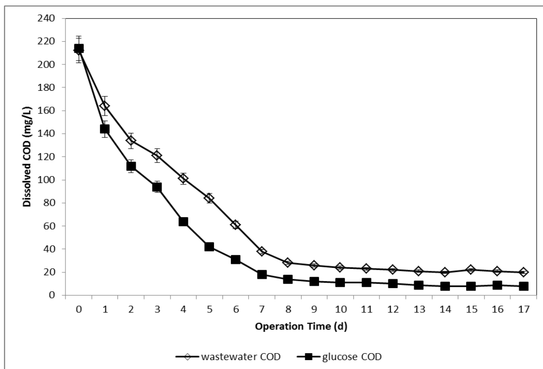
Figure 6.12 Variation of the COD_{dis} concentration with time in the effluent of glucose reactor ( COD_i = 12 \text{ mg/L} )
