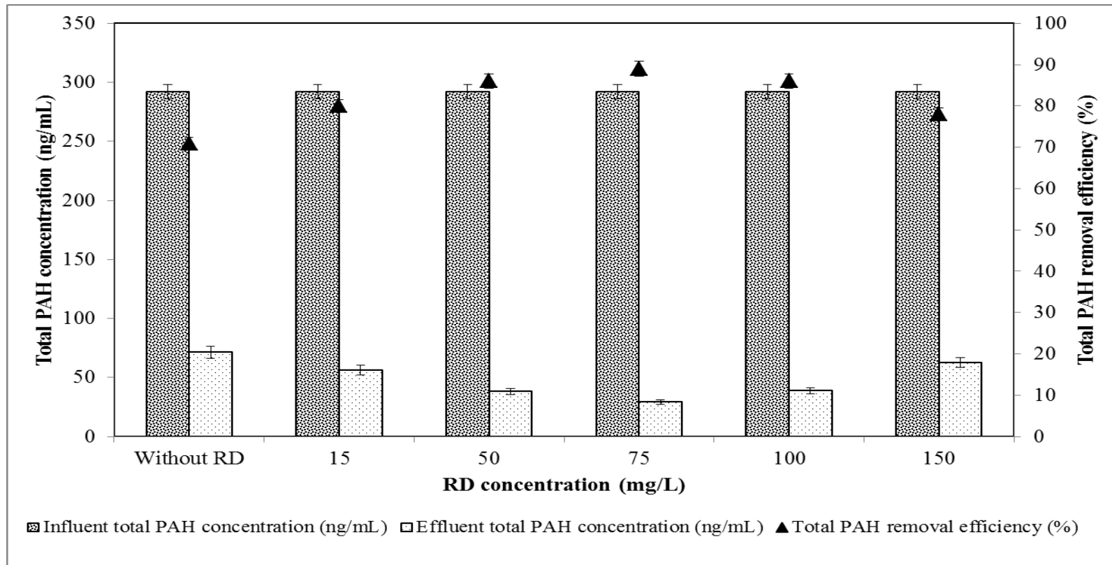
Figure 6.19 PAH removal efficiencies in the anaerobic ITBR system at increasing RD concentrations (influent PAH concentration=292 ng/mL, HRT=2.75 days, SRT=63 days, OLR= 106.18 ng PAH/mL.day)
