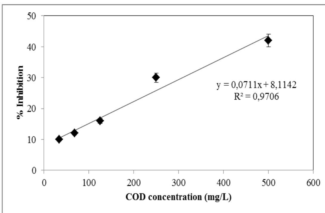
Figure 6.123 Variations of inhibition percentages versus COD_{dis} concentrations in the effluent of anaerobic ITBR system at a HRT of 11 days with 75 mg/L RD ( EC_{50} = 589 mg/L)
