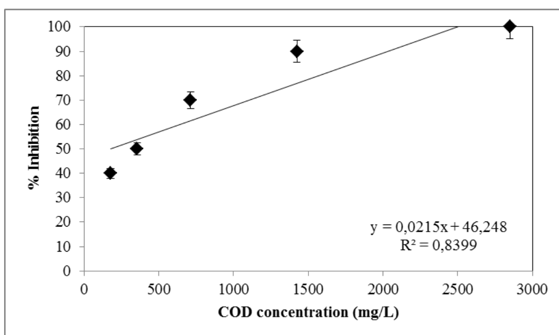
Figure 6.86 Variations of inhibition percentages versus COD_{dis} concentrations in the influent raw petrochemical wastewater ( EC_{50} = 174 mg/L, SRT=25 days)
