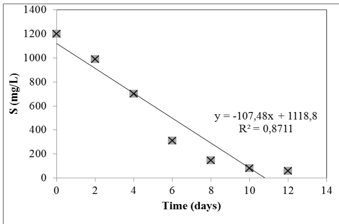
Figure 6.40 The model plot of zero order substrate removal for \text{COD}_{\text{dis}} at a SRT of 25 days with 15 mg/L RD
