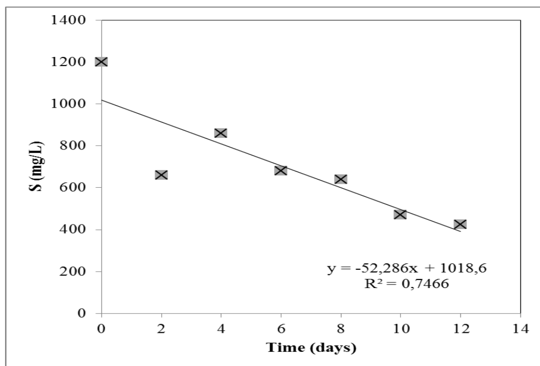
Figure 6.41 The model plot of zero order substrate removal for \text{COD}_{\text{dis}} at a SRT of 25 days without RD
