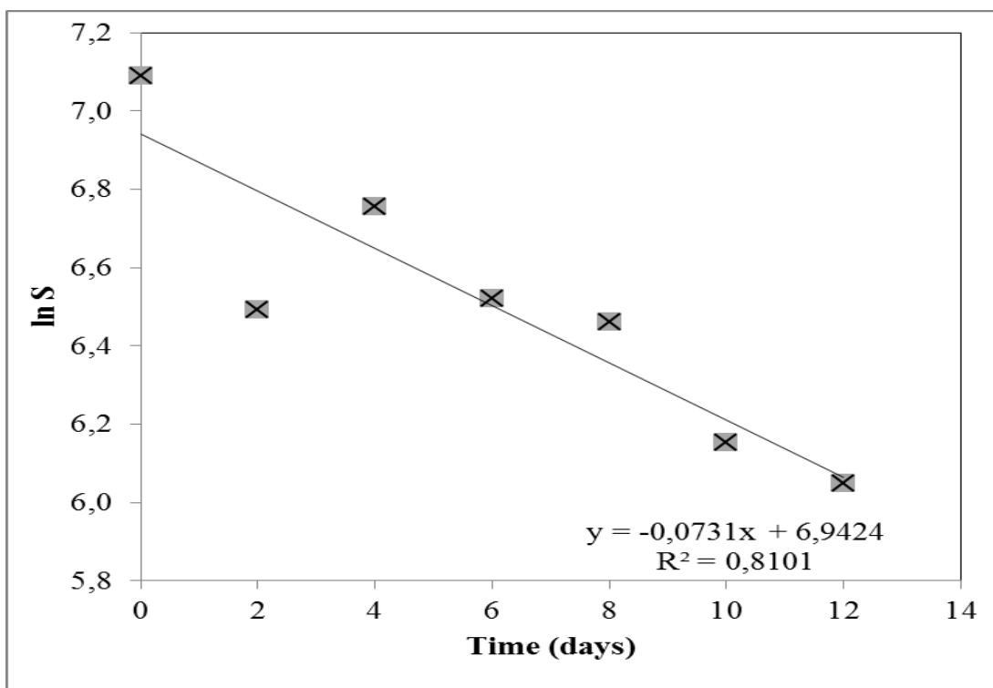
Figure 6.49 Determination of first order substrate removal for \text{COD}_{\text{dis}} without RD at a SRT of 25 days
