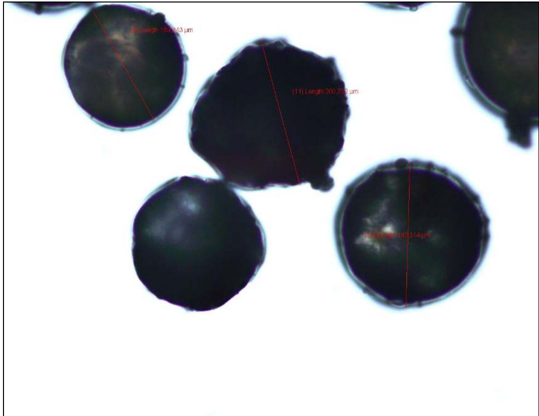
Figure 5.4 Microscopic observation of carrier material before operation the anaerobic ITBR system (magnification 20X10, average diameter: 195 \mu m)
