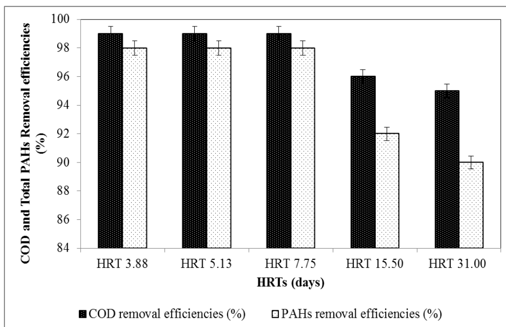
Figure 6.29 COD_{dis} and total PAHs removal efficiencies in the sequential anaerobic ITBR/aerobic CSTR system with increasing HRTs (total OLR=1.039 \text{ g } COD_{dis}/m^3.day and total OLR=113.19 \text{ ngPAH}/mL.day )
