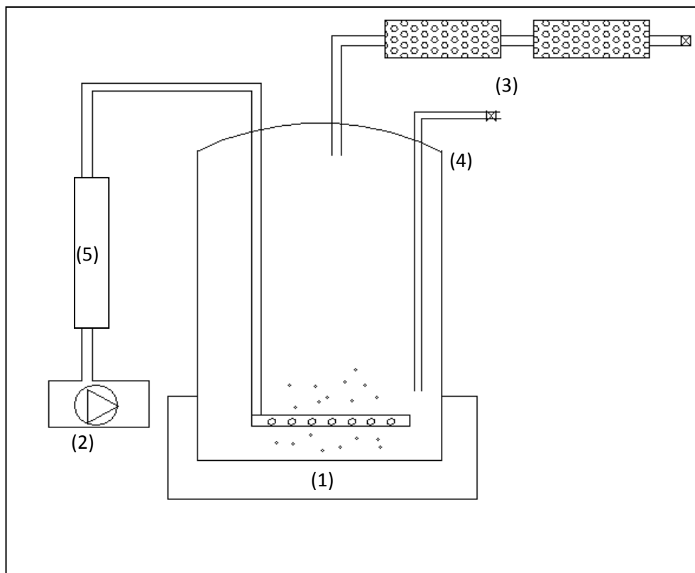
Figure 5.1 Configuration of batch reactors for biodegradation, volatilization and adsorption studies (1: magnetic stirred, 2: air pump, 3: resin colon, 4: sample port)
