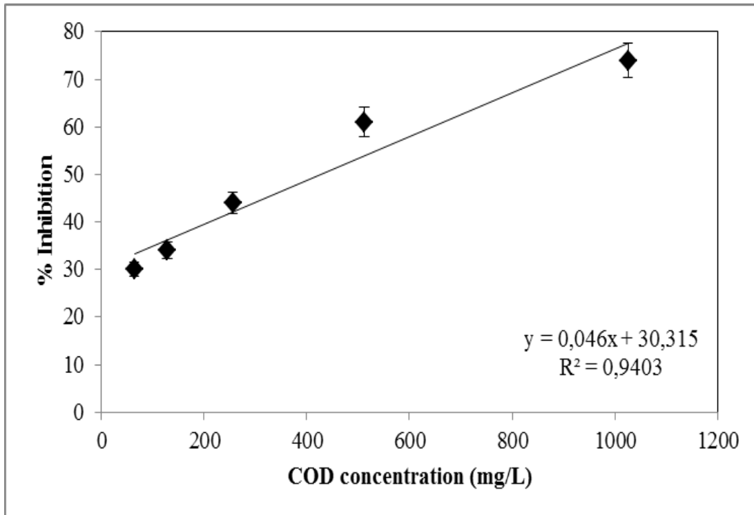
Figure 6.92 Variations of inhibition percentages versus \text{COD}_{\text{dis}} concentrations in the effluent of aerobic CSTR system at a HRT of 2.5 days without RD ( \text{EC}_{50} = 428 \text{ mg/L} , \text{SRT} = 25 \text{ days} )
