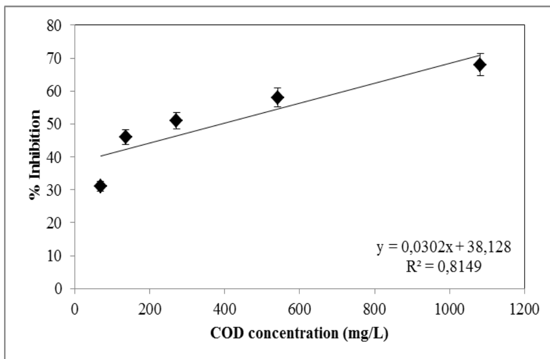
Figure 6.95 Variations of inhibition percentages versus \text{COD}_{\text{dis}} concentrations in the effluent of aerobic CSTR system at a HRT of 10 days without RD ( \text{EC}_{50} = 393 mg/L, SRT=25 days)
