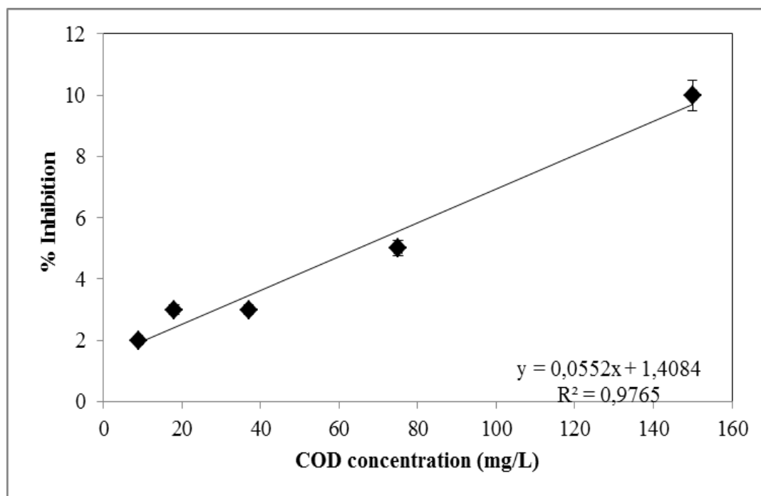
Figure 6.133 Variations of inhibition percentages versus COD_{dis} concentrations in the effluent of sequential anaerobic ITBR/aerobic CSTR system at a HRT of 11.00 days with 75 mg/L RD ( EC_{50} = 880 mg/L)
