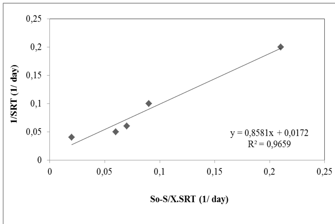
Figure 6.33 Determination of yield coefficient ( Y ), maximum specific substrate utilization rate ( \mu_{max} ), death rate constant ( k_d ) for COD_{dis} at 15 mg/L RD
