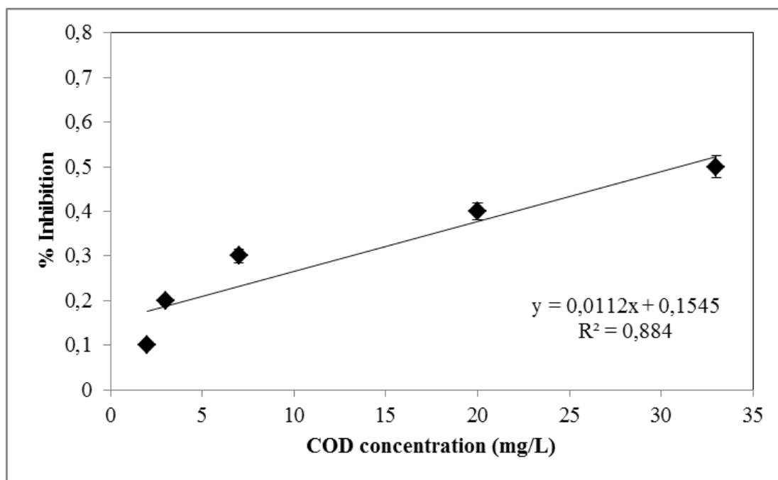
Figure 6.131 Variations of inhibition percentages versus COD_{dis} concentrations in the effluent of sequential anaerobic ITBR/aerobic CSTR system at a HRT of 2.75 days with 75 mg/L RD ( EC_{50} = 4455 mg/L)
