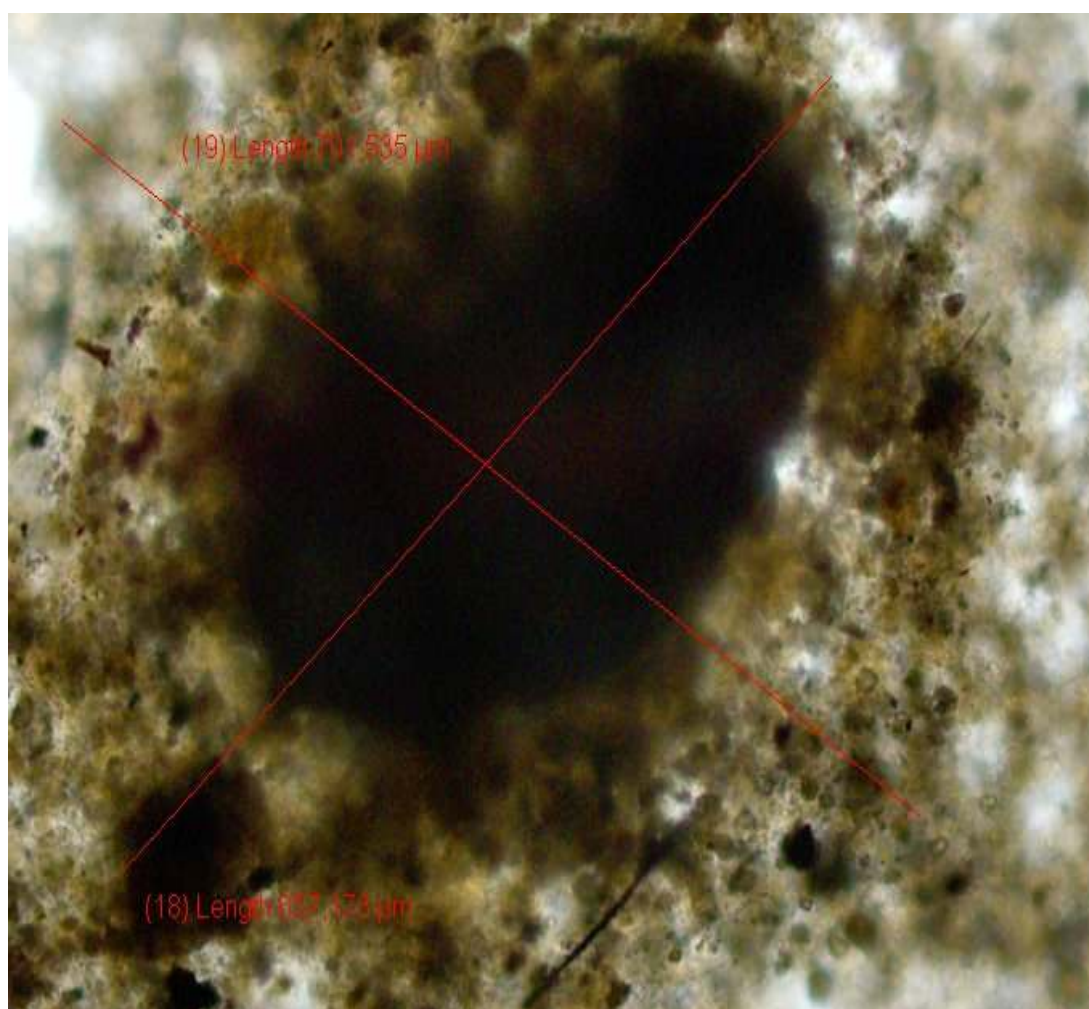
Figure 6.30 Microscopic observation of carrier at the end of operation period in the anaerobic ITBR system at 75 mg/L RD (magnification 20X10, average diameter: 675µm)
