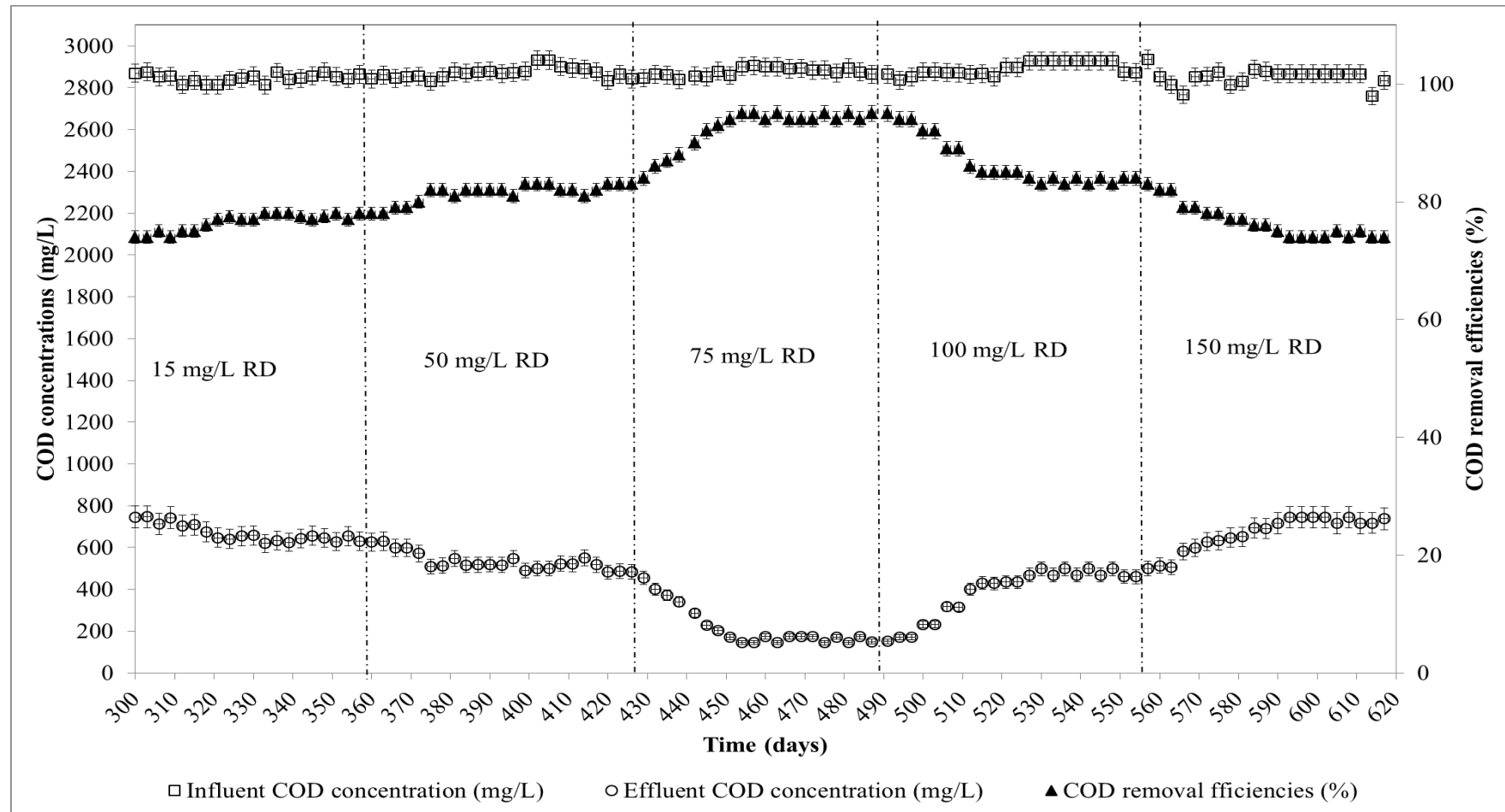
Figure 6.18 Variations of COD dis concentrations (mg/L) and removal efficiencies (%) in the continuous operation periods in the ITBR system containing 15, 50, 75, 100 and 150 mg/L RD concentrations (influent COD dis concentration=2760-2935 mg/L; effluent COD=150-830 mg/L)
