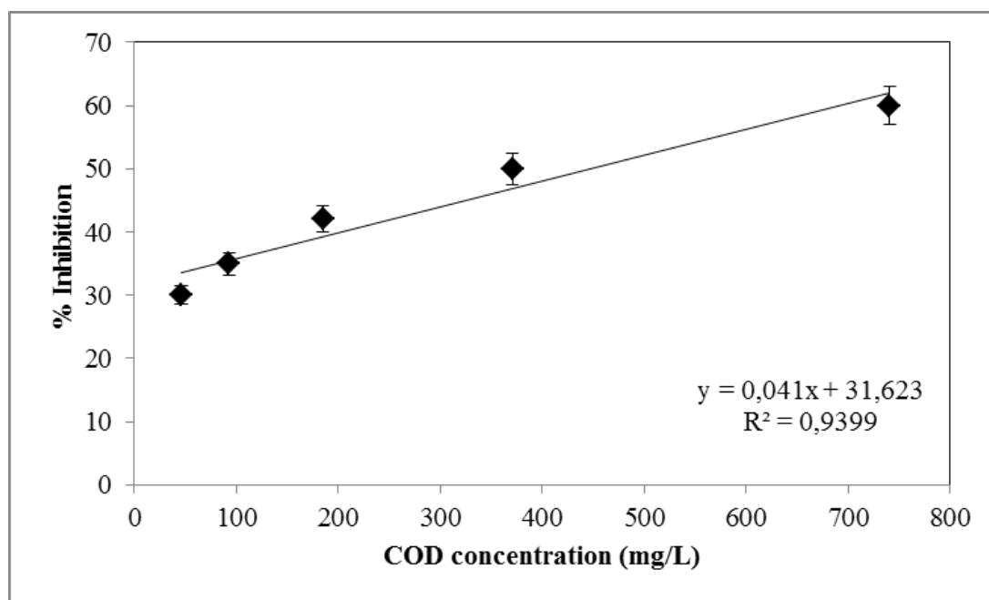
Figure 6.117 Variations of inhibition percentages versus \text{COD}_{\text{dis}} concentrations in the effluent of the anaerobic ITBR system with containing 150 mg/L RD ( \text{EC}_{50} = 448 mg/L SRT=63 days, HRT= 2.75 days)
