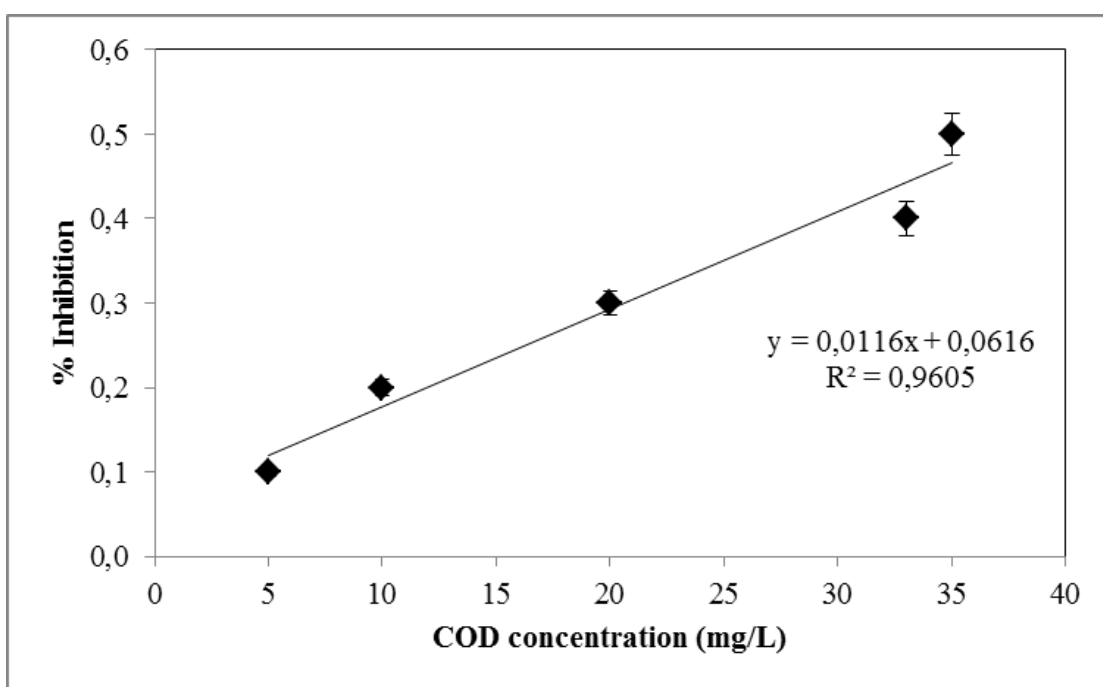
Figure 6.130 Variations of inhibition percentages versus COD_{dis} concentrations in the effluent of sequential anaerobic ITBR/aerobic CSTR system at a HRT of 1.83 days with 75 mg/L RD ( EC_{50} = 4315 mg/L)
