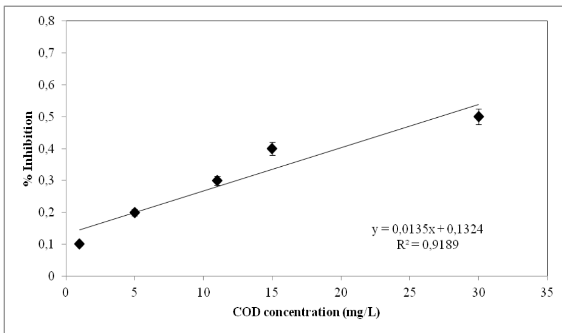
Figure 6.129 Variations of inhibition percentages versus COD_{dis} concentrations in the effluent of sequential anaerobic ITBR/aerobic CSTR system at a HRT of 1.38 days with 75 mg/L RD ( EC_{50} = 3690 mg/L)
