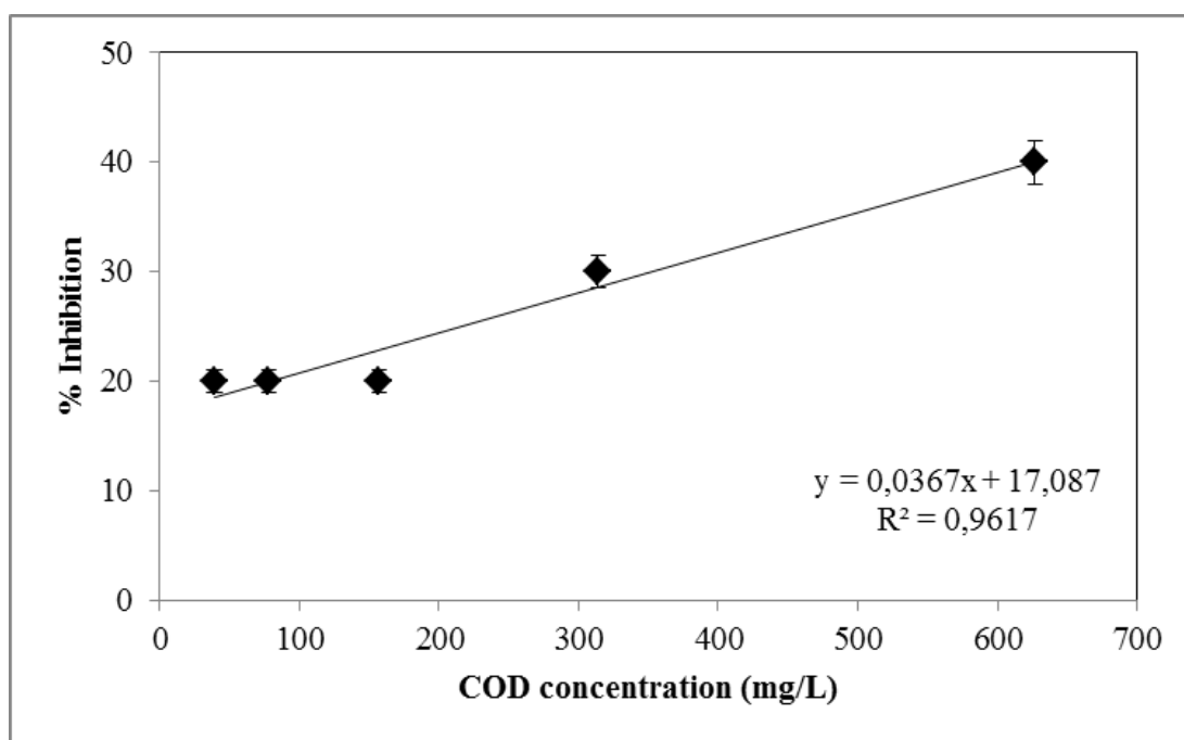
Figure 6.96 Variations of inhibition percentages versus COD_{dis} concentrations in the effluent of aerobic CSTR system at a HRT of 2.5 days with 15 mg/L RD ( EC_{50} = 897 mg/L, SRT=25 days)
