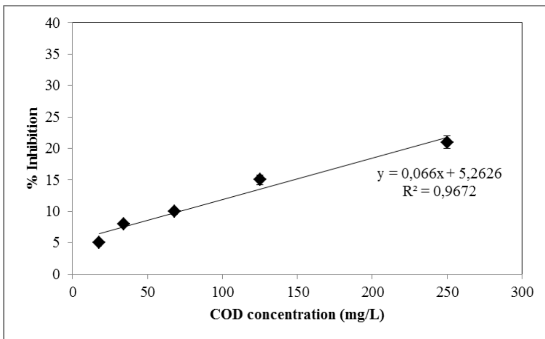
Figure 6.71 Variations of % inhibition versus COD concentration in the effluent of the aerobic CSTR for SRT 25 days EC_{50} = 678 mg/L without RD at a HRT of 5 days
