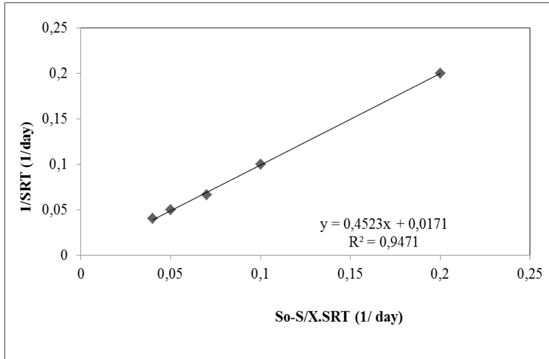
Figure 6.35 Determination of yield coefficient ( Y ), maximum specific substrate utilization rate ( \mu_{max} ), death rate constant ( k_d ) for COD_{dis} without RD
