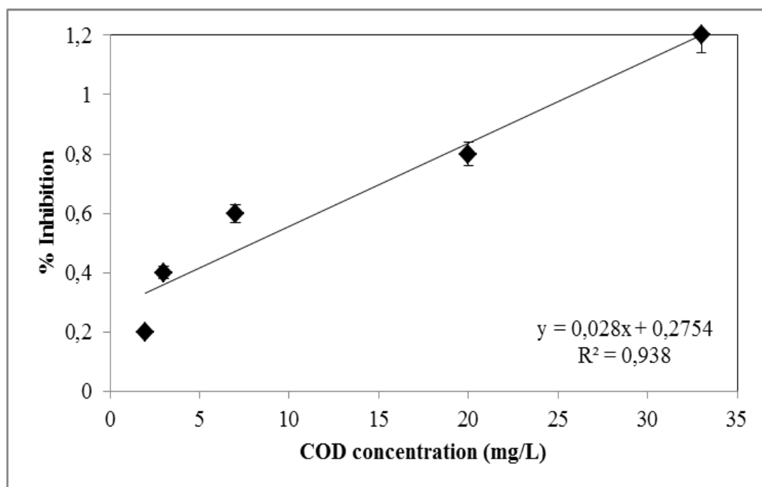
Figure 6.136 Variations of inhibition percentages versus COD_{dis} concentrations in the effluent of sequential anaerobic ITBR/aerobic CSTR system at a HRT of 2.75 days with 75 mg/L RD ( EC_{50} = 1773 mg/L)
