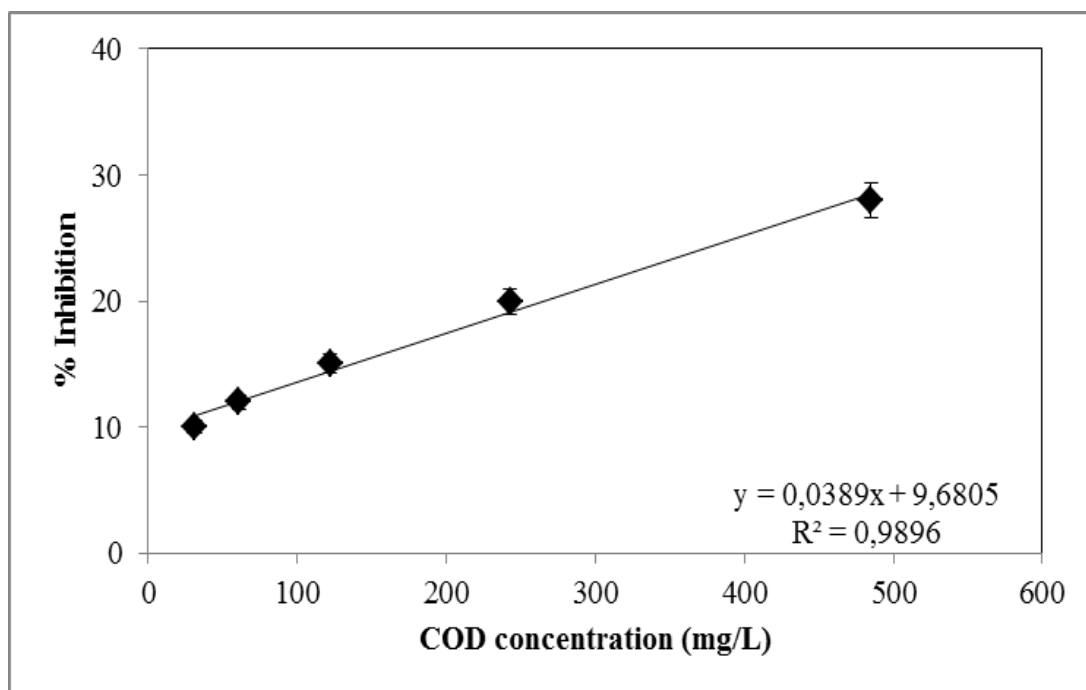
Figure 6.107 Variations of inhibition percentages versus COD_{dis} concentrations in the effluent of anaerobic ITBR system with containing 50 mg/L RD ( EC_{50} = 1038 mg/L, SRT=63 days, HRT= 2.75 days)
