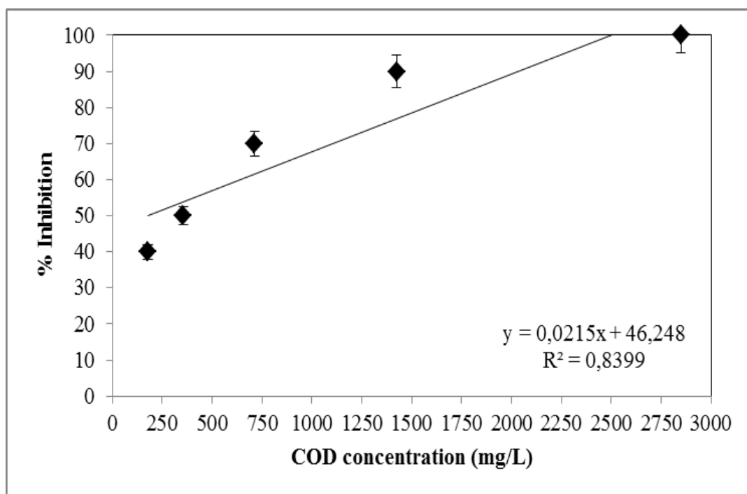
Figure 6.118 Variations of inhibition percentages versus \text{COD}_{\text{dis}} concentrations in the influent raw petrochemical wastewater ( \text{EC}_{50} = 174 \text{ mg/L} )
