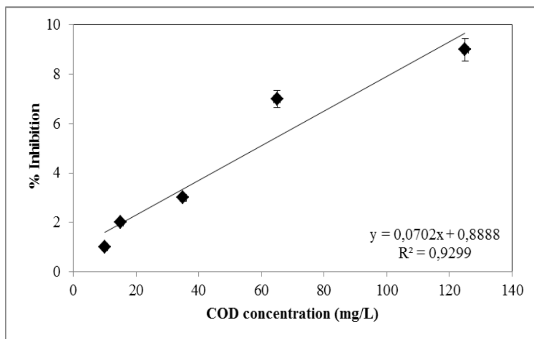
Figure 6.137 Variations of inhibition percentages versus COD_{dis} concentrations in the effluent of sequential anaerobic ITBR/aerobic CSTR system at a HRT of 5.50 days with 75 mg/L RD ( EC_{50} = 699 mg/L)
