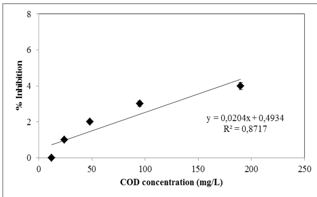
Figure 6.120 Variations of inhibition percentages versus \text{COD}_{\text{dis}} concentrations in the effluent of anaerobic ITBR system at a HRT of 1.83 days with 75 mg/L RD ( \text{EC}_{50} = 2425 mg/L)
