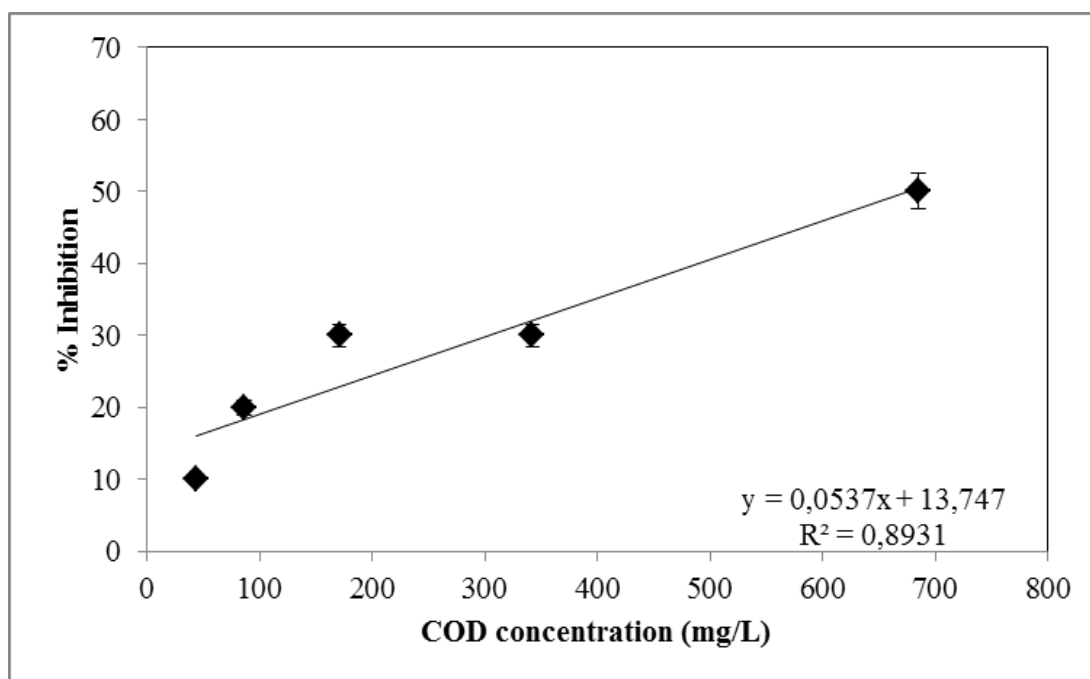
Figure 6.99 Variations of inhibition percentages versus COD dis concentrations in the effluent of aerobic CSTR system at a HRT of 10 days with 15 mg/L RD (EC 50 = 675 mg/L, SRT=25 days)
