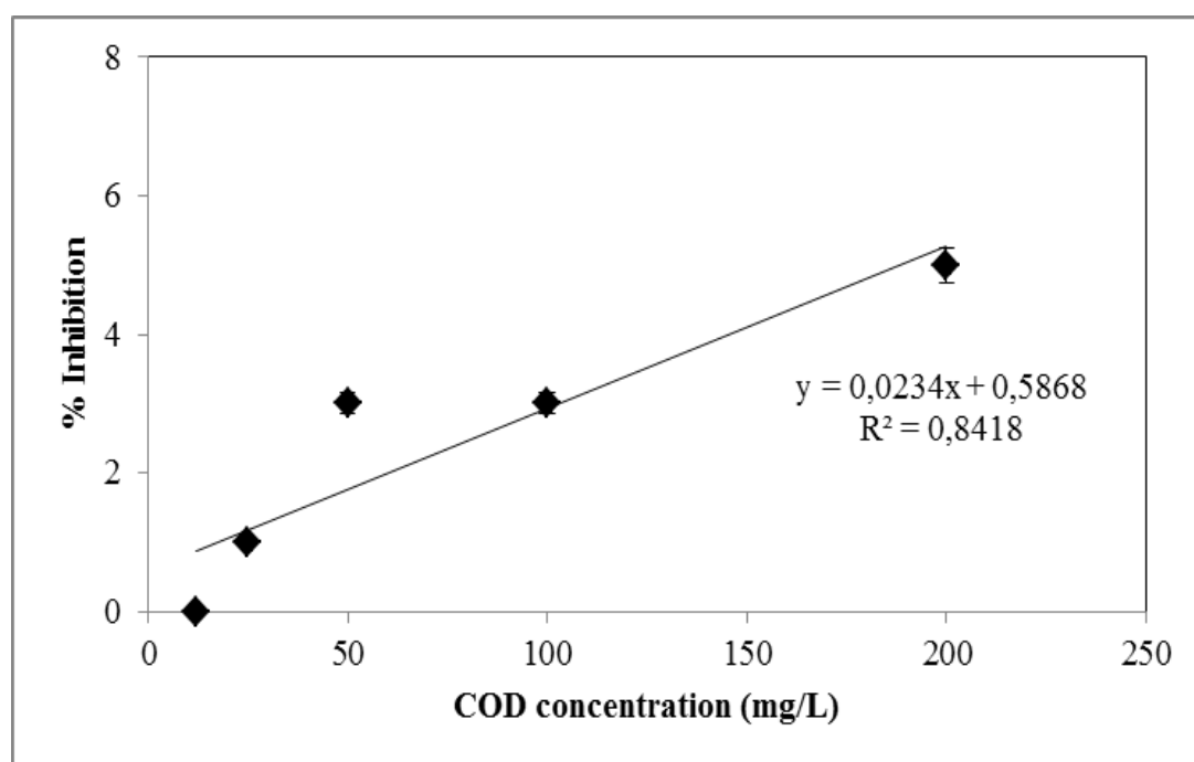
Figure 6.119 Variations of inhibition percentages versus \text{COD}_{\text{dis}} concentrations in the effluent of anaerobic ITBR system at a HRT of 1.38 days with 75 mg/L RD ( \text{EC}_{50} = 2109 \text{ mg/L} )
