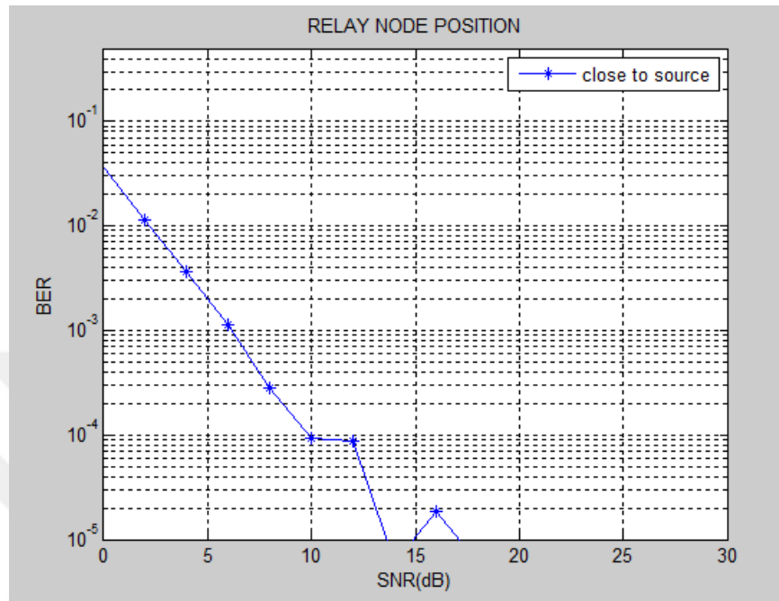
Figure 30. Relay node close to source 1.
