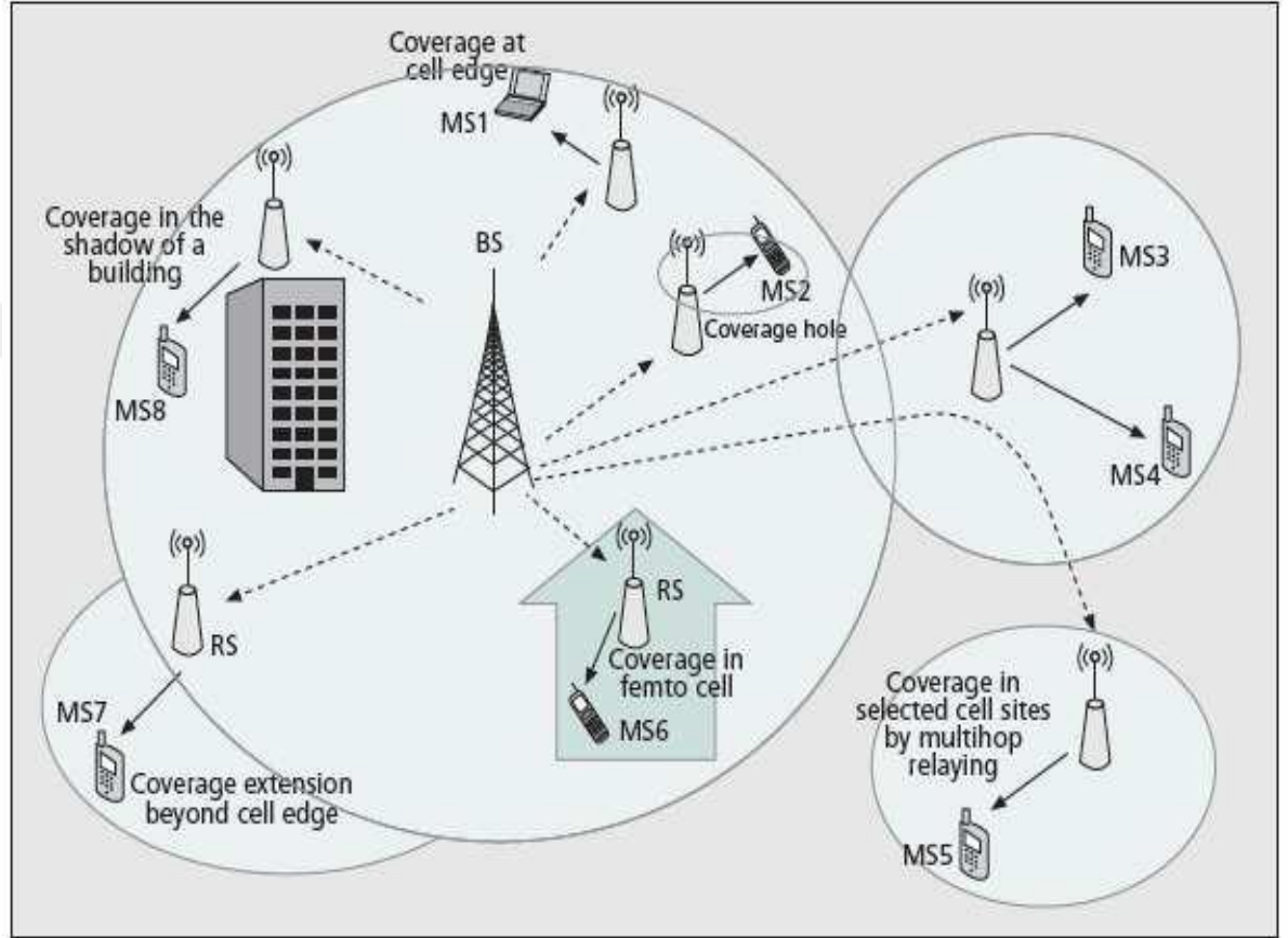
Figure 12. Relay node disposition in a wireless communication [14].
