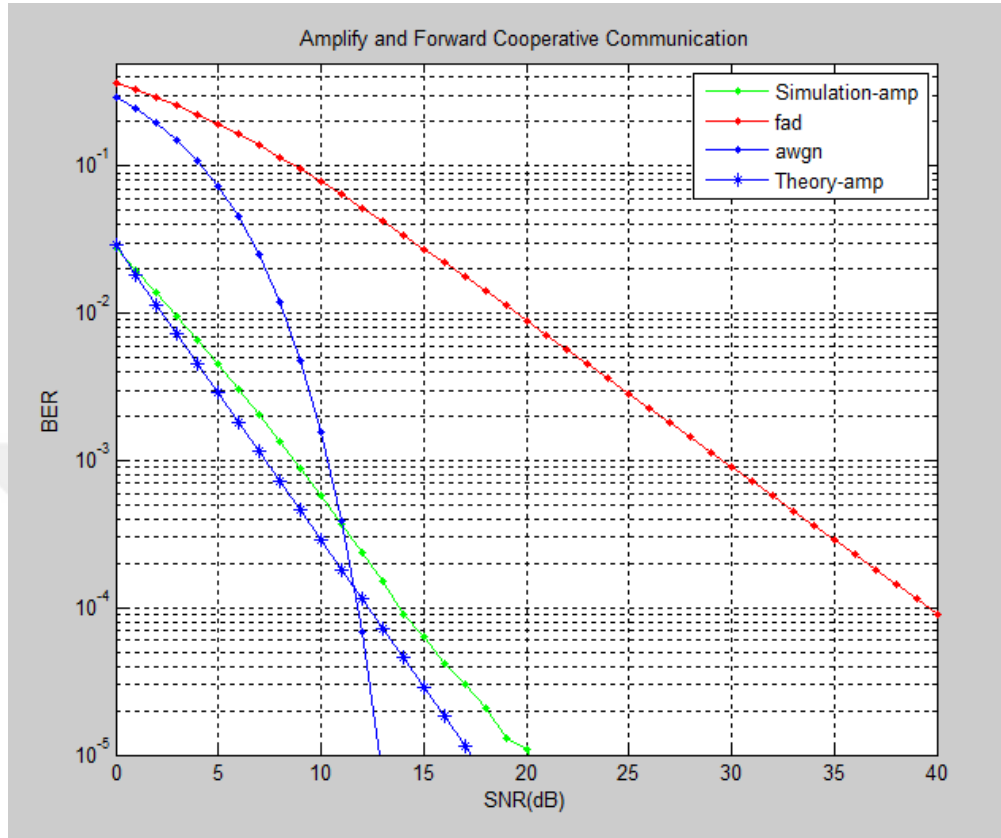
Figure 21. The power of source to relay and relay to destination are same and equal to ten times the source destination power.
