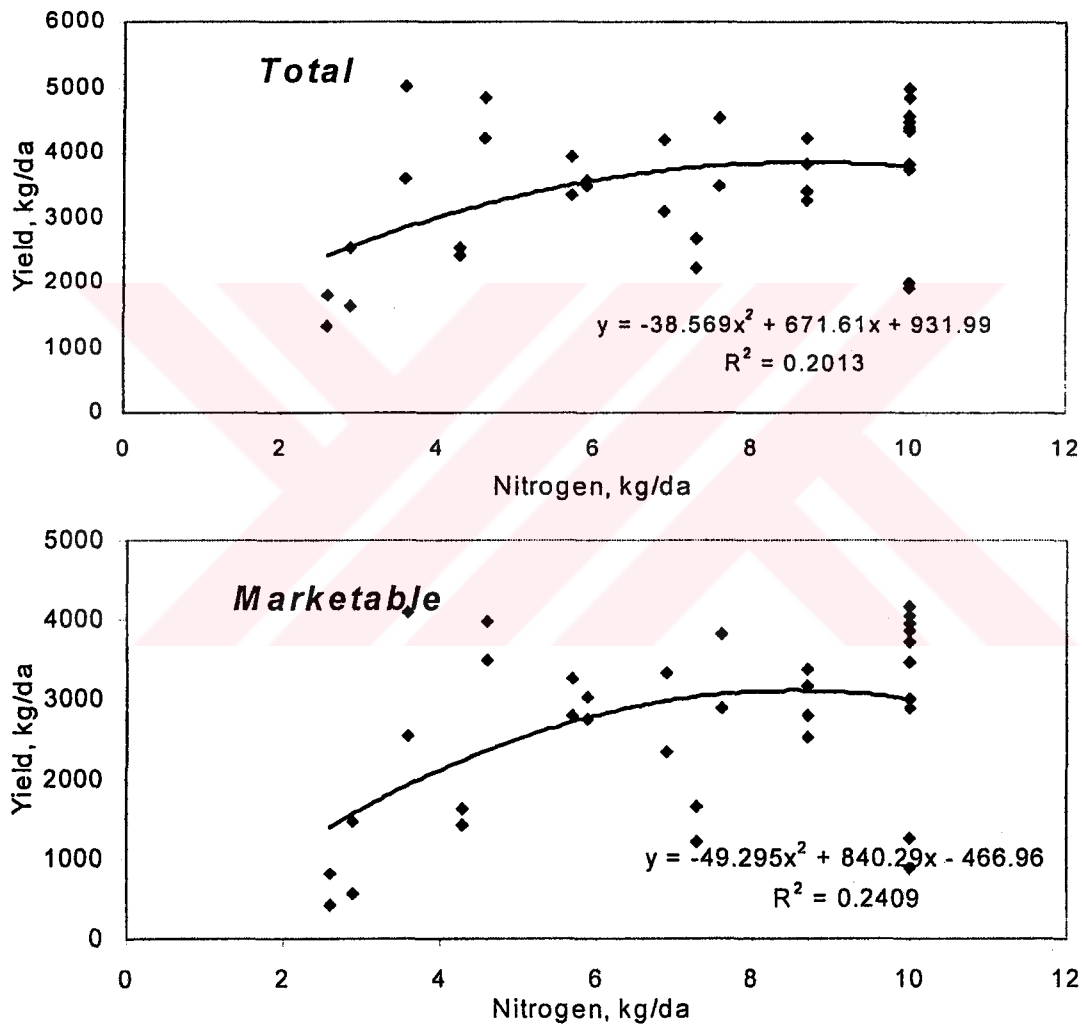
Figure 4.4 Relationships between nitrogen levels and yield (total and marketable)
