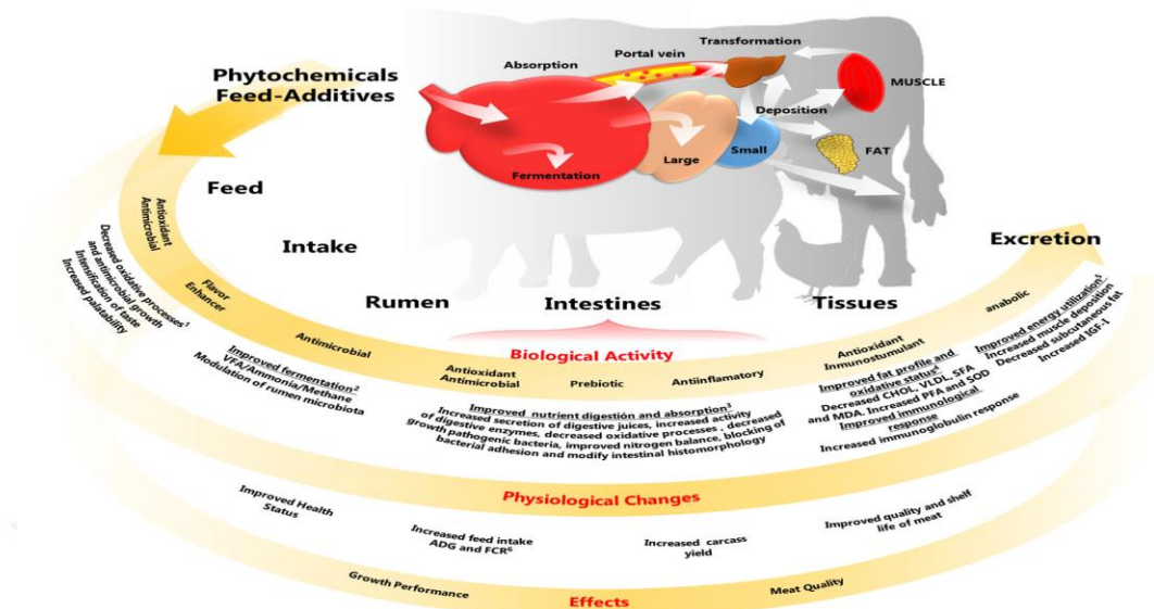
Figure 1.3: Schematic diagram of mechanism of action and effects of PFA
