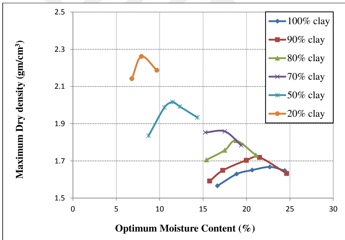
Figure 4.2 The OMC results for clay and sand-clay mixtures
