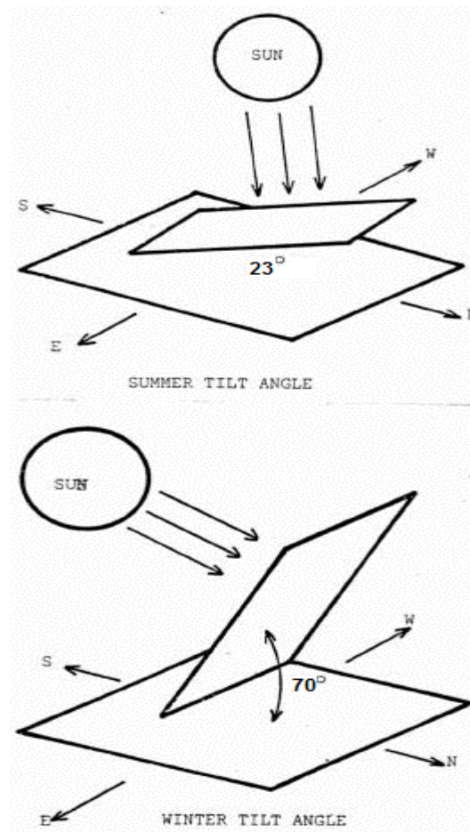
Figure 46. Average solar collector tilt angle in Famagusta http://www.solarpaneltilt.com
