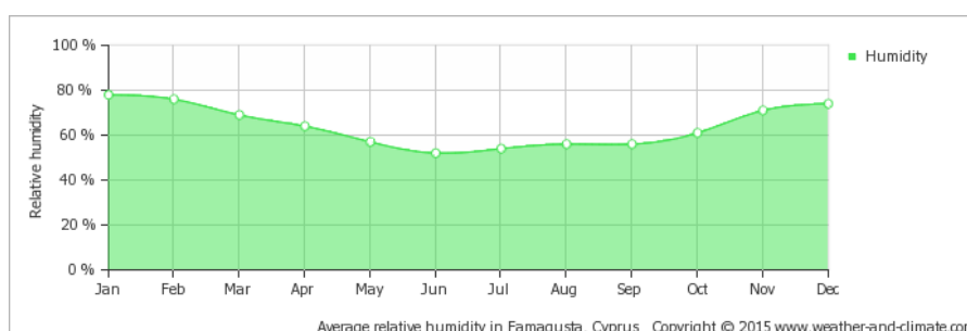
Figure 26. Average monthly humidity in Famagusta. http://www.weather-and-climate.com/average-monthly-Rainfall-Temperature-Sunshine,Famagusta,Cyprus , (2015)
