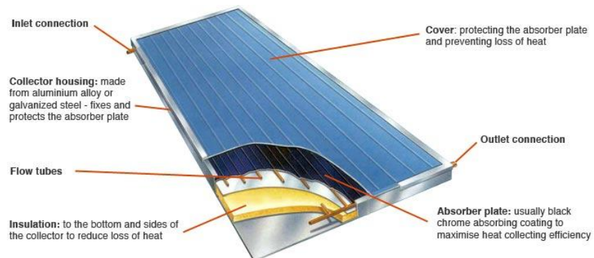
Figure 4. Parts of flat plate solar thermal collector http://mcensustainableenergy.pbworks.com/f/1260939446/solarcol2.jpg
