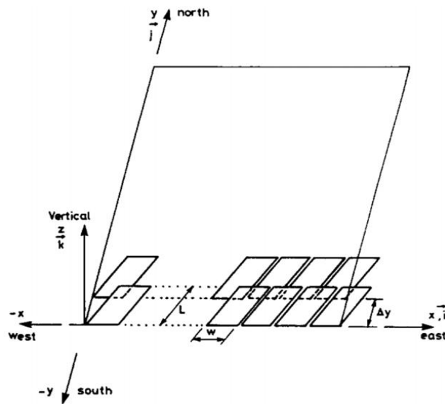
Figure 48. Collectors field geometry
