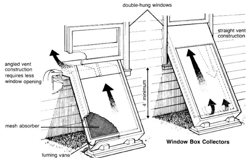
Figure 3. Window box of air based collector. http://www.exposingtruth.com/wp-content/uploads/2013/08/Solar_Air_Window_Box_Collectors.gif
