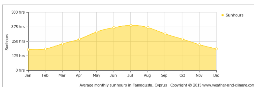
Figure 25. Average monthly hours of sunshine in Famagusta. http://www.weather-and-climate.com/average-monthly-Rainfall-Temperature-Sunshine,Famagusta,Cyprus , (2015)
