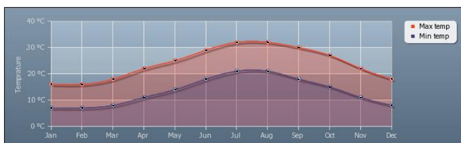
Figure 24. Maximum & minimum annually average temperature in Famagusta. URL: http://www.weather-and-climate.com/average-monthly-Rainfall-Temperature-Sunshine,Famagusta,Cyprus .
