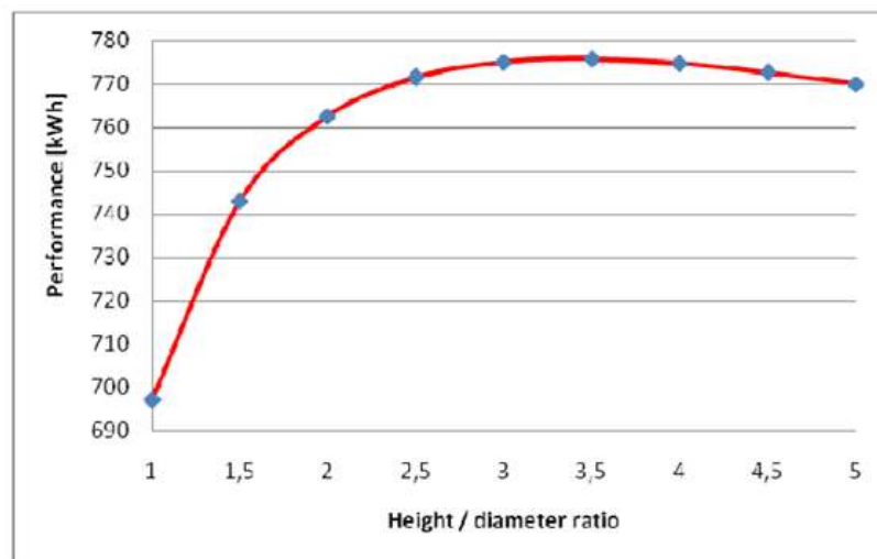
Figure 51. The impact of height/diameter ratio on performance of solar thermal system (Skalik,2014)
