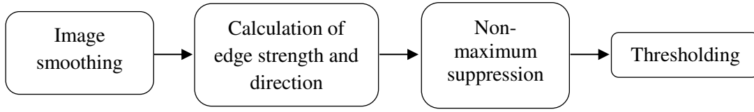
Figure 1.12: steps of canny edge detector
