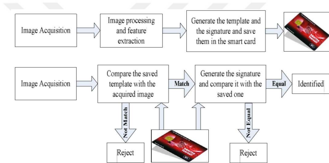
Figure 2.15: The block diagram of the designed system [103]
