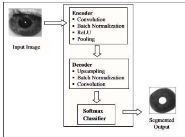
Figure 2.10: The proposed system for iris segmentation [92]
