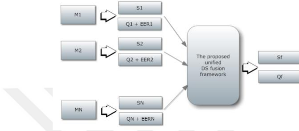
Figure 2.16: Combining multiple sources of evidence using DS theory [107]
