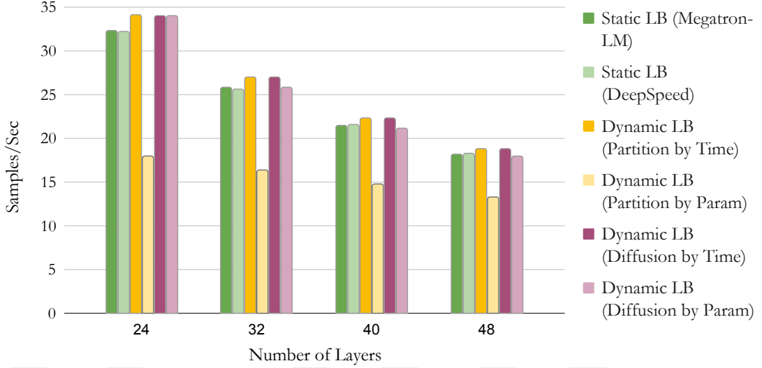
Figure 4.1: End-to-end training throughput (samples/sec) comparison for different balancer types where the target sparsity is 90% in a gradual pruning setting. Time-based dynamic load balancers outperform the baseline static load balancers and dynamic parameter-based load balancers in all model sizes. Higher is better.
