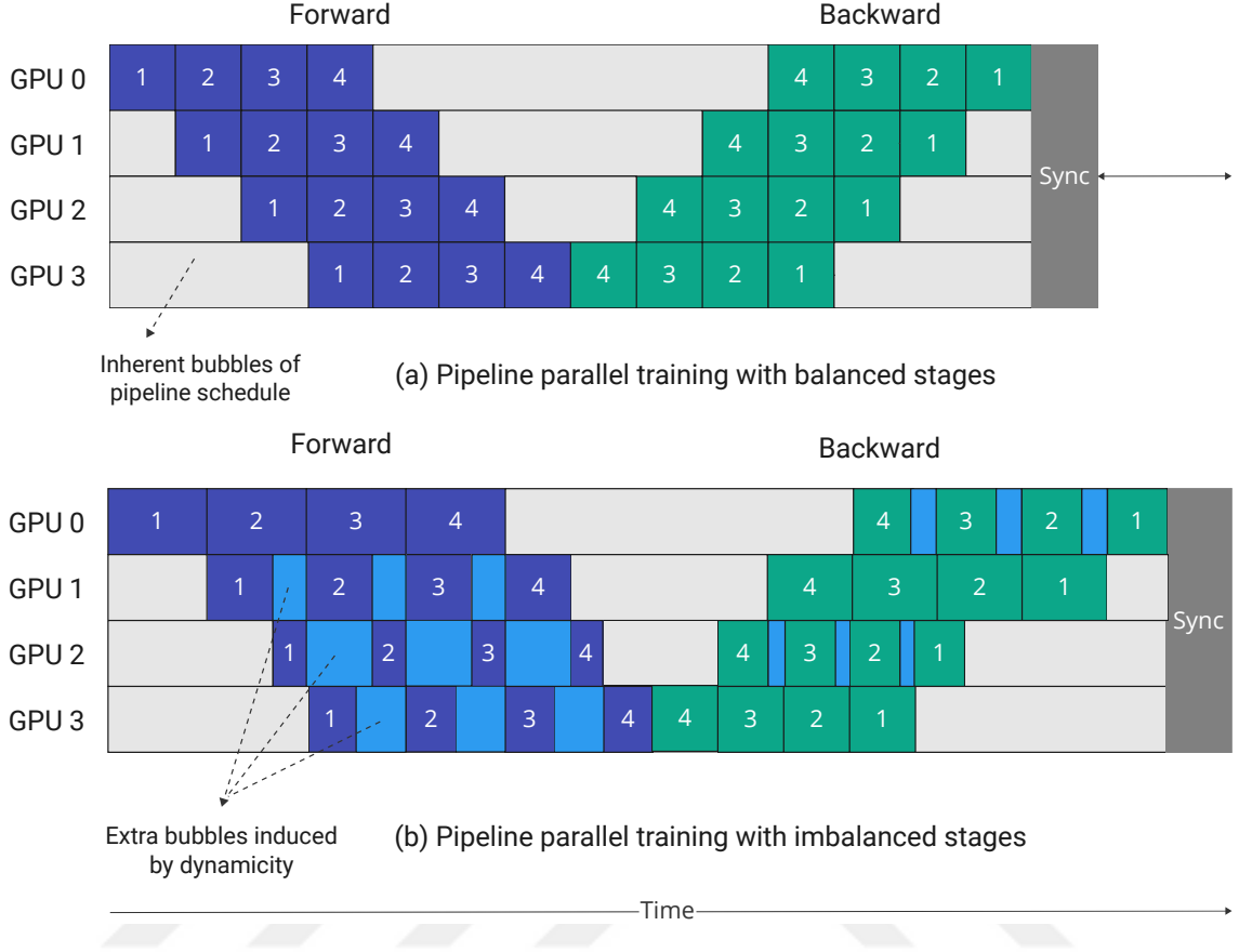
Figure 2.1: Bubble types in a pipeline with 4 microbatches. Inherent bubbles in the pipeline are shown in gray and bubbles introduced by dynamicity (e.g. sparsity) are shown in light blue.
