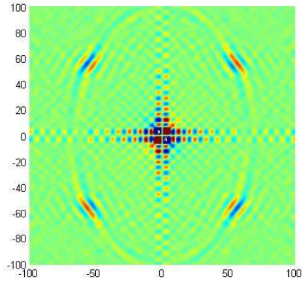
(a) E_1^3(x_1, 0, x_3, 50/c)
