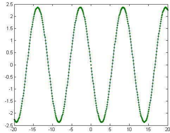
Figure 4.70: Graphs of \tilde{\mathcal{H}}_1^3(z,t) and \tilde{H}_1^3(z,t) . The dotted line represents \tilde{H}_1^3(v,t)(z,t) at t = 1/c (our method ). The continuous line represents \tilde{\mathcal{H}}_1^3(z,t) at t = 1/c (the explicit formula ( 4.224)).
