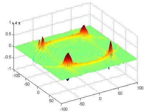
(b) H_2^3(x_1, 0, x_3, 50/c)
