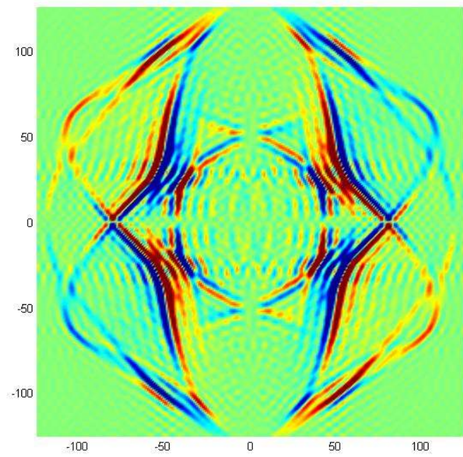
Figure 3.63: The map surface plot (plan) of 3D surface z = w_2^6(0, x_2, x_3, 0.15) in Al-Cu-Li .
