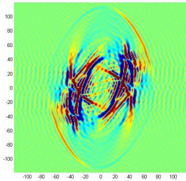
Figure 3.56: The map surface plot (plan) of 3D surface z = w_1^3(x_1, 0, x_3, 0.3) (triclinic crystal).
