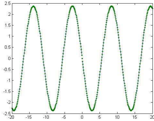
Figure 4.71: Graphs of \tilde{\mathcal{H}}_2^3(z, t) and \tilde{H}_2^3(z, t) . The dotted line represents \tilde{H}_2^3(v, t)(z, t) at t = 1/c (our method). The continuous line represents \tilde{\mathcal{H}}_2^3(z, t) at t = 1/c (the explicit formula (4.224)).
