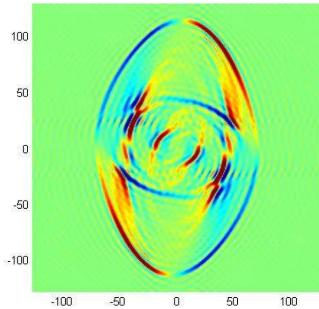
Figure 3.37: The map surface plot (plan) of 3D surface z = u_1^4(x_1, 0, x_3, t) for t = 2 in triclinic QC
