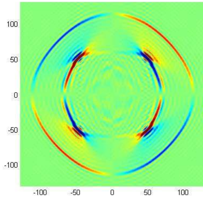
Figure 3.29: The map surface plot (plan) of 3D surface z = u_1^3(x_1, 0, x_3, t) for t = 0.8 in trigonal QC
