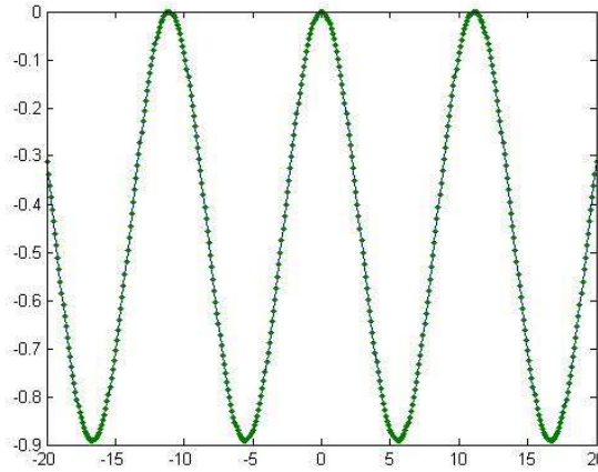
Figure 4.68: Graphs of \tilde{E}_j^3(z,t) and \tilde{E}_j^3(z,t) . The dotted line represents \tilde{E}_j^3(v,t)(z,t) at t = 1/c (our method). The continuous line represents \tilde{E}_j^3(z,t) at t = 1/c (the explicit formula (4.223)), j = 1, 2 .
