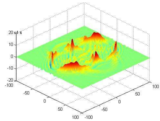
(b) H_2^3(x_1, x_2, -\sqrt{1/3}x_1, 1/c)
