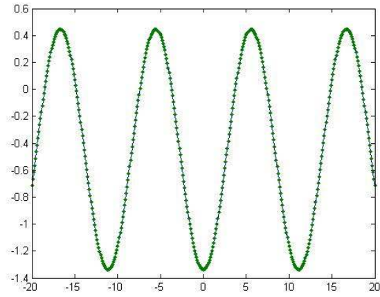
Figure 4.69: Graphs of \tilde{\mathcal{E}}_3^3(z,t) and \tilde{E}_3^3(z,t) . The dotted line represents \tilde{E}_3^3(v,t)(z,t) at t = 1/c (our method ). The continuous line represents \tilde{\mathcal{E}}_3^3(z,t) at t = 1/c (the explicit formula ( 4.223)).
