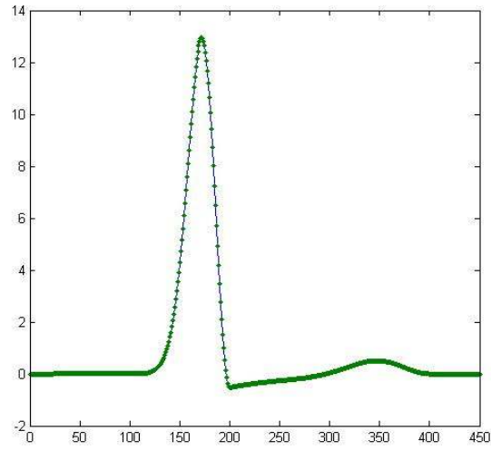
Figure 2.14: Graphs of the third component u_3^3(\sqrt{6}z/4, \sqrt{6}z/4, z/2, t) of solutions (2.84), (2.85) for h(t) = \theta(t)t^2 \exp(-3t^2) at t = 5\sqrt{\frac{\rho}{\mu}} for an isotropic solid with wave speed quotient C_L/C_T = 2 . The dotted line represents analytical solution found by (2.109). The continuous line represents our method.
