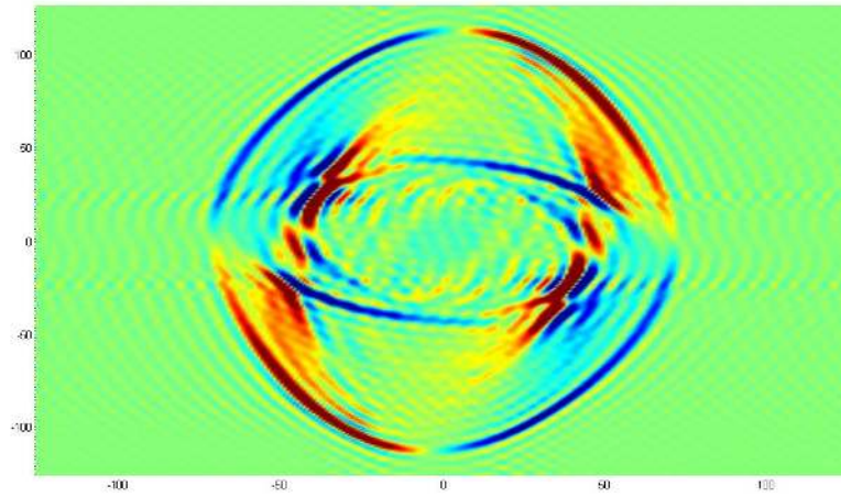
Figure 2.10: 2- D plot of the first component of the displacement \mathbf{u}^3(x_1, 0, x_3, t) for t = 0.3 in albite (triclinic structure of anisotropy)
