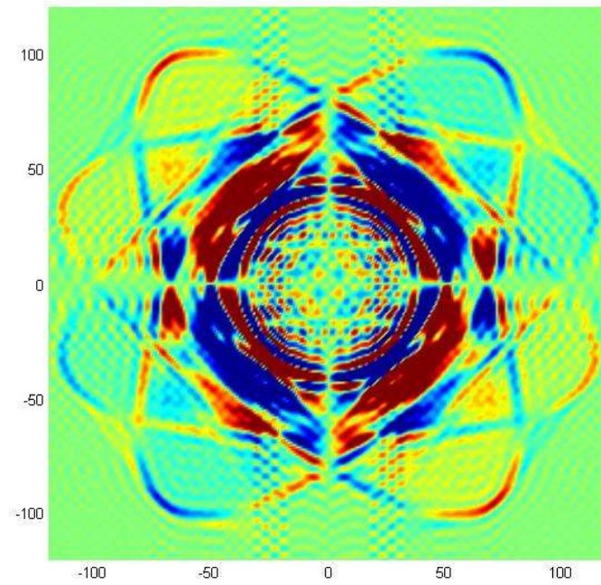
Figure 3.59: The map surface plot (plan) of 3D surface z = w_2^3(x_1, x_2, 0, 0.15) in Al-Cu-Li.
