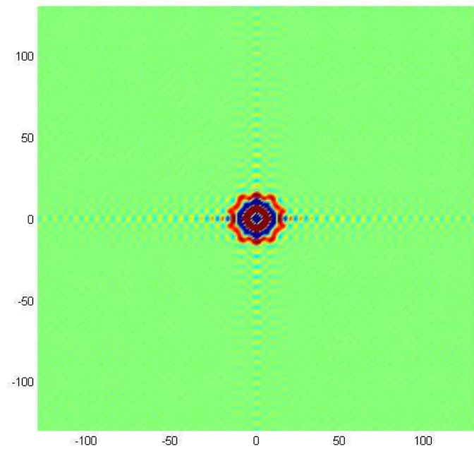
Figure 3.64: The map surface plot (plan) of 3D surface z = w_3^6(x_1, x_2, 0, 0.02) in Al-Cu-Li .
