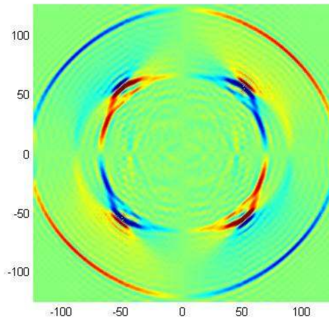
Figure 3.31: The map surface plot (plan) of 3D surface z = u_1^3(x_1, 0, x_3, t) for t = 1.75 in tetragonal QC
