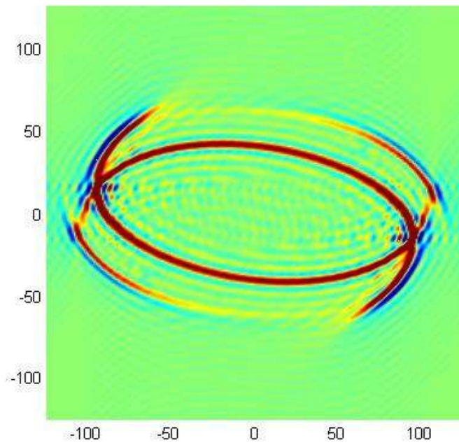
Figure 3.38: The map surface plot (plan) of 3D surface z = w_3^4(x_1, 0, x_3, t) for t = 1.5 in triclinic QC
