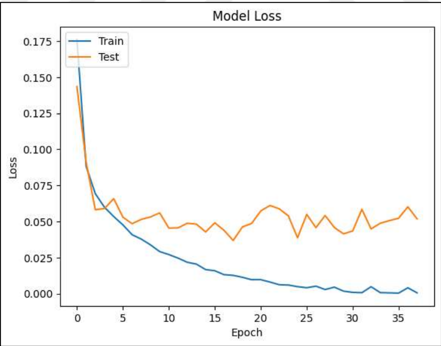
Figure 4.2: Loss Curve for the Neural Network.
